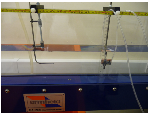
(a) Kiel-reverse and the reference Pitot-tube: setting for calibration (b) Hydraulic jump for simulating surge effects of the pipeline environment.
