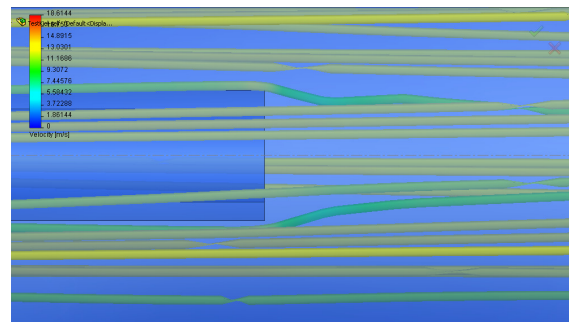
(b) Design A, wake of the pressure tap. Curved lines, adhering to the tap contour, are responsible for the lower static pressure compared with the real one
