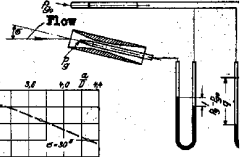
Figure 4.5.- Variation of total-pressure error with angle of attack for cylindrical tubes with different size impact openings. M = 0.26 . (Adapted from ref. 4.)
