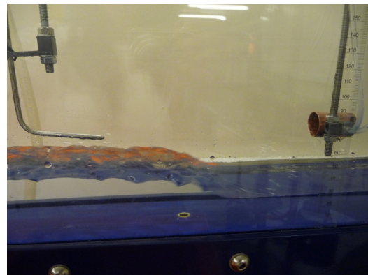
(a) Kiel-reverse and the reference Pitot-tube: setting for calibration (b) Hydraulic jump for simulating surge effects of the pipeline environment.
