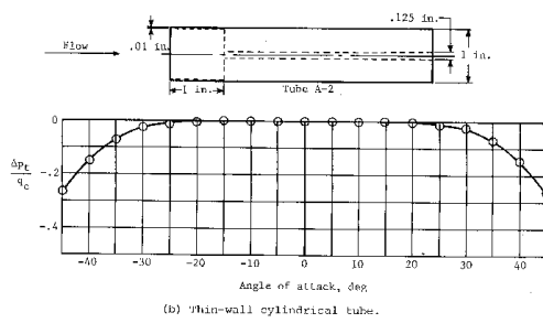
Figure 4.5.- Variation of total-pressure error with angle of attack for cylindrical tubes with different size impact openings. M = 0.26 . (Adapted from ref. 4.)
