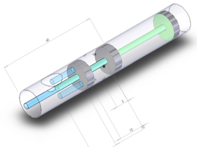
(b) Pitot-Gracey Probe design inert structure of static pressure chamber, enclosed by the two grey seals, and surrounded by the static holes. The grey seal in the front is to lower the sensibility of the probe to misalignments.
