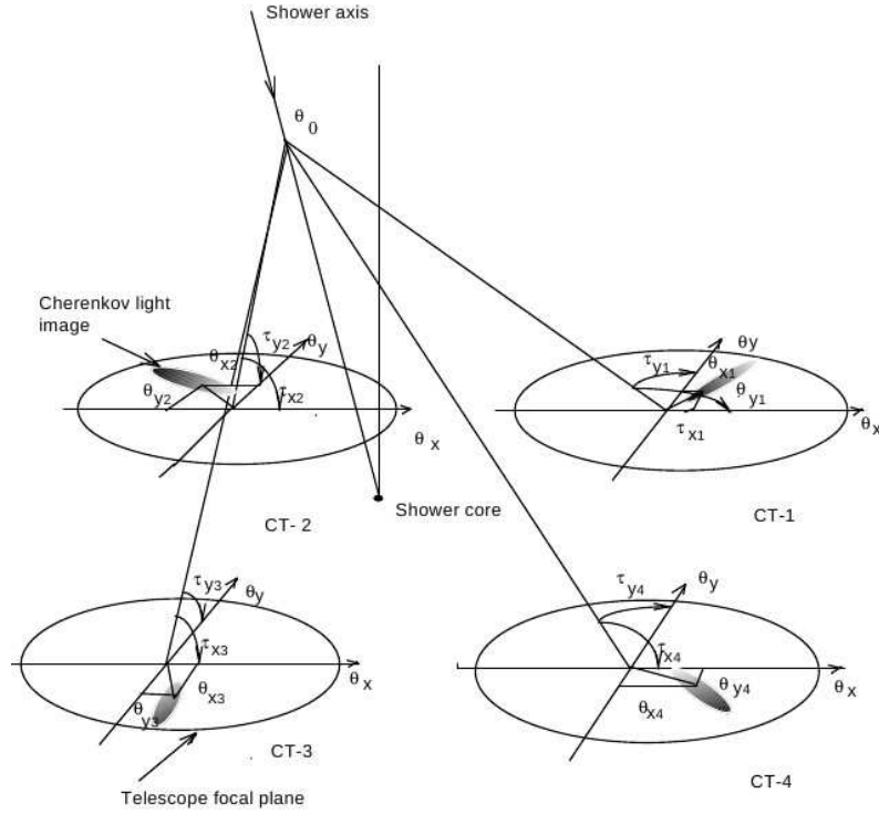
Figure 2.14: Reconstruction of the shower parameters from stereoscopic observations of 4 IACTs. Credits: Aharonian & Konopelko [9].
