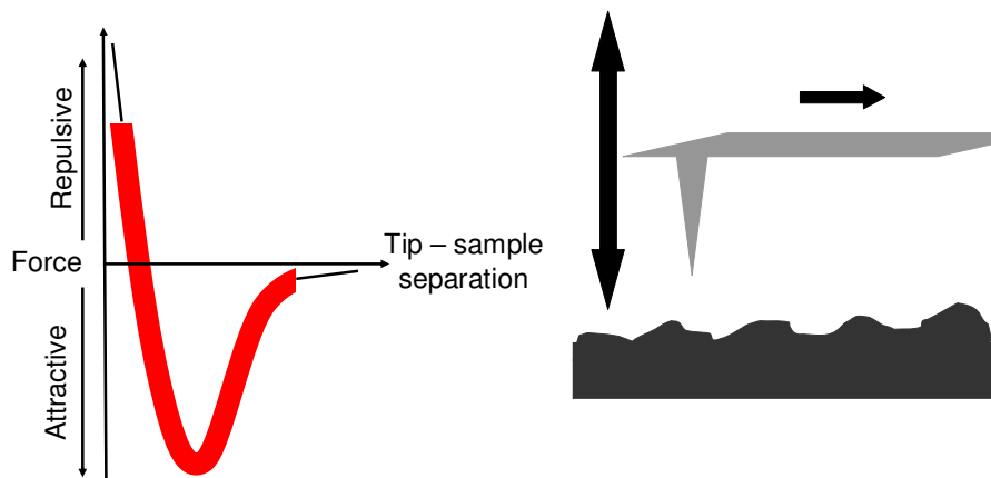
Scheme 1.12: Forces acting upon the AFM probe as a function of probe tip-to-sample separation with attractive and repulsive forces active during intermittent contact mode highlighted (left) and probe movement over the substrate surface (right).
