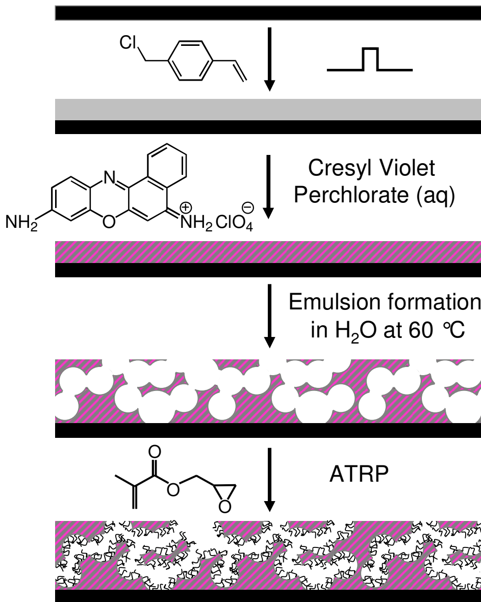
Scheme 4.1: Formation of porous pulsed plasma deposited poly(vinylbenzyl chloride) films by seeding with cresyl violet perchlorate, followed by spontaneous emulsion formation in water at elevated temperature (60 °C), and then additional surface functionalisation of pores (e.g., ATRP).
