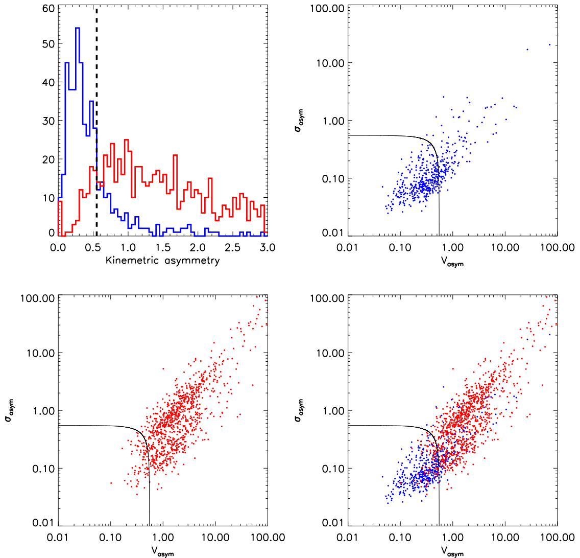
Figure 6.2: Here we compare the kinematic asymmetries of our model disks with the asymmetries of all models which are not disks (both non-disks and mergers. Top Left - A histogram of the total kinematic asymmetry for disk models (blue) and non-disk/merger models (red). The disk models show a clear drop off at a kinematic asymmetry of K_{asym} = 0.55 (shown by the dashed line), which is consistent with the value found by Shapiro et al. (2008). Top Right - Here we show a plot of the asymmetry in the mean velocity field against the asymmetry in the velocity dispersion field for the disk models. The line shows the cut of of K_{asym} = 0.55 , which most of the disk models fall below. Bottom Left - A plot of the asymmetry in the mean velocity field against the asymmetry in the velocity dispersion field for the non-disk and merger models (mergers and non-disks). The line shows the cut of of K_{asym} = 0.55 , which most of the models which are not disks lie above. Bottom Right - Asymmetry in mean velocity field and velocity dispersion field for both the disks (blue) and non-disks/mergers (red). The line shows the cut off of K_{asym} = 0.55 which clearly separates the two distributions.
