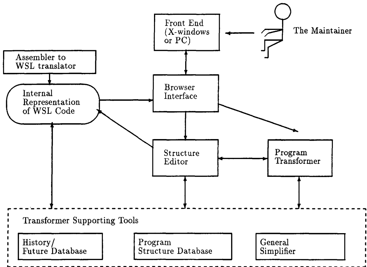
Figure 2.1: The Architecture for the Maintainer's Assistant
