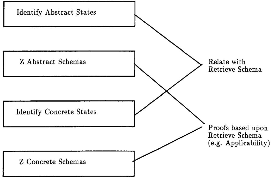
Figure 3.1: The IBM Hursley Park Method
