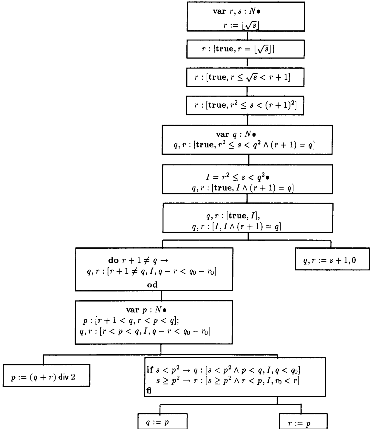
Figure 4.1: Morgan's refinement of the square root problem
