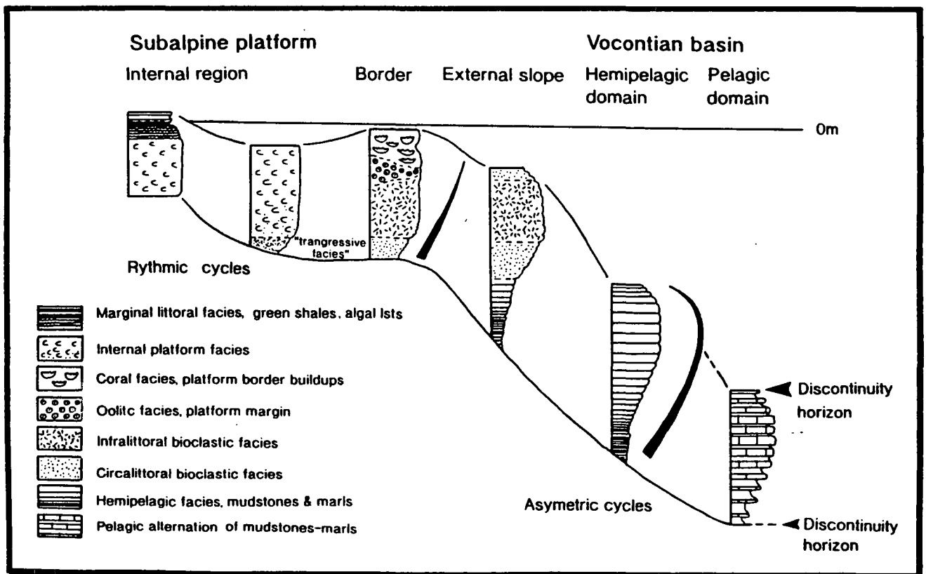
Fig. 3.4a Vertical and lateral arrangement of facies within the Urgonian. From Arnaud-Vanneau et al. (1987). This figure illustrates the rapid development of platform facies (F5 to F11) within the internal regions compared to the margin and external slope where inner platform facies never developed. Note: true reef barriers never developed on the platform margin border. Fig. 3.4b (opposite page) Comparison of the sequence stratigraphic schemes of Jaquin et al. (1991) and Hunt (1992) developed for the Urgonian of the northern Vercors and southern Chartreuse. Sb = sequence boundary, mfs = maximum flooding surface, TST = transgressive sequence tract, HST = highstand sequence tract. Figure courtesy of D. Hunt.
