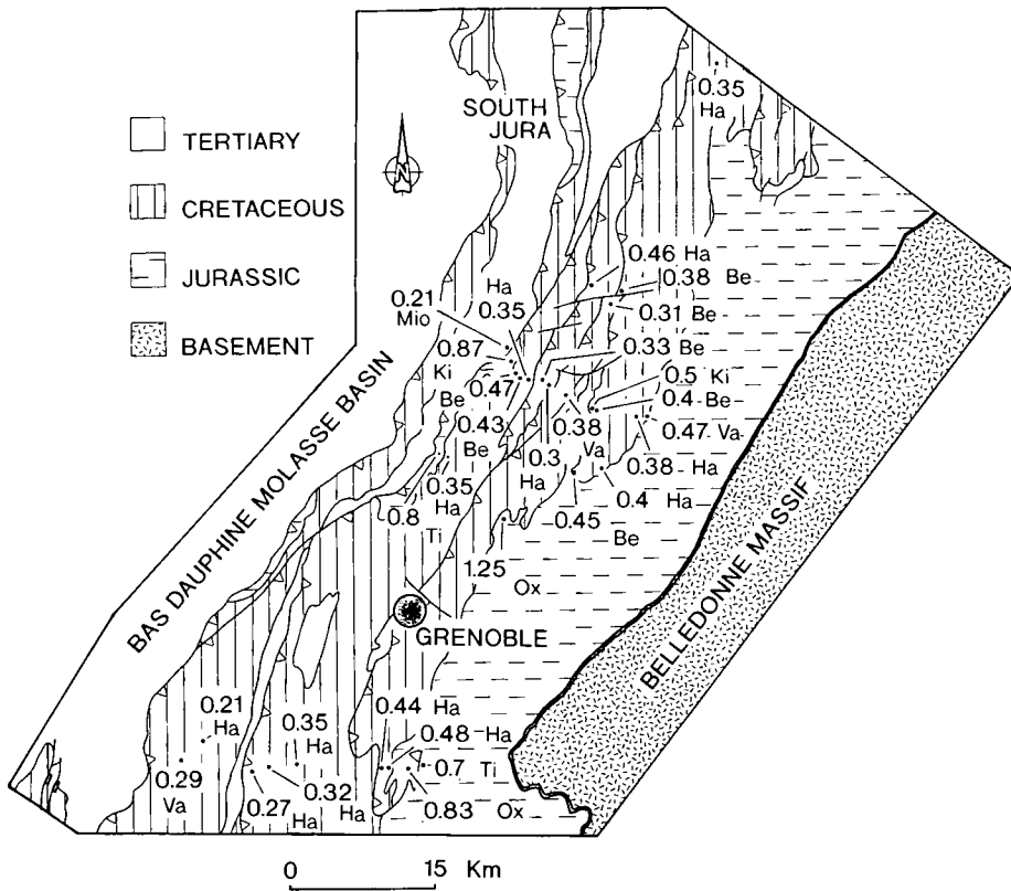
Fig. 3. Mean R_0 (%) values for the southwest study area of the French Subalpine Chains. Stratigraphic ages of the samples used for the determinations are indicated by abbreviations: Mio, Miocene; Ha, Hauterivian; Va, Valangian; Be, Berriasian; Ki, Kimmeridgian; Ti, Tithonian; Ox, Oxfordian.
