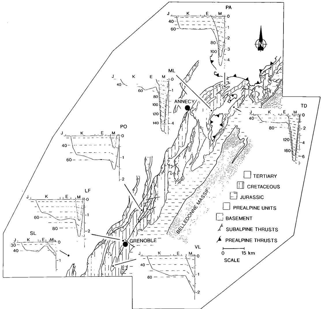
Fig. 7. Burial history models for several locations throughout the Subalpine Chains. The lower of the two horizons modelled (unornamented area) is the base of the Lower Cretaceous Hauterivian mudstones, and the upper horizon (stippled area) is the inferred Tertiary load (foredeep sediments and/or tectonic loads). Ages (horizontal axes) are as follows: J, Jurassic; K, Cretaceous; E, Eocene; M, Miocene; depths (vertical axes) are in kilometres. Temperature contours (dashed lines on the models) are shown in degrees centigrade. These were generated at the same time as the burial history models using the conditions shown in Table 3. Locations are as follows: TD, Combe de Tardevant, Aravis massif; PA, Plateau d'Andey, Bornes massif; ML, Mont Lachat, Bornes massif; PO, Pic d'Oeilette, Chartreuse massif; LF, La Fontanil, southern Chartreuse massif; SL, St Lattier borehole, Romans region, western Vercors massif; VL, Villard-de-Lans, Vercors massif. Timescale from Haq et al. (1987).
