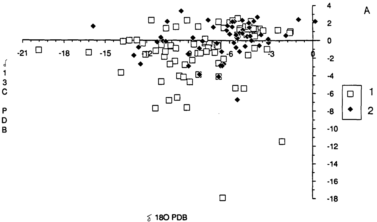
Fig. 5.17a Isotope plot of all veins. 1= veins within the Urganian; 2= veins within non-Urganian strata. Fig. 5.17b Sr^{2+} versus Mn^{2+} for all veins. Key as for 5.17a. Fig. 5.17c Fe^{2+} and Mn^{2+} plot for all veins. Key as for 5.17a. Fig. 5.17d Sr^{2+} versus \delta^{18}O PDB plot for all veins. Key as for 5.17a. See opposite page for Figs 5.17c and 5.17d.
