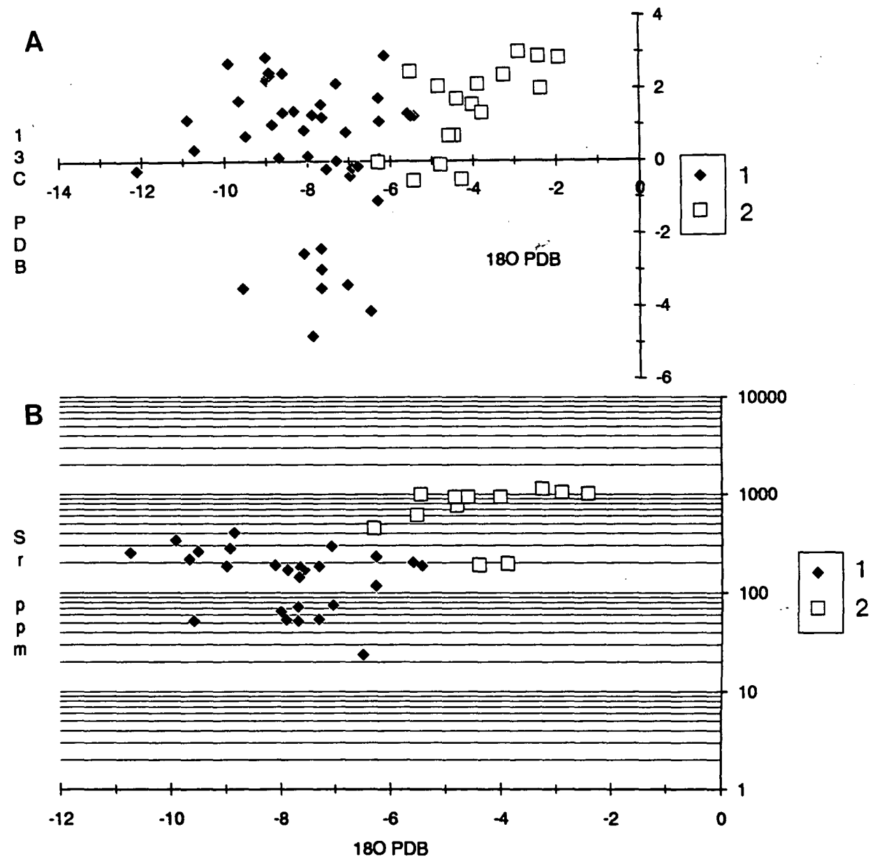
Fig. 4.16a Comparison of the stable isotope composition of rudist shells and equant burial cements. The depletion in the \delta^{18}O value and in ^{13}C (in some cases) of the equant cements reflects the increased temperature of precipitation and the incorporation of light CO_2 from organic maturation in some cases. 1= cements; 2= rudist shells. Fig. 4.16b Comparison of the \delta^{18}O composition versus Sr concentration for rudist shells and equant cements. 1= cements; 2= rudist shells.
