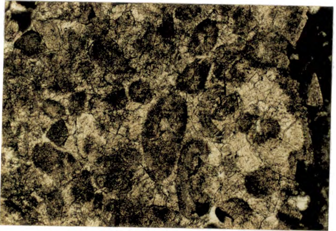
Fig. 3.36 Poor mimetic replacement of a grainstone by hypidiotopic mosaic dolomite. 368/90, Dents d'Arclusaz, Bauges. Field of view= 3.25mm.
