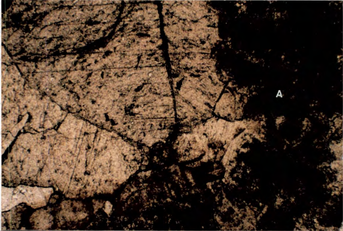
Fig. 3.42a Micritised dolomite rhombs can be seen on the right (area labelled A) and coarse calcite infilling vuggy porosity. 143/90 Gorge du Nant (#6 on Fig. 3.1, see log #3, Appendix 1). Fig. 3.42b Spectacularly zoned calcite infilling intercrystalline porosity around calcitized dolomite rhombs. 143/90 Gorge du Nant (#6 on Fig. 3.1, see log #3, Appendix 1). The dedolomitized rhombs have a bright orange core. On the basis of this distinctive luminescence these areas can be distinguished from the post-dolomite spar. Field of view= 4mm.
