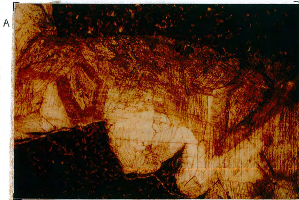
Fig. 5.5a Zoning within a calcite vein fill as revealed by staining. Field of view= 17mm. 210/89, Urgonian, lower Bourne gorge, Vercors. Fig. 5.5b CL shot of zoned calcite within a vein fill. 553/90, Urgonian, Pic de Jallouvre, Bornes. Field of view= 4mm. Fig. 5.5c PPL shot of the same field of view as Fig. 5.4b. Fig. 5.5d Clasts of brecciated wall rock within a vein. 342/90, Nummulite limestone, Tête du Sallaz, Aravis. Field of view= 3.25mm. Figs 5.5c and 5.5d are underneath the foldout.
