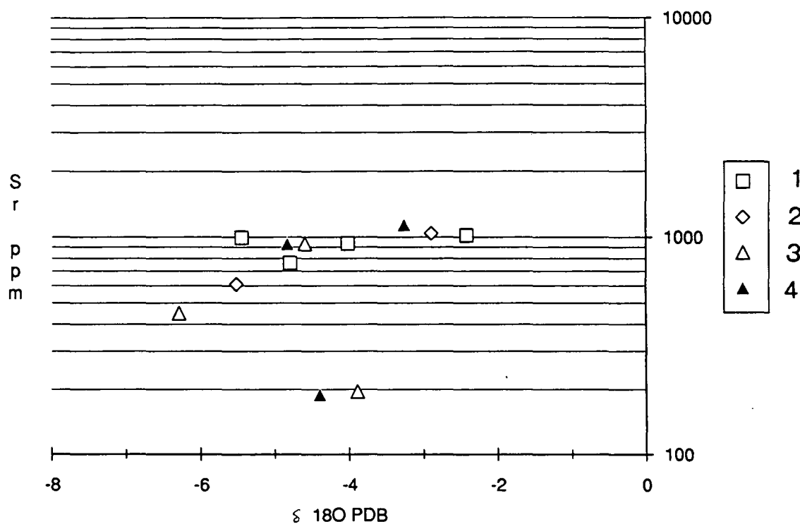
Fig. 4.10 Plot of Sr^{2+} concentration versus \delta^{18}O composition of the same shell samples. A slight correlation can be seen, more depleted ^{18}O values coincide with lower concentrations of Sr^{2+} . Location of samples; 1= Chartreuse; 2= Vercors; 3= Bauges; 4= Aravis.
