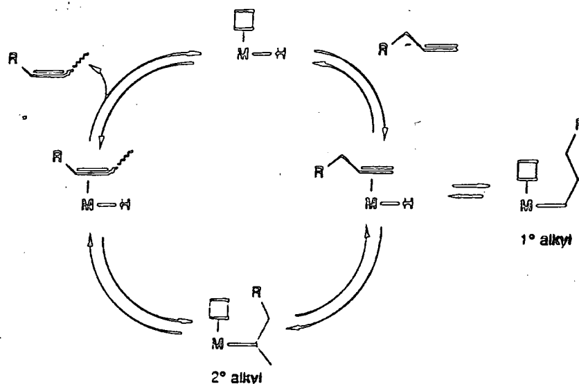
Figure 2.15 Schematic View of Alkene Isomerization
