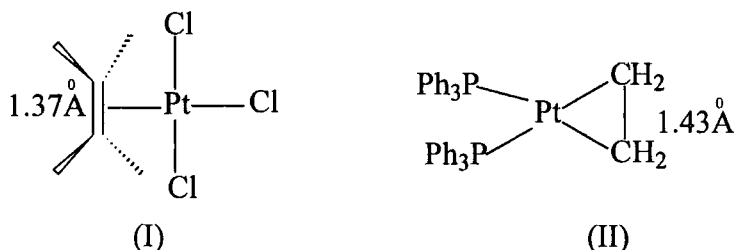
Figure 2.2 Transition Metal-Alkene Complexes
