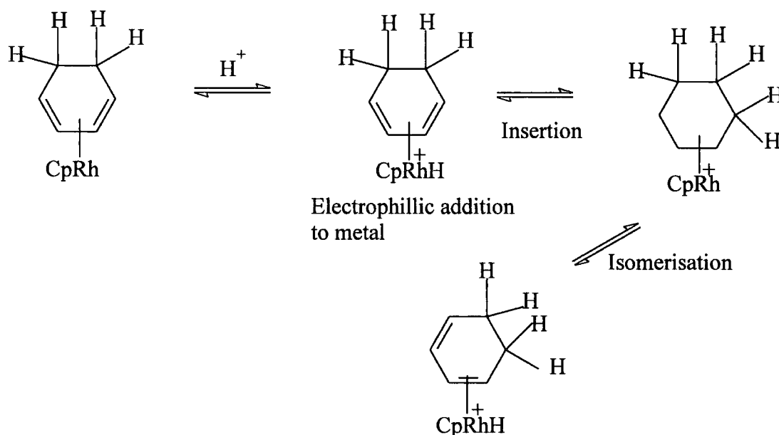
Figure 2.9 Electrophilic Attack at Coordinated Alkene
