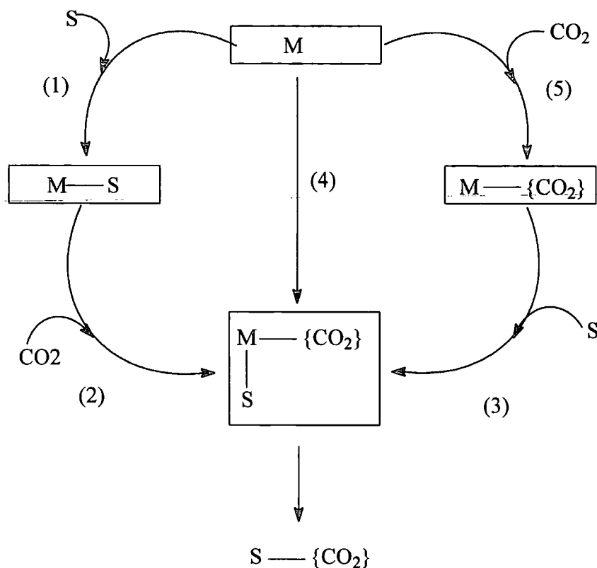
FIG. 1.1 Possible routes for interaction between carbon dioxide(CO 2 ), substrate(S), and transition metal(M).
