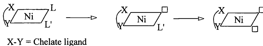
Figure 3.3 Proposed Model for the Formation of Free Coordination Sites in Nickel-Chelate Systems
