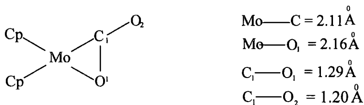
Figure 1.6 Selected X-Ray Crystal Data for Cp 2 Mo(CO 2 )
