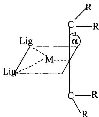
Figure 2.4 Out of Plane Twisting of Substituted Alkenes
