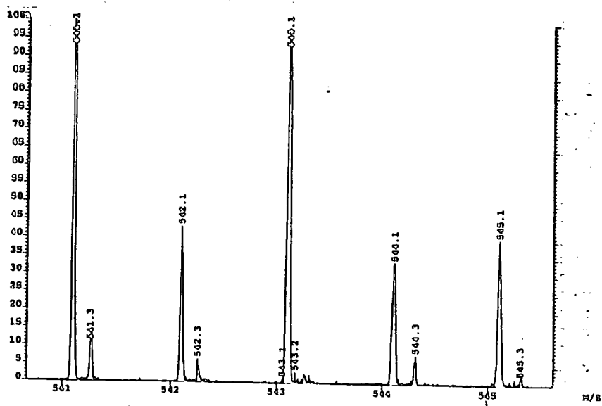
High Resolution Mass Spectrum of M/z 541.
