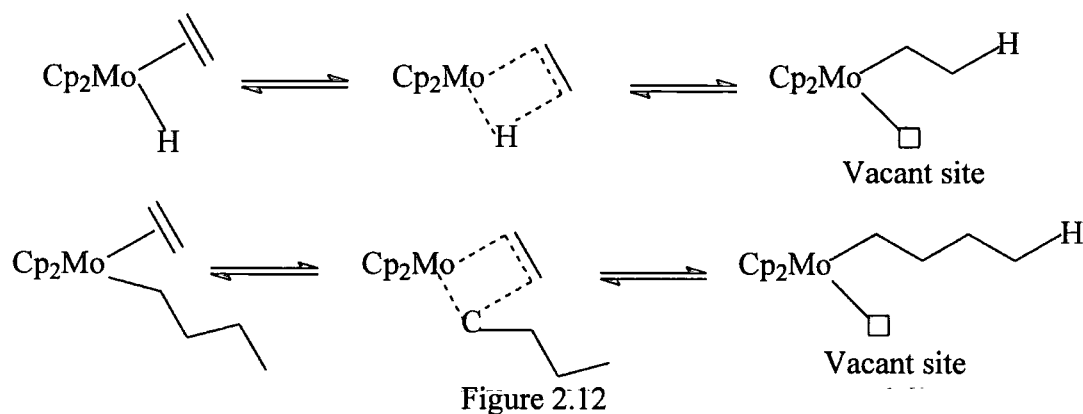
Theoretical Mechanism of Insertion into Metal-Hydride Bond
