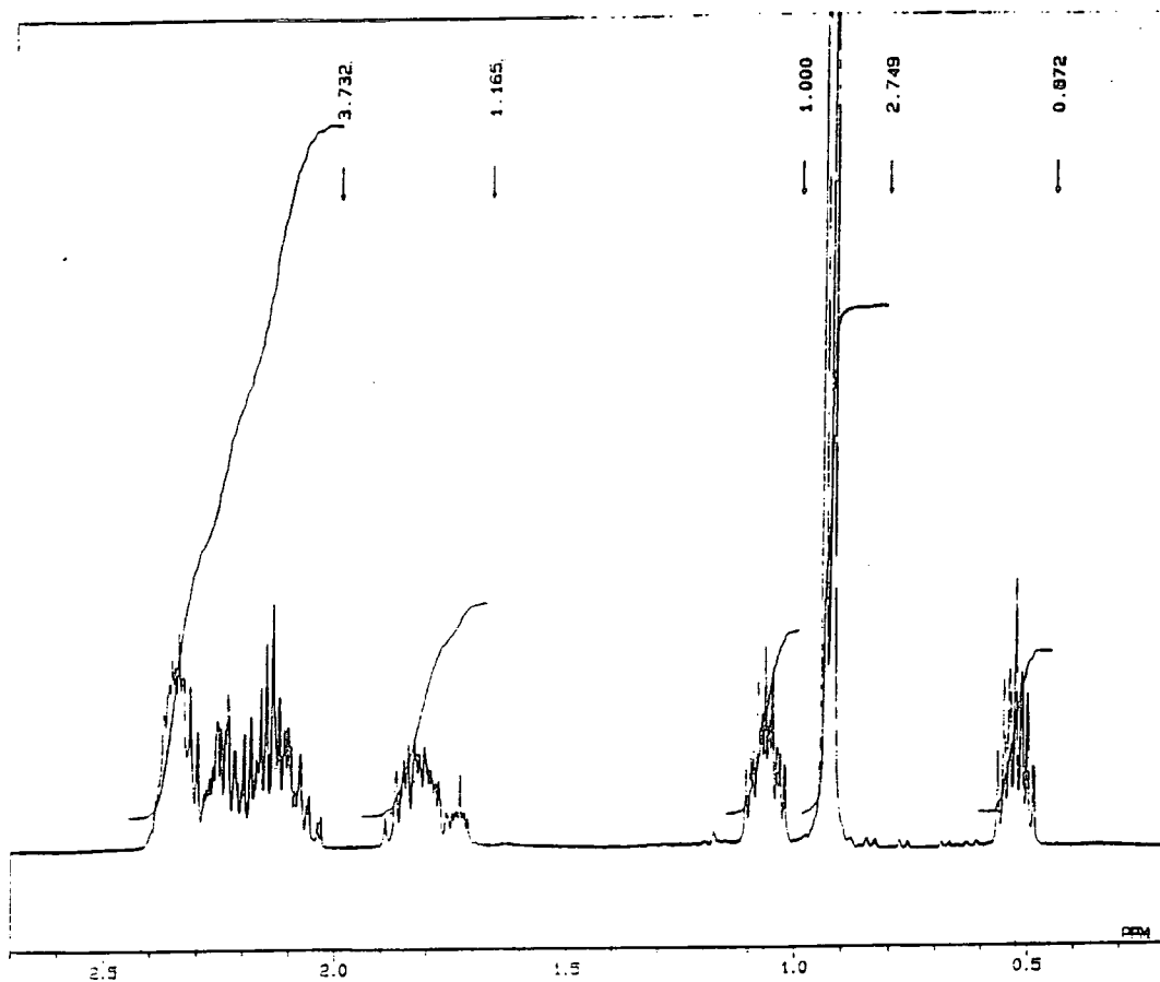
1 H NMR Spectrum of [(DPPE)NiCH 2 CH(CH 3 )COO], (0-2.7ppm).
