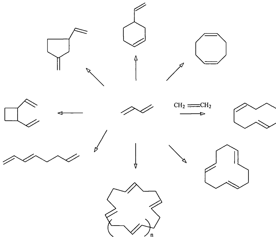
Figure 3.2 Ring Synthesis from Butadiene
