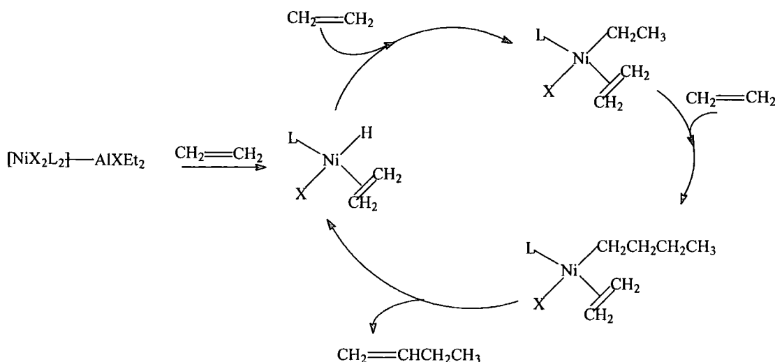
Figure 2.11 Schematic View of Alkene Oligomerization
