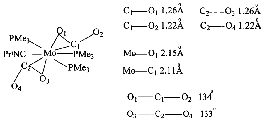
Figure 1.10 Selected X-Ray Crystal Data for Mo(CO_2)_2(PMe_3)_3(CNPr^i)
