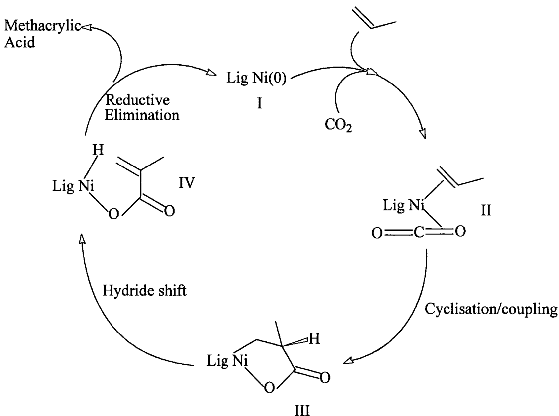
Proposed catalytic cycle for the propene and carbon dioxide oxidative coupling reaction
