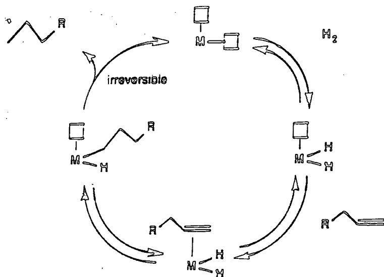
Figure 2.14 Schematic View of Alkene
