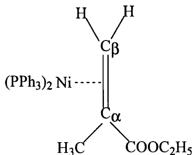
Figure 2.5 Structure of Ni(PPh_3)_2(Ema) , Ema = ethylmethacrylate
