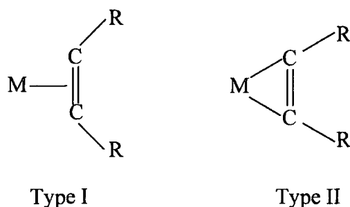
Figure 2.10 Extremes of Metal-Alkyne Bonding
