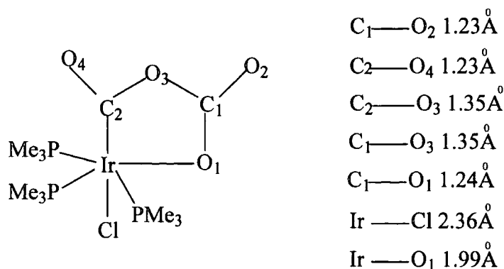
Figure 1.9 Selected X-Ray Crystal Data for \text{Ir}(\text{Cl})(\text{C}_2\text{O}_4)(\text{PMe}_3)_3 \cdot 0.5\text{C}_6\text{H}_6
