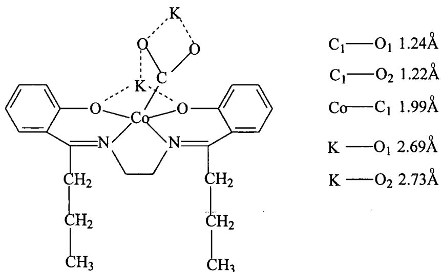
Figure 1.12 Selected X-Ray Crystal Data for Co(pr-salen)K_2CO_2 \cdot THF
