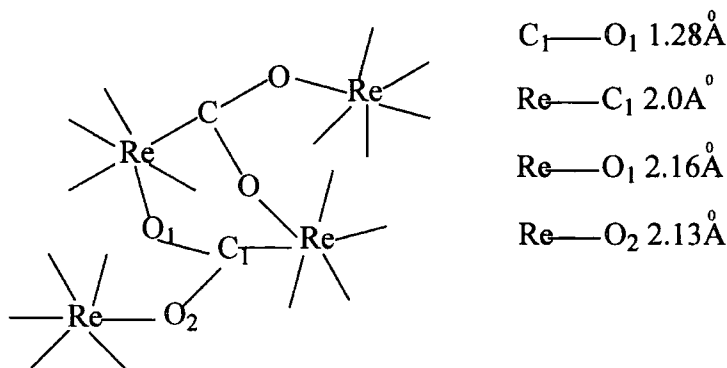
Figure 1.11 Selected X-Ray Crystal Data for Re_4(CO)_{18}(CO_2)_2
