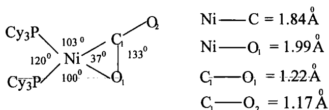
Figure 1.4 Selected X-Ray Crystal Data for \text{Ni}(\text{CO}_2)(\text{PCy}_3)_2 0.75(\text{toluene})
