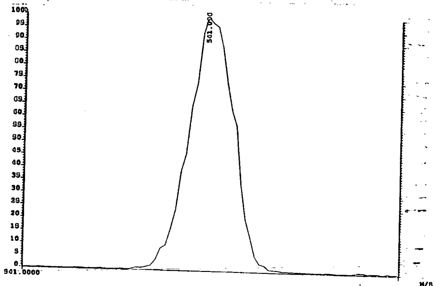
High Resolution Mass Spectrum of M/z 543.
