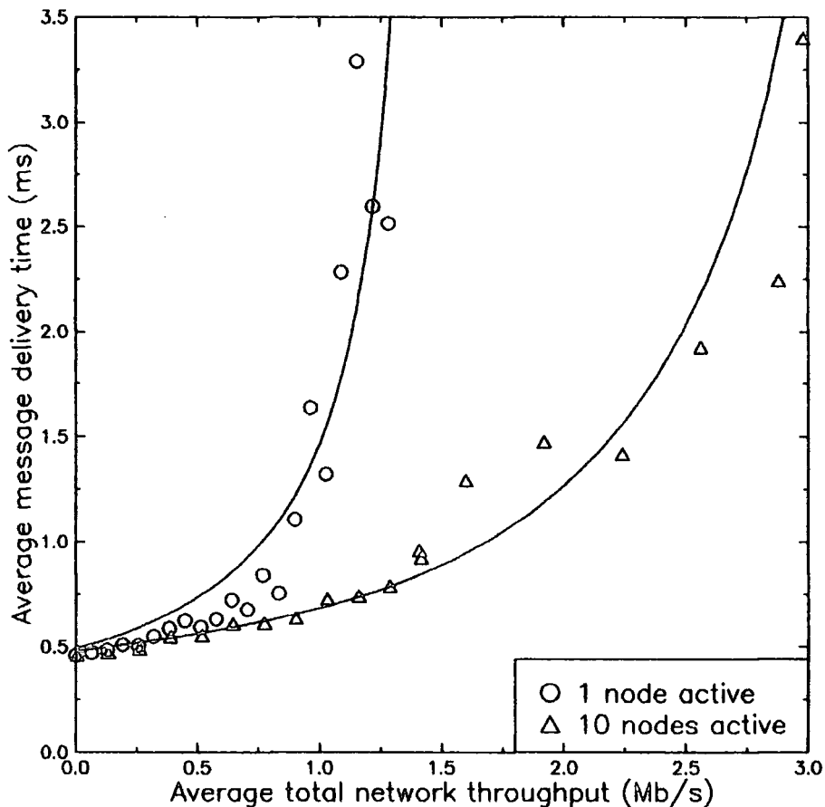
Figure 5.14: Dual ring, 1 packet per message
