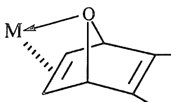
figure 4.12 2,3 substituted 7-oxanorbornadienes
