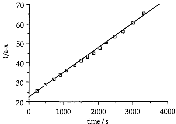
figure 3.14 2nd order plot for chloride-butoxide exchange between \text{CpNb}(\text{NBu}^t)\text{Cl}_2 and \text{CpNb}(\text{NBu}^t)(\text{OBu}^t)_2
