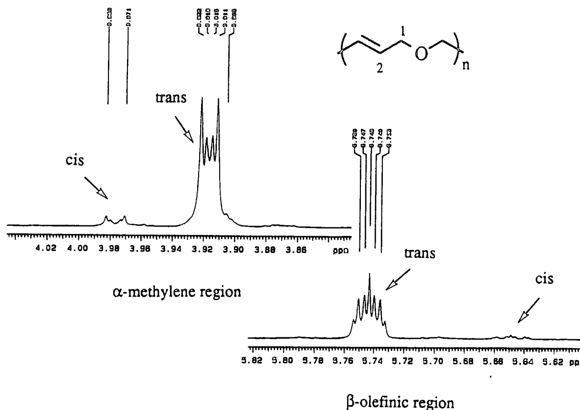
figure 4.3 ^1\text{H} NMR spectrum (400 MHz) of poly(oxy-1-butenylene) (1)
