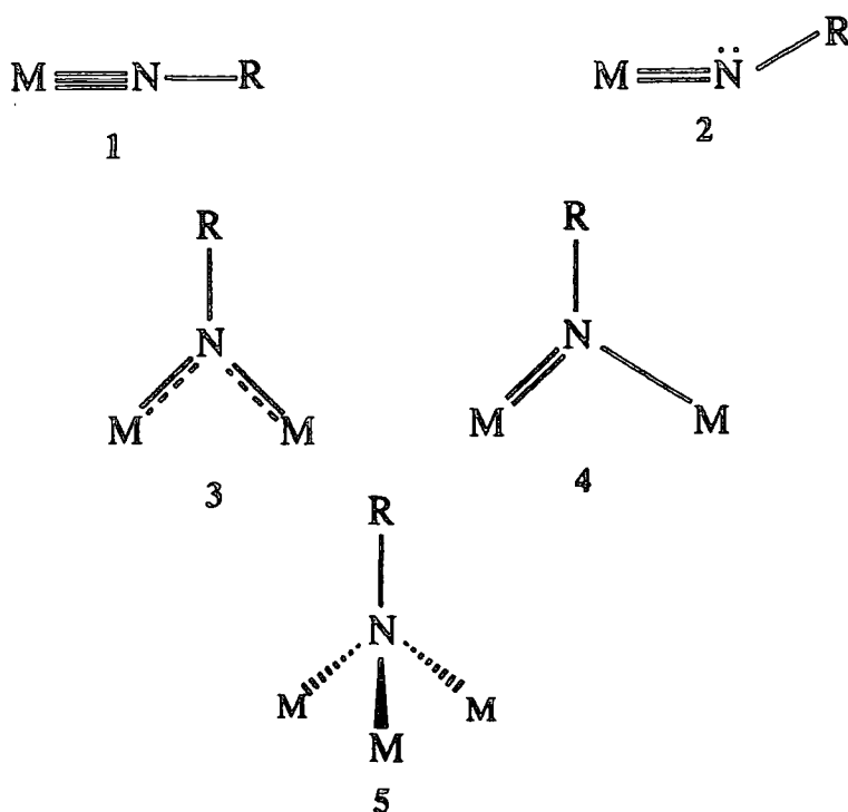
Figure 1.5 Bonding modes of imido ligands.
