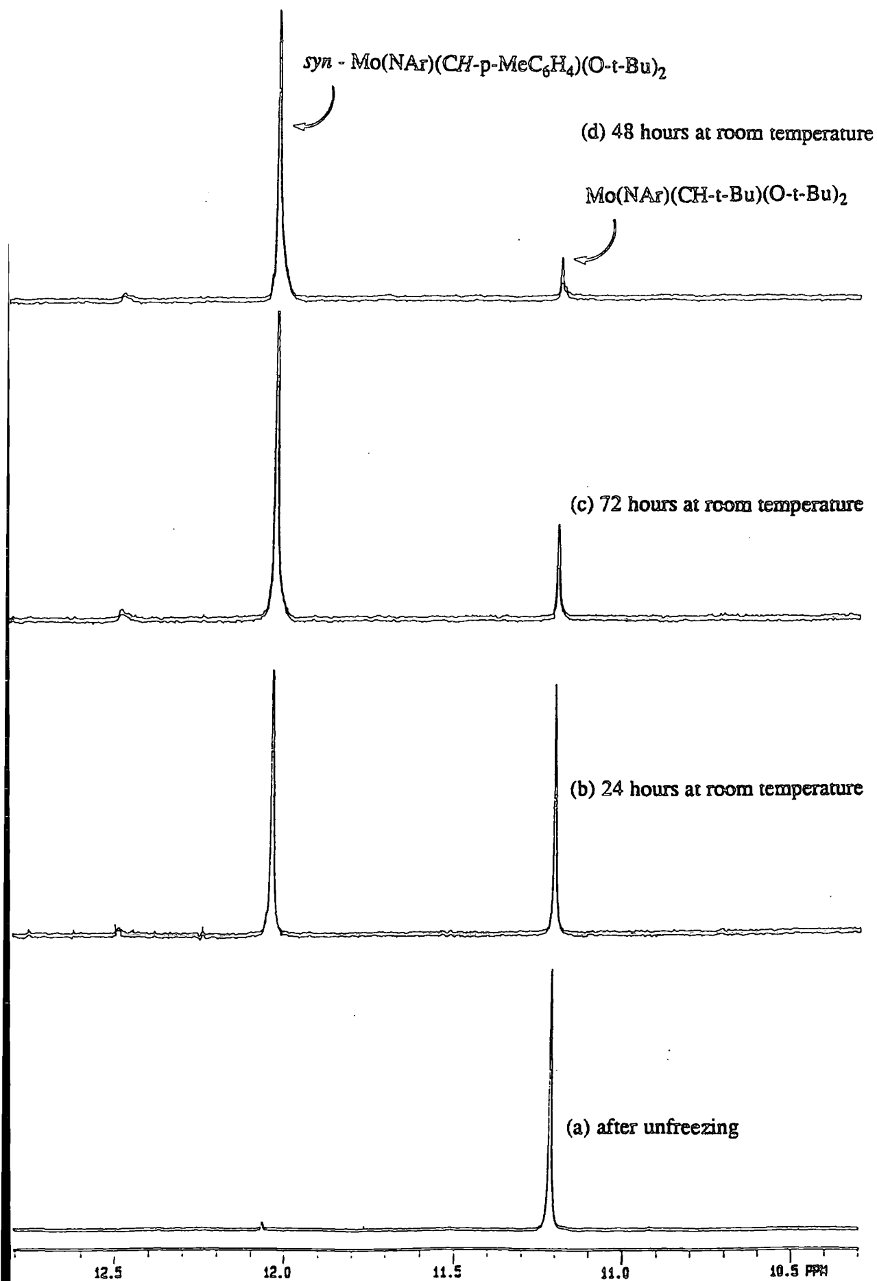
Figure 3.3 Formation of \text{Mo}(\text{NAr})(\text{CH-p-MeC}_6\text{H}_4)(\text{O-t-Bu})_2
