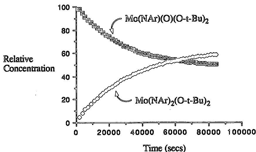
Figure 4.1 Relative Concentrations of (1) and (2) as a function of time at 30°C.
