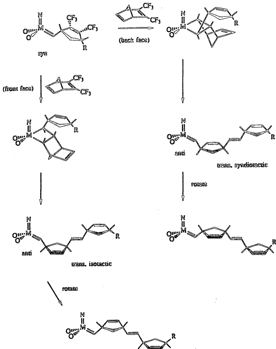
Figure 1.21 Stereoregular polymerization of BTFMND.
