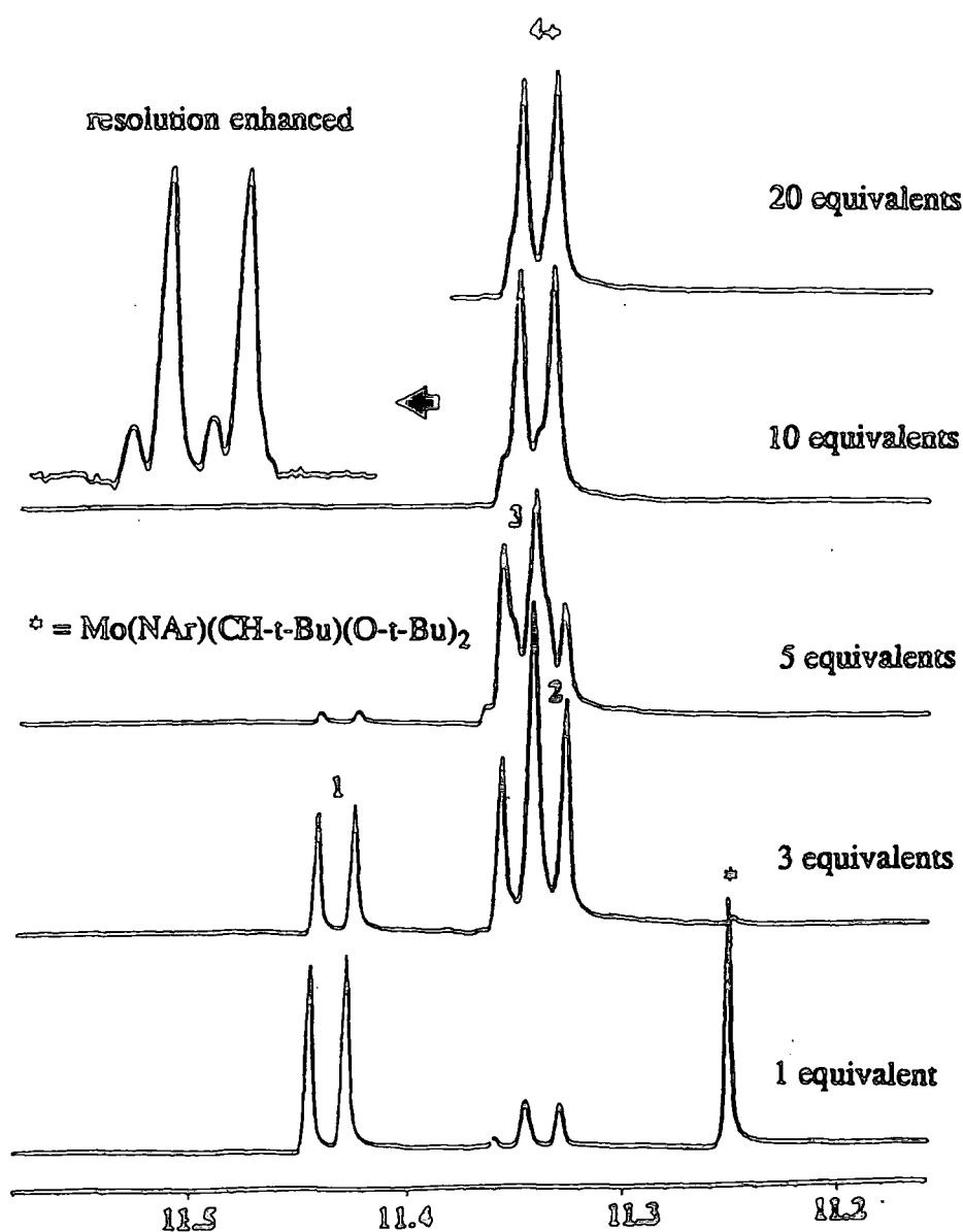
Figure 1.18 ^1\text{H} NMR spectra of \text{Mo(NAr)(CH-t-Bu)(O-t-Bu)}_2 and 1, 3, 5, 10 and 20 equivalents of BTFMND.
