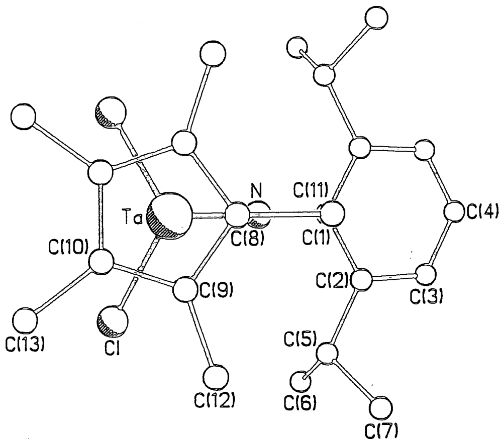
(b) View along the ring centroid-Ta vector
