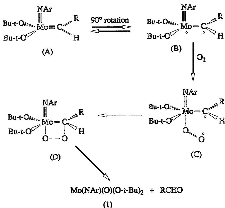
Figure 4.13 A Postulated Mechanism for the reaction of \text{Mo(NAr)(CHR)(O-t-Bu)}_2 with dioxygen.
