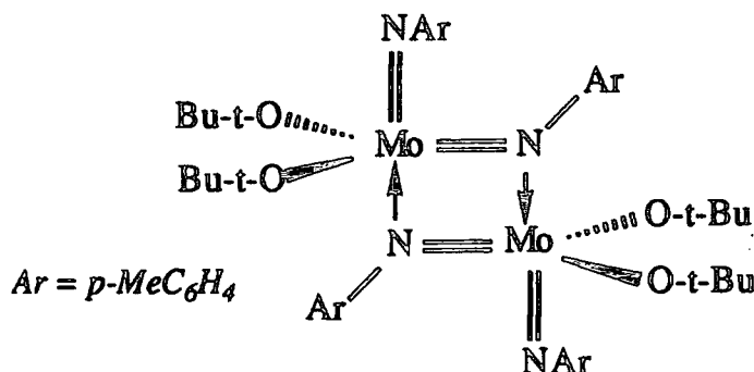
Figure 4.2 Molecular structure of [\text{Mo}(\text{N-}p\text{-tol})_2(\text{O-}t\text{-Bu})_2]_2 .
