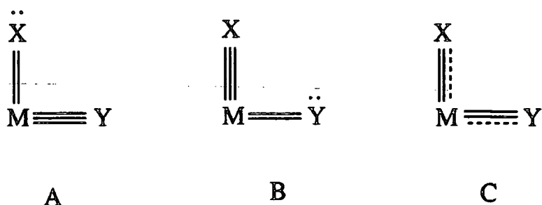
Figure 1.9 Possible bonding modes for M(X)(Y)
