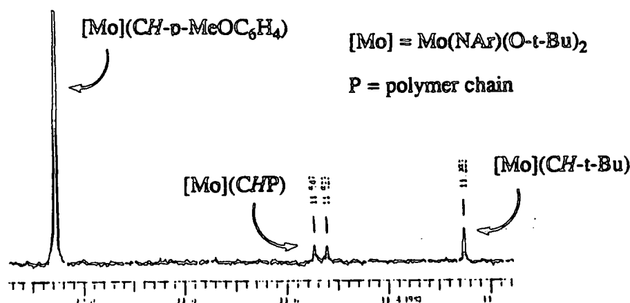
Figure 3.4 Reaction of living polynorbornene with p -methoxystyrene.
