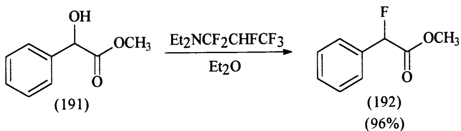
Scheme 107.
