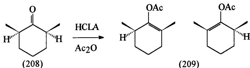
Scheme 112. Reaction of HCLA with cis 2,6-dimethylcyclohexanone
