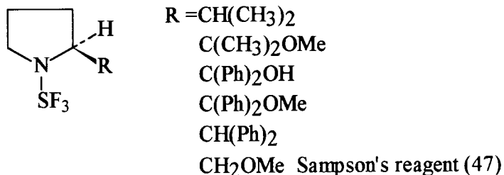
Figure 35. DAST homologues
