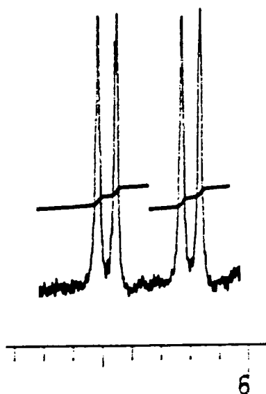
Figure 20. 1 H NMR of racemic (44) in the presence of [Eu(tfc) 3 ]
