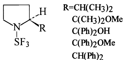
Figure 4. Homologues of DAST
