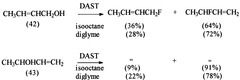
Scheme 24
