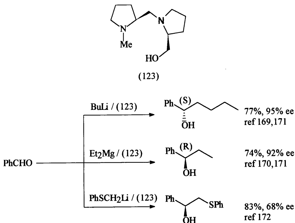
Scheme 72
