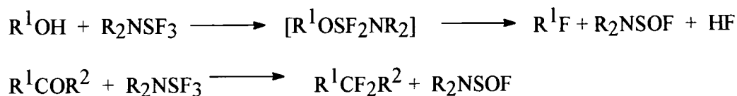
Scheme 20
