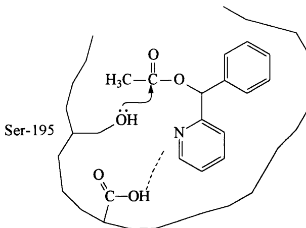
Figure 33. Lipase resolution of 2-( \alpha -acetoxy)benzylpyridine (136)
