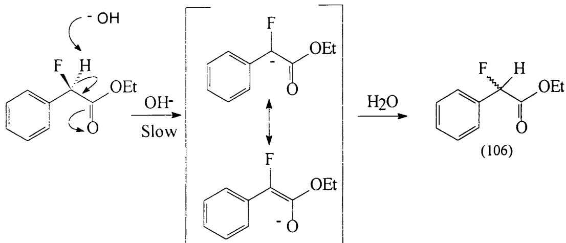
Scheme 62
