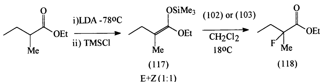
Scheme 68
