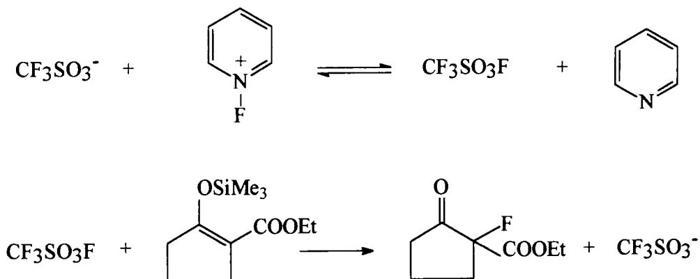
Scheme 71
