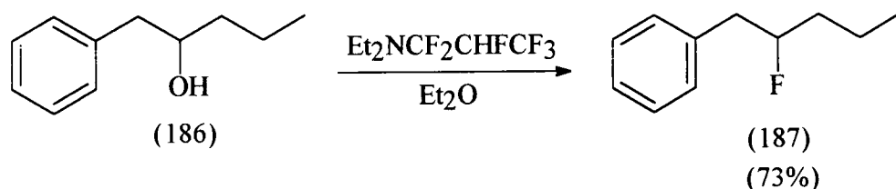
Scheme 104.
