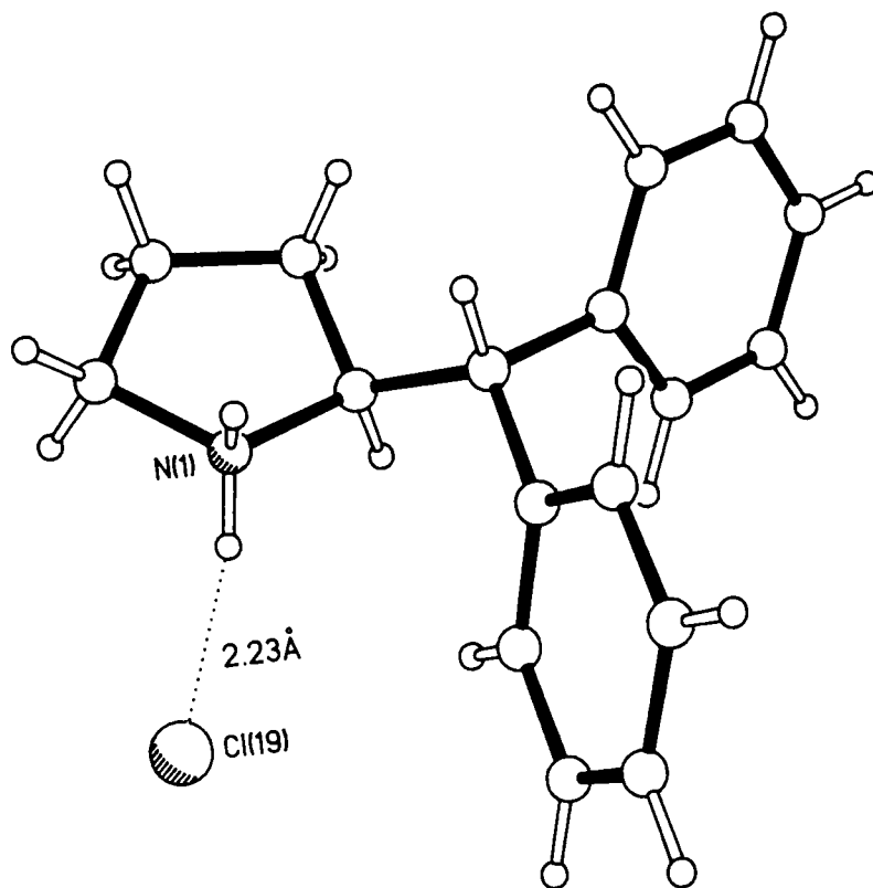
Figure 40. X-Ray crystal structure of (2S)-(diphenyl)methylpyrrolidine (168) HCl salt
