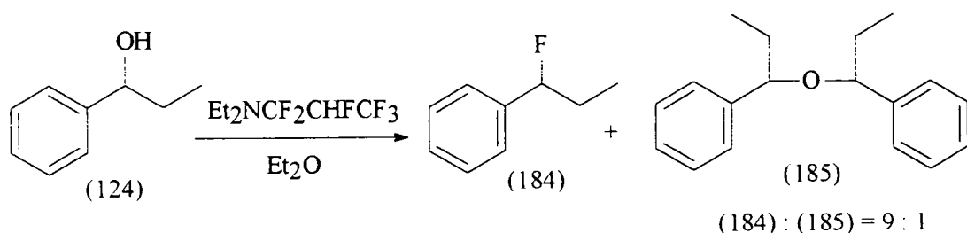
Scheme 103. (ratios of products determined by GC/MS)
