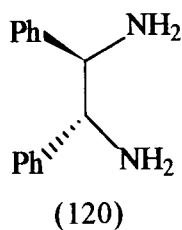
1,2-diphenyl-1,2-diaminoethane
