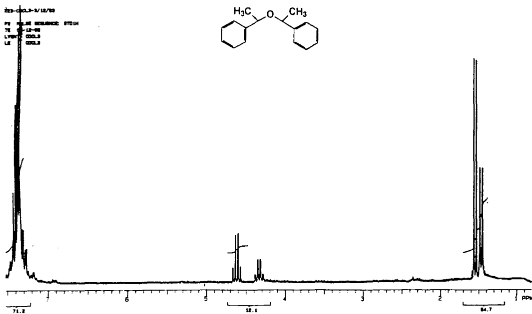
Figure 50. ^1\text{H} NMR of bis-(1-phenylethyl)ether (183) from (R)-1-phenylethanol
