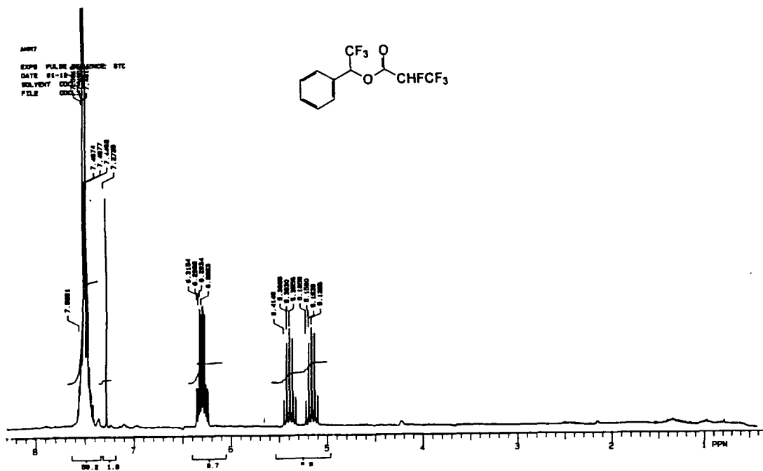
Figure 51. ^1\text{H} NMR of 2,2,2-trifluoro-1-phenylethyl 2',3',3',3'-tetrafluoropropionate (194)
