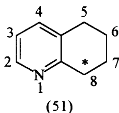
5,6,7,8-tetrahydroquinoline
