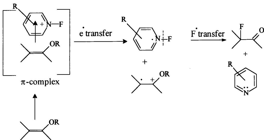
Scheme 15
