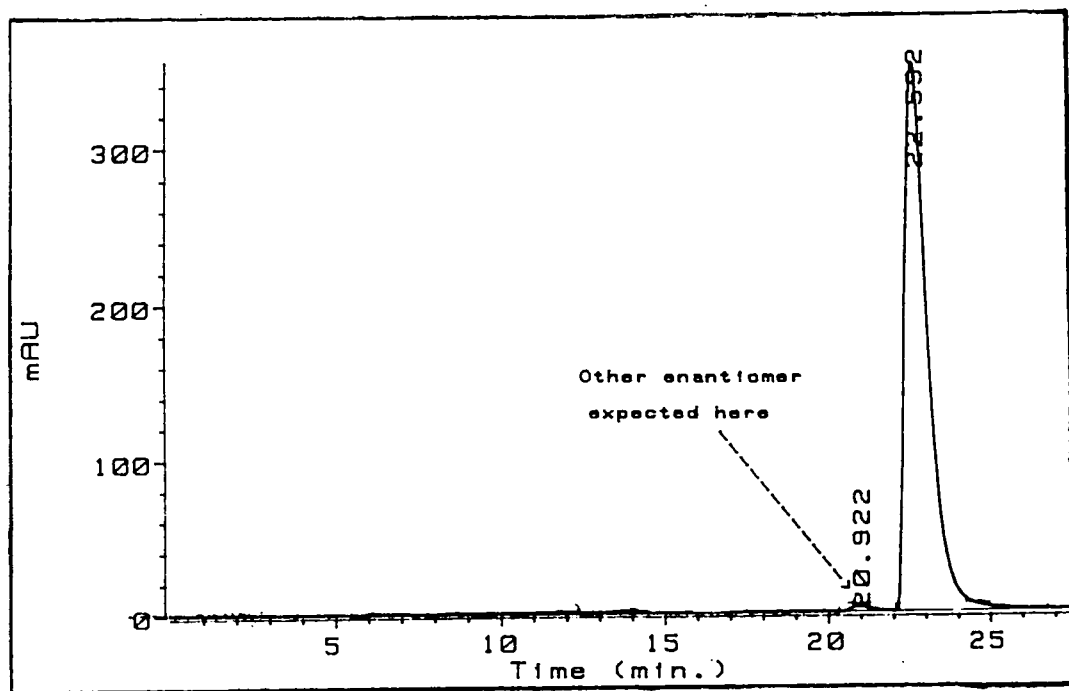
Figure 9. Chiral HPLC of (2S)-(1-hydroxyethyl)pyridine (55)
