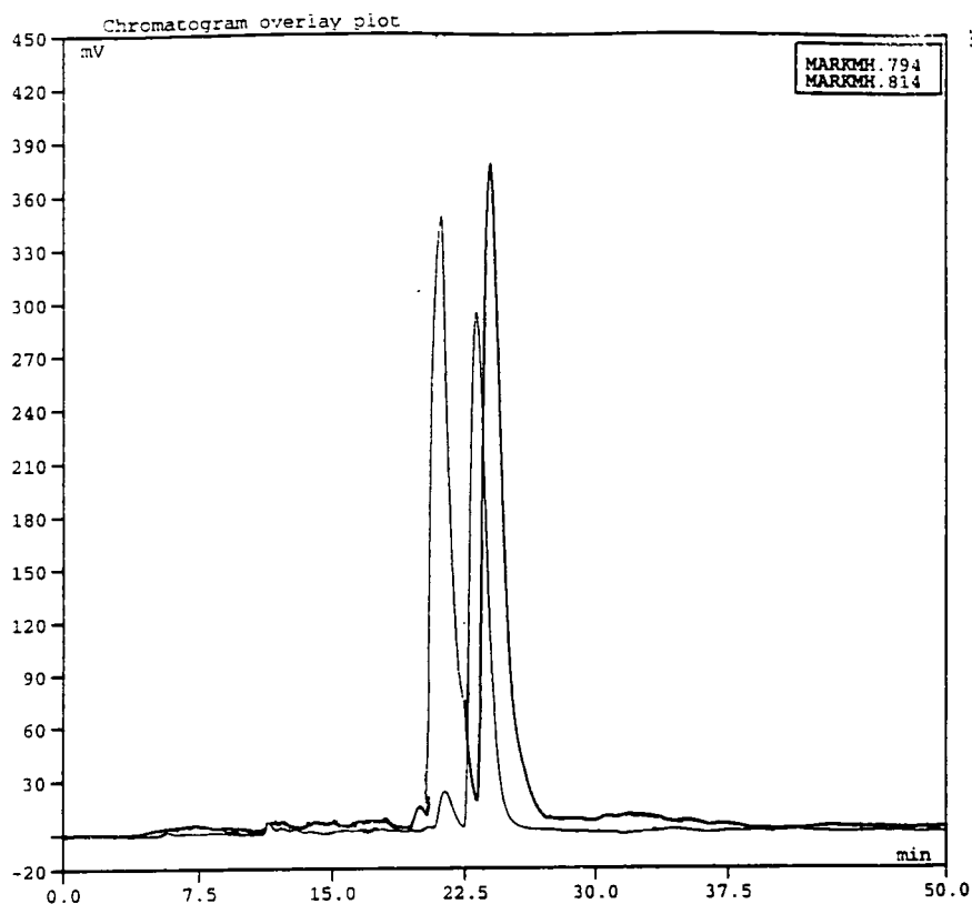
Figure 27. Chiral HPLC trace for 3-( \alpha -hydroxy)benzylpyridine optically enriched overlaid on racemic
