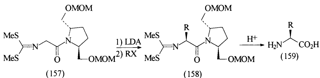
Scheme 88
