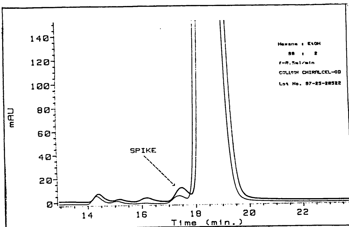
Figure 15. (2S),(6S)-diethyl( \alpha -4'-bromobenzoyloxy)pyridine (85) spiked with 0.5 % racemic 2,6-diethyl( \alpha -4'-bromobenzoyloxy)pyridine (85)
