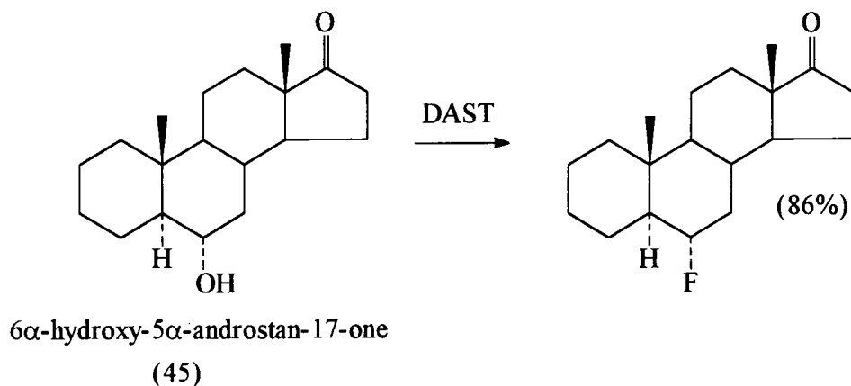
Scheme 26
