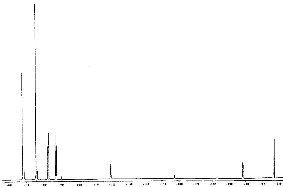
Figure 48. ^{19}\text{F} NMR of Ishikawa's reagent (179) & (180)
