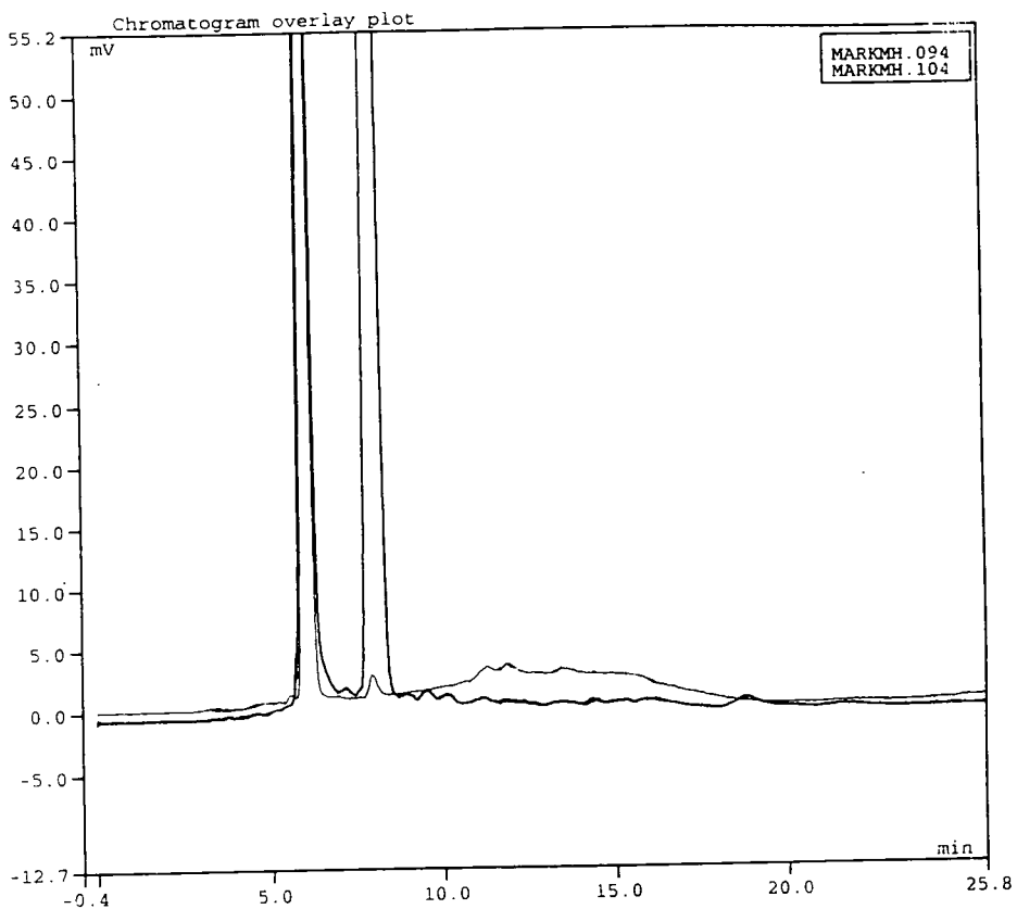
Figure 43. Overlay of (±)-2-(diphenyl)methylpyrrolidine on (2S)-(diphenyl)methylpyrrolidine (168)
