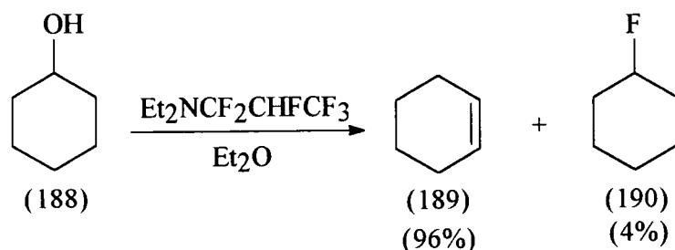
Scheme 105. (ratios of products determined by GC/MS)
