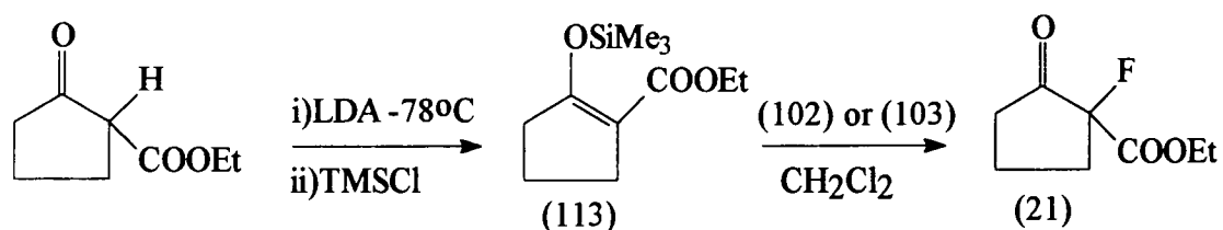
Scheme 65
