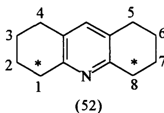
1,2,3,4,5,6,7,8-octahydroacridine
