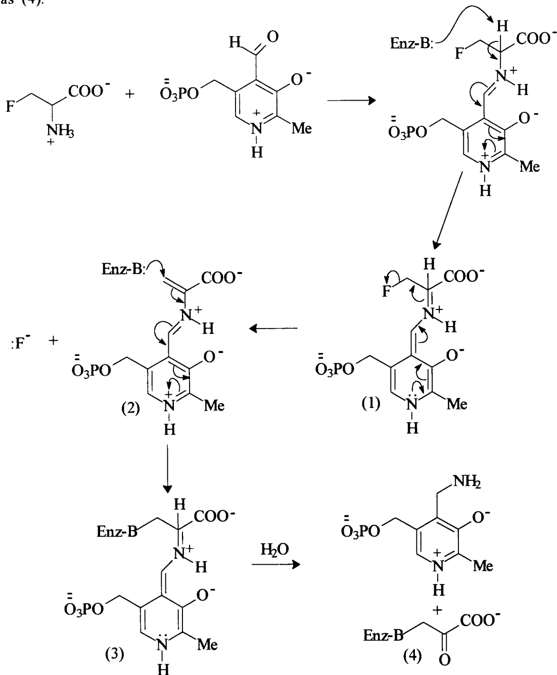
Scheme 1
