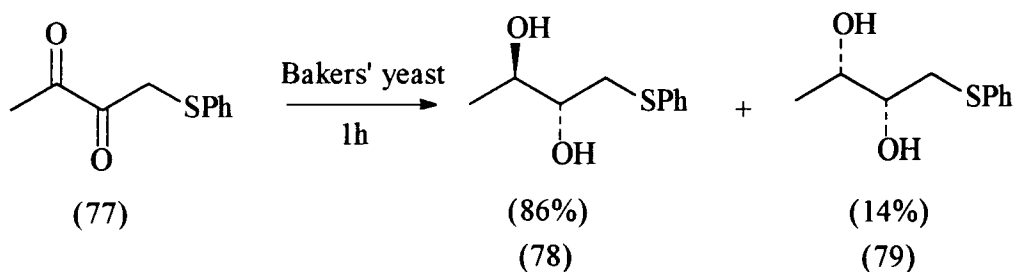
Scheme 45
