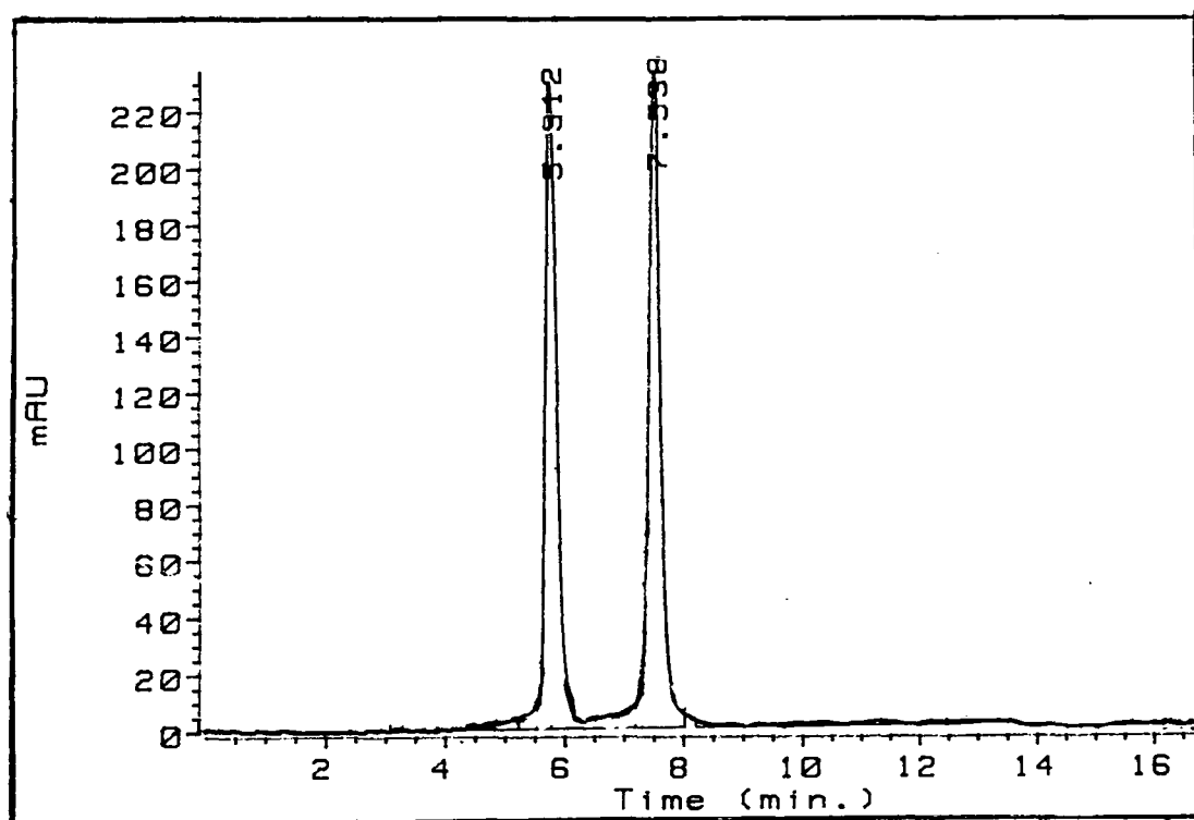
Figure 8. Chiral HPLC of ( \pm ) 2-acetyl-6-( \alpha -(2'S)-methylbutyryloxy)ethylpyridine (75)
