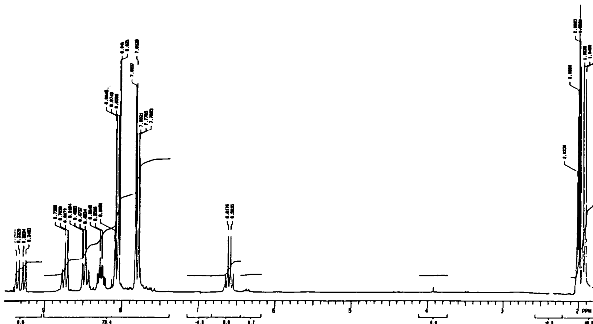
1 H NMR Spectra of N-Fluoro 2-( \alpha -4'-bromobenzoyloxy)ethylpyridinium triflate (102) Figure 19.
