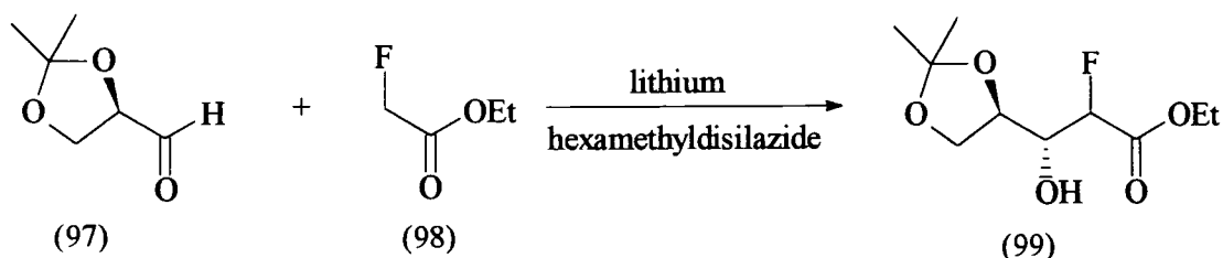
Scheme 58
