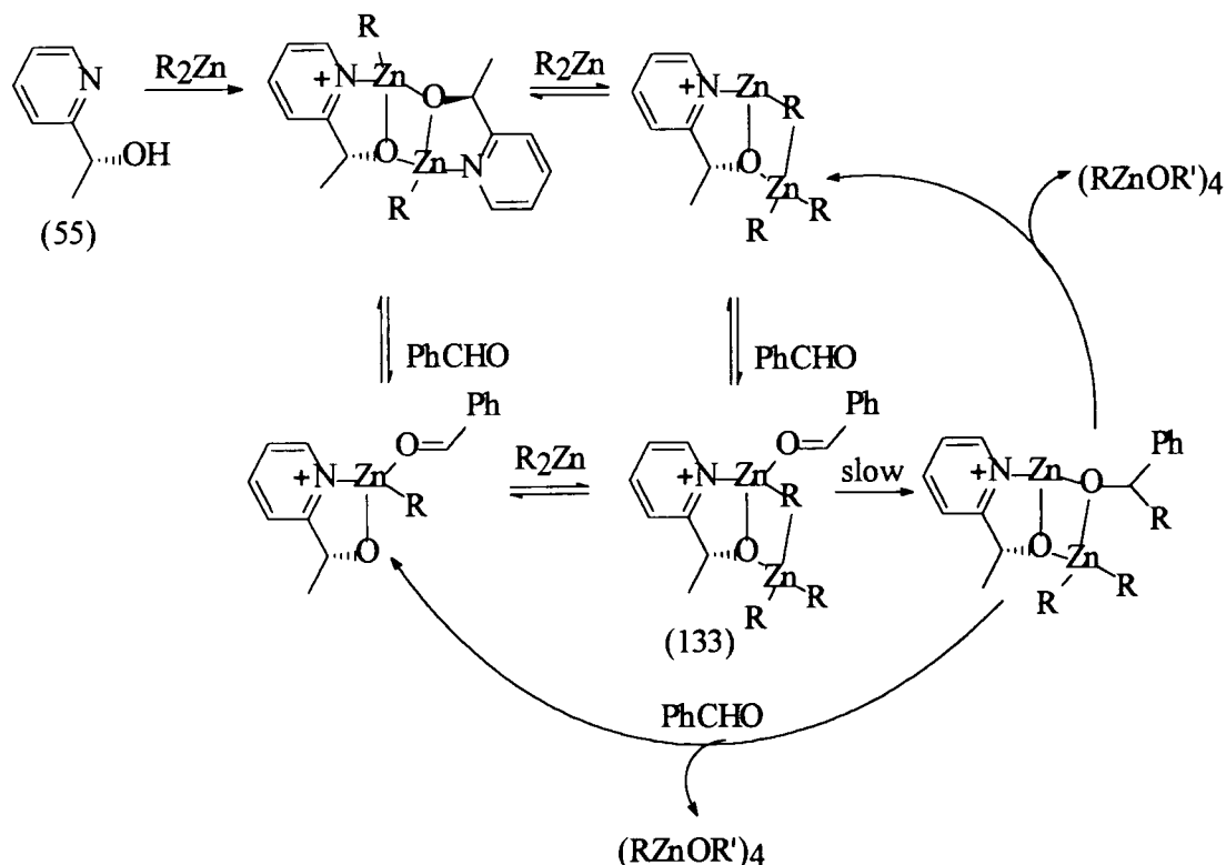
Scheme 78
