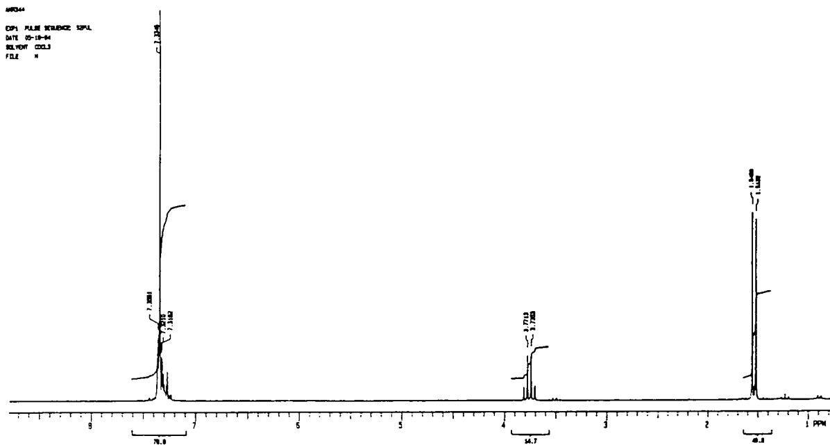
Figure 58. ^1\text{H} NMR of 2-phenylpropionic acid (214)
