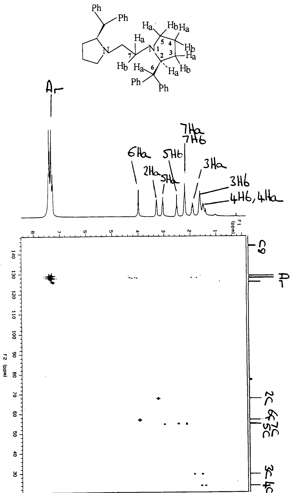
Figure 45. ^1H - ^{13}C HETCOR of N,N' -1,2-ethane-bis((2 S )-(diphenyl)methyl)pyrrolidine
