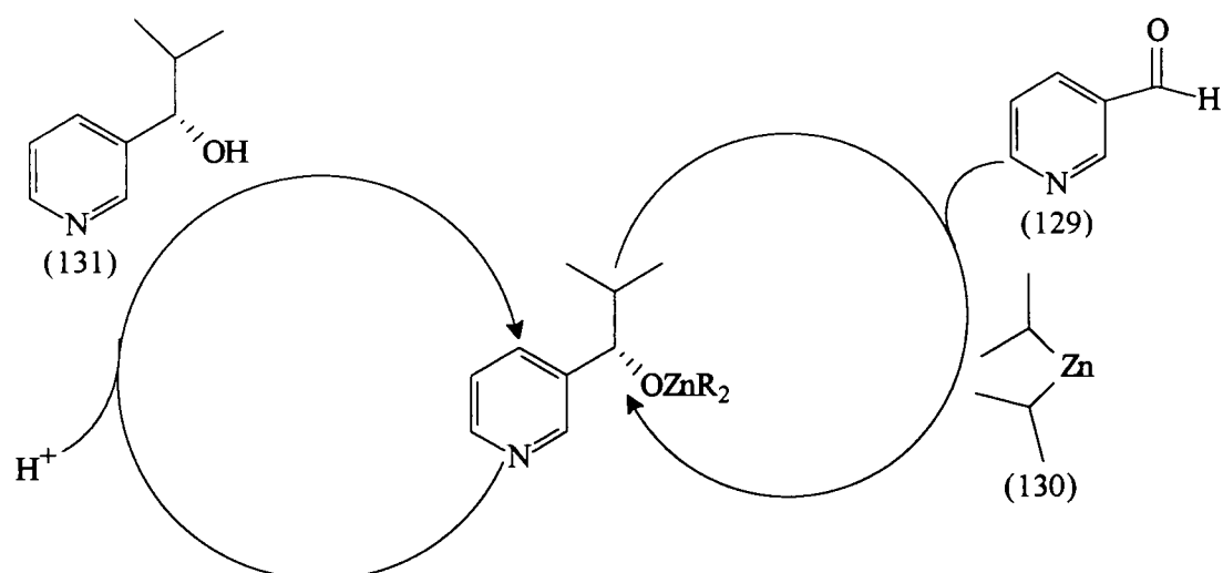
Scheme 77
