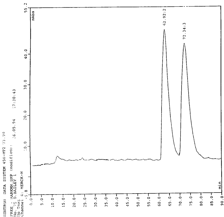
Figure 29. Chiral HPLC trace for racemic 4-( \alpha -hydroxy)benzylpyridine
