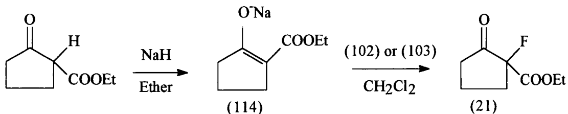
Scheme 66
