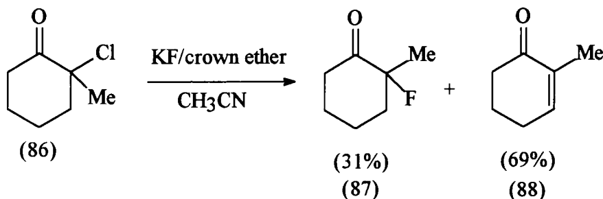
Scheme 52
