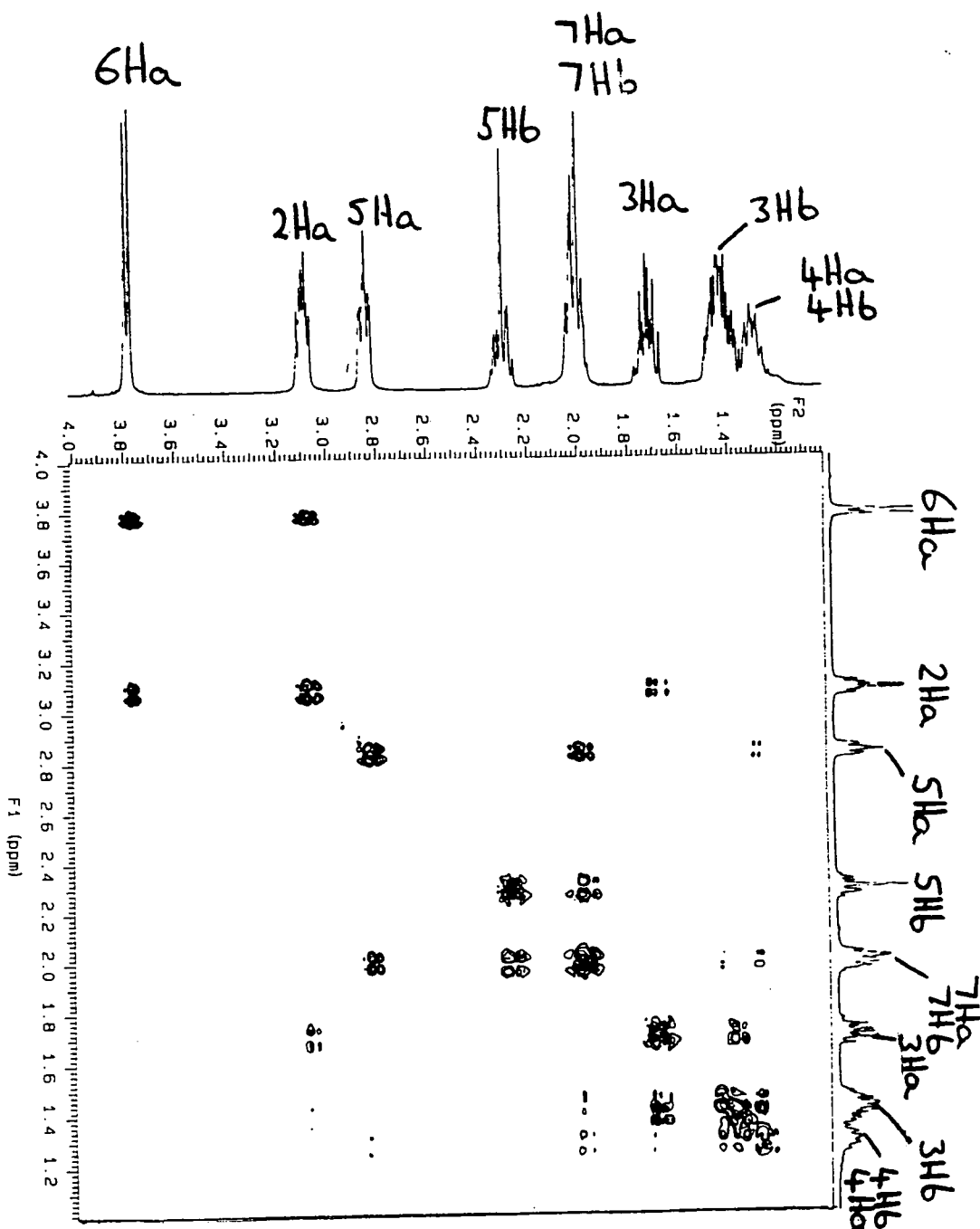
Figure 44. ^1\text{H} - ^1\text{H} COSY of N,N'-1,2-ethane-bis((2S)-(diphenyl)methyl)pyrrolidine (177)
