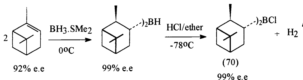
Scheme 39
