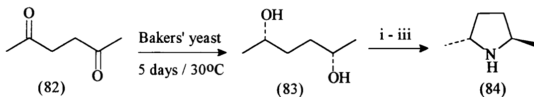
Scheme 47. i) Et_3N , methanesulfonyl chloride. ii) benzylamine, 25°C, 96h, NaOH. iii) glacial acetic acid, 10% Pd(OH)_2/C , H_2 , 30-40 Psi, NaOH.
