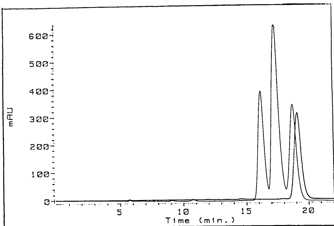
Figure 14. Overlay of racemic 2,6-diethyl( \alpha -4'-bromobenzoyloxy)pyridine (85) on (2S),(6S)-diethyl( \alpha -4'-bromobenzoyloxy)pyridine (85)
