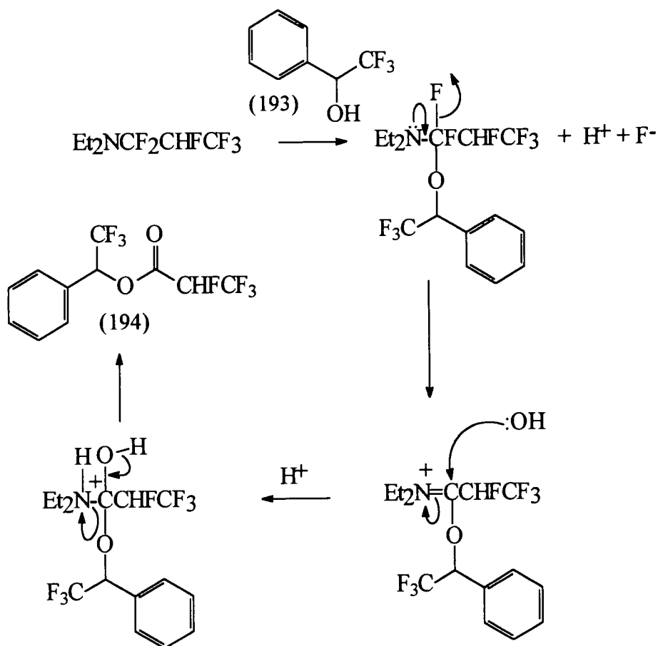
Scheme 108.
