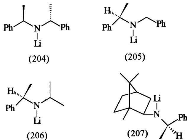
Figure 56. Homochiral lithium amide bases (HCLA)
