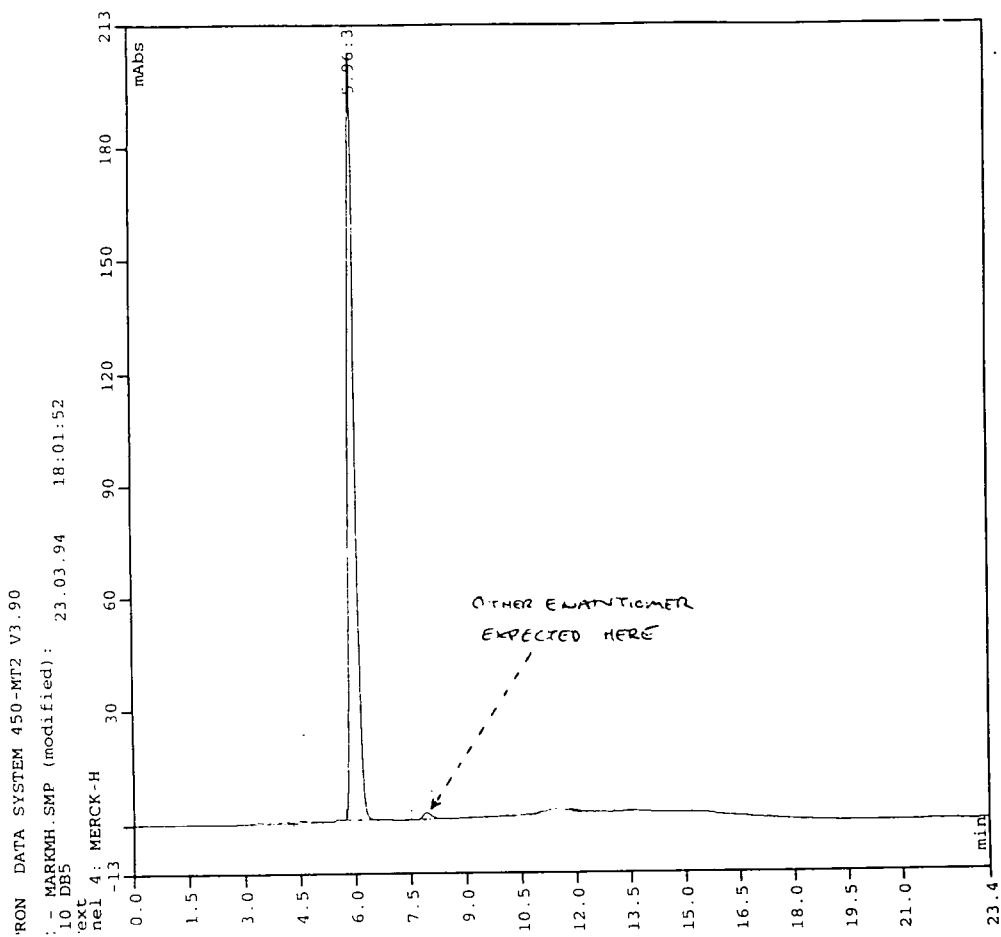
Figure 42. Chiral HPLC of (2S)-(diphenyl)methylpyrrolidine (168)
