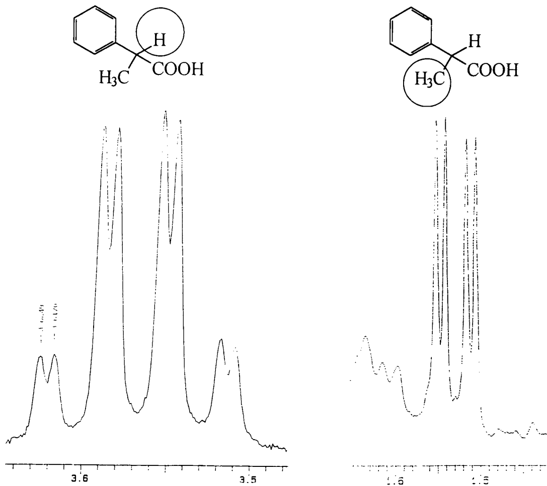
Figure 59. ^1\text{H} NMR Splitting patterns for ( \pm ) 2-phenylpropionic acid (214) in the presence of amine (168)
