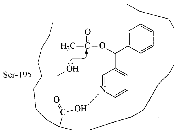
Figure 31. Lipase resolution of 3-( \alpha -acetoxy)benzylpyridine (138)
