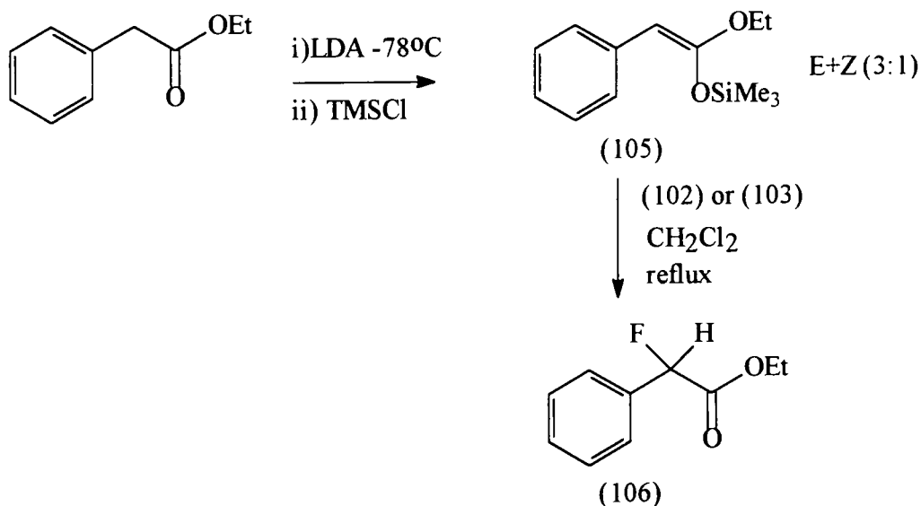
Scheme 60
