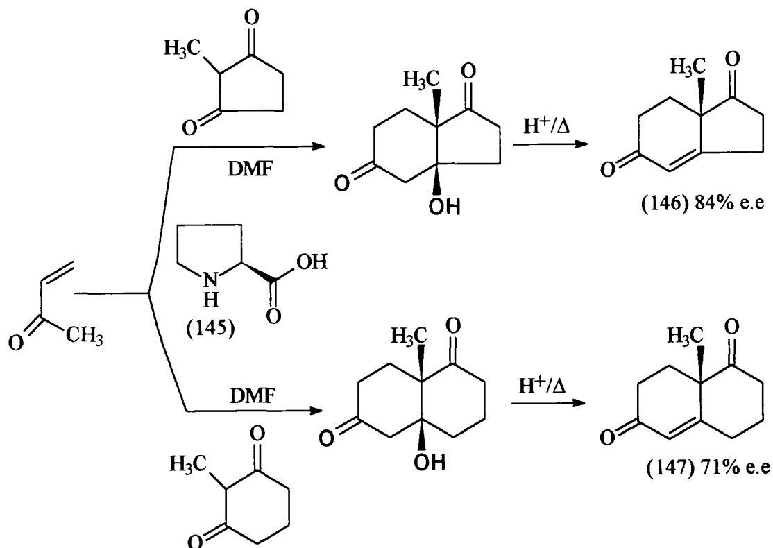
Scheme 82
