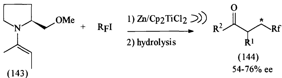
Scheme 81
