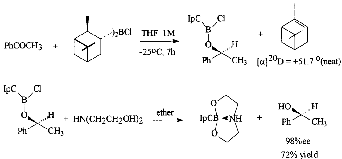
Scheme 40
