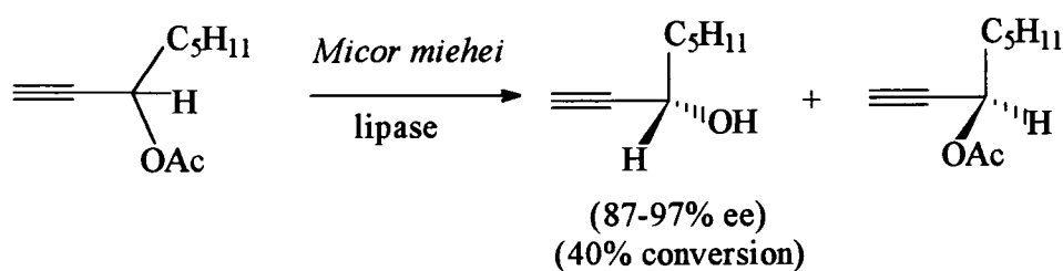
Scheme 34
