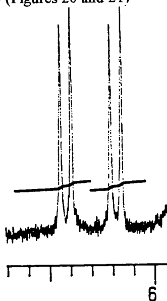
Figure 21. 1 H NMR of optically enriched (44) in the presence of [Eu(tfc) 3 ]
