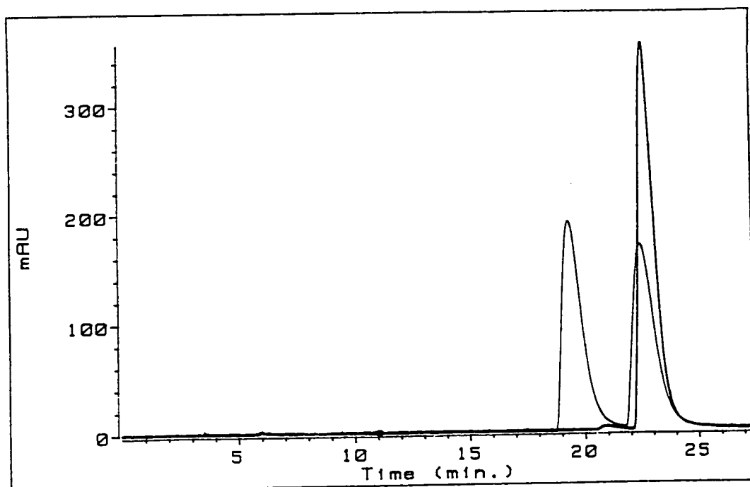
Figure 11. Overlay of racemic 2-(1-hydroxyethyl)pyridine (55) on (2S)-1-hydroxyethylpyridine (55)
