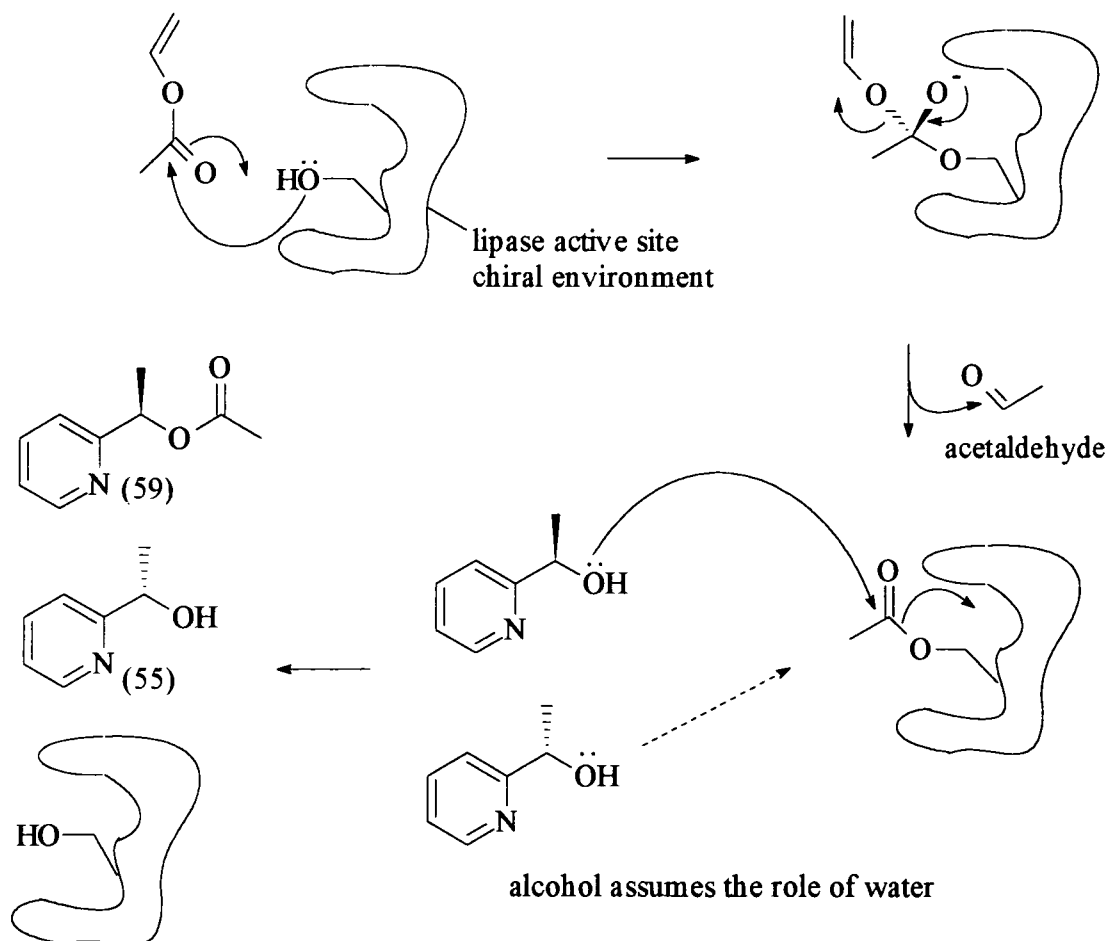
Scheme 36. Transesterification of 2-(1-hydroxyethyl)pyridine using lipase enzymes
