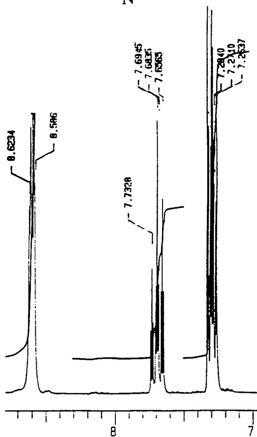
Figure 18. ^1\text{H} NMR of pyridine
