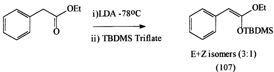
Scheme 61
