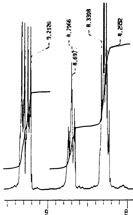
Figure 17. ^1\text{H} NMR of N-fluoropyridinium triflate
