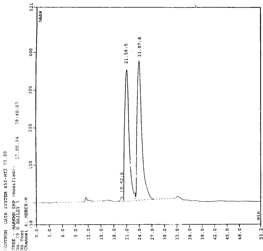
Figure 26. Chiral HPLC trace for racemic 3-( \alpha -hydroxy)benzylpyridine
