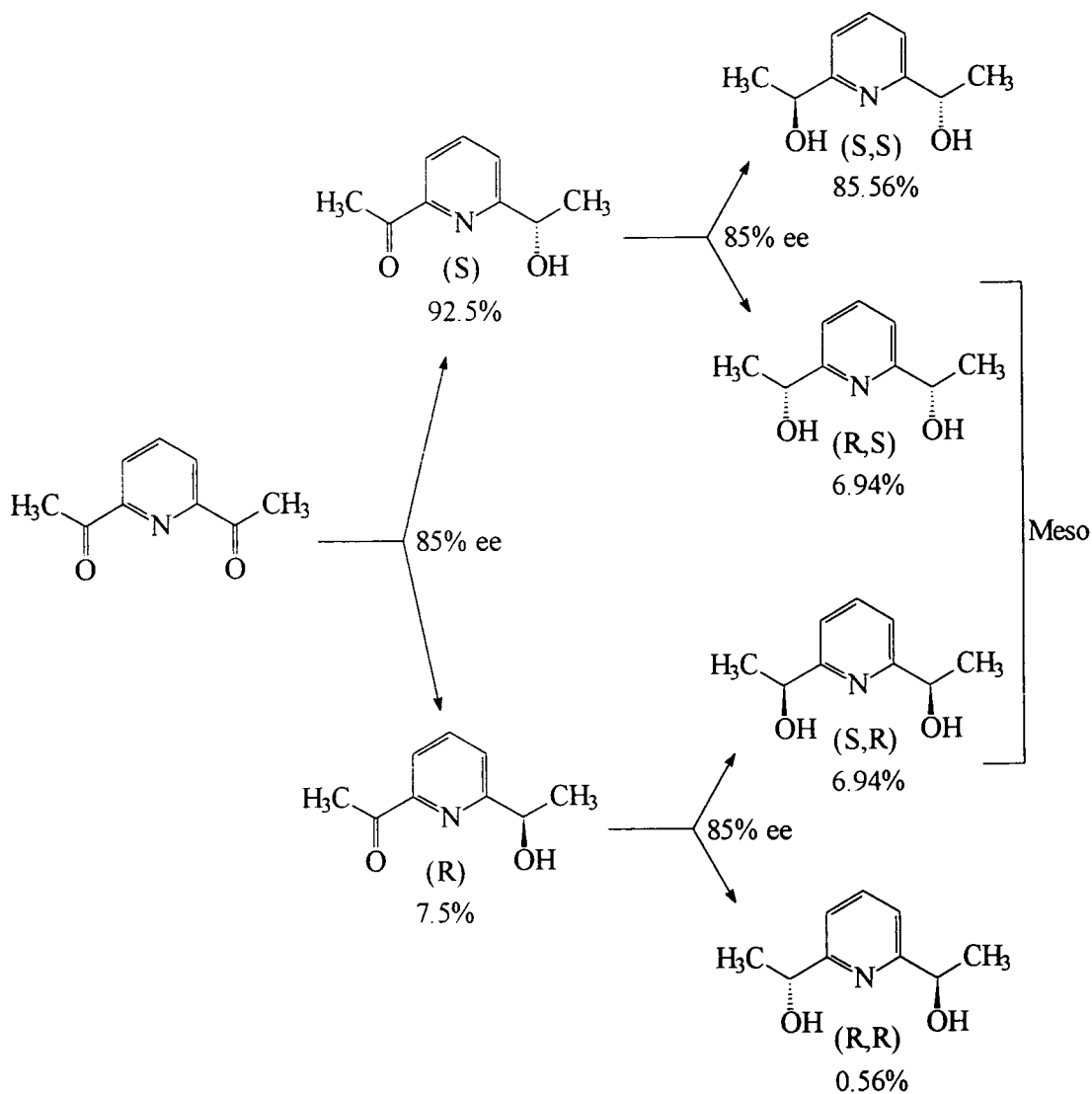
Scheme 49. The relationship between mono and di reductions for baker's yeast reduction of 2-acetylpyridine
