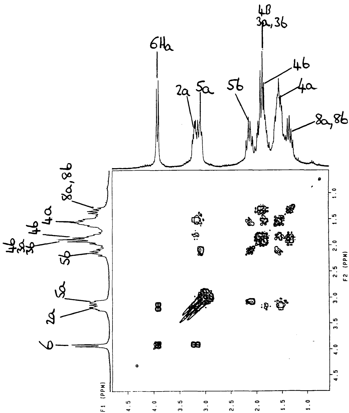
Figure 46. ^1\text{H} - ^1\text{H} COSY of N,N'-1,3-propane-bis((2S)-(diphenyl)methyl)pyrrolidine (178)
