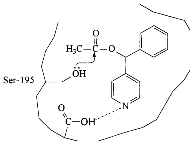
Figure 32. Lipase resolution of 4-( \alpha -acetoxy)benzylpyridine (140)
