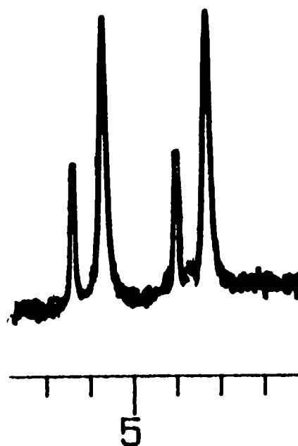
Figure 55. ^1\text{H} NMR of methyl 2-fluorophenylacetate (192) in the presence of [\text{Eu}(\text{tfc})_3] produced by reaction of (R)-(-)-methyl mandelate with reagent (201)
