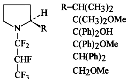
Figure 5. Homologues of Ishikawa's reagent
