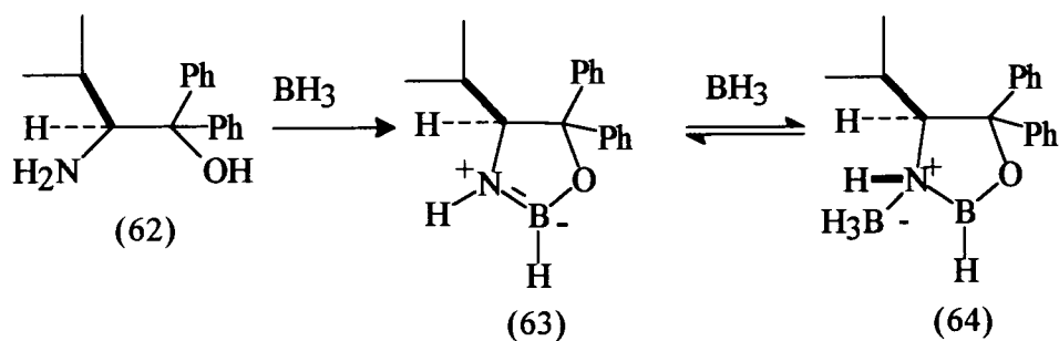
Scheme 38
