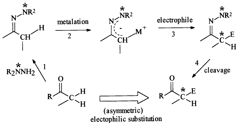
Scheme 86
