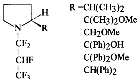
Figure 36. Homologues of Ishikawa's reagent
