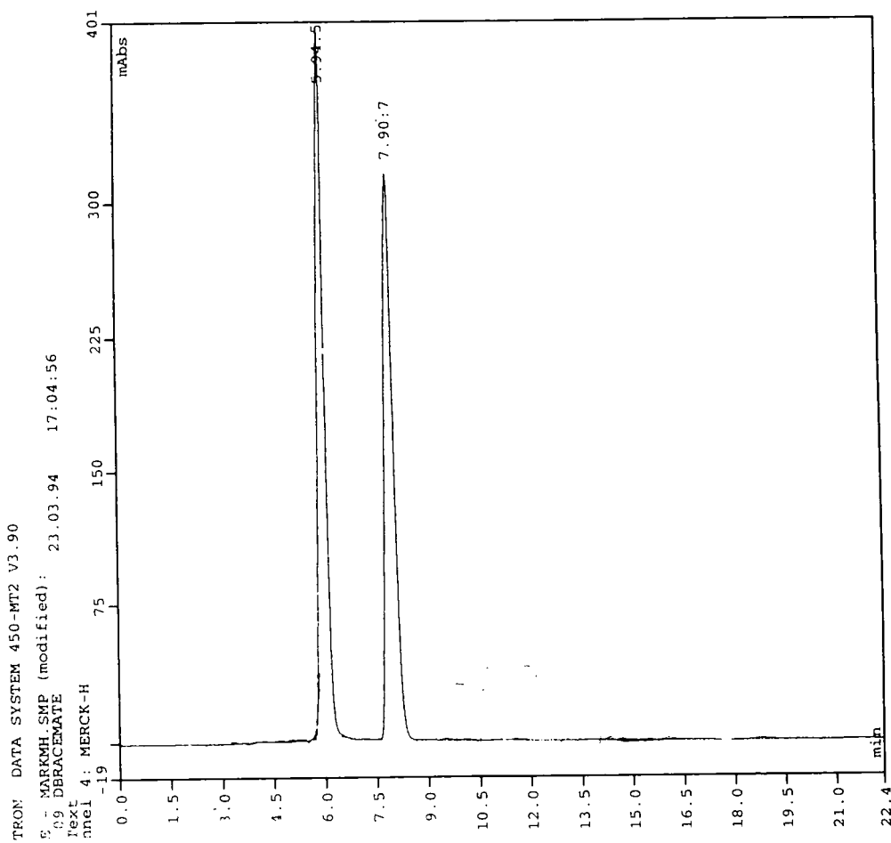
Figure 41. Chiral HPLC of (±)-2-(diphenyl)methylpyrrolidine (168)
