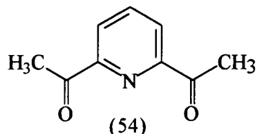
2,6-diacetylpyridine
