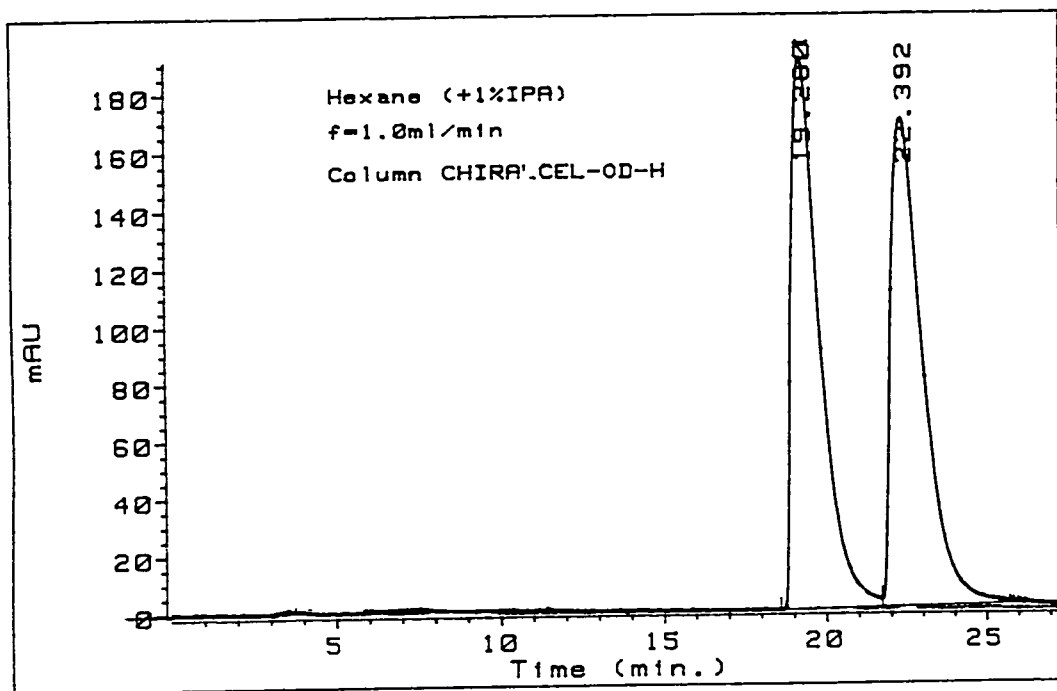
Figure 10. Chiral HPLC of racemic 2-(1-hydroxyethyl)pyridine (55)
