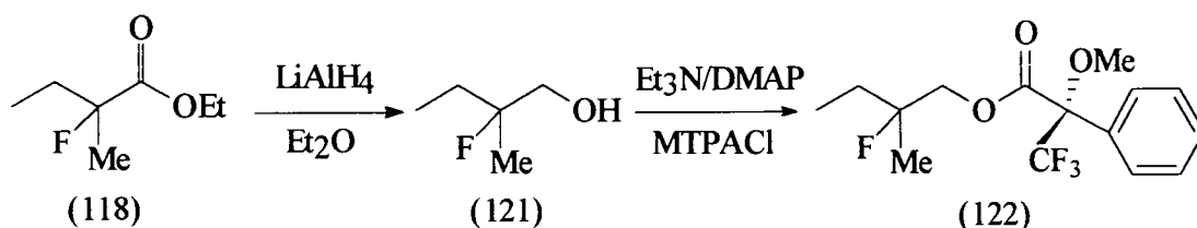
Scheme 70
