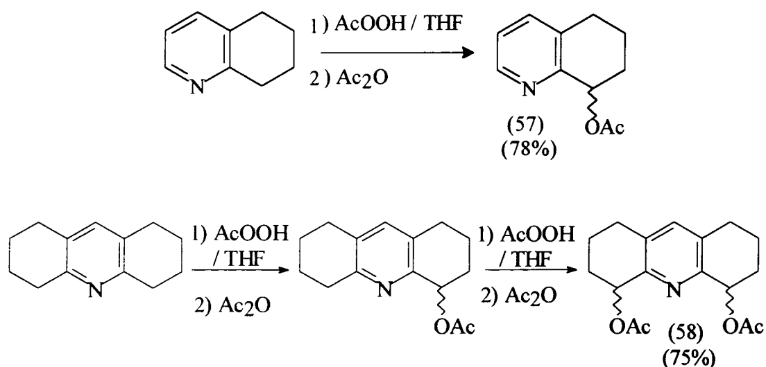
Scheme 35
