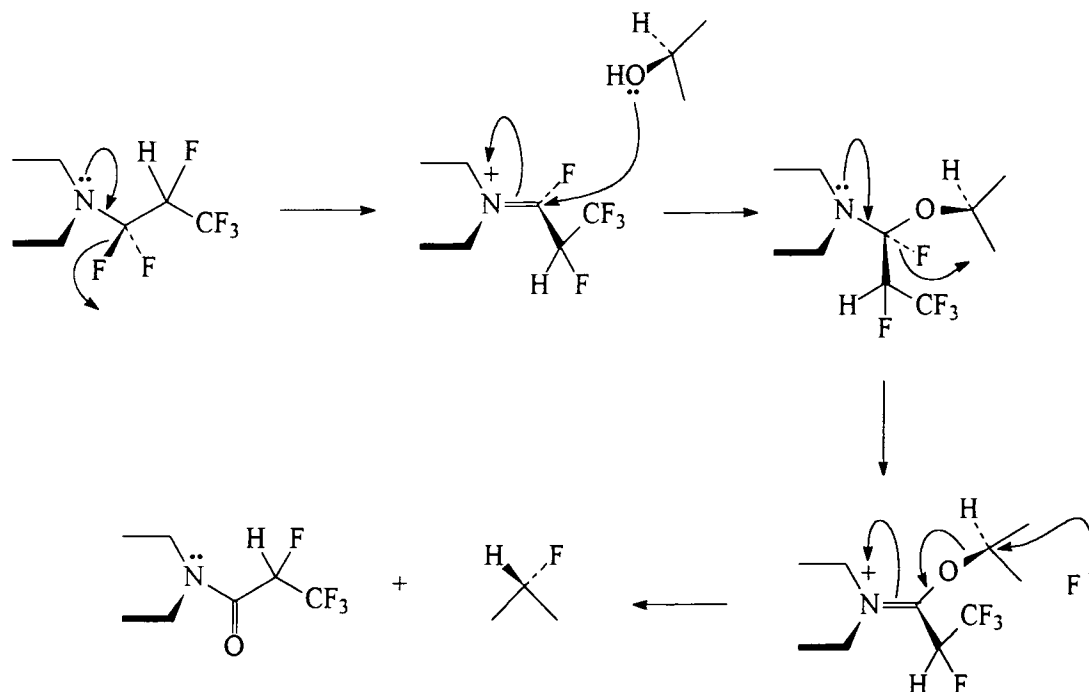
Scheme 18
