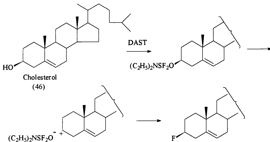
Scheme 27
