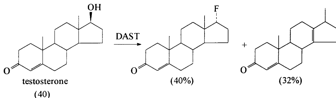
Scheme 22
