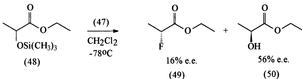
Scheme 29
