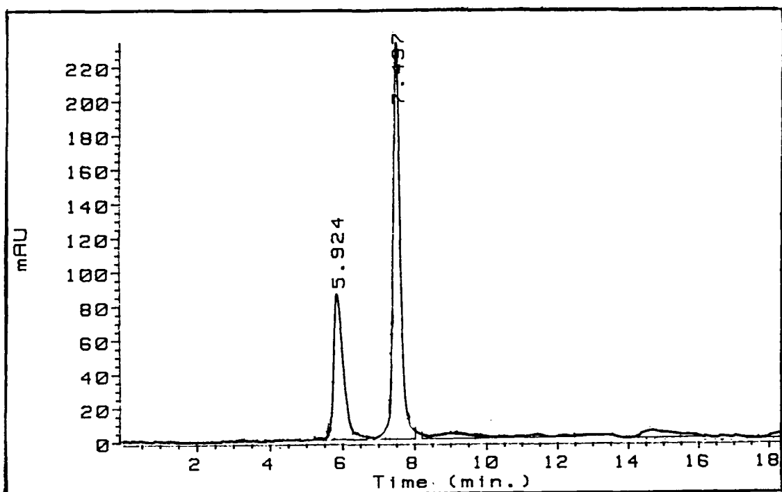
Figure 7. Chiral HPLC of optically enriched 2-acetyl-6-( \alpha -(2'S)-methylbutyryloxy)ethylpyridine (75)
