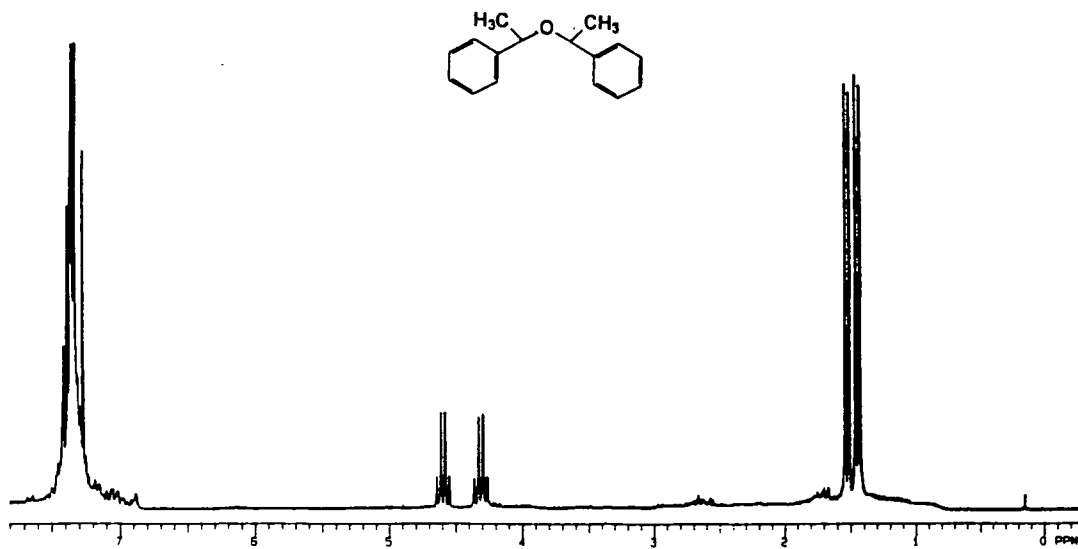
Figure 49. ^1\text{H} NMR of bis-(1-phenylethyl)ether (183)
