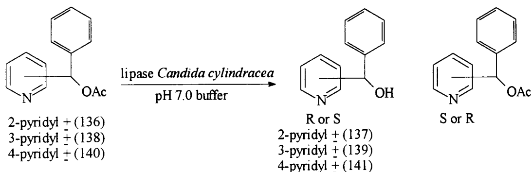
Scheme 79
