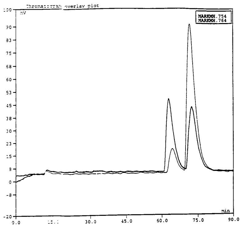
Figure 30. Chiral HPLC trace for 4( \alpha -hydroxy)benzylpyridine optically enriched overlaid on racemic
