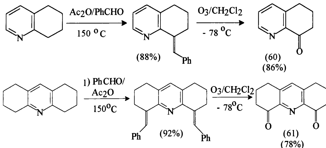
Scheme 37
