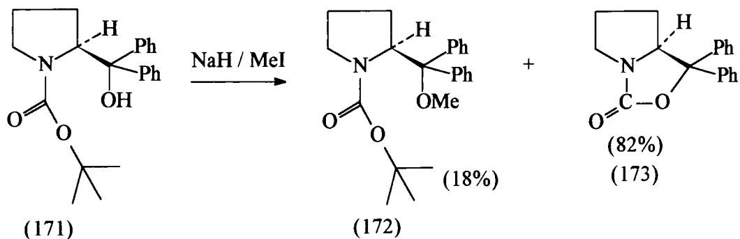
Scheme 93
