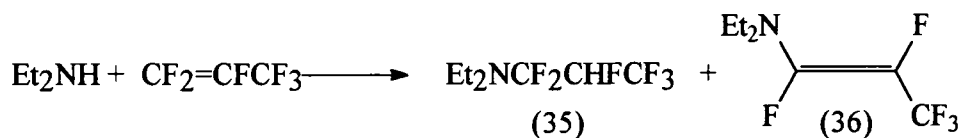
Scheme 17
