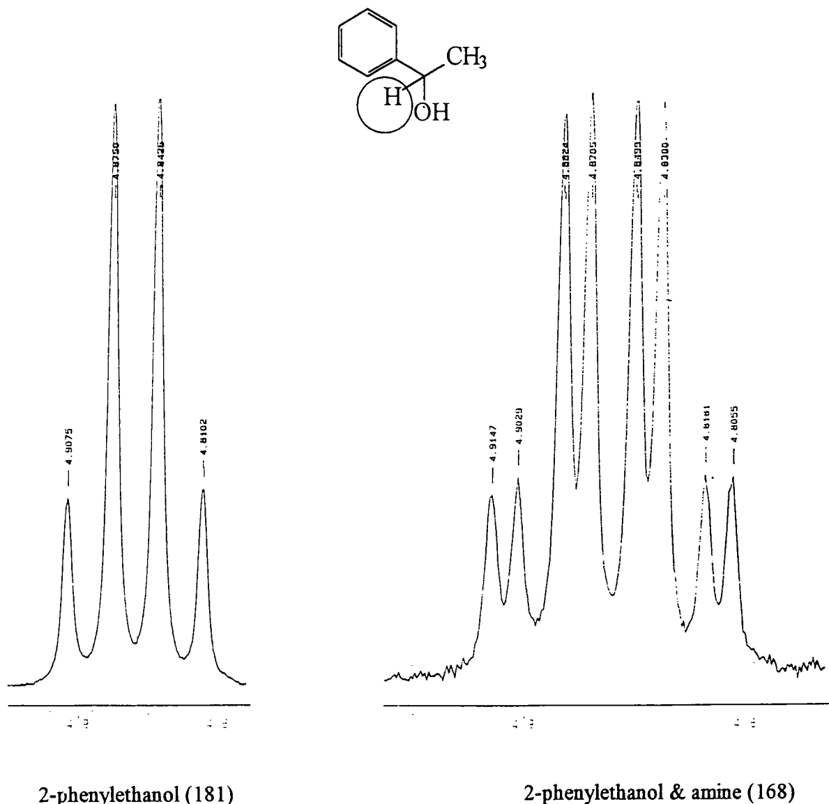
Figure 60. ^1\text{H} NMR Splitting patterns for ( \pm ) 2-phenylethanol (181) in the presence of amine (168)
