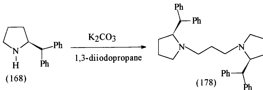
Scheme 101
