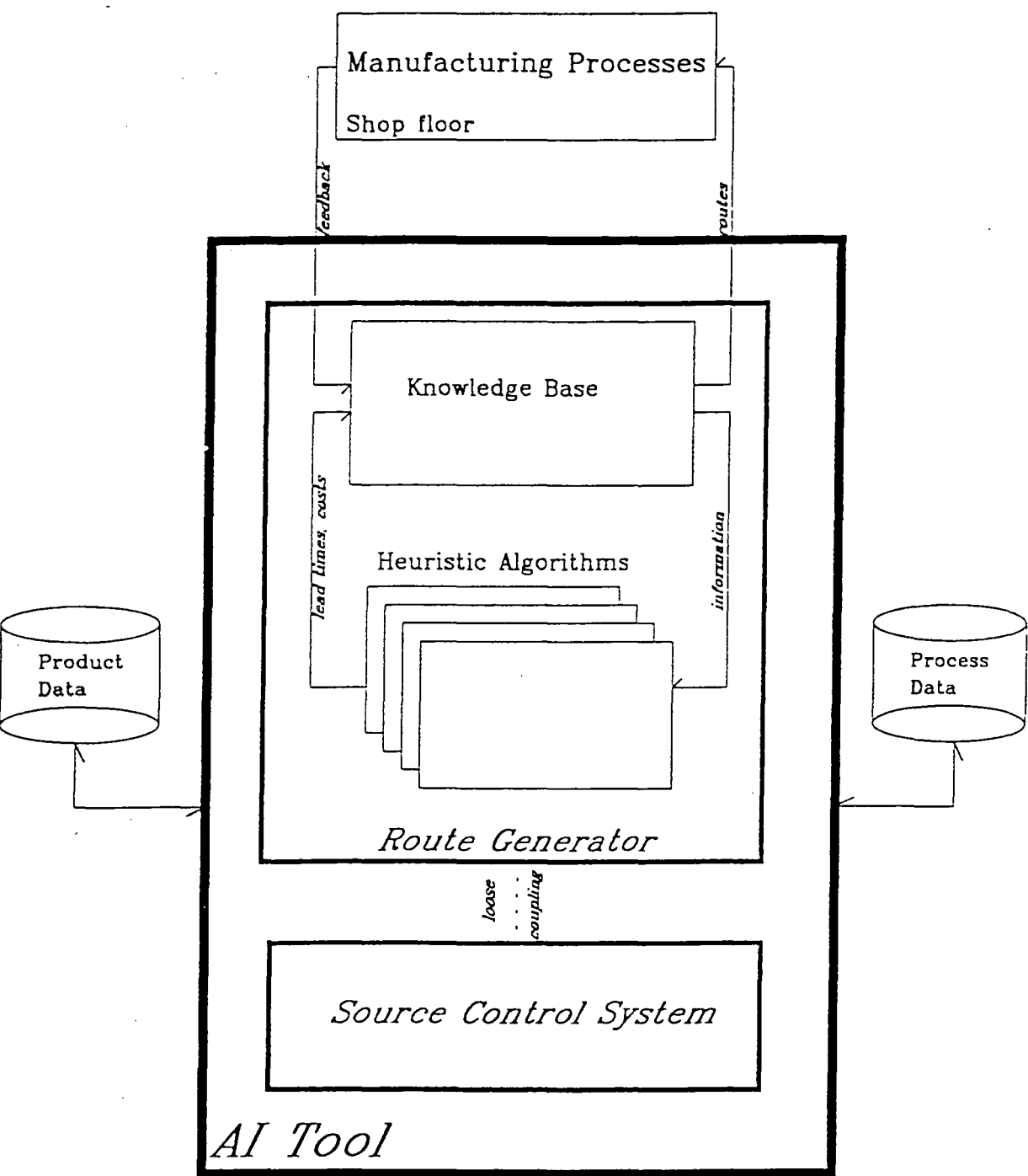
Figure 1. Overall structure of the proposed AI tool
