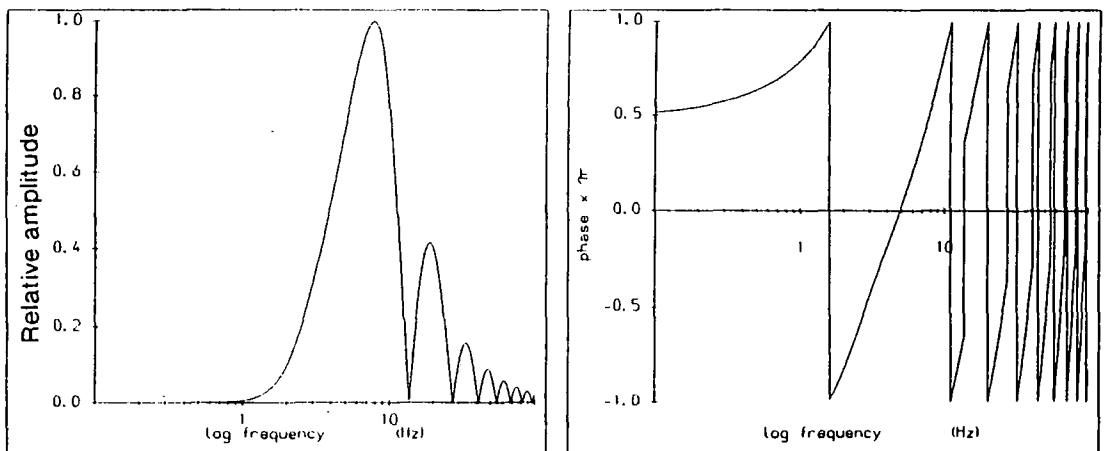
Fig. 5.2 Source signatures computed for the reflectivity method to yield: (a) ground displacement and (b) ground velocity synthetic seismograms.
