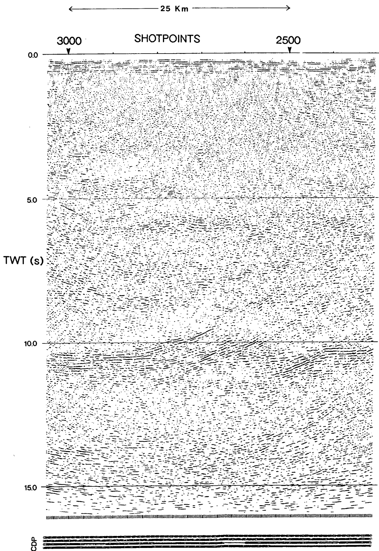
Fig. 7.4 Migrated 1 normal-incidence section from line 1, for velocity 5.5 kms -1 (courtesy of Richard Hobbs, BIRPS).
