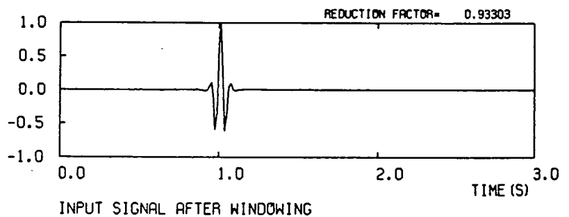
Fig. 5.6 Example of plot of input signal generated by program SYNT.
