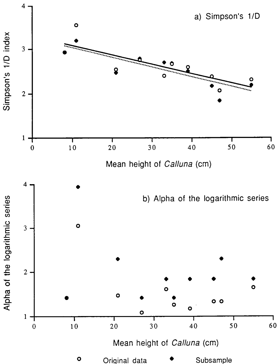
Figure 6.3a-b. The relationship between Calluna height and a) Simpson's 1/D and b) \alpha of the logarithmic series at Slaley (16 July-5 November 1992). Indices were calculated for the original data and for a derived subsample of 46 larvae. Index values for the subsample were based on an average of five random replicates. The dark circle represents the sample of 46 larvae in the original data and has been included in both regressions. Regressions for the original data are shown by a solid line. Regression data are for a) original data Y = -0.021(\pm 0.006)X + 3.31(\pm 0.197) , r = -0.80 , df = 8 , P < 0.01 ; derived data Y = -0.022(\pm 0.005)X + 3.26(\pm 0.18) , r = -0.84 , df = 8 , P < 0.01 b) original data r = 0.42 , df = 8 , NS; derived data r = 0.30 , df = 8 , NS. Derived values of \alpha in Figure 6.3b are higher than values calculated from the original data.
