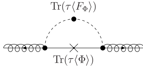
Figure 3.1: One-loop contribution to the gaugino masses from messengers f, \tilde{f} . The dashed (solid) line is a bosonic (fermionic) messenger. The blob on the scalar line indicates an insertion of the F -term VEV into the propagator of the scalar messengers and the cross denotes an insertion of the R -symmetry breaking VEV into the propagator of the fermionic messengers.
