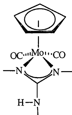
Figure 4.3 Proposed structure of [\text{Mo}(\eta\text{-C}_5\text{H}_5)(\text{TPGH})(\text{CO})_2]
