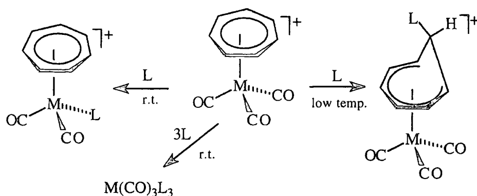
Figure 4.4 Reactions involving [M(\eta\text{-C}_7\text{H}_7)(\text{CO})_3][\text{BF}_4] ( M=\text{Mo}, \text{W} ). L =phosphines
