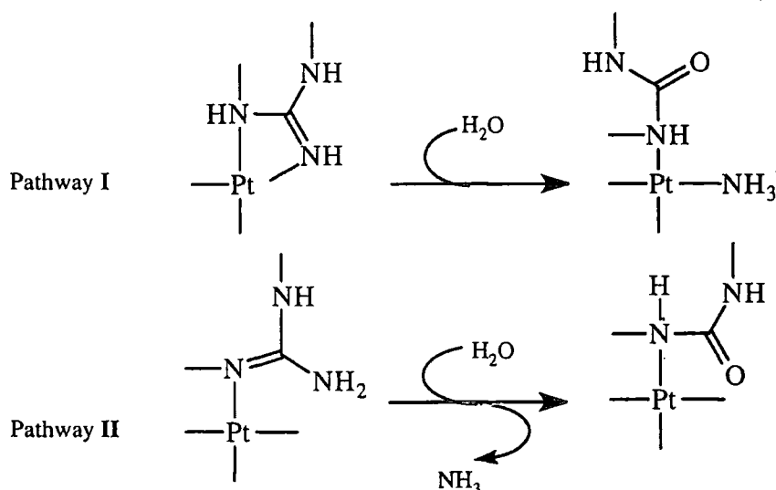
Figure 6.6 Nucleophilic attack of water towards coordinated DPGH 3
