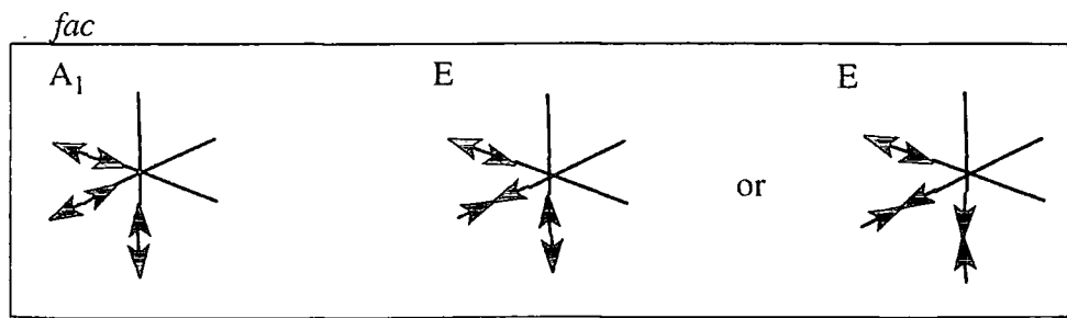
Figure B5 Theoretical vibrational modes for [M(X)_3(CO)_3] -type complex (X = monodentate ligand)
