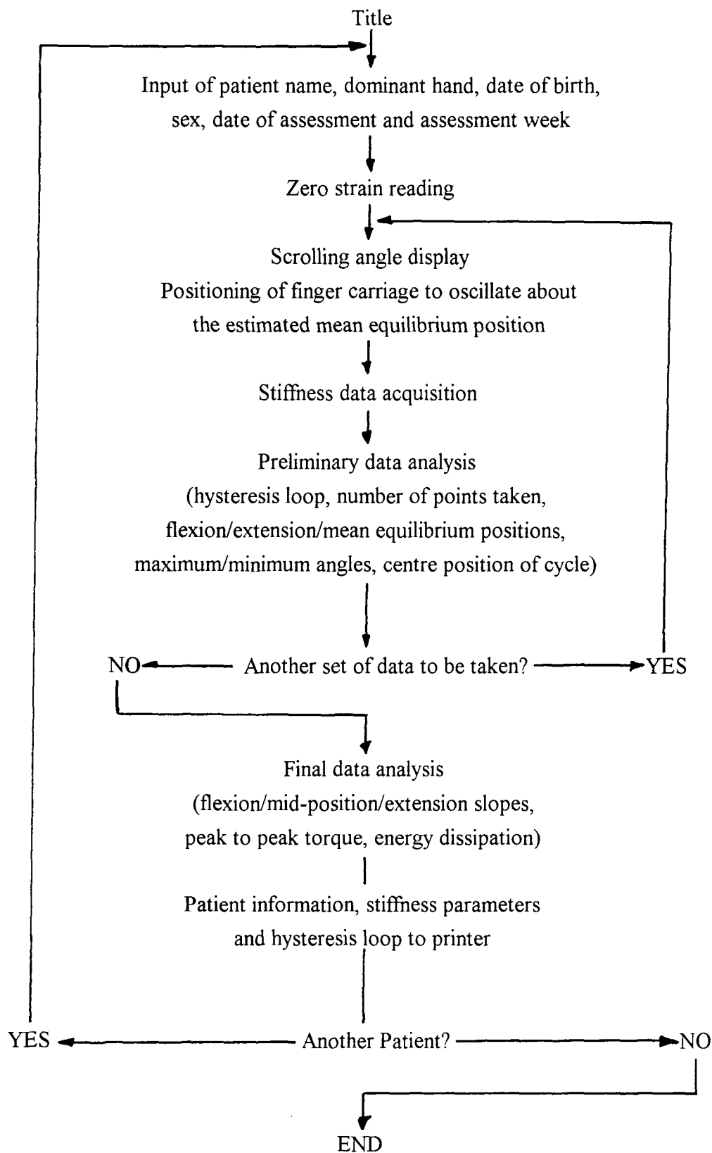
Figure 6.6 Flow diagram of Apple-Basic arthrograph data acquisition and analysis program
