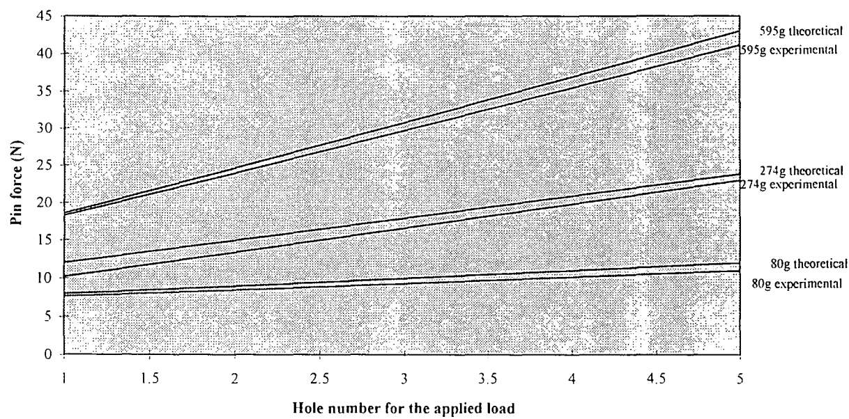
Figure A4.7 Experimental and theoretical pin forces
