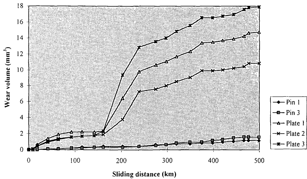
Figure 5.4 : Pin-on-plate test of XLPE pins against XLPE plates under 40N loading (Test 3)
