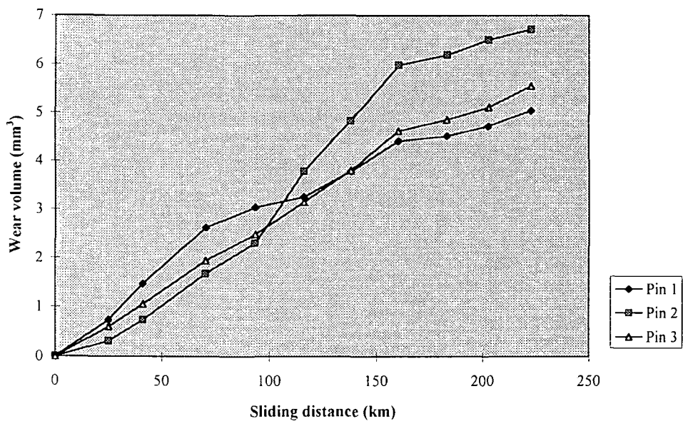
Figure 5.11 : Pin-on-plate wear test of UHMWPE pins against stainless steel plates under 40N loading (Test 10)
