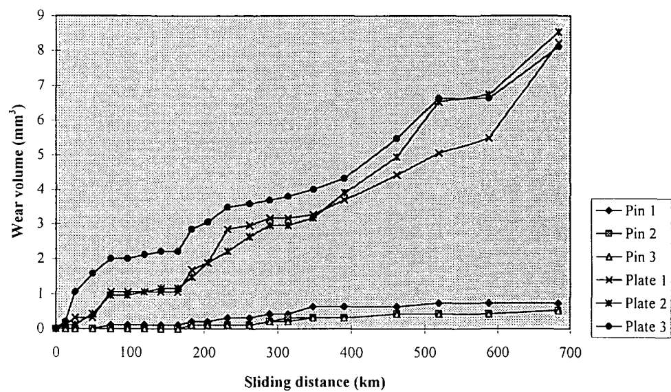
Figure 5.6 : Pin-on-plate test of XLPE pins against XLPE plates under 40N loading (Test 5)
