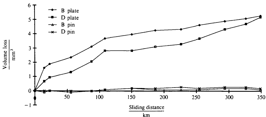
Fig. 4 Wear of XLPE pins and corresponding XLPE plates loaded at 40 N in the reciprocating pin-on-plate machine
