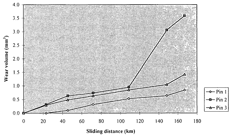
Figure 5.12 : Pin-on-plate wear test of XLPE pins against stainless steel plates under 10 N loading (Test 11)
