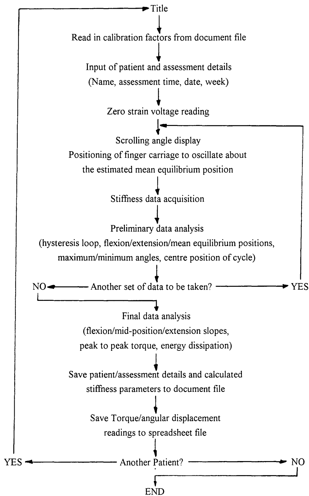
Figure 6.8 Flow diagram of the LabVIEW joint stiffness data acquisition and analysis program
