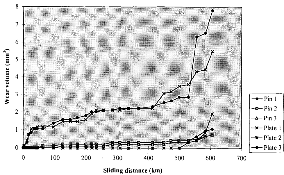
Figure 5.3 : Pin-on-plate wear test of XLPE pins against XLPE plates under 10N loading (Test 2)
