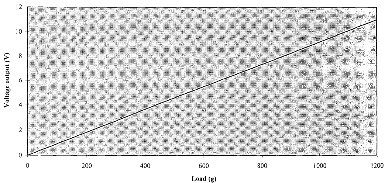
Figure A4.6 Calibration graph for the 100x amplifier
