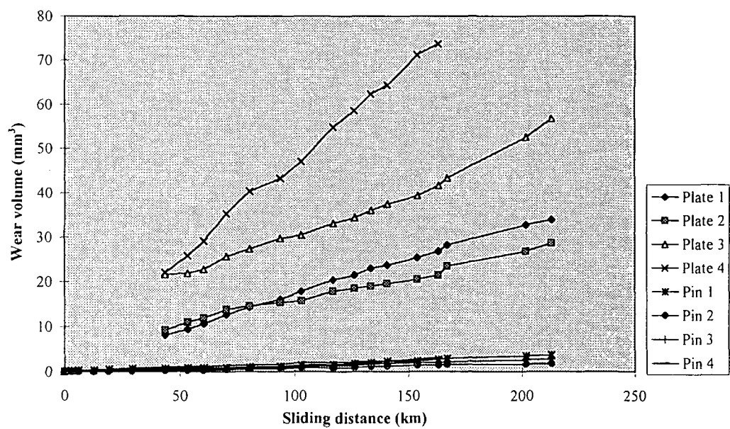
Figure 5.2 : Pin-on-Plate Wear Test of XLPE Pins against XLPE Plates Under 10N Loading (Test 1)
