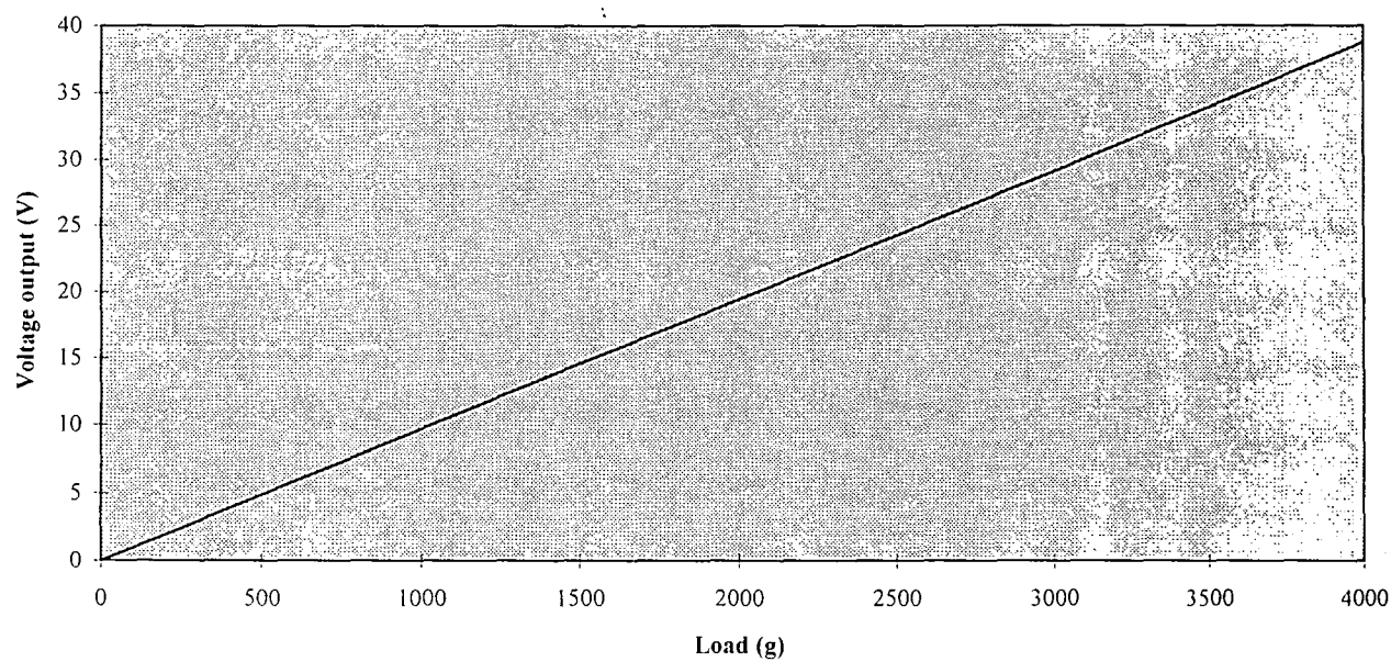
Figure A4.5 Calibration graph for the 10x amplifier
