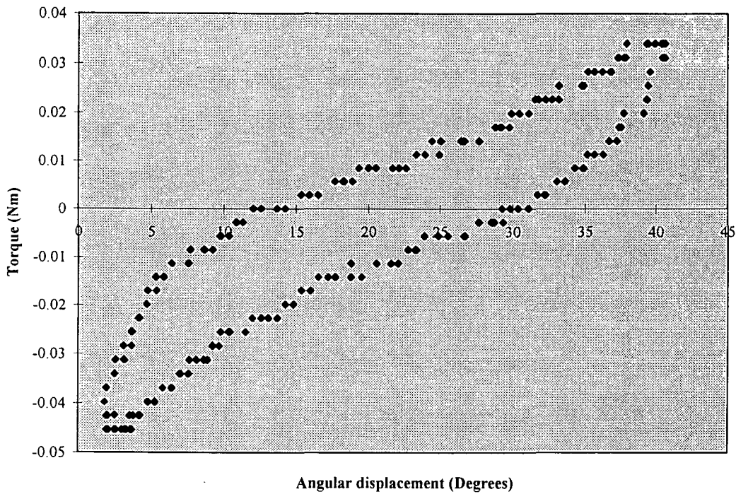
b) Female MCPJ stiffness hysteresis loop
