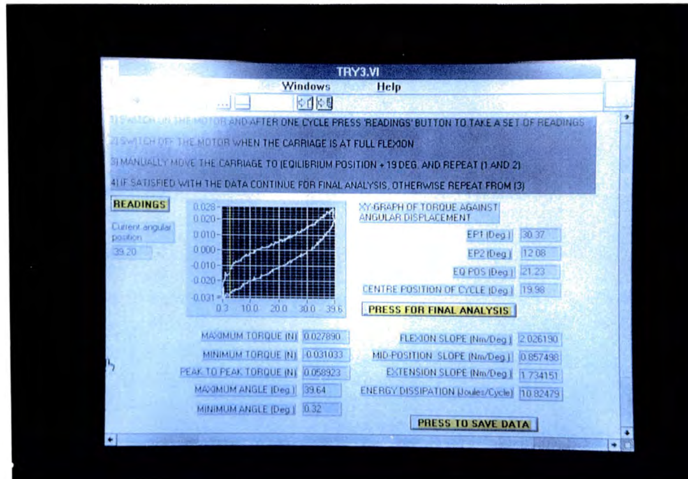
Figure 6.11 Main screen for the LabVIEW joint stiffness data acquisition and analysis program
