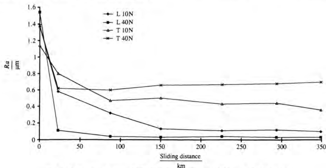
Fig. 6 Mean roughness of XLPE plates loaded at 10 N and 40 N in the transverse (T) and longitudinal (L) directions
