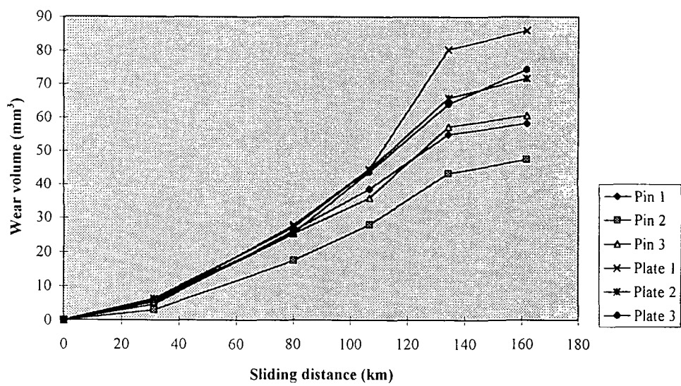
Figure 5.8 : Pin-on-plate wear test of UHMWPE pins against UHMWPE plates under 10N loading (Test 7)
