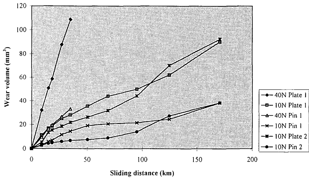
Figure 5.9 : Pin-on-plate test of UHMWPE pins against UHMWPE plates under 10N and 40N loading (Test 8)
