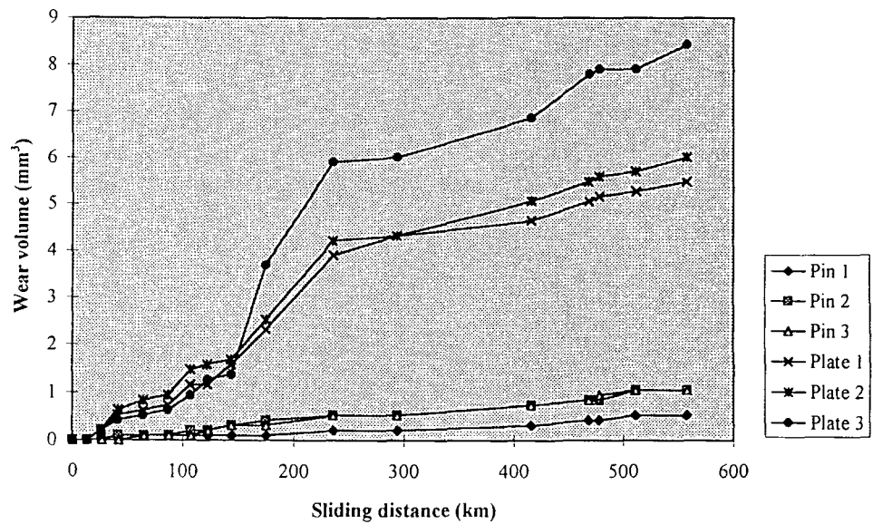
Figure 5.5 : Pin-on-plate test of XLPE pins against XLPE plates under 10N loading (Test 4)
