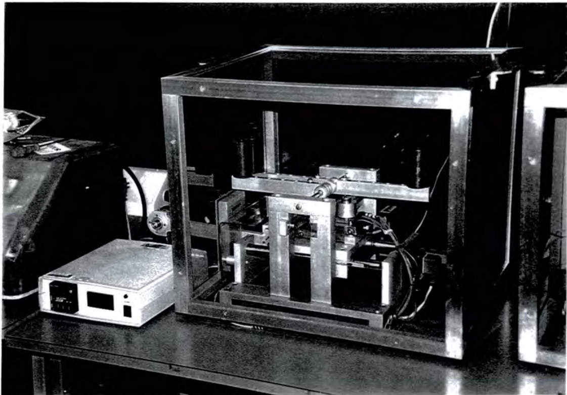
Figure 5.1 Reciprocating pin-on-plate apparatus
