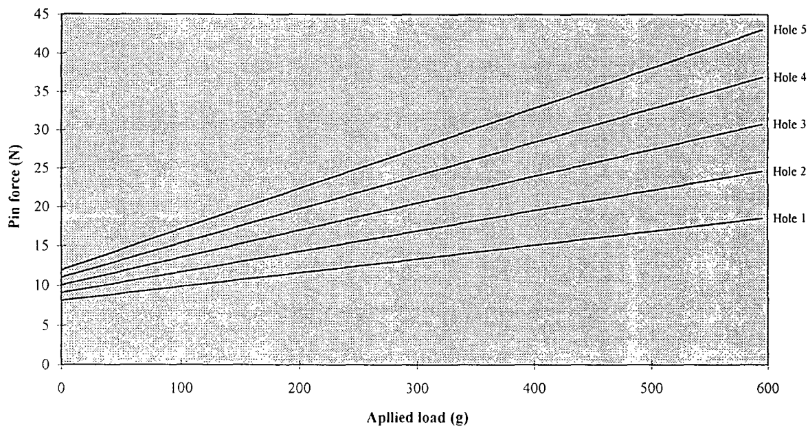
Figure A4.8 Experimental pin forces
