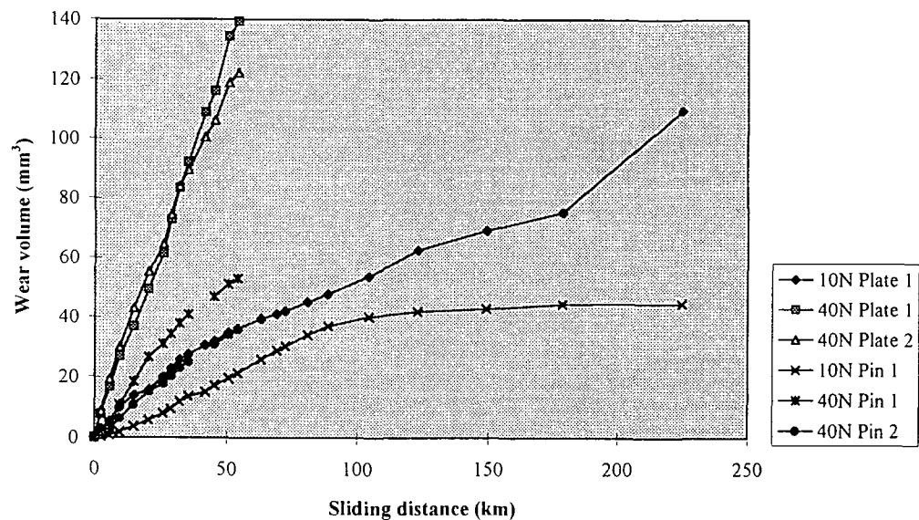
Figure 5.7 : Pin-on-plate test of UHMWPE pins against UHMWPE plates under 10 N and 40 N loading (Test 6)
