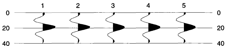
Figure 5.25. Wavelet number 1 is the initial guess wavelet, and wavelets numbered 2-5 are the solution wavelets for the four iterations of inversion run number 4 in Table 5.25. Note that the vertical axis represents the two-way travel-time in ms.
