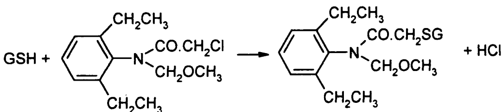
Figure 1.2.4 GSH conjugation of alachlor by nucleophilic displacement
