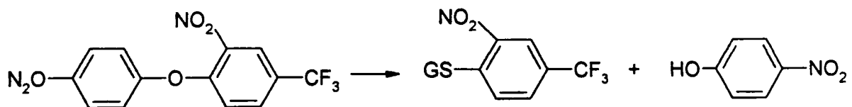
Figure 1.2.5 GSH conjugation of flurodifen by nucleophilic displacement
