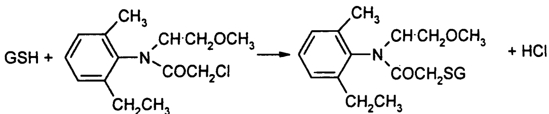
Figure 1.2.3 GSH conjugation of metolachlor by nucleophilic displacement
