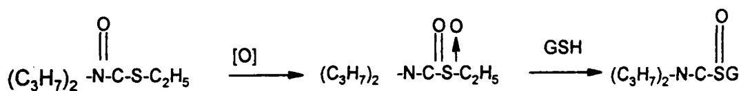
Figure 1.2.1 Metabolism of EPTC in maize
