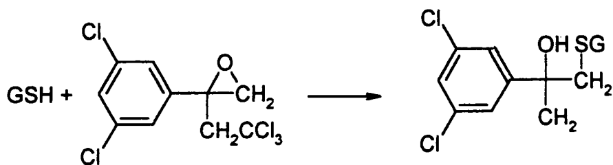
Figure 1.2.6 GSH conjugation of tridiphane by nucleophilic addition
