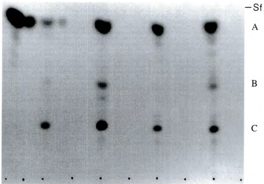
Figure 3.3 An autoradiograph of TLC plates showing the formation of radioactive metabolites of [ ^{14}\text{C} ]-atrazine fed to maize and a range of weed species. Where A = atrazine, B = hydroxyatrazine and C = GS-atrazine. The solvent front (Sf) is indicated and the extracts were derived from Z = Zea mays , P = P. miliaceum , E = E. crus-galli , D = D. sanguinalis , Ab = A. theophrasti , Sorg = S. bicolor , Set = S. faberi , S = sample of purified [ ^{14}\text{C} ]-atrazine and I = a control; incubation of GSH and [ ^{14}\text{C} ]-atrazine.
