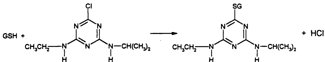
Figure 1.2.2 GSH conjugation of atrazine by nucleophilic displacement
