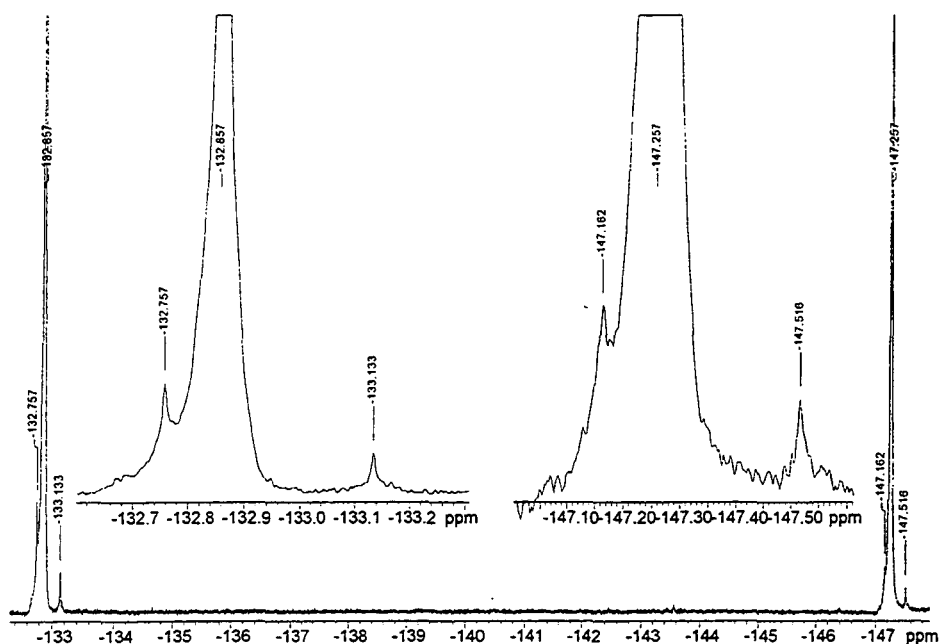
Fig. 3.15 ^{19}\text{F} - \{^1\text{H}\} -NMR spectrum of the S. cattleya supernatant from the [1-^{13}\text{C}] -pyruvate feeding experiment
