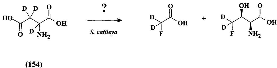
Scheme 18
