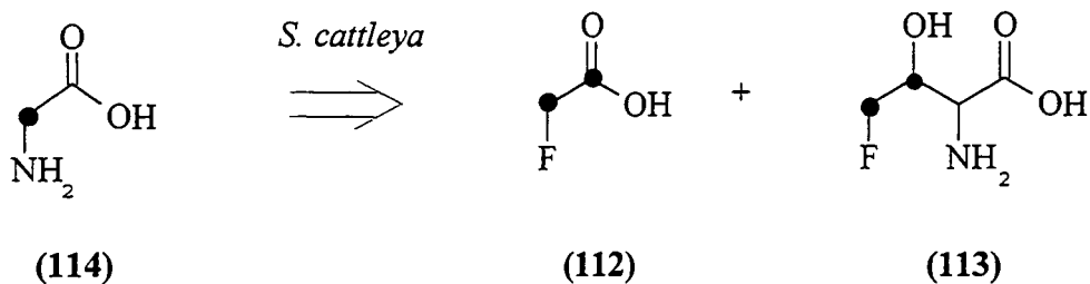
Scheme 8
