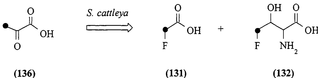
Scheme 12
