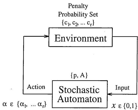
Figure 2.33: Learning Automaton.
