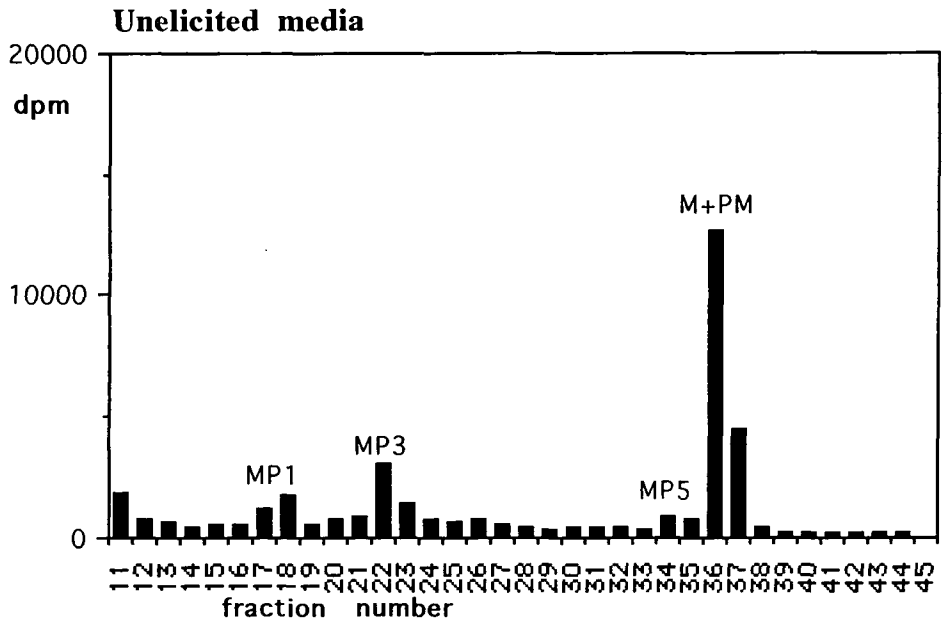
Figure 5.4.3c The distribution of radioactivity between medicarpin and its metabolites in media of (i) elicited cells and (ii) unelicited cells after 8h incubation with [ 3 H-ring]-labelled phytoalexin.
