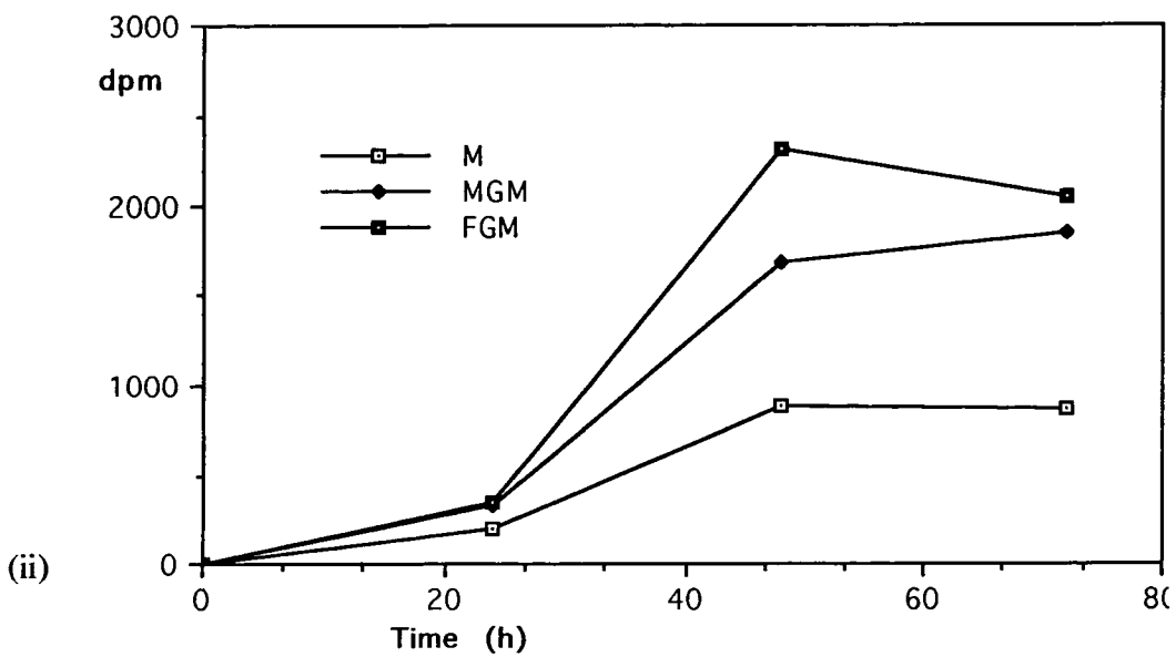
Figure 6.3.4a The incorporation of L-[U- 14 C-phenylalanine into medicarpin, MGM and FGM after treatment with (i) 50 \mu M and (ii) 500 \mu M copper chloride. Data points represent the means of duplicate determinations.
