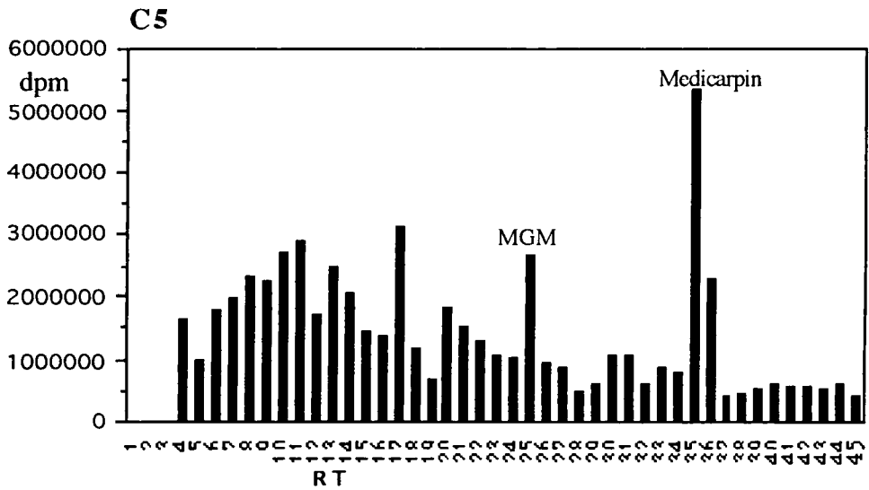
Figure 4.4.3d Incorporation of [ 3 H]-phenylalanine into phenolic compounds in fractions (i)M3 and (ii) C5.
