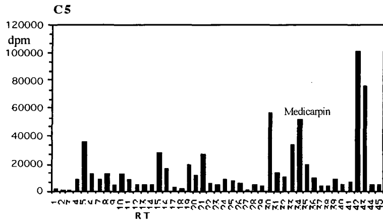
Figure 4.3.3d Incorporation of [ ^3\text{H} -methyl]-methionine into phenolic compounds in fractions (i)M5, (ii)M6 and (iii)C5.
