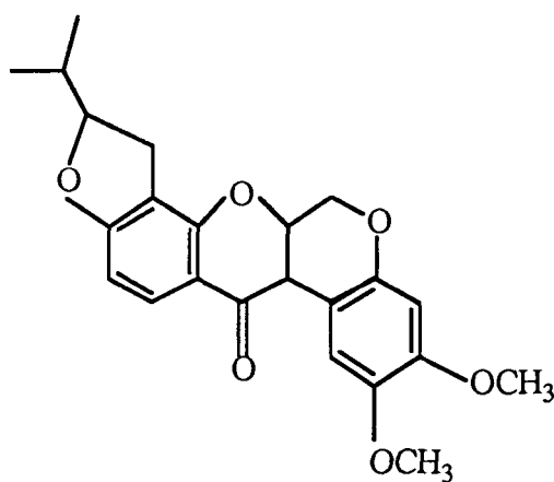
(ii) Rotenone
