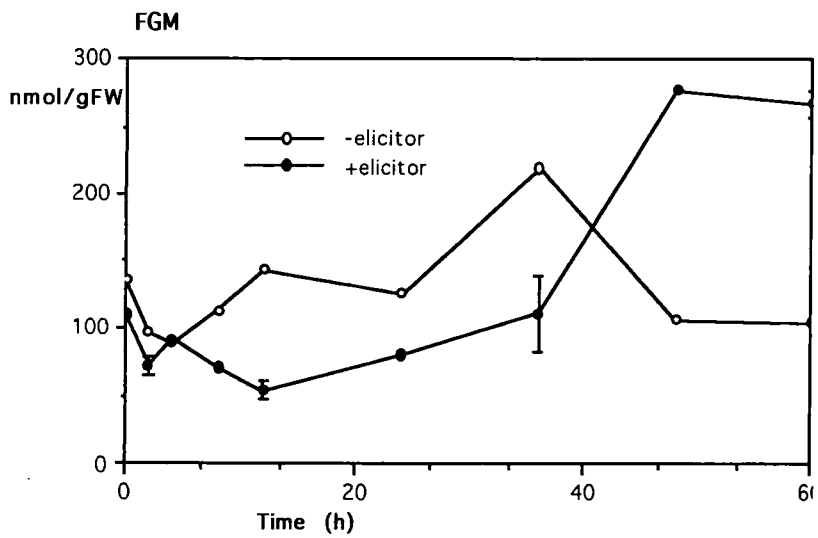
Figure 3.3.3(a) The accumulation and disappearance of (i) medicarpin, (ii) MGM and (iii) FGM in alfalfa cell cultures following elicitor treatment. Data points represent the means of duplicate determinations with the error bars showing variation in the means.
