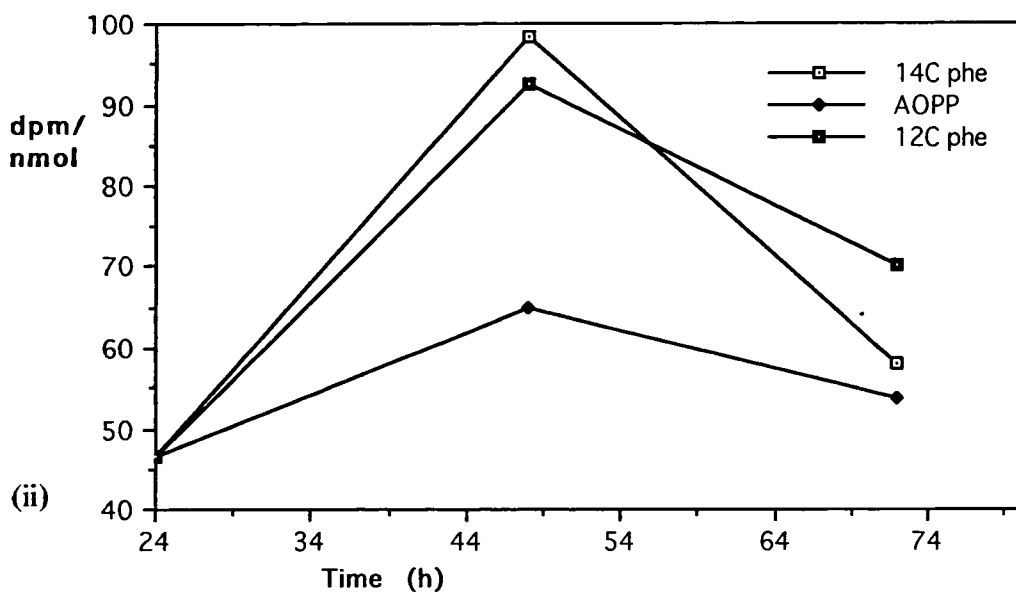
Figure 6.3.4(b) The specific activity of medicarpin in seedlings treated with (i) 50\mu\text{M} and (ii) 500\mu\text{M} copper chloride after continuing treatment with ^{14}\text{C} phenylalanine, treatment with AOPP or treatment with unlabelled phenylalanine. Changes in treatment were initiated at 24h. Data points represent the means of duplicate determinations.
