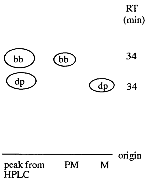
Figure 4.2.3g A diagram of a typical TLC plate showing that although the medicarpin appeared to be pure when analysed by HPLC it could clearly be resolved into two peaks by TLC (chloroform: methanol 98:2). bb=bright blue under UV light ( \lambda 254), dp=dark purple. Authentic medicarpin (M) was dark purple and the unknown compound termed pseudomedicarpin (PM) had a bright blue fluorescence.
