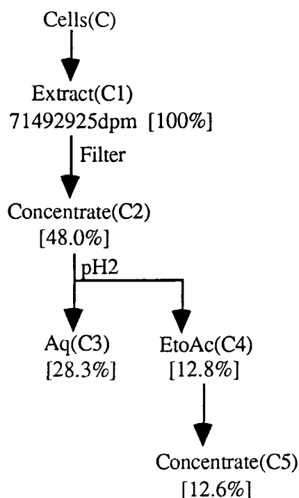
Figure 4.3.3c The distribution of radioactivity during the extraction of cells labelled with [ ^3\text{H} -methyl]-methionine.
