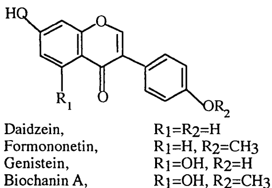
Figure 1.2.1a The isoflavones
