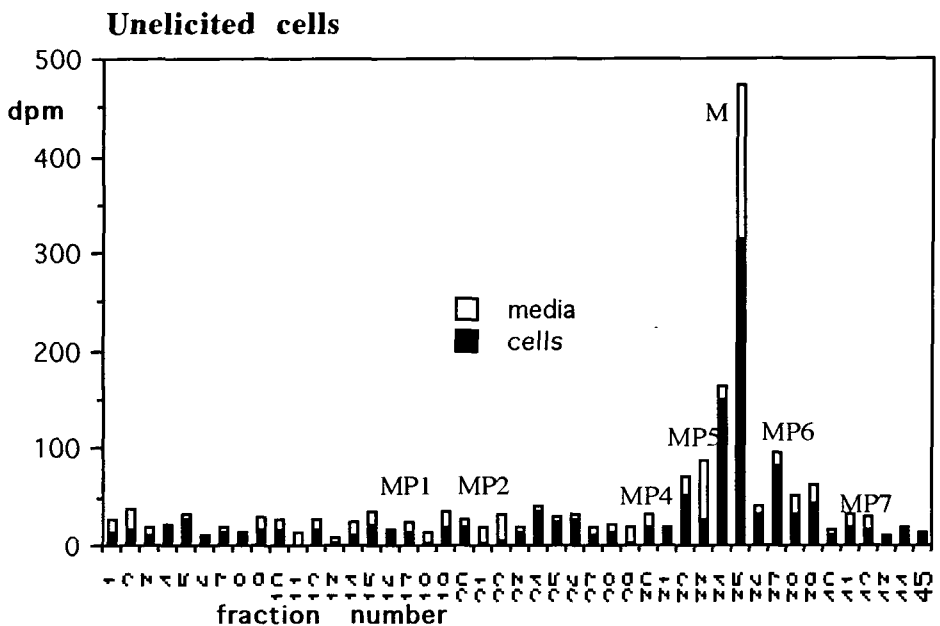
Figure 5.2.3d The distribution of radioactivity between medicarpin and its metabolites as separated by HPLC after a 60 minute incubation of [ ^{14}\text{C} ]-medicarpin with (i) elicitor-treated cells and (ii) untreated cells.
