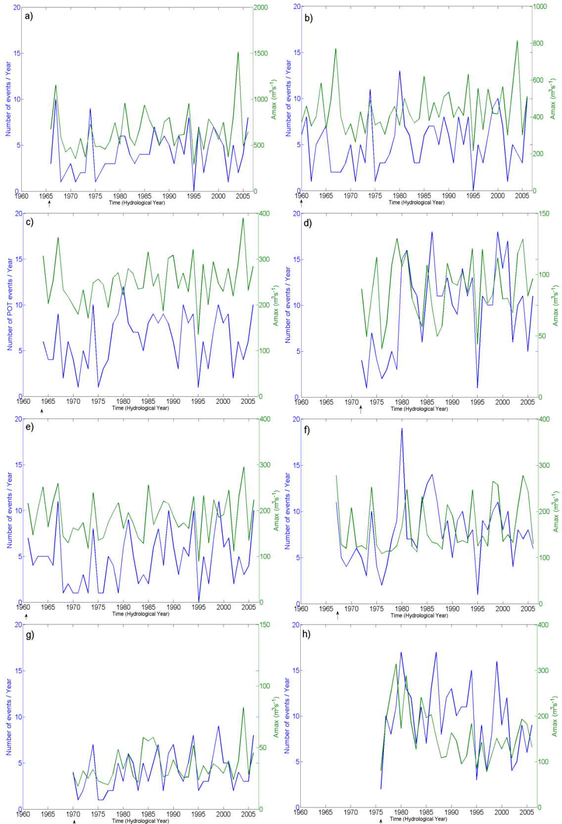
Figure 4.17. Number of >Q1 flood events per hydrological year and the Amax series over time for each gauging station. a) Lower Eden in Carlisle (Sheepmount), b) Lower Eden (Warwick Bridge), c) Upper Eden (Temple Sowerby), d) Upper Eden (Kirkby Stephen), e) Eamont (Udford), f) Irthing (Greenholme), g) Petteril (Harraby Green), and h) Caldew (Cummersdale). Arrows show start of record.
