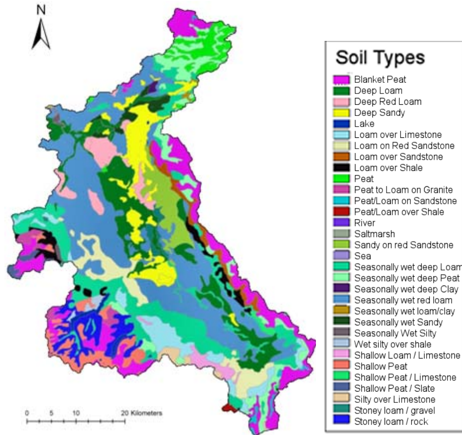
Figure 1.7 Soil types of the Eden Catchment.
