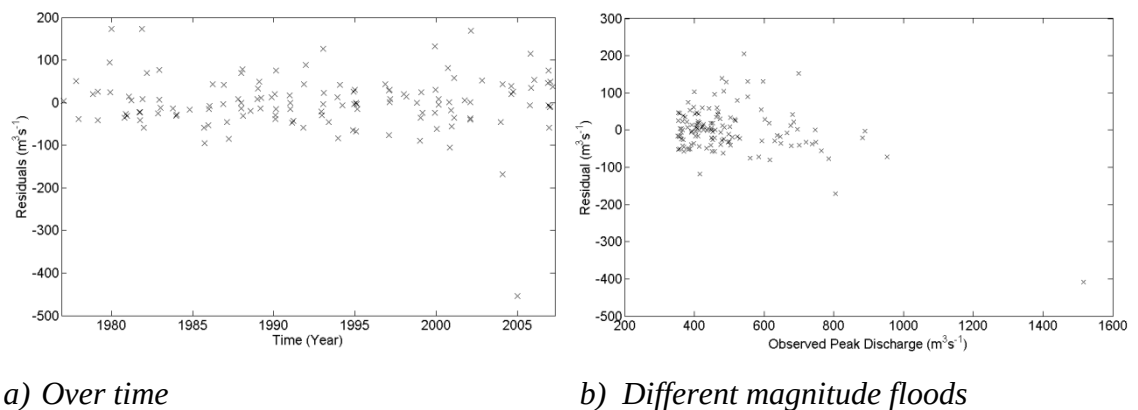
Figure 6.15 Residuals of regression
