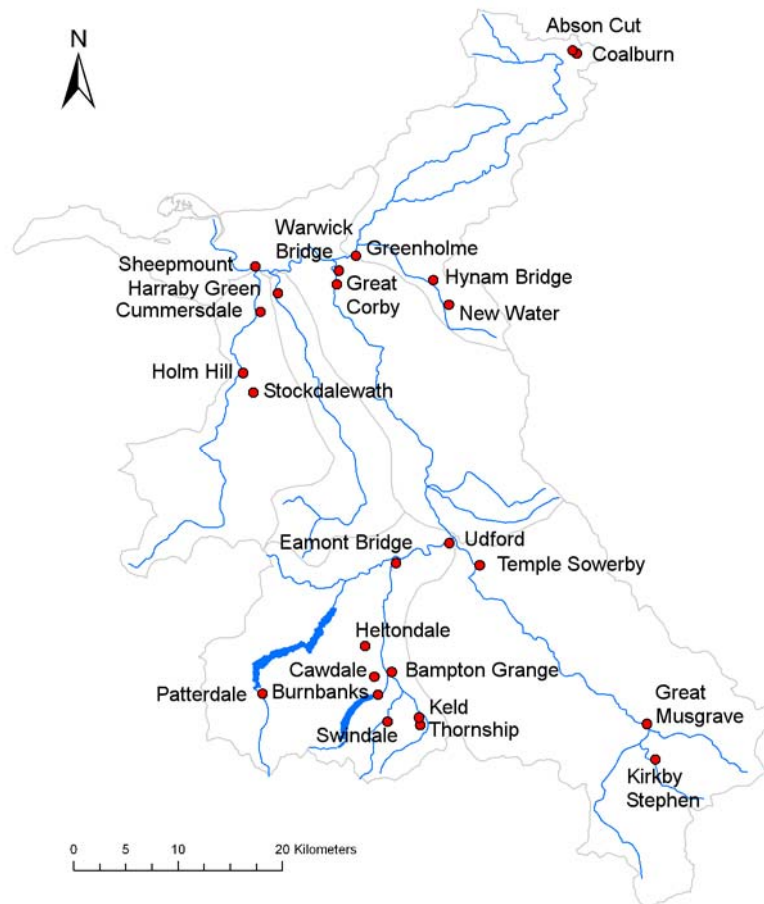
Figure 3.1 Map of gauging stations in the Eden Catchment monitoring stage and with stage-discharge rating curve.
