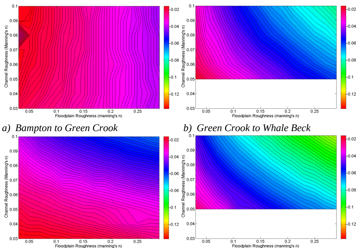
Figure 9.36 Impact of roughness modification on sub-catchment scale (Askham) peak flow magnitude for the 10 th January 2005 flood event. Units are Stage in metres, where negative values are decreases.
