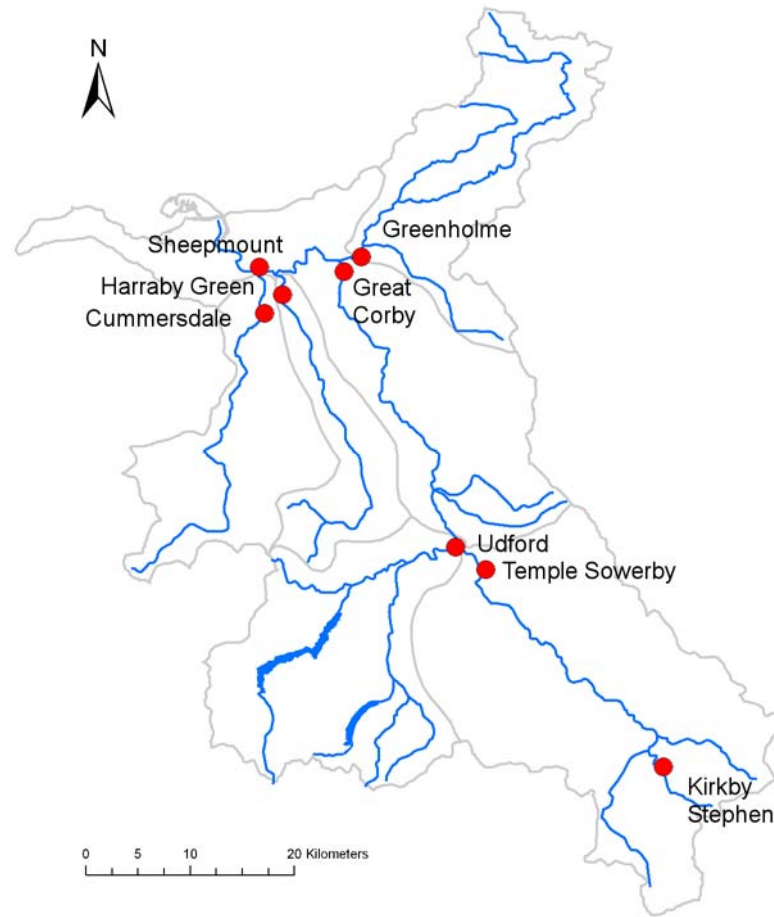
Figure 3.17 Map of chosen discharge gauging stations which will be used through the rest of the thesis.
