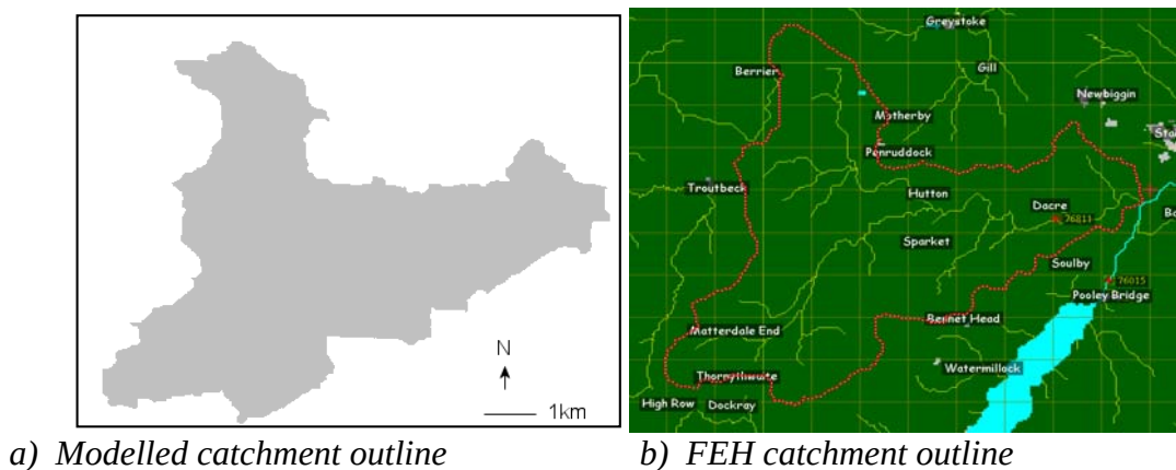
Figure 9.2 Comparison of the catchment area from the modelling and FEH
