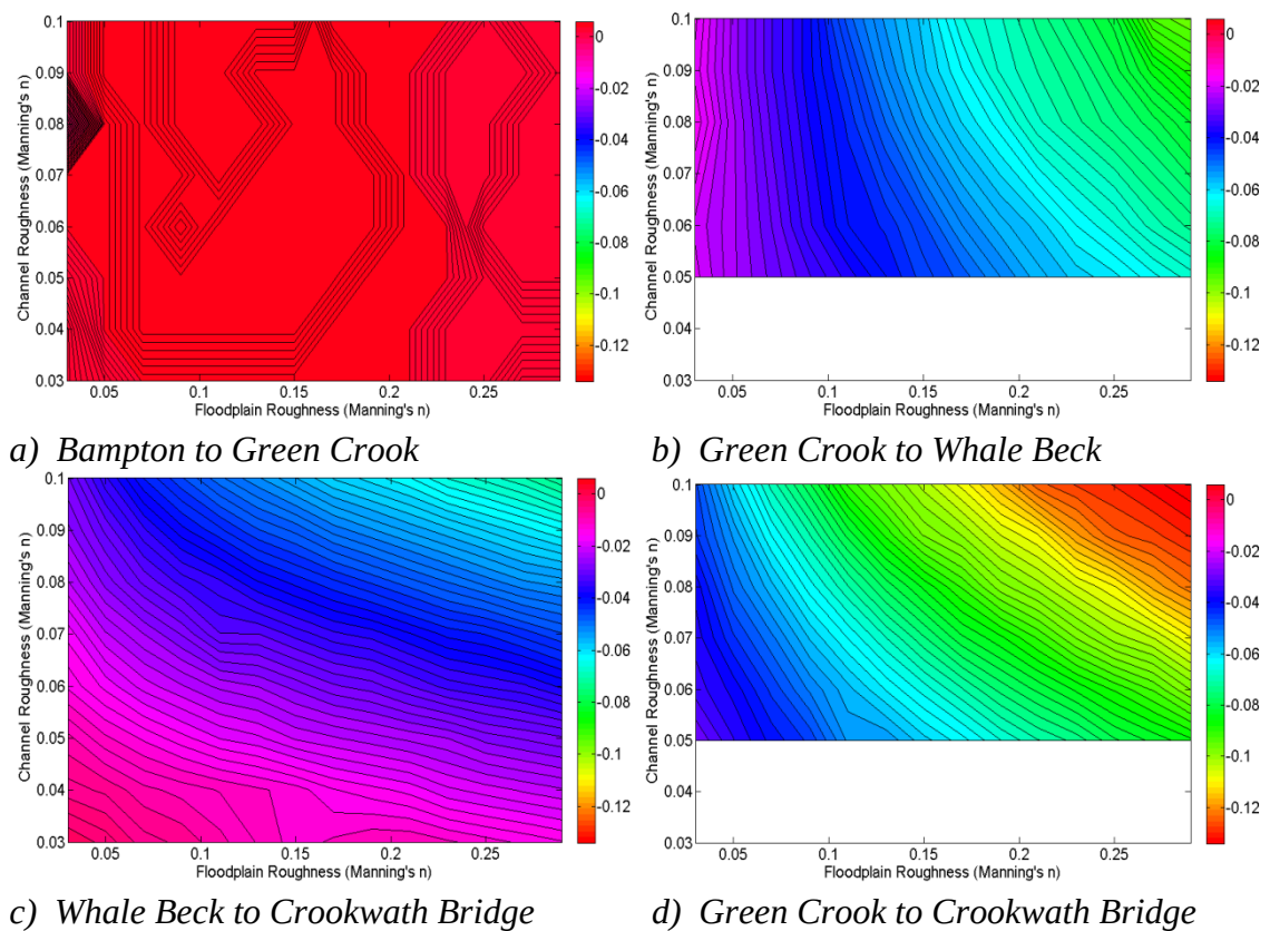
Figure 9.29 Impact of roughness modification on sub-catchment scale (Eamont Bridge) flood magnitude for the 8 th January 2005 flood event. Units are Stage in metres, where negative values are decreases.
