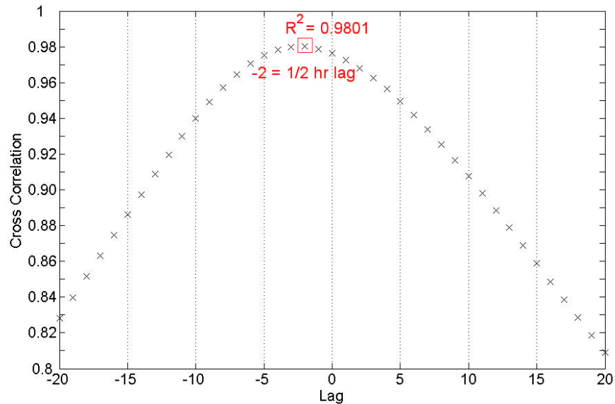
Figure 3.22 Cross correlation plot between Holm Hill and Cummersdale gauging stations. Lag refers to the data point number, which have a time step of 15 minutes. Therefore when lag = -2 = -2 * 15 = -30 minutes.
