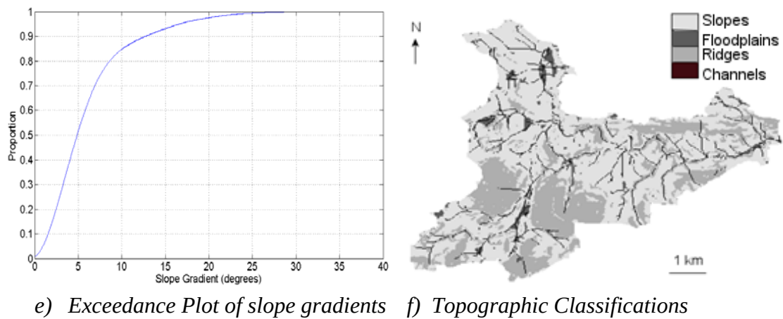
Figure 9.1 Catchment characteristics for input into CRUM3 model
