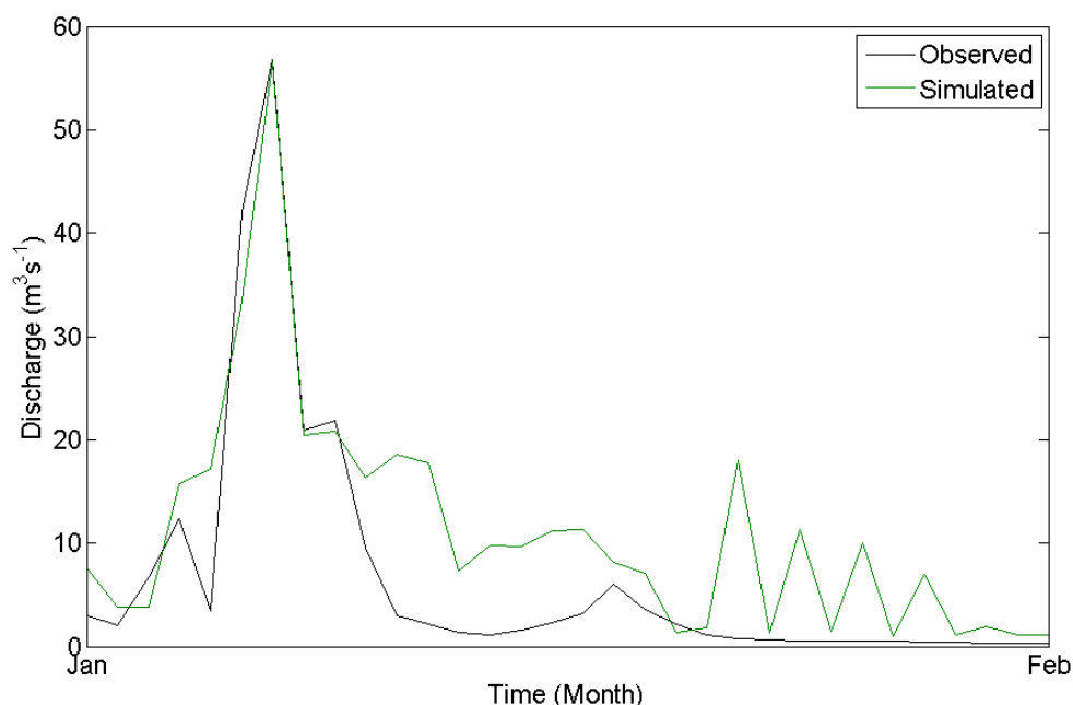
Figure 9.4b Validation of CRUM3 for the month January 2005, comparing simulated and observed discharges at Dacre Bridge
