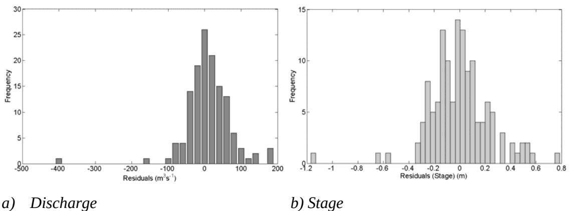
Figure 6.16 Histogram of regression residuals
