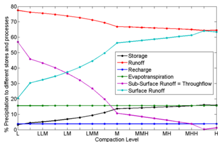
Figure 9.10 Proportion of rainfall that is partitioned into different hydrological processes
