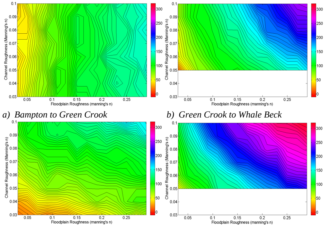
Figure 9.37 Impact of roughness modification on sub-catchment scale (Askham) peak flow timing for the 10 th January 2005 flood event.
