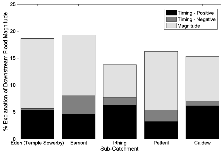
Figure 6.11 Contribution of each sub-catchment in terms of peak flow magnitude and timing in explaining downstream flood risk.
