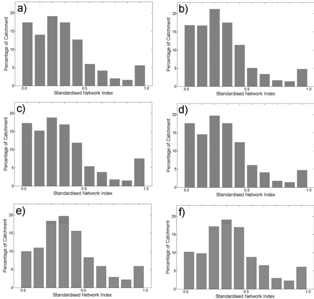
Figure 7.13 Frequency distributions for the network index of various sub-catchments of the Eden a) Whole Eden; b) Upper Eden; c) Eamont; d) Irthing; e) Petteril; and f) Caldew
