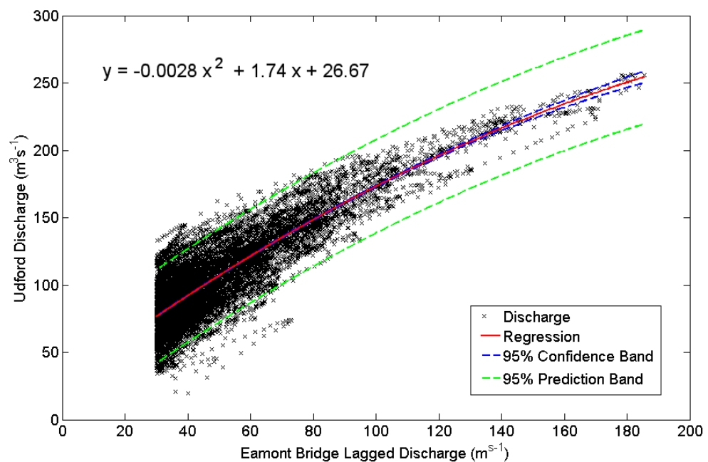
Figure 3.25 Scatter plot showing relation between delayed Eamont Bridge and Udford discharges.
