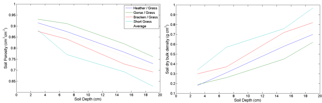
b) Soil porosities with soil depth
