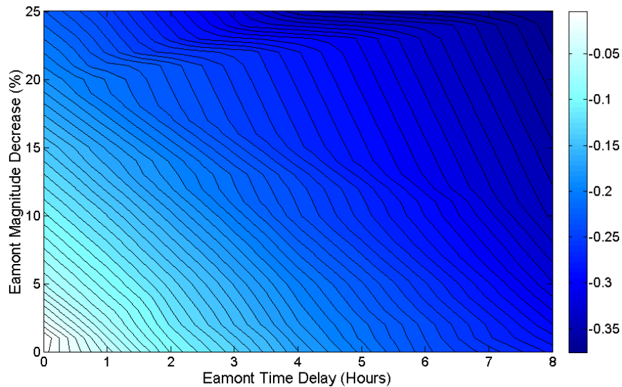
Figure 6.31 Sensitivity of peak stage at Sheepmount to both timing delays and magnitude reductions of the Eamont
