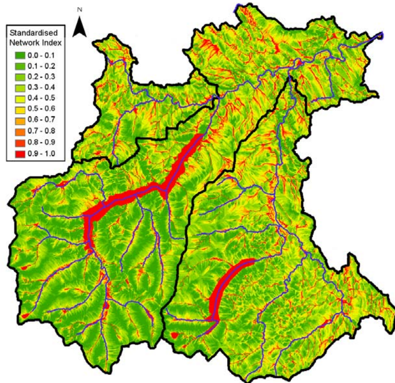
Figure 7.14 Network Index of the Eamont sub-catchment
