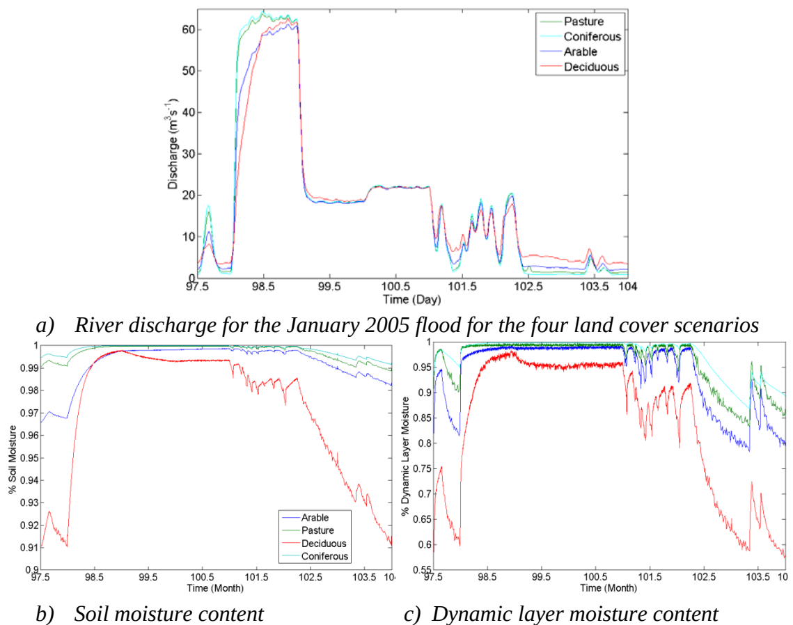
Figure 9.21 River flow and soil saturation levels for the January 2005 flood for the four land cover scenarios.
