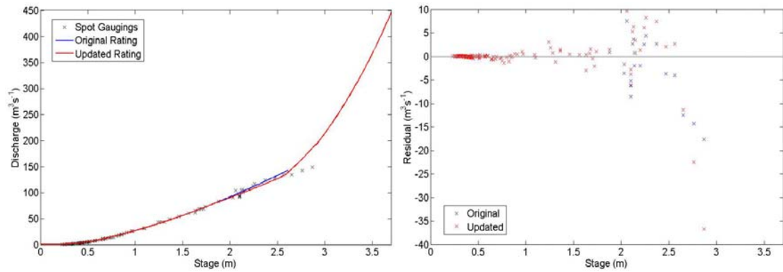
a) Rating curve and spot gaugings b) Residuals of spot gauging from curve Figure 3.13 Assessment of the Cummersdale rating curve
