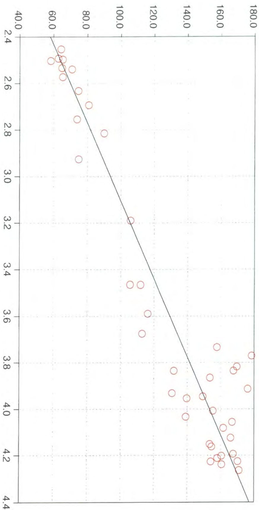
Figure 8.4.1 - Scatterplot of d(HY) versus a(HX_1Y) for short X-H\cdots\pi contacts.
