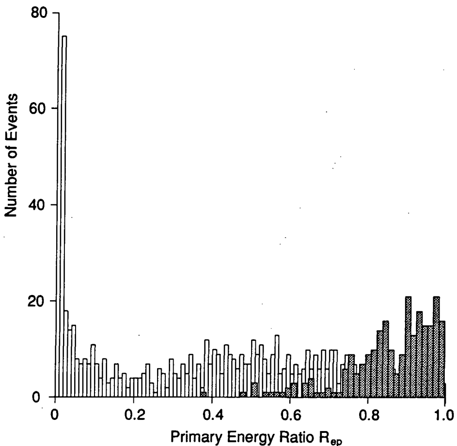
Figure 5.6: Distribution of the primary energy Ratio, R_{ep} , for simulations of EAS with gamma ray (shaded) and hadron primaries.
