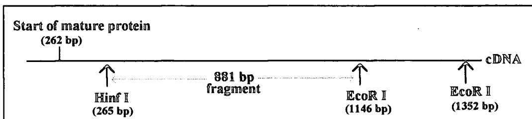
Figure 3.1 Positions of EcoR I and Hinf I restriction sites in Brassica napus seed enoyl-ACP reductase cDNA (λEAR7).
