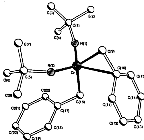
Fig. 1 Molecular structure of 1, without H atoms and with atom labels. Selected dimensions (Å and ^\circ ): \text{Cr}\text{--N}(1) 1.625(2), \text{Cr}\text{--N}(2) 1.632(2), \text{Cr}\text{--C}(9) 2.071(2), \text{Cr}\text{--C}(10) 2.357(2), \text{Cr}\text{--C}(16) 2.096(3), \text{C}(9)\text{--C}(10) 1.443(3), \text{C}(10)\text{--C}(11) 1.411(3), \text{C}(10)\text{--C}(15) 1.406(3), other \text{C}\text{--C} in this ligand in range 1.371(3)–1.384(3), \text{C}(16)\text{--C}(17) 1.475(3), other \text{C}\text{--C} in this ligand in range 1.375(3)–1.402(3); \text{N}(1)\text{--Cr}\text{--N}(2) 116.09(8)^\circ , \text{C}(9)\text{--Cr}\text{--C}(10) 82.16(11)^\circ , \text{C}(9)\text{--Cr}\text{--C}(16) 131.93(8)^\circ , \text{C}(10)\text{--Cr}\text{--C}(16) 94.86(7)^\circ , \text{Cr}\text{--N}(1)\text{--C}(1) 166.07(13)^\circ , \text{Cr}\text{--N}(2)\text{--C}(5) 160.60(13)^\circ , \text{Cr}\text{--C}(9)\text{--C}(10) 82.16(11)^\circ , \text{Cr}\text{--C}(16)\text{--C}(17) 114.73(13)^\circ .
