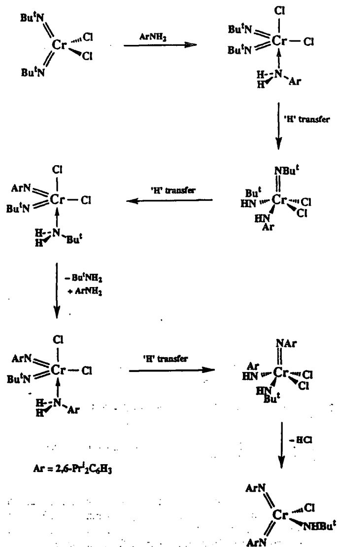
Scheme 1. A plausible mechanism for the formation of 1.
