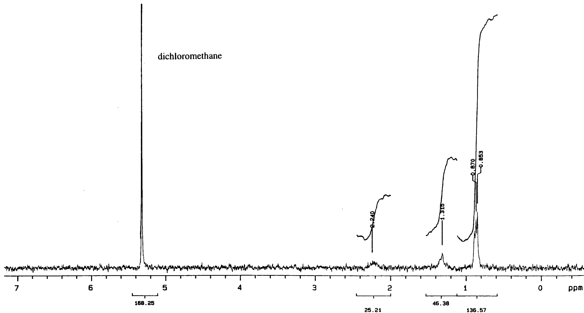
^2\text{H} NMR spectrum of piliformic acid after feeding perdeuterated butyric acid
