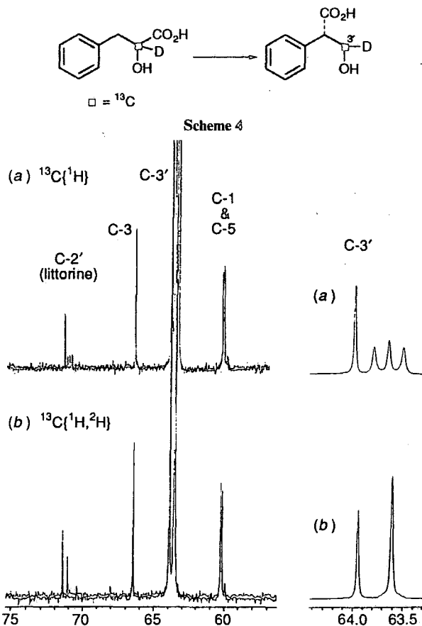
Fig. 1 (a) ^{13}\text{C}\{^1\text{H}\} and (b) ^{13}\text{C}\{^1\text{H},^2\text{H}\} NMR spectra of hyoscyamine after incorporation of sodium DL-3-phenyl[2- ^{13}\text{C} ,2- ^2\text{H} ]lactate. The ^{13}\text{C} - ^2\text{H} incorporation is evident by a triplet in spectrum (a) at \delta 63.6, upfield from the ^{13}\text{C} -signal assigned to C-3' of tropate at \delta 63.9. The triplet collapses to a singlet in spectrum (b) (see inset for clarification). The triplet at \delta 71.5 in spectrum (a) also collapses to a singlet in spectrum (b), 0.35 ppm upfield from the enriched uncoupled signal corresponding to C-2' of littorine. The signals from C-1, C-3 and C-5 of hyoscyamine are also shown.
