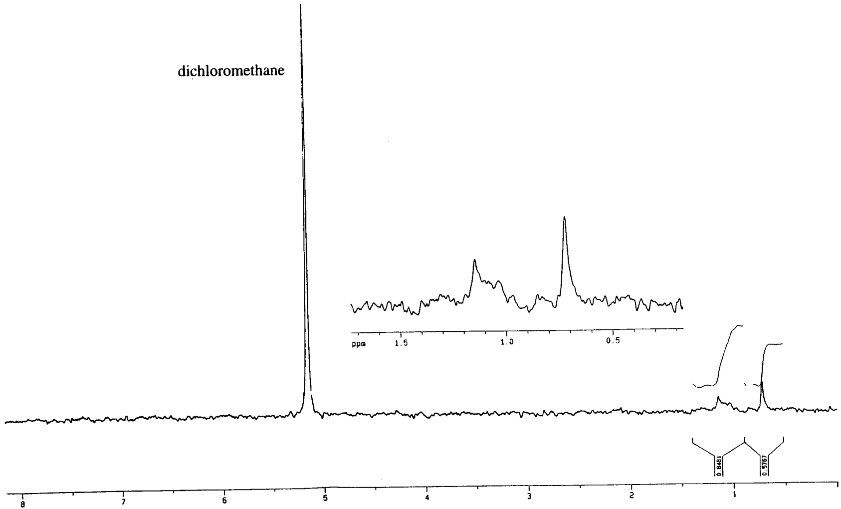
^2\text{H} NMR spectrum of piliformic acid after feeding [1\text{-}^{13}\text{C}, 2\text{-}^2\text{H}] -octanoic acid
