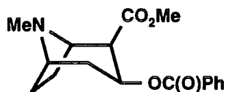
cocaine (9)
