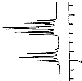
tropic acid
