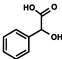
mandelic acid (47)
