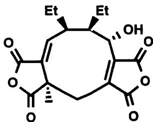
glauconic acid (95) Penicillium purpurogenum
