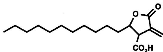
nephrosterinic acid (86) Cetraria endocrocea
