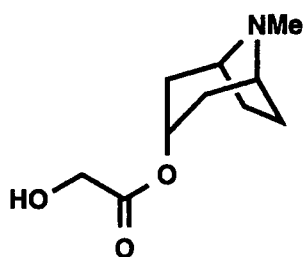
2'-hydroxyacetoxytropine (34)
