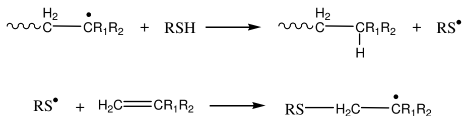
Figure 1.4: Chain transfer mechanism using a thiol CTA.
