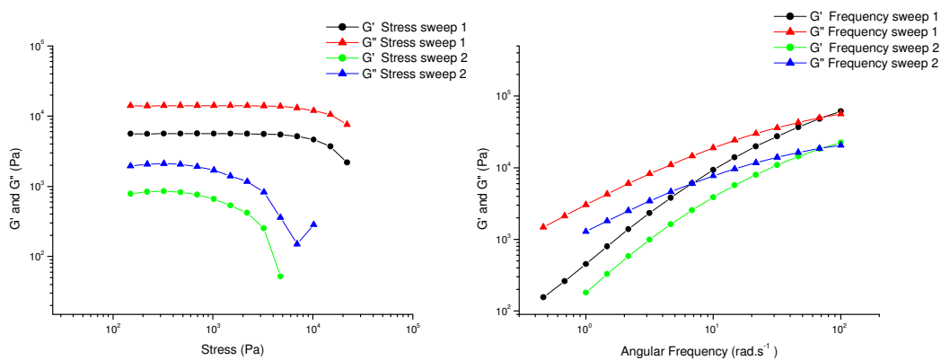
Figure 5.15: First and second, stress and frequency sweeps for PMMA.
