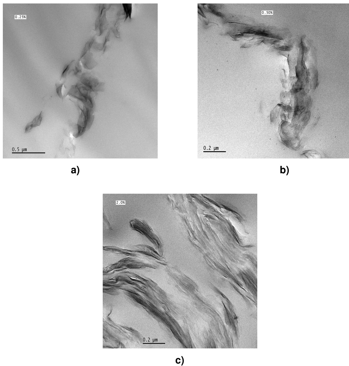
Figure A.1: TEM images of a) 0.25% C15a on a 0.5 μm scale, b) 0.5% C15a and c) 2% C15a on a 0.2 μm scale.
