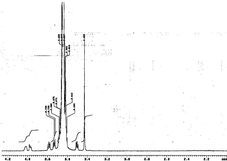
Figure A.10: ^1\text{H} NMR of 5K mono functionalised quaternary amino PEO.
