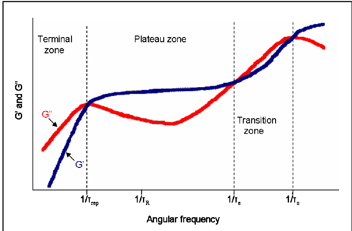
Figure 2.8: Master curve of an entangled polymer. Where \tau_{\text{rep}} is the reptation relaxation time, \tau_{\text{R}} is the Rouse relaxation time, \tau_e is the entangled Rouse relaxation time and \tau_0 is the Kuhn monomer relaxation time.
