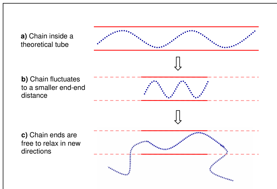
Figure 1.10: Schematic diagram of the contour length fluctuation process.
