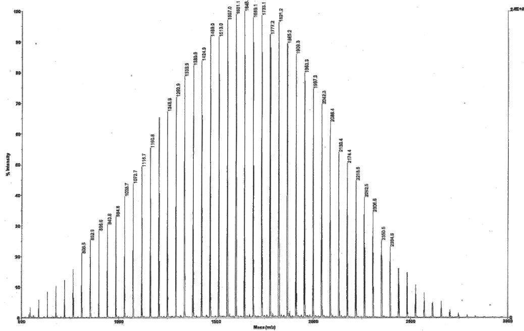
Figure A. 12: MALDI-ToF spectra of 1.6K mono functionalised amino PEO.
