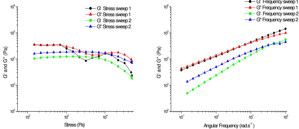
Figure A.7: First and second, stress and frequency sweeps for 0.5% LRD.
