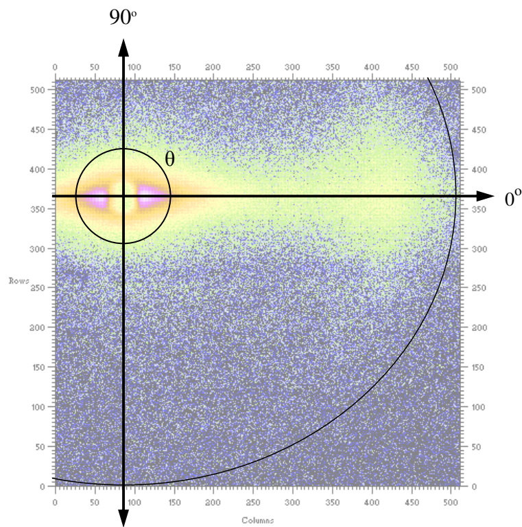
Figure 4.22: Illustration of SAXS scattering axis.
