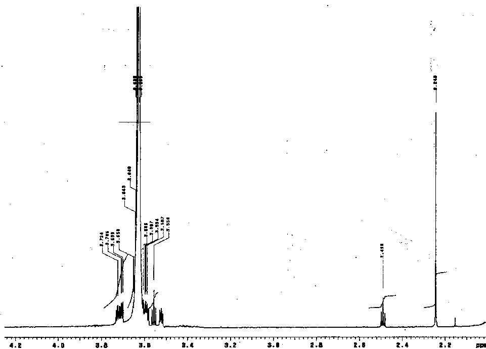
Figure A.9: ^1\text{H} NMR of 5K mono functionalised amino PEO.
