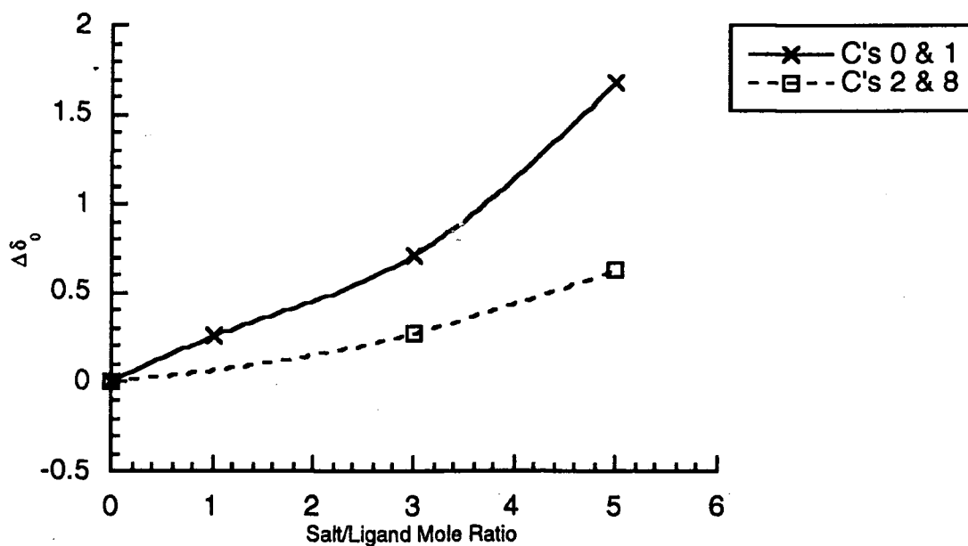
Figure 4.4 Chemical Shift Change Measured at Reduced Ligand Concentration and Increased Salt Concentration. No "limiting shift" is detectable
