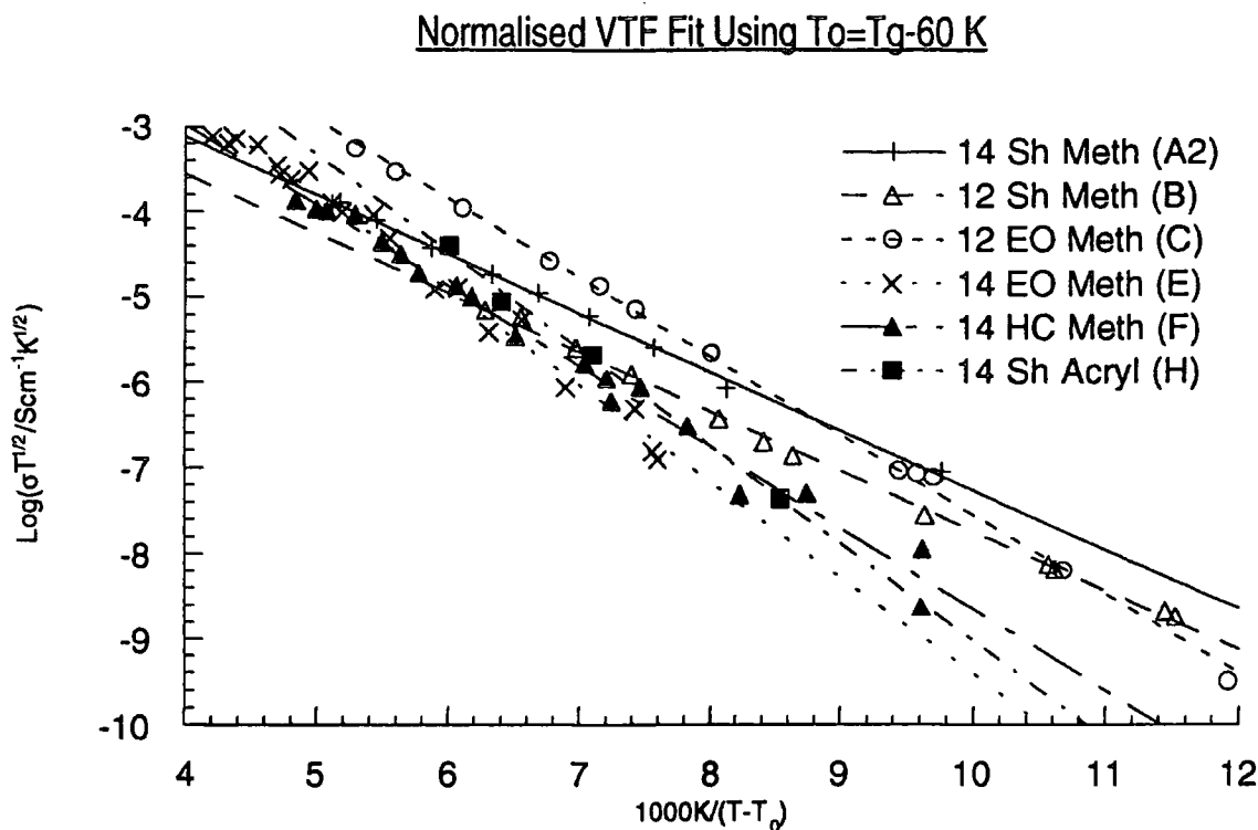
Figure 4.13(a) Normalised VTF plot, constructed from the first set of polymer conductivity data using T_0 = T_g - 60\text{K}
