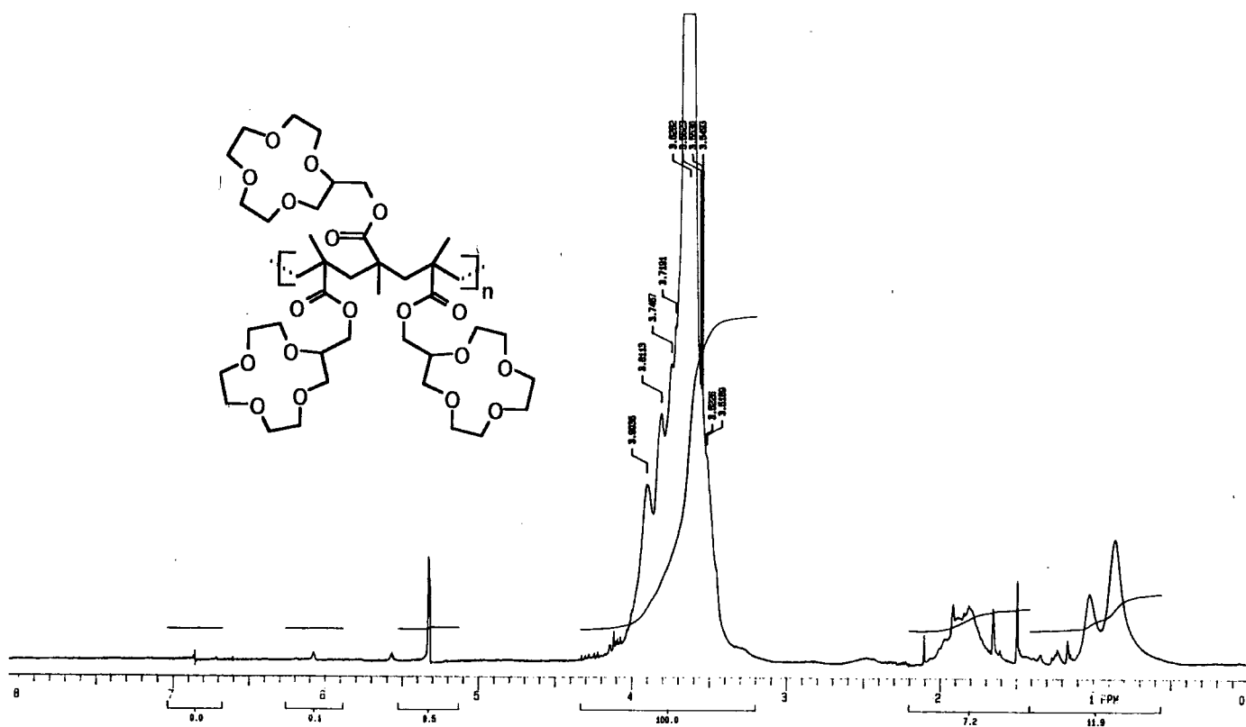
Figure 2.3(b) Proton NMR Spectrum of Polymer (B) in \text{CD}_2\text{Cl}_2
