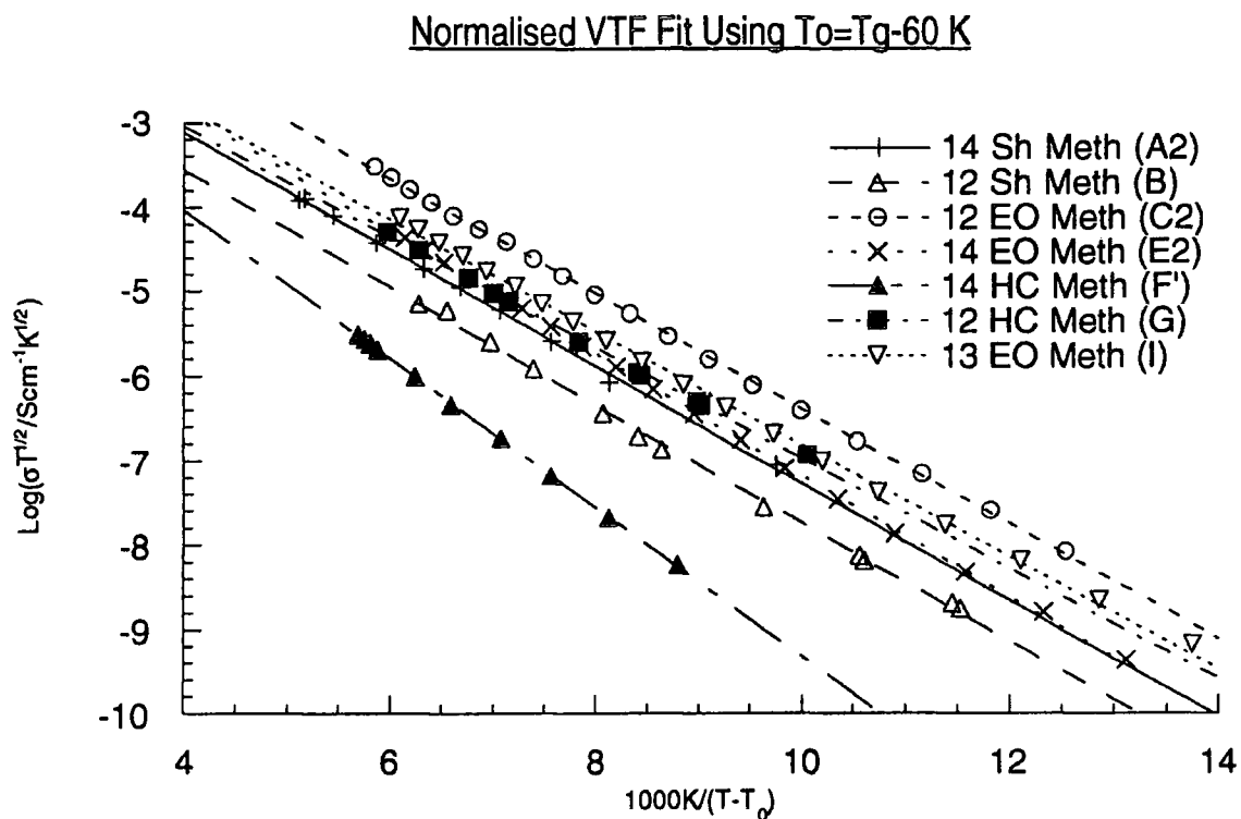
Figure 4.14a) Normalised VTF plot, constructed from the revised set of polymer conductivity data using T_0 = T_g - 60 K
