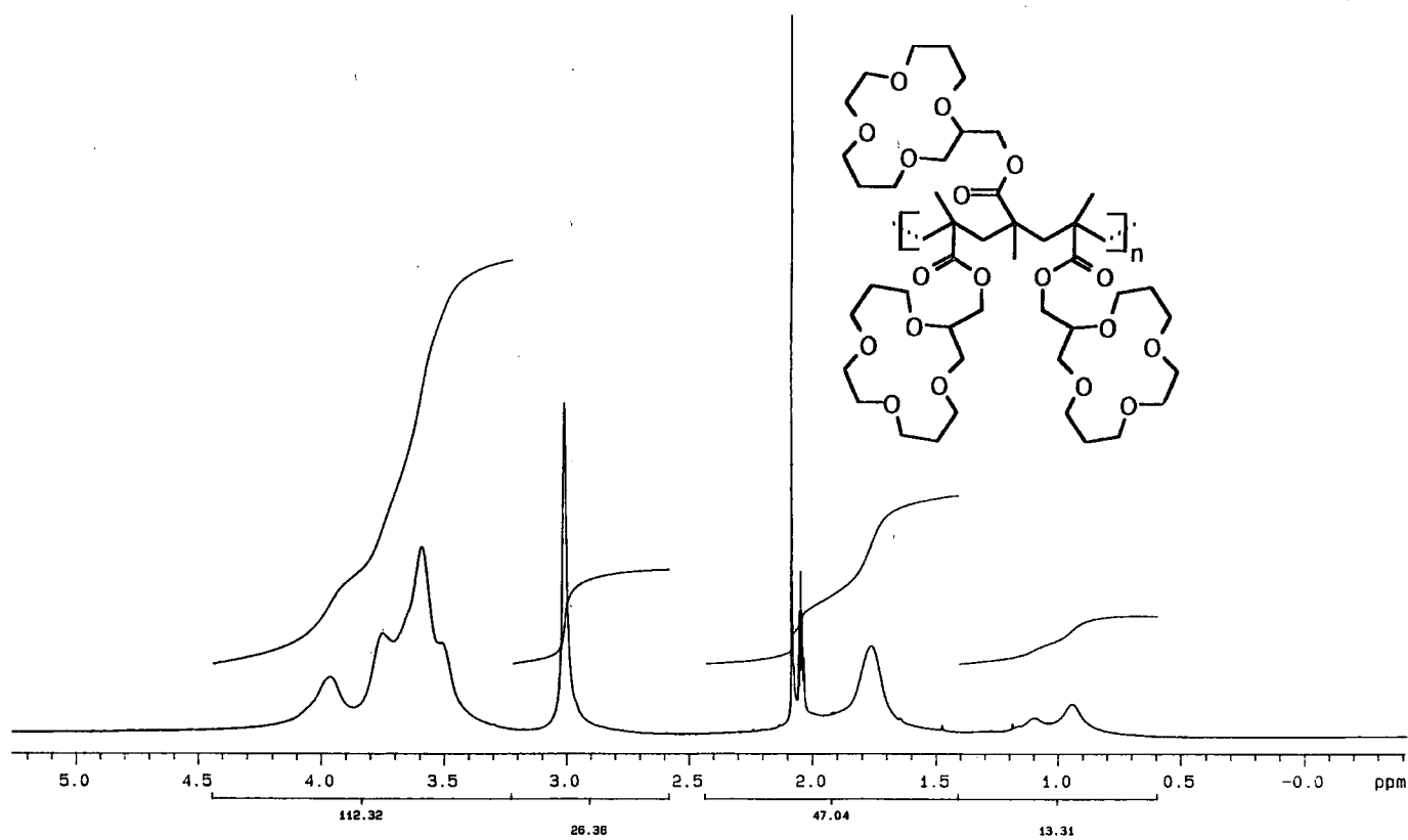
Figure 2.3(a) Proton NMR Spectrum of Polymer (A) in (\text{CD}_3)_2\text{CO}
