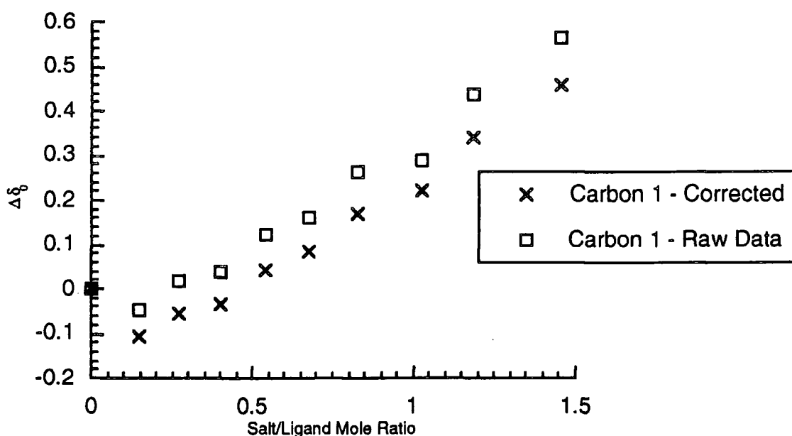
Figure 4.2 Change in Carbon-13 Chemical shift of C-1 (raw data) and in the shift difference between C-1 and C-11 (corrected) on addition of LiClO 4
