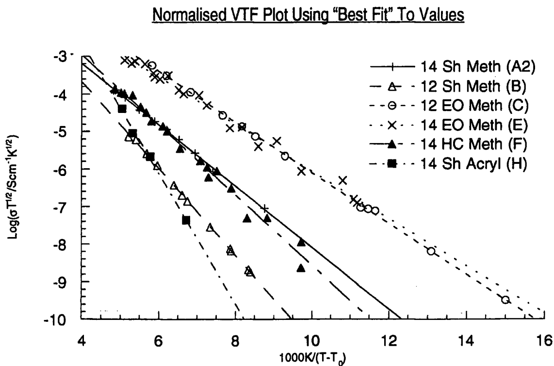
Figure 4.13(b) Normalised VTF plot, constructed from the first set of polymer conductivity data using "Best Fit" T_0 values
