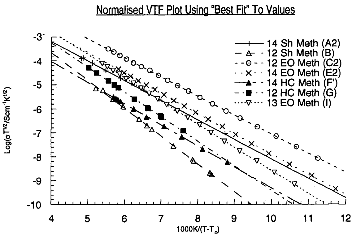
Figure 4.14b) Normalised VTF plot, constructed from the revised set of polymer conductivity data using "Best Fit" T_0 values
