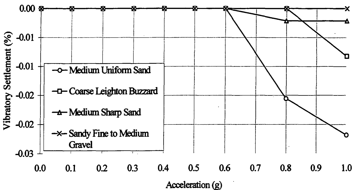
Figure 5.2.2. Partially saturated vibration test settlement results, at 25Hz and 10kPa (see Appendix 3: Table A3.4.3; A3.6.4; A3.7.3, A3.11.6 for test data sheet).
