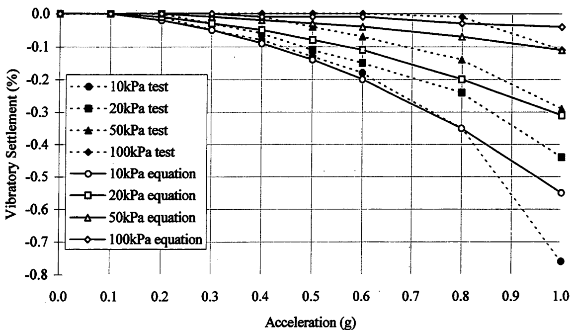
Figure 5.9.1b. Comparison between vibration test settlement and derived equivalent values (medium Leighton Buzzard sand, saturated, 40Hz).
