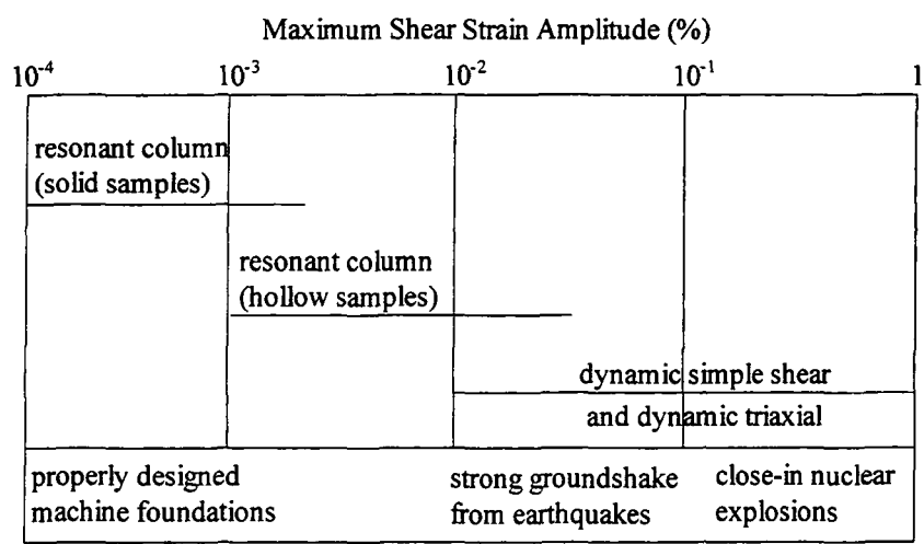
Figure 3.8. Laboratory methods for determining shear stress-strain properties of cohesionless soil (After Silver and Seed, 1971a).
