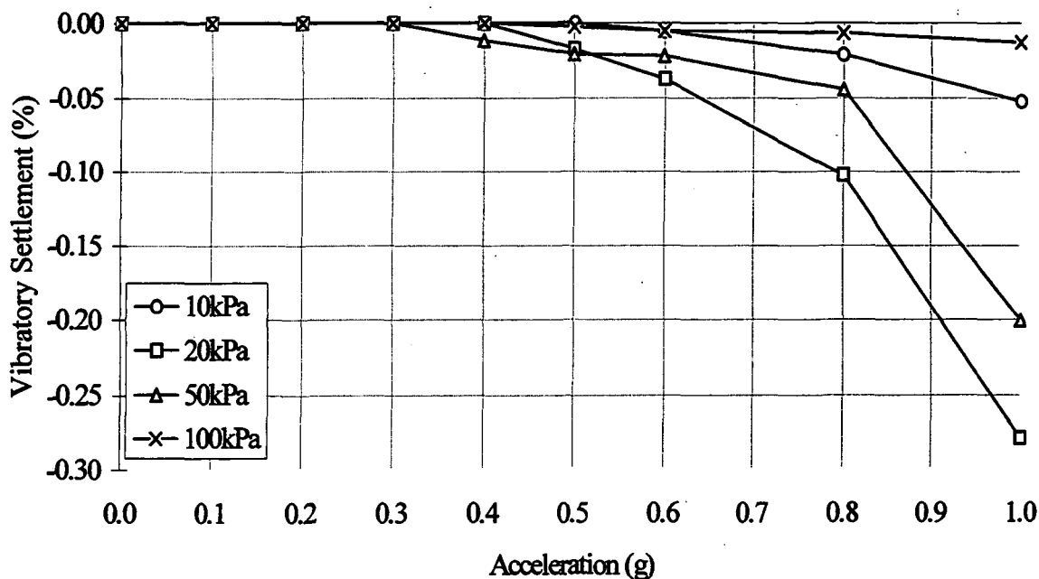
Figure 5.1.6b. Coarse Leighton Buzzard sand vibration test settlement results. Saturated, at 40Hz (see Appendix 3: Table A3.6.2, for test data sheet).
