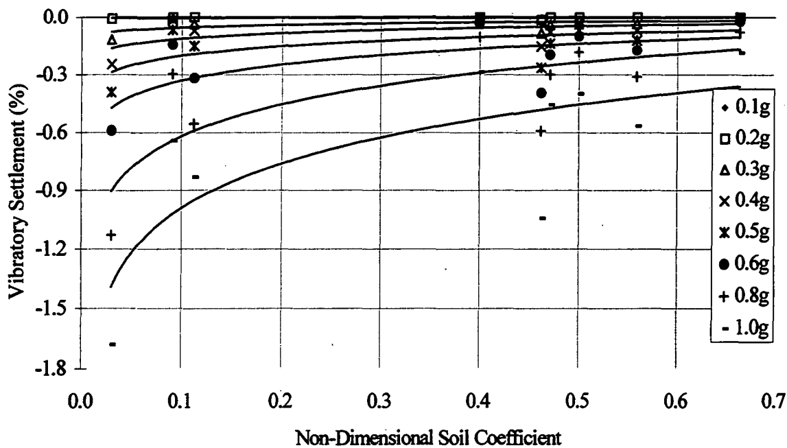
Figure 5.7.3a. Relationship between the non-dimensional coefficient ( D_x ) and settlement (mean stress values, saturated, 25Hz).
