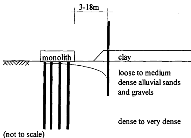
Figure 6.23. Cross-section of piling near existing structure (Paper #3).
