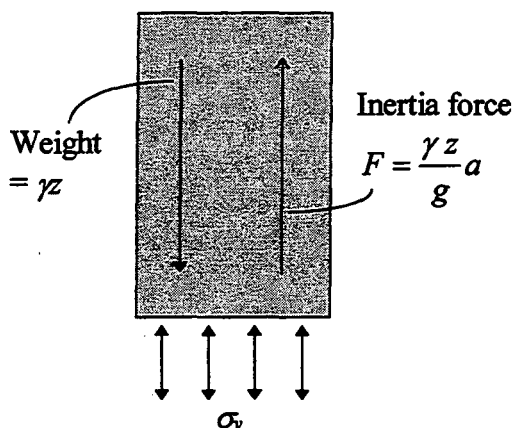
Figure 3.17. Forces acting upon a soil unit during vertical vibration, without vertical confining stress. Where: \gamma = soil unit weight; z = height of soil unit; g = acceleration due to gravity; a = applied acceleration; \sigma_v = vertical vibration.
