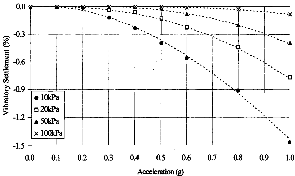
Figure 5.6.2a. Vibration settlement response of a protosoil to static stress (saturated, 25Hz).
