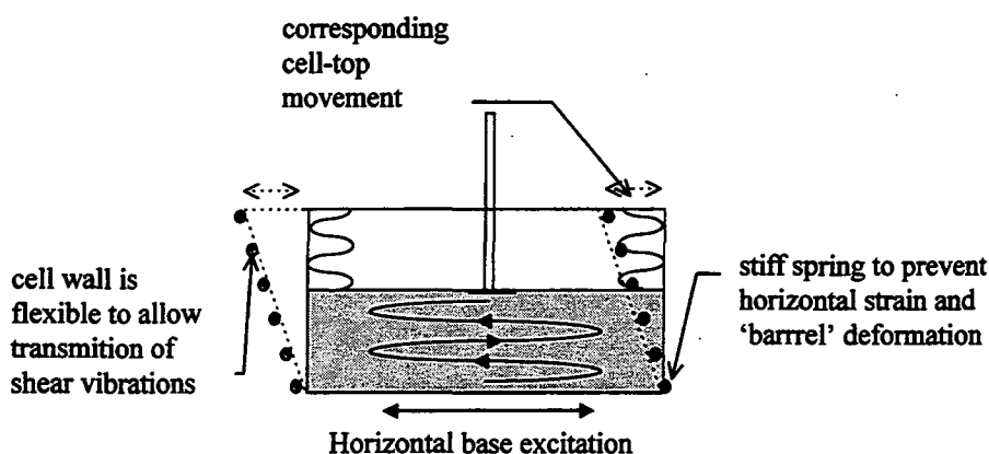
Figure 6.7. Illustrating Rowe cell modification to enable simple shear wave testing.
