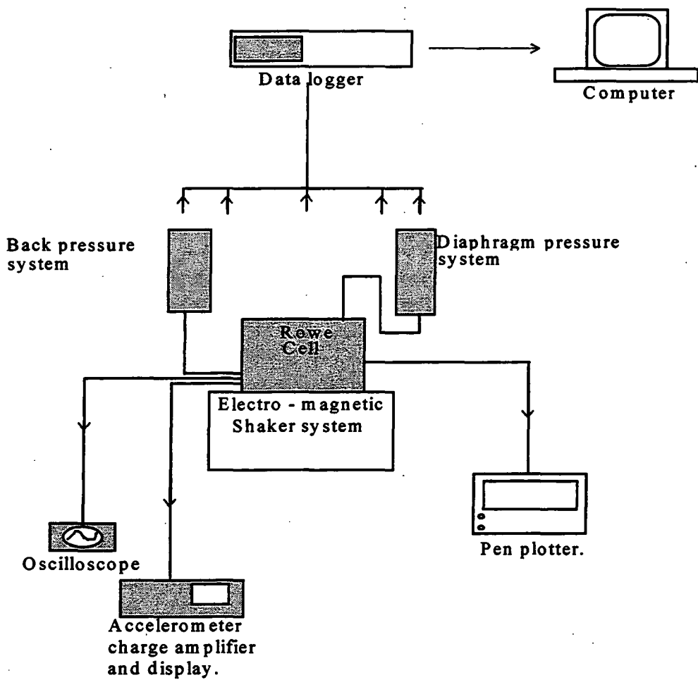
Figure 4.8 The complete laboratory system (see Plate 4.2).
