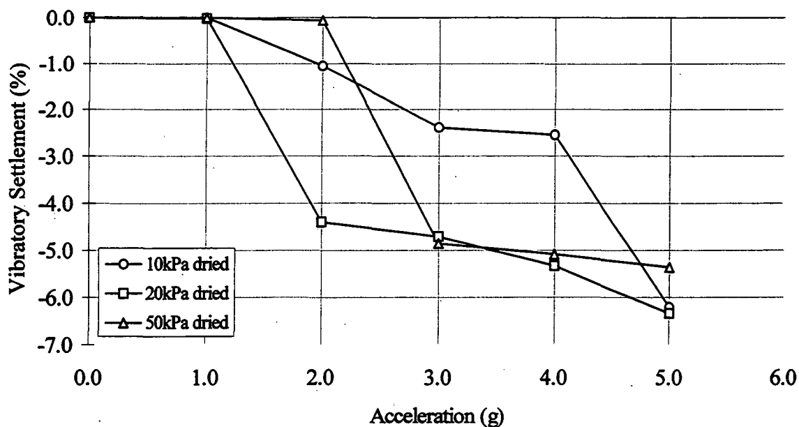
Figure 5.4.1. Silty fine sand dried high acceleration vibration test settlement results, at 25Hz.(see Appendix 3: Table A3.1.4, for test data sheet).
