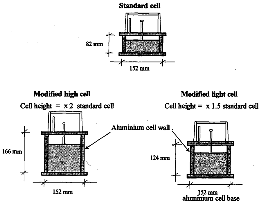
Figure 4.5. The dimensions of the available Rowe cells (see Plate 4.13).
