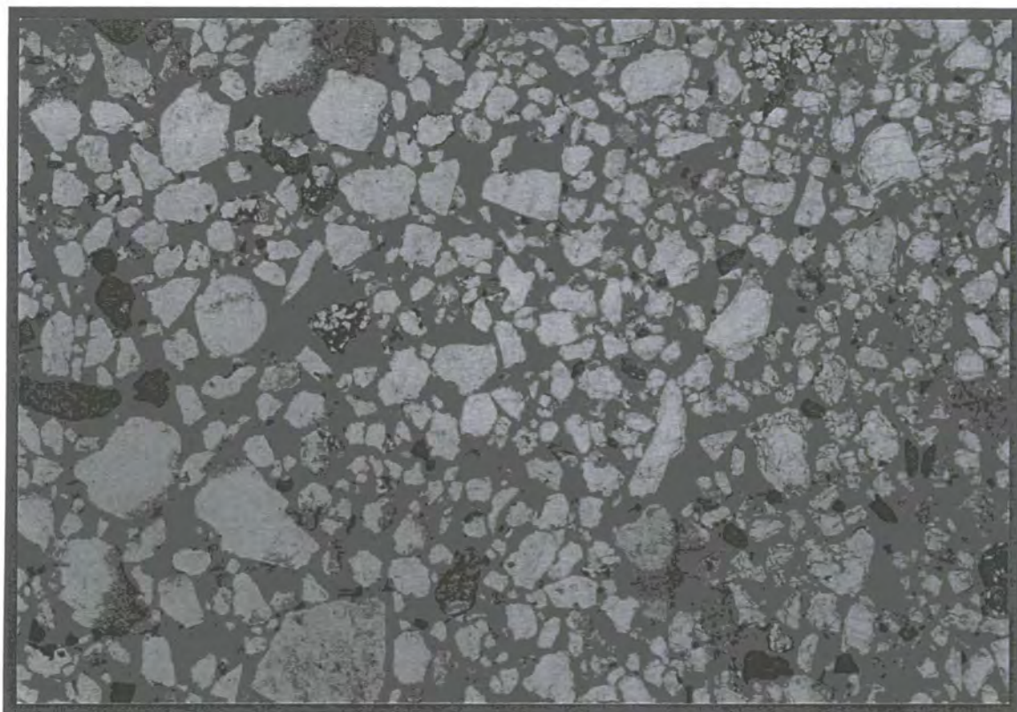
Plate 4.12. Thin-section of medium sharp sand (x 25 magnification).
