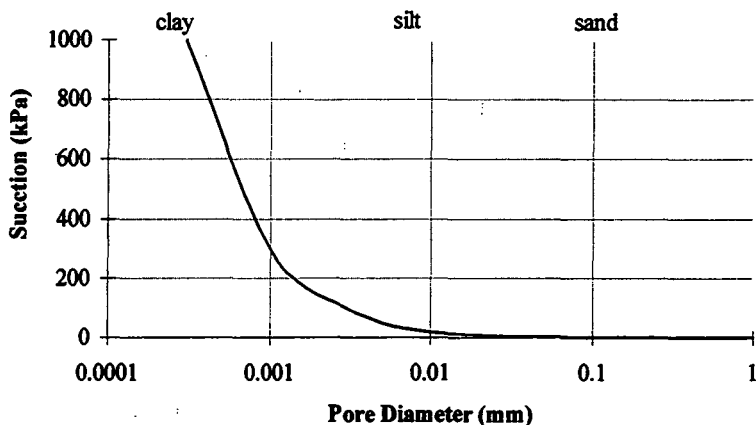
Figure 3.4. The influence of pore size diameter on limiting values of suction for a soil with uniformly shaped pores (from Toll et al. , 1987).
