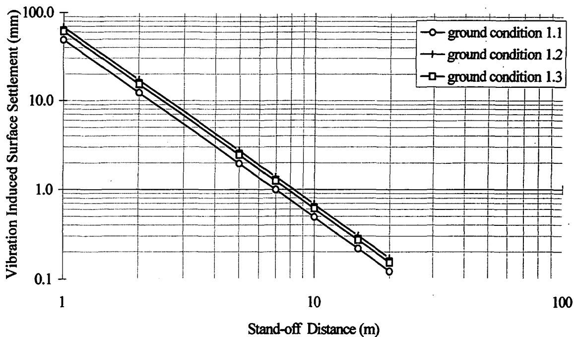
Figure 5.11.6a. Effect of varying ground condition 1.1 on surface settlement (vibrodriver 1) (see Appendix 4: Tables 4.1.1 - 4.1.3 for test data sheets).
