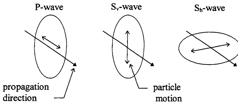
Figure 2.4. Particle motion due to different body waves.
