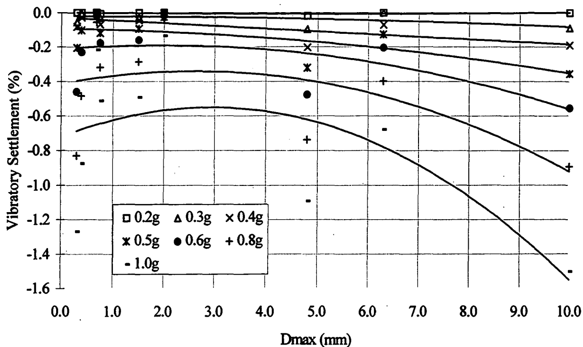
Figure 5.7.1b. Relationship between maximum particle size ( D_{max} ) and settlement (mean stress values, saturated, 40Hz).
