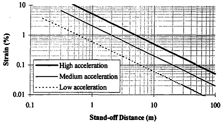
Figure 3.25. Vertical strain induced in loose to medium sand by vibratory sheetpile driving (Clough and O'Rourke, 1990).
