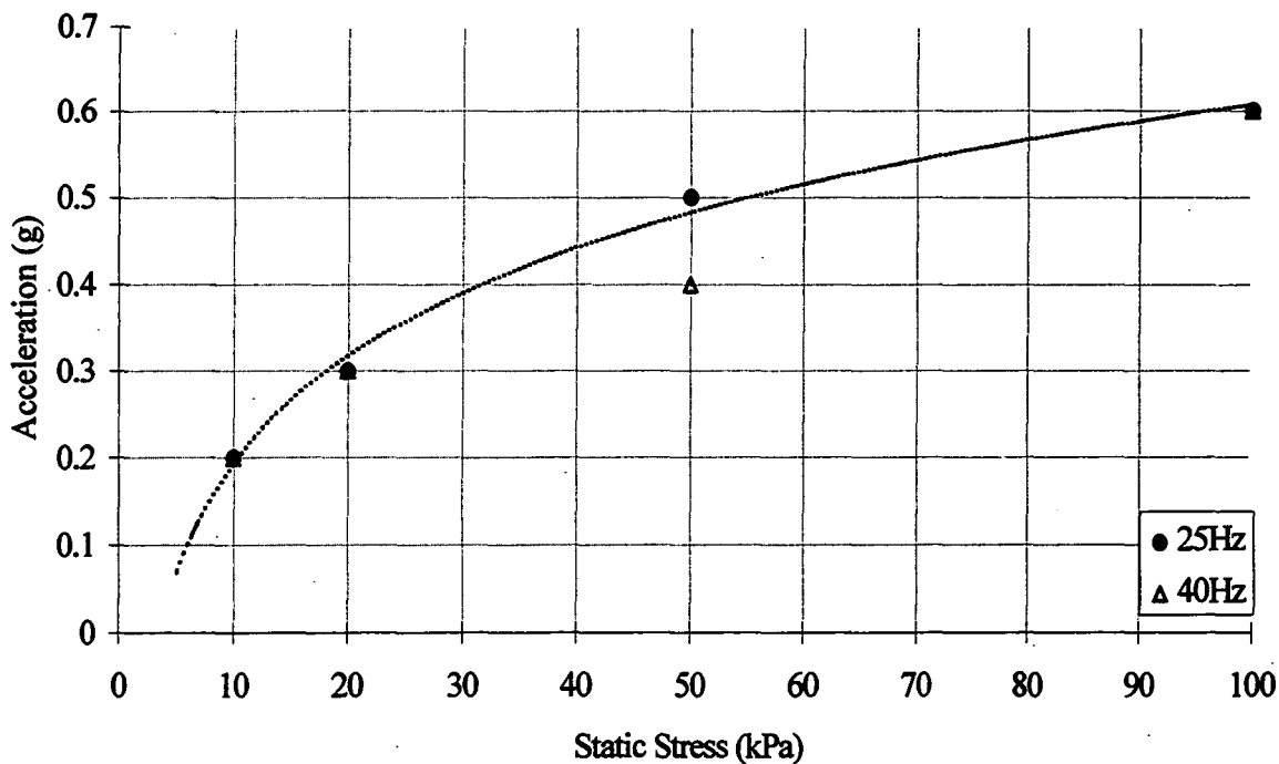
Figure 5.6.4. Minimum level of acceleration that induces initial soil settlement (protosoil, saturated).
