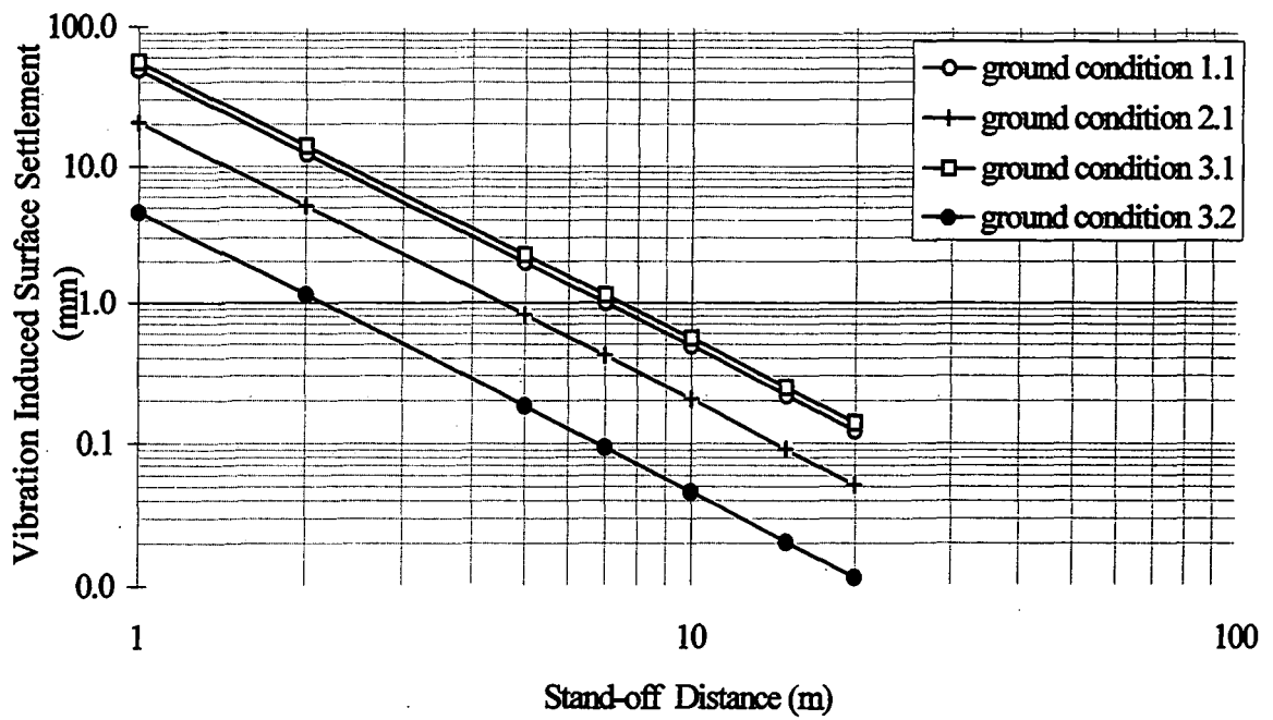
Figure 5.11.7a. Effect of varying ground conditions on surface settlement vibrodriver 1) (see Appendix 4: Tables 4.1.1, 4.1.4, 4.1.5 for test data sheets).
