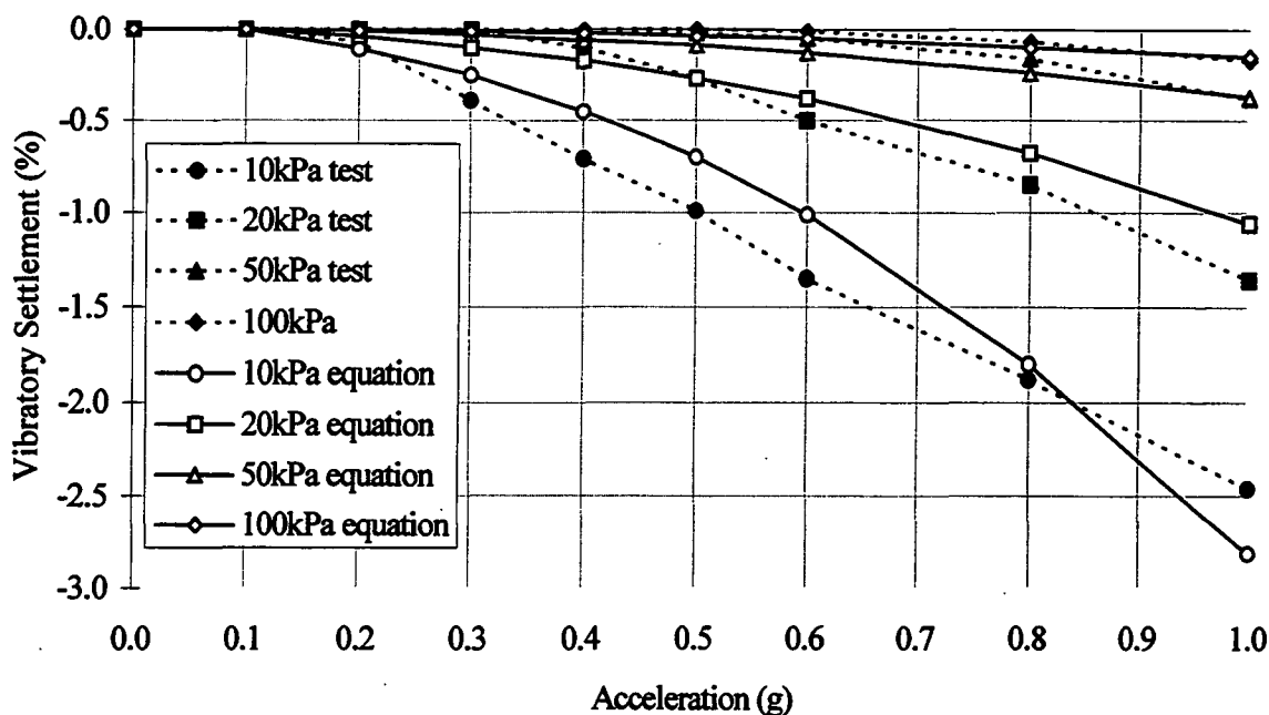
Figure 5.9.1c. Comparison between vibration test settlement and derived equivalent values (medium sharp sand, saturated, 25Hz).
