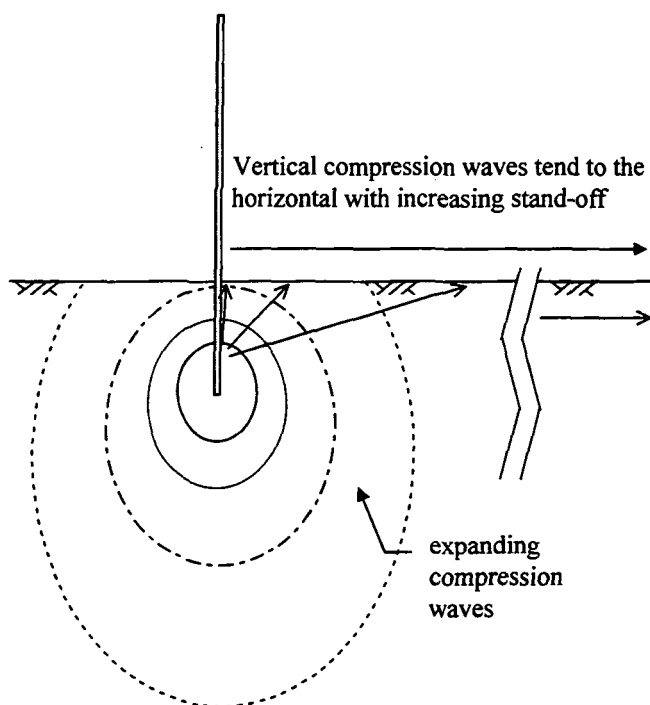
Figure 6.6 Compression waves.
