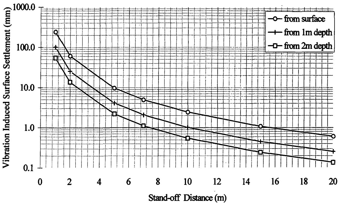
Figure 5.11.9b. As Figure 5.11.9a, semi-log plot.
