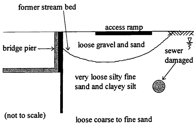
Figure 6.30. Cross-section of bridge cofferdam (Case E).
