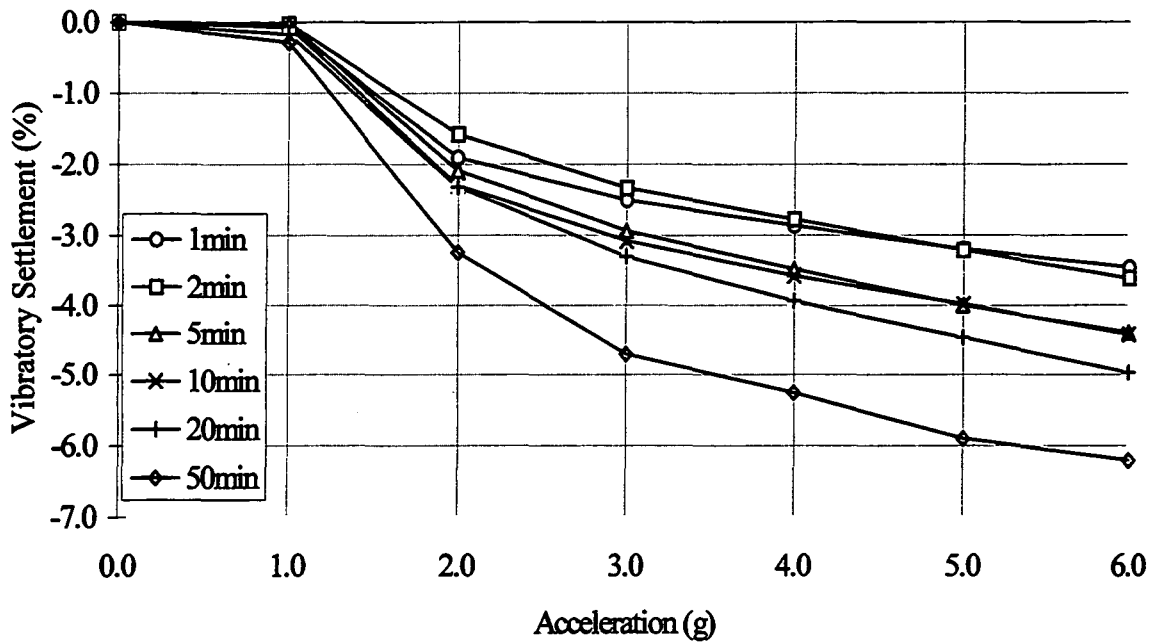
Figure 5.5.3. Coarse Leighton Buzzard sand settlement response to tests of fixed time length per acceleration increment (saturated, 50kPa, 25Hz) (see Appendix A3.6.6, for test data sheet).
