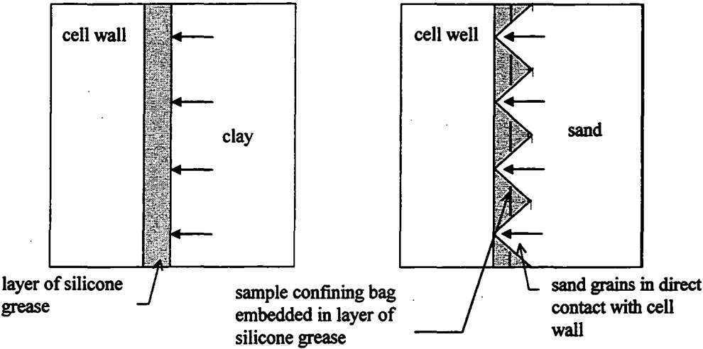
Figure 6.2. Comparison of the wall friction of fine grained soils and tests that use coarse grained soil.
