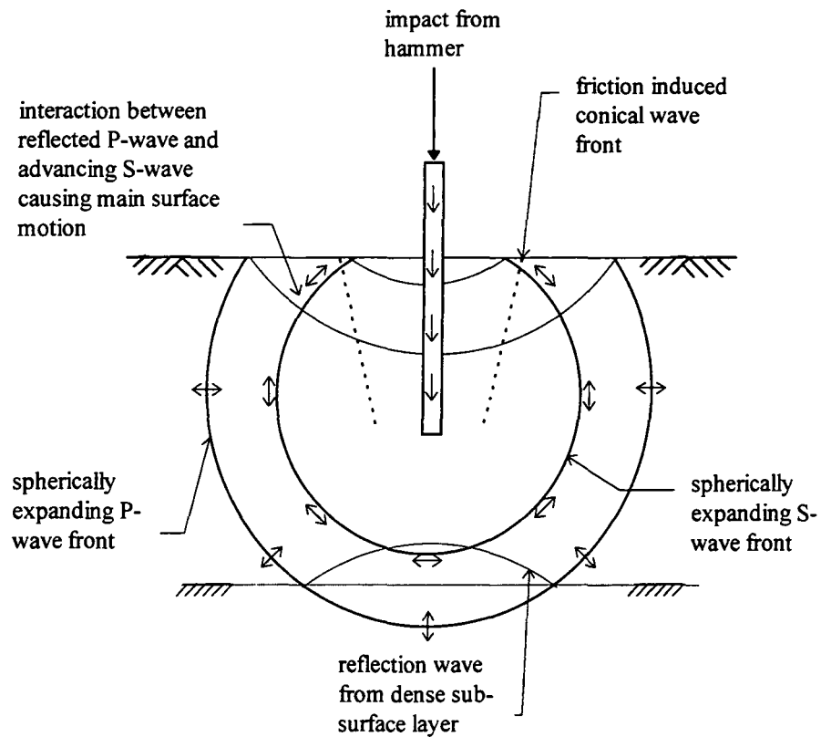
Figure 2.5 Propagation of ground vibrations from a pile driving operation (after Attewell and Farmer, 1973).
