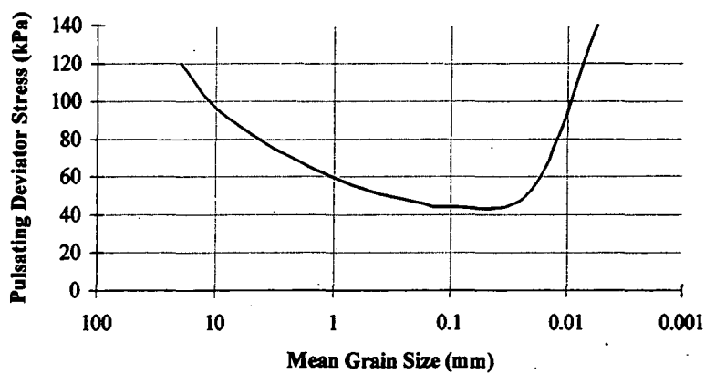
Figure 3.11. Comparison of (0.1Hz) pulsating loading strengths of soils with different grain size after 30 cycles ( D_r = 50\% , for 20% strain and \sigma_c = 105\text{kPa} , after Lee and Fitton, 1969).
