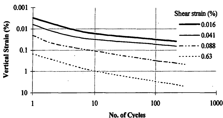
Figure 3.13a. The influence of shear strain amplitude on vertical strain, using D_r = 60\% , and \sigma_v = 24\text{kPa} (after Silver and Seed, 1971b).
