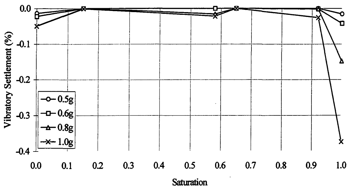
Figure 5.2.4. Influence of degree of saturation on medium uniform sand vibration test settlement results (25Hz, 10kPa) (see Appendix A3.4.3, for test data sheet).
