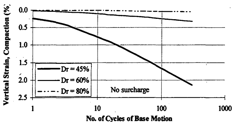
Figure 3.14. The effect of relative density on settlement of a sand layer, using acceleration of 0.3g (after Seed and Silver, 1972).
