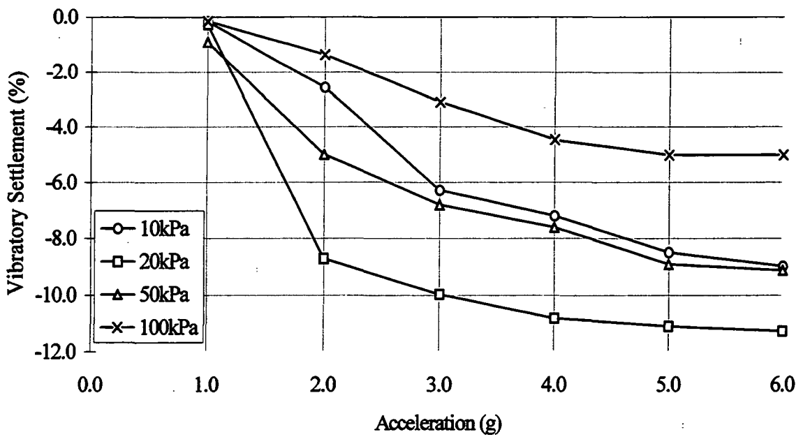
Figure 5.3.7. Medium sharp sand, high acceleration vibration test settlement results. Saturated, at 25Hz (see Appendix 3: Table A3.7.5, for test data sheet).
