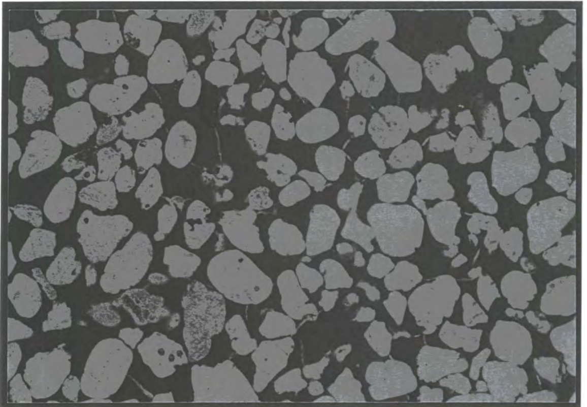
Plate 4.9. Thin-section of medium uniform sand (x 25 magnification).
