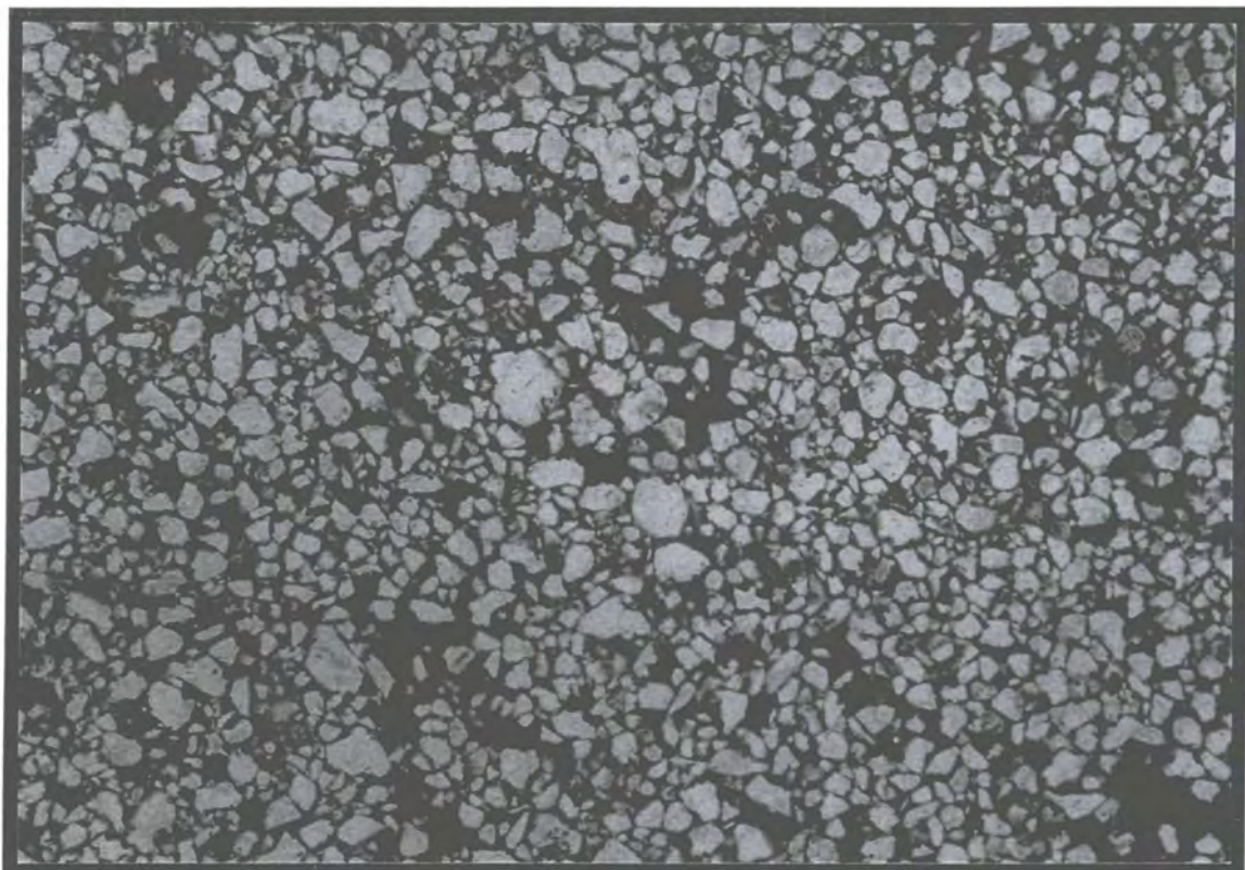
Plate 4.6. Thin-section of silty fine sand (x 25 magnification).
