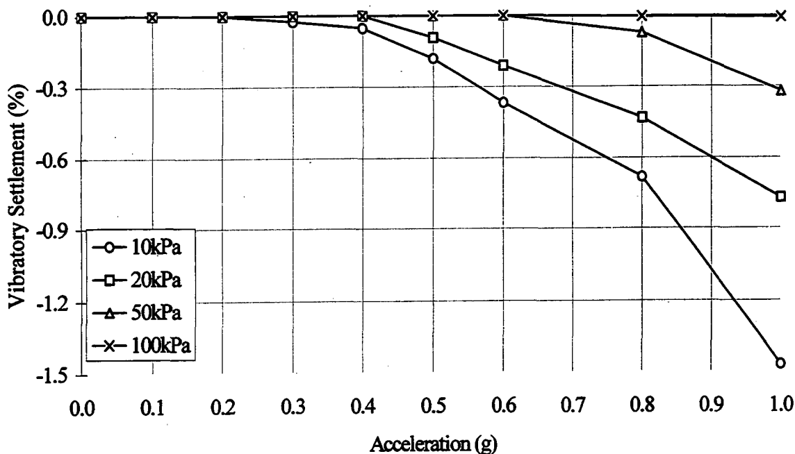
Figure 5.1.8a. Sandy fine gravel vibration test settlement results. Saturated, at 25Hz (see Appendix 3: Table A3.10.1, for test data sheet).
