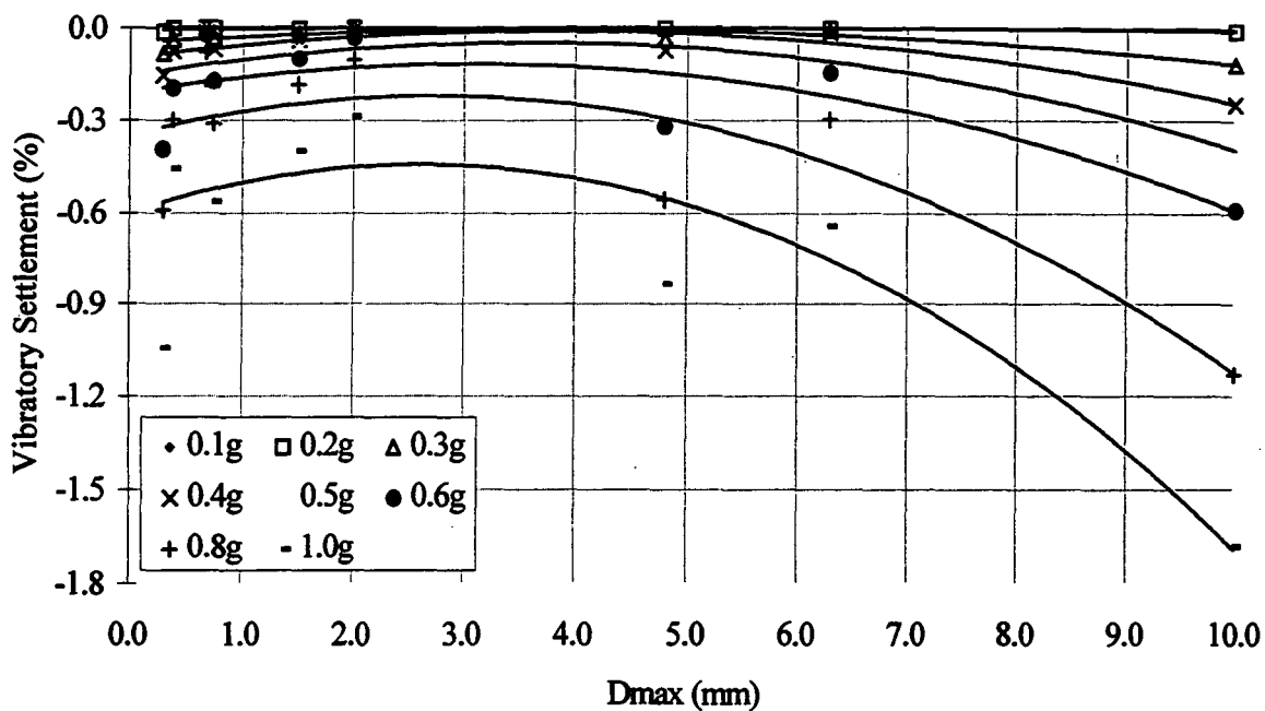
Figure 5.7.1a. Relationship between maximum particle size ( D_{max} ) and settlement (mean stress values, saturated, 25Hz).
