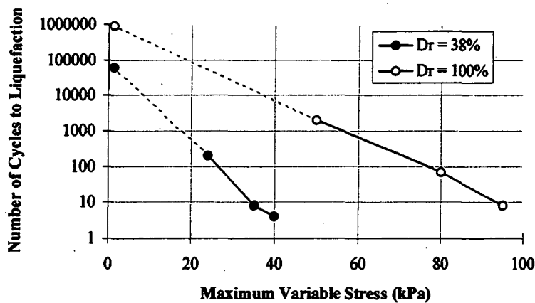
Figure 3.10. Number of cycles to initial liquefaction of a fine river sand, for a range of variable stress with a confining pressure of 100kPa (after Lee and Seed, 1967).
