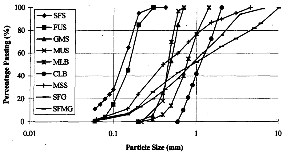
Figure 4.9. Particle size distribution of the soils (see Table 4.2).
