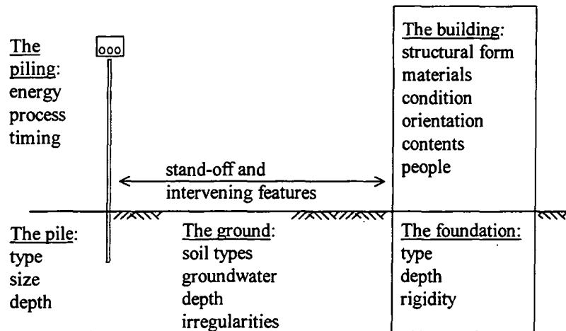
Figure 2.1 Summary of the variables associated with ground-borne vibration and piling (from the CIRIA Technical Note 142, 1992).
