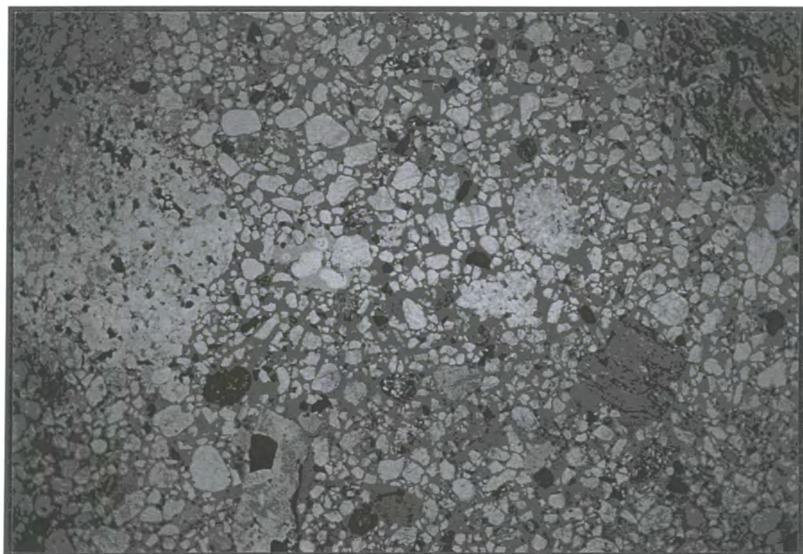
Plate 4.13. Thin-section of coarse sharp sand (x 25 magnification).
