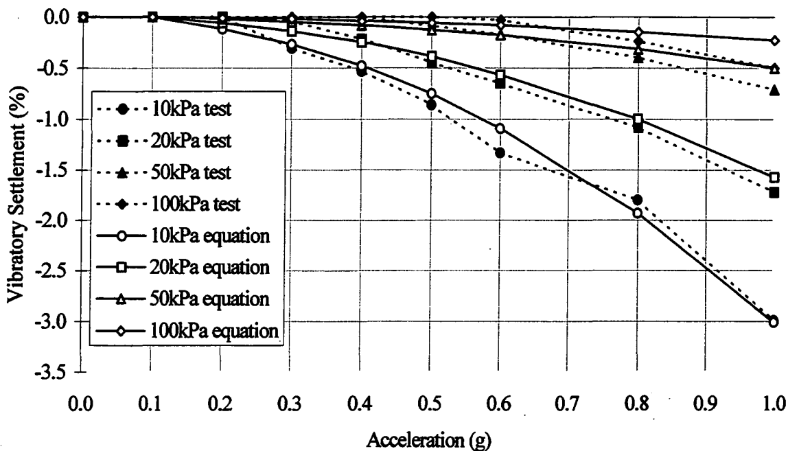
Figure 5.9.1d. Comparison between vibration test settlement and derived equivalent values (sandy fine to medium gravel, saturated, 40Hz).
