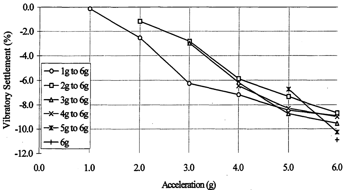
Figure 5.5.4. Medium sharp sand settlement response to increase in initial acceleration magnitude (saturated, 10kPa, 25Hz) (see Appendix 3: Table A3.7.6, for test data sheet).
