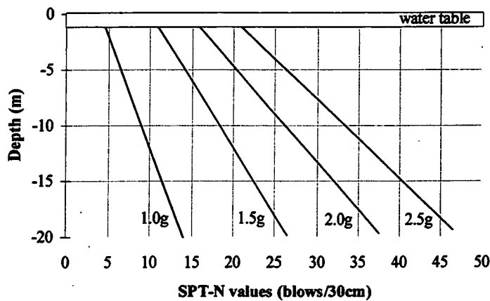
Figure 3.29. Values of SPT-N for which liquefaction is not likely to occur under any given earthquake condition (after Seed and Idriss, 1971).
