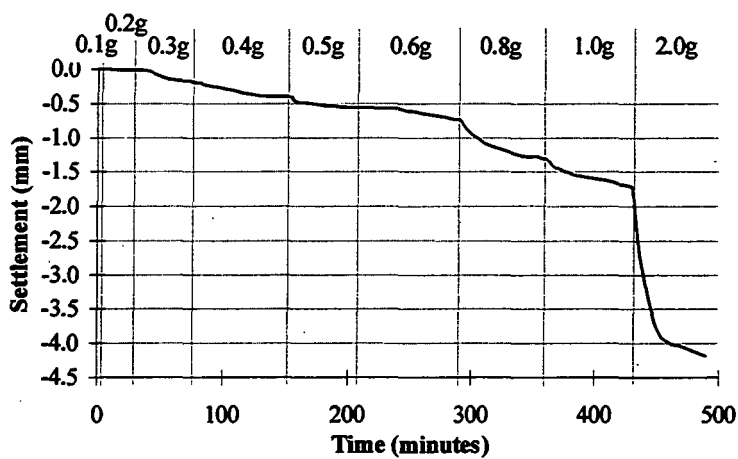
Figure 4.13 Typical form of a vibratory test result.
