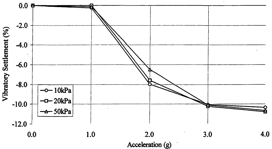
Figure 5.3.8. Coarse sharp sand >63\mu , high acceleration vibration test settlement results. Saturated, at 25Hz (see Appendix 3: Table A3.8.1, for test data sheet).
