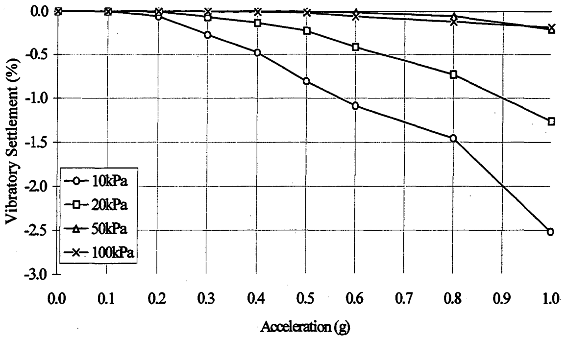
Figure 5.1.2a. Fine uniform sand vibration test settlement results. Saturated, at 25Hz (see Appendix 3: Table A3.2.1, for test data sheet).
