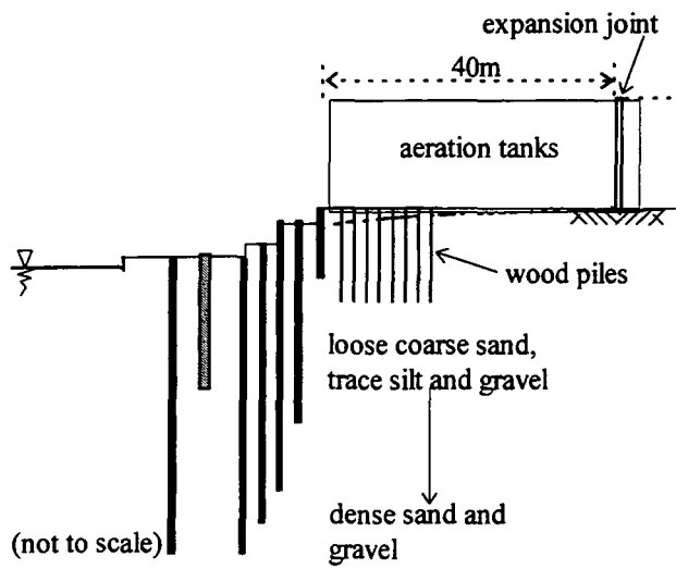
Figure 6.27. Cross-section of treatment plant expansion (Case B).
