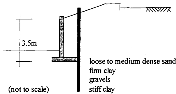
Figure 6.17. Cross-section of temporary works (Example #1).
