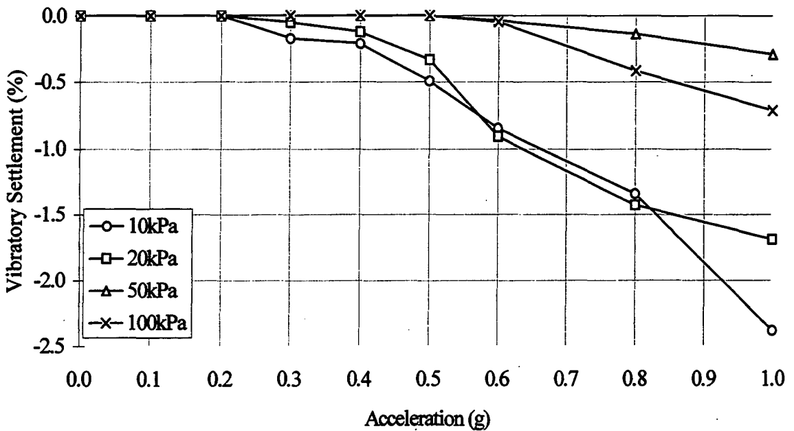
Figure 5.1.2b. Fine uniform sand vibration test settlement results. Saturated, at 40Hz (see Appendix 3: Table A3.2.2, for test data sheet).
