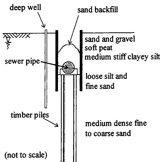
Figure 6.31. Cross-section of sewer repair (Case F).
