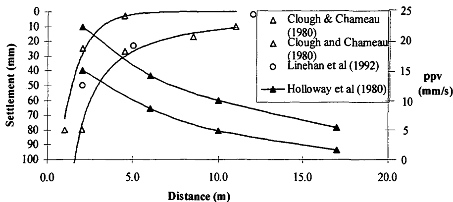
Figure 3.24. Comparison of settlement and particle velocities produced by pile driving (from Dowding, 1994) (closed symbols are peak particle velocity data).
