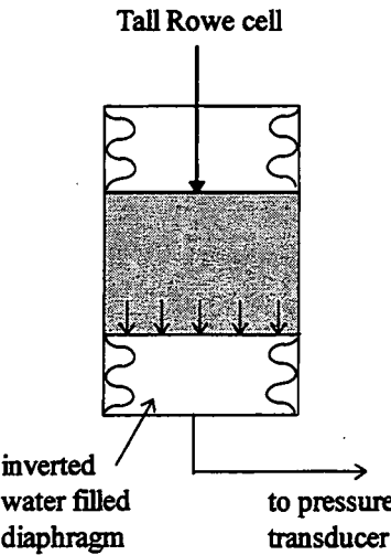
Figure 6.1. Testing the pressure applied to the base of the cell.
