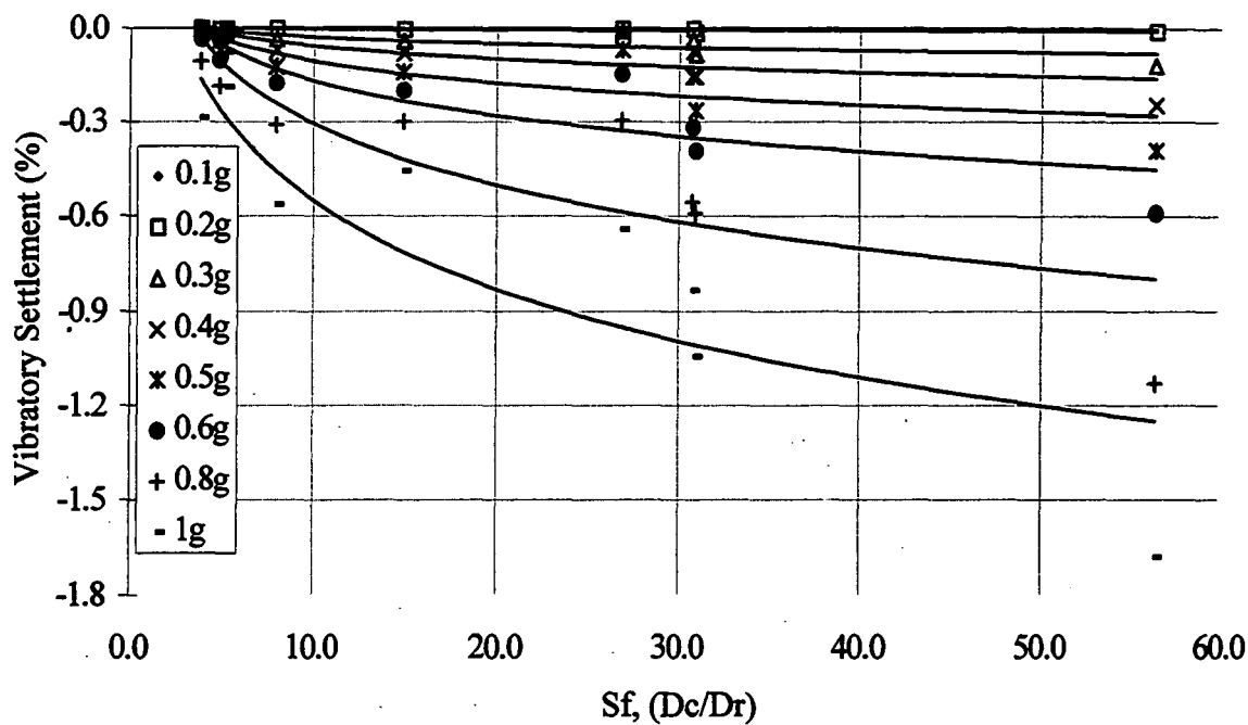
Figure 5.7.5a. Relationship between soil parameter ( S_f ) and settlement (mean stress values, saturated, 25Hz).
