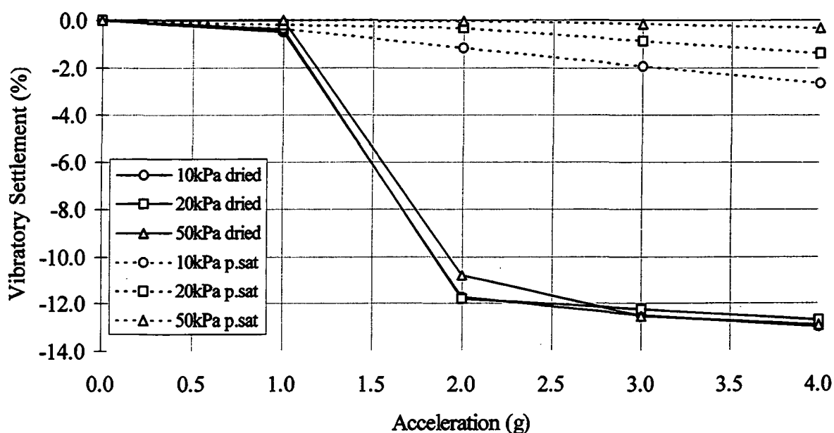
Figure 5.4.6. Coarse sharp sand >63μ partially saturated and dried high acceleration vibration test settlement results at 25Hz (see Appendix 3: Table A3.8.2; A3.8.3, for test data sheet).
