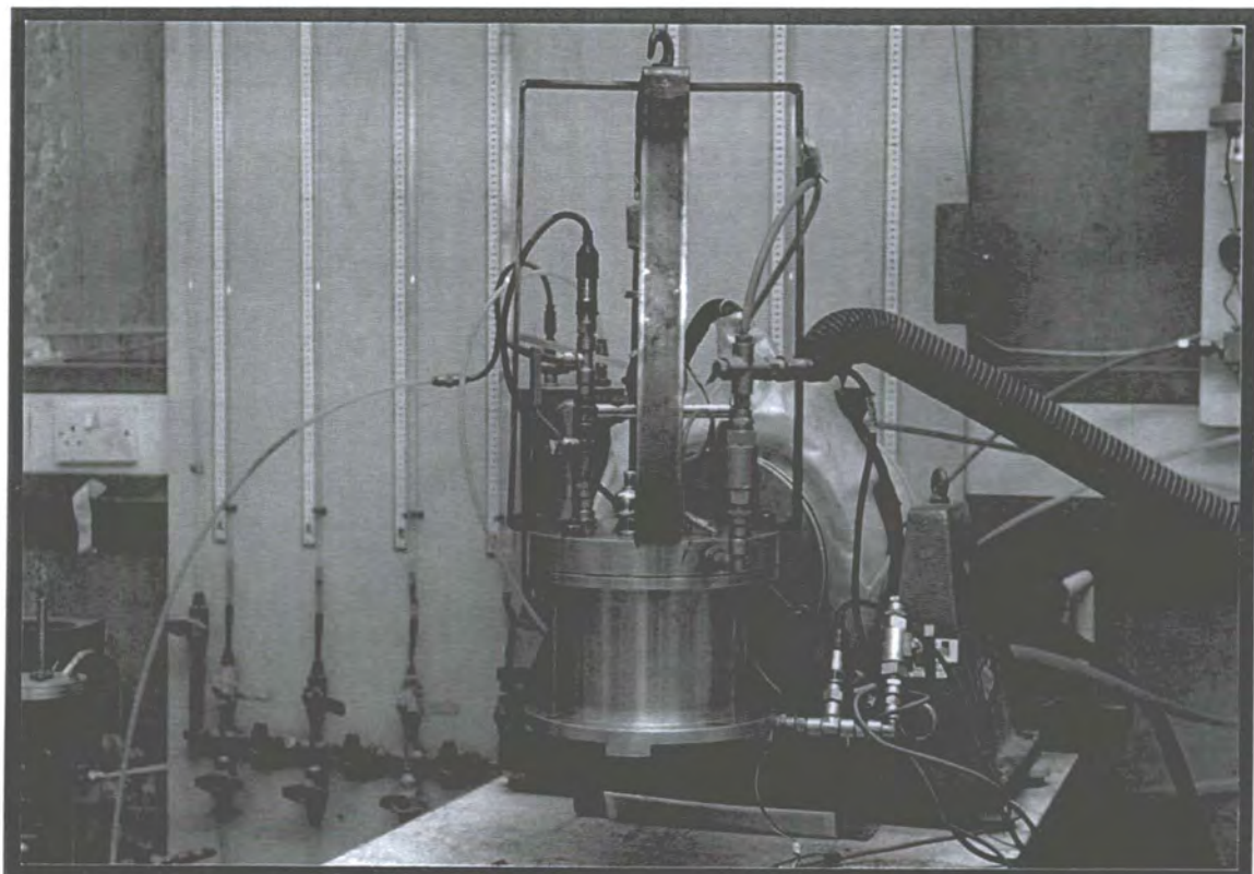
Plate 4.4. Rowe cell and shaker configured for horizontal vibration.
