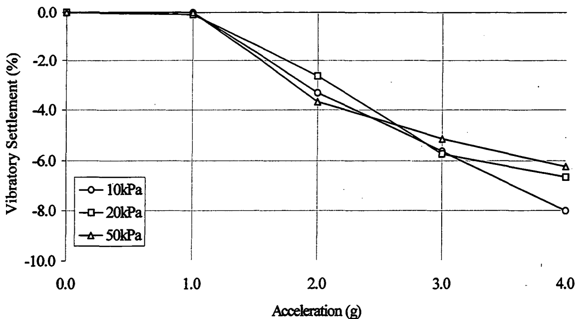
Figure 5.3.9. Coarse sharp sand , high acceleration vibration test settlement results. Saturated, at 25Hz (see Appendix 3; Table A3.9.1, for test data sheet).
