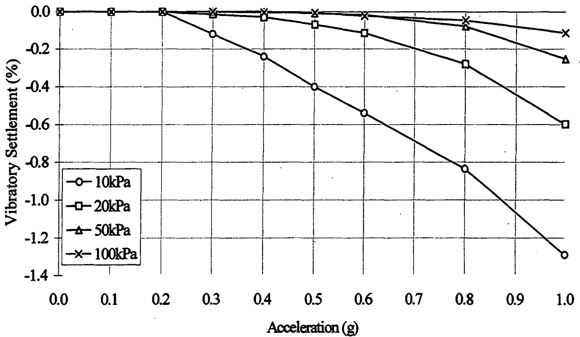
Figure 5.1.3a. Garside medium sand vibration test settlement results. Saturated, at 25Hz (see Appendix 3: Table A3.3.1, for test data sheet).
