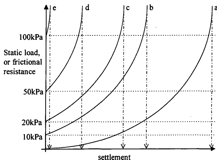
Figure 6.10. Illustrating the influence of static load and frictional resistance on the settlement potential of a soil (for a given density and acceleration).
