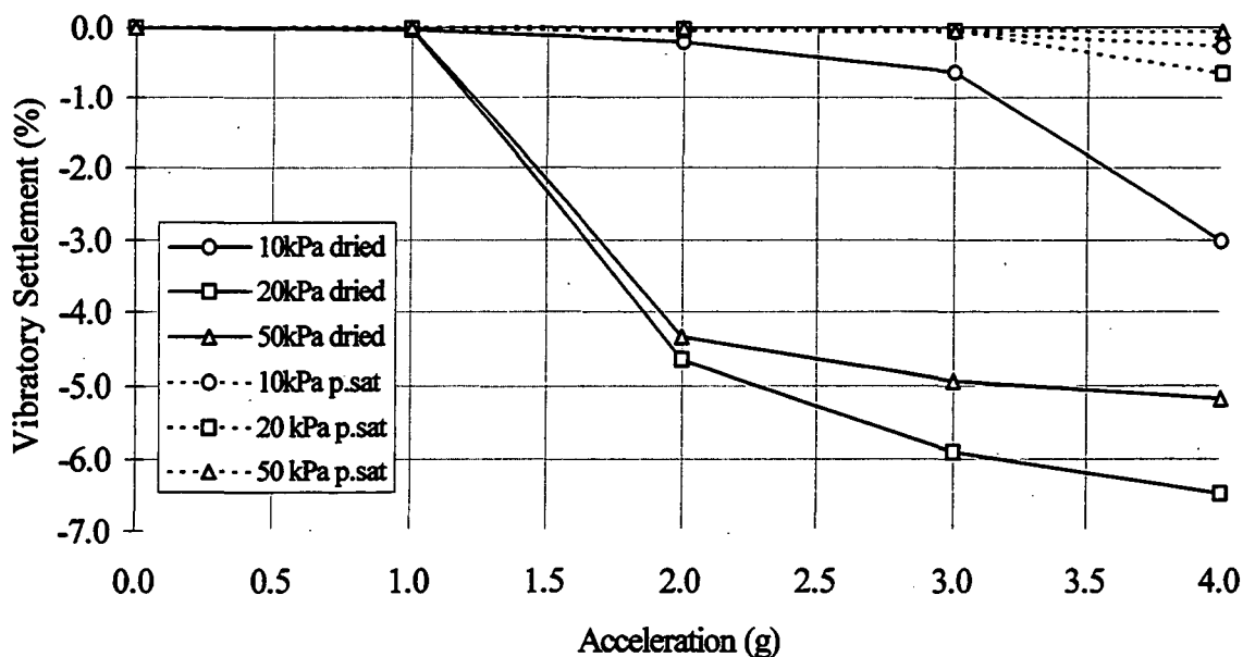
Figure 5.4.3. Medium uniform sand partially saturated and dried high acceleration vibration test settlement results at 25Hz (see Appendix 3: Table A3.4.6; A3.4.7, for test data sheet).
