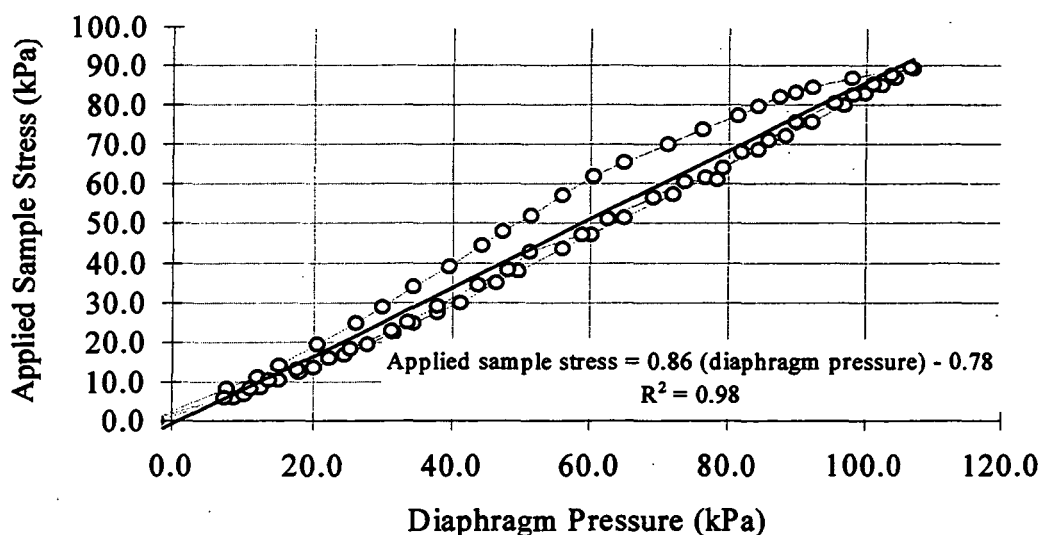
Figure A2.1.2. Diaphragm calibration graph (see Table A2.1.1b).
