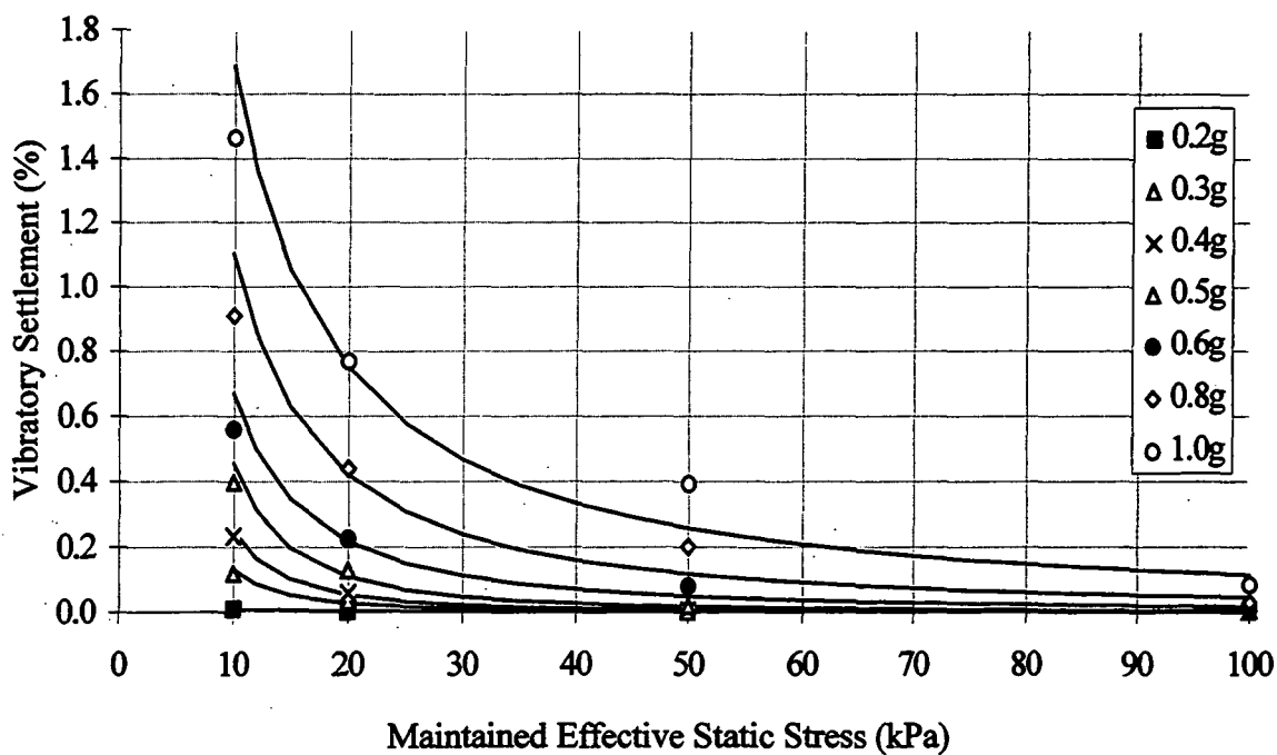
Figure 5.7.6a. General relationship between maintained effective static stress and settlement (protosoil values, saturated, 25Hz).
