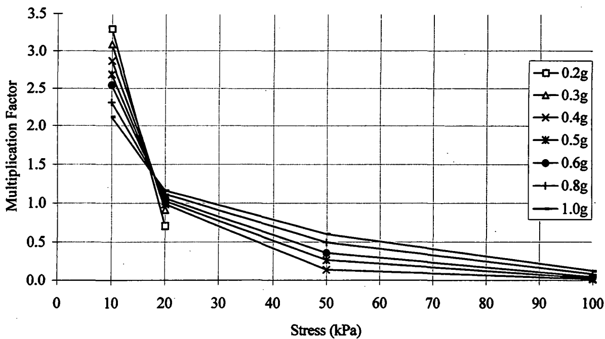
Figure 5.7.7a. Stress correction multiplication factor (using protosoil values, saturated, 25Hz).
