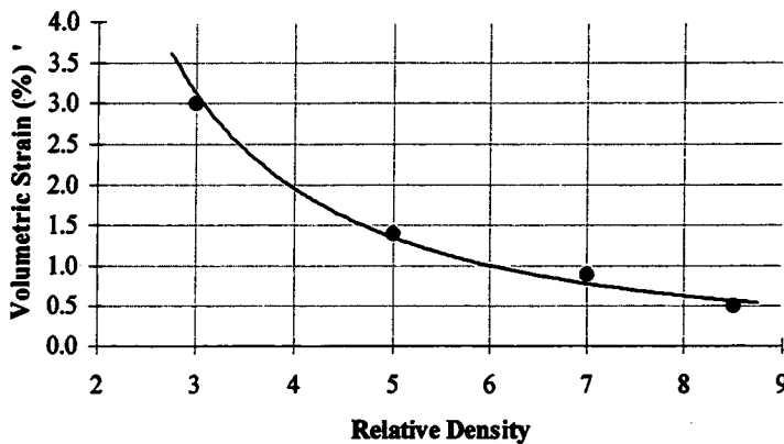
Figure 3.28 The effect of initial relative density on volumetric strain post-liquefaction (after Lee and Albaisa, 1974). Using the mean data of 33 tests in the range 100–430 kPa, D_{50} = 0.6 mm.
