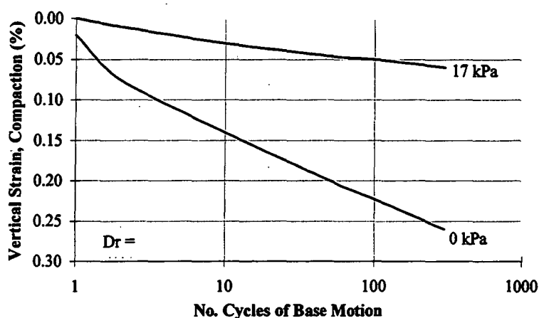
Figure 3.16. The effect of surcharge on vertical strain at 4Hz and 0.3g (after Seed and Silver, 1972).
