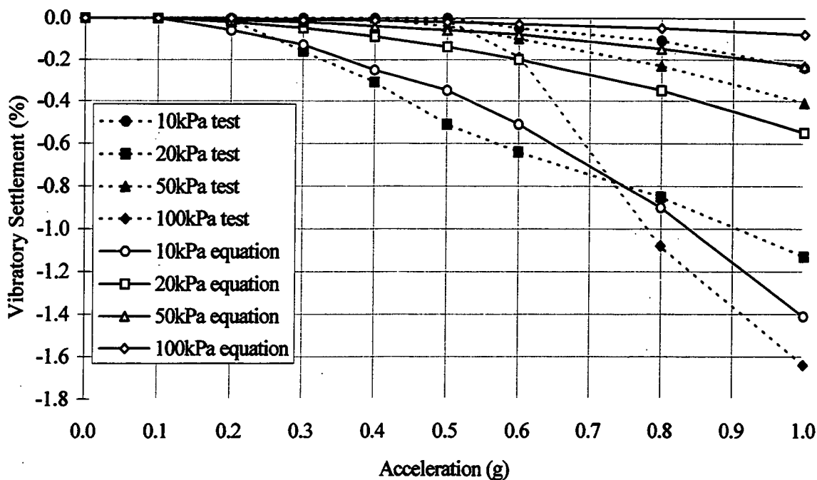
Figure 5.9.1a. Comparison between vibration test settlement and derived equivalent values (silty fine sand, saturated, 25Hz).
