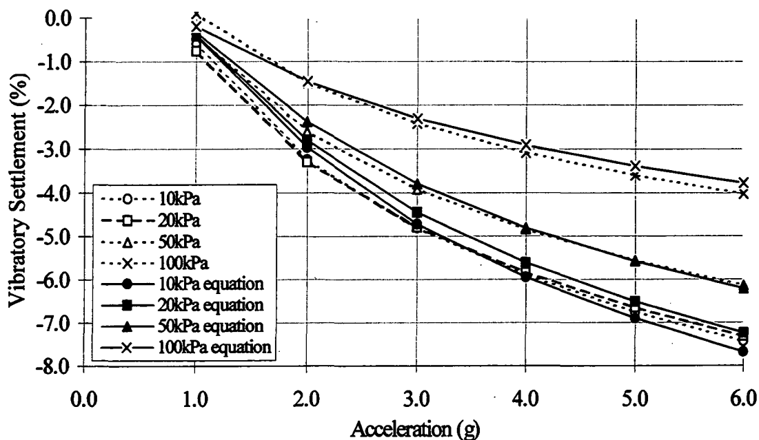
Figure 5.8.2. Comparison between high acceleration vibration test settlement and derived equivalent values (protosoil, saturated, 25Hz).
