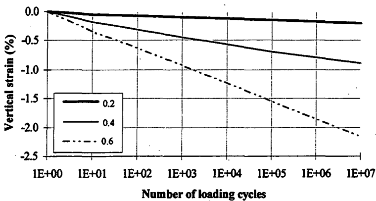
Figure 3.18. Compression of sands under controlled cyclic vertical stress.
