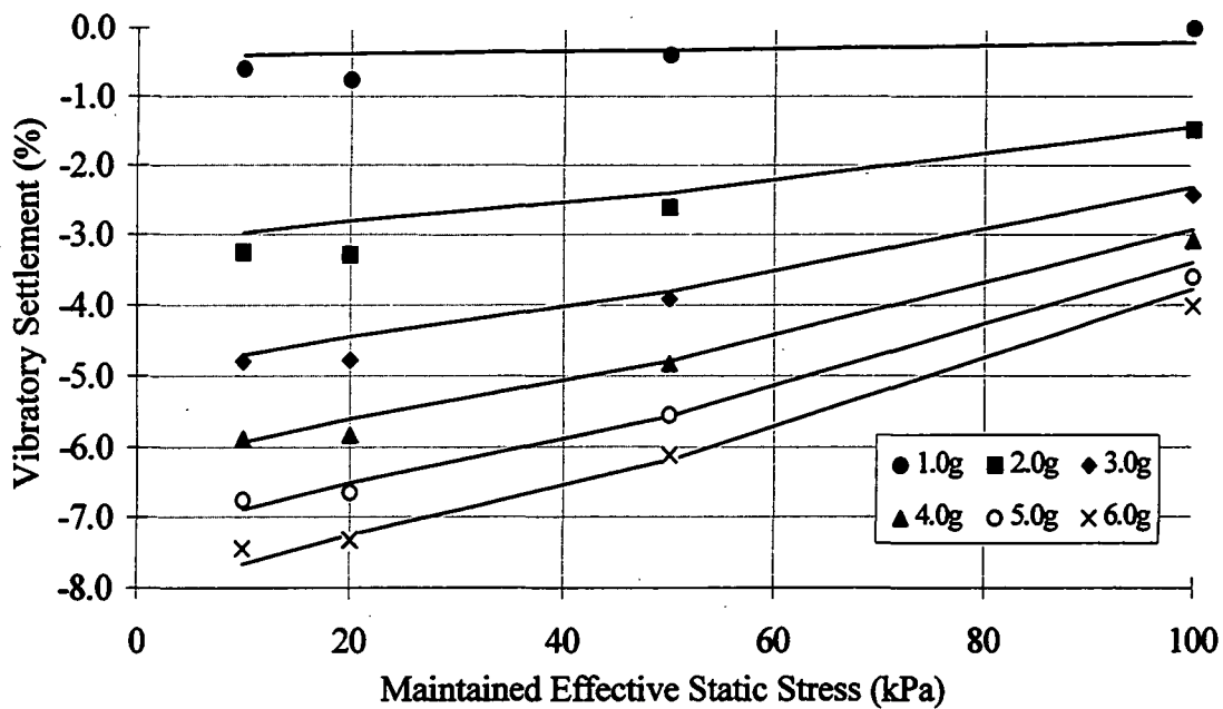
Figure 5.8.1. General relationship between static stress and high acceleration vibration settlement (protosoil values, saturated, 25Hz).
