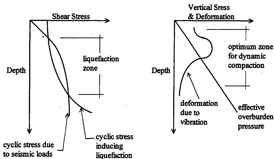
Figure 3.22. An analogy between liquefaction (after Seed and Idriss, 1971) and the optimum zone for dynamic compaction (after Oteo, 1983).
