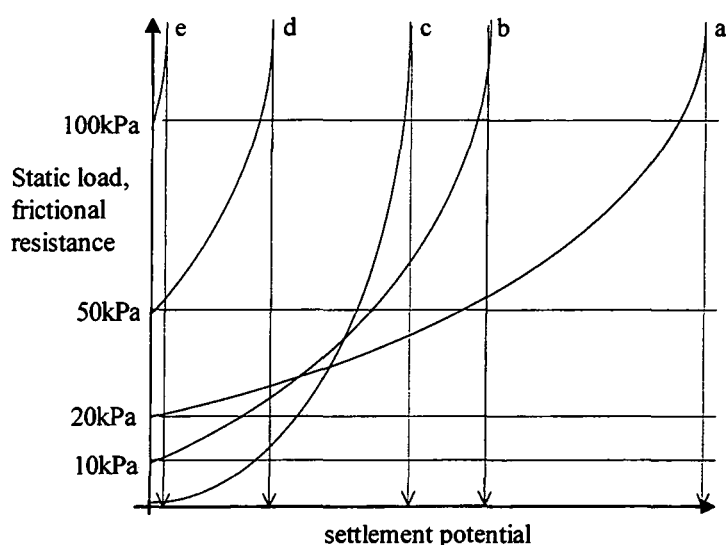
Figure 6.11. Modification of Figure 6.10, accounting for the optimum superposition of the influences of soil type, density, acceleration, frequency and static load.
