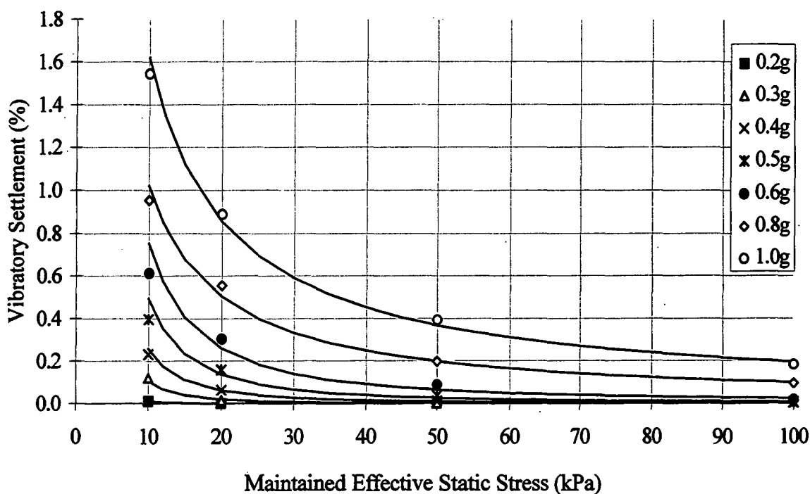
Figure 5.7.6b. General relationship between maintained effective static stress and settlement (protosoil values, saturated, 40Hz).
