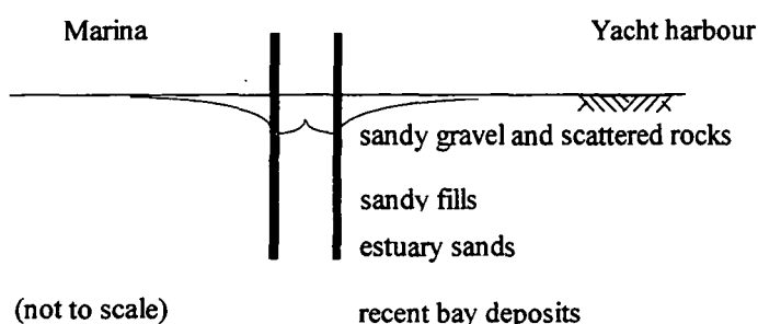
Figure 6.24. Cross-section of sewer culvert (Paper #4).
