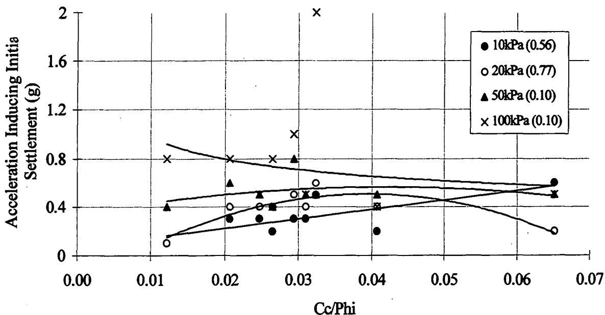
Figure 5.6.5. Best relationship between soil-type and minimum acceleration required to induce initial settlement (saturated, 25Hz). Data in brackets are best R^2 values.
