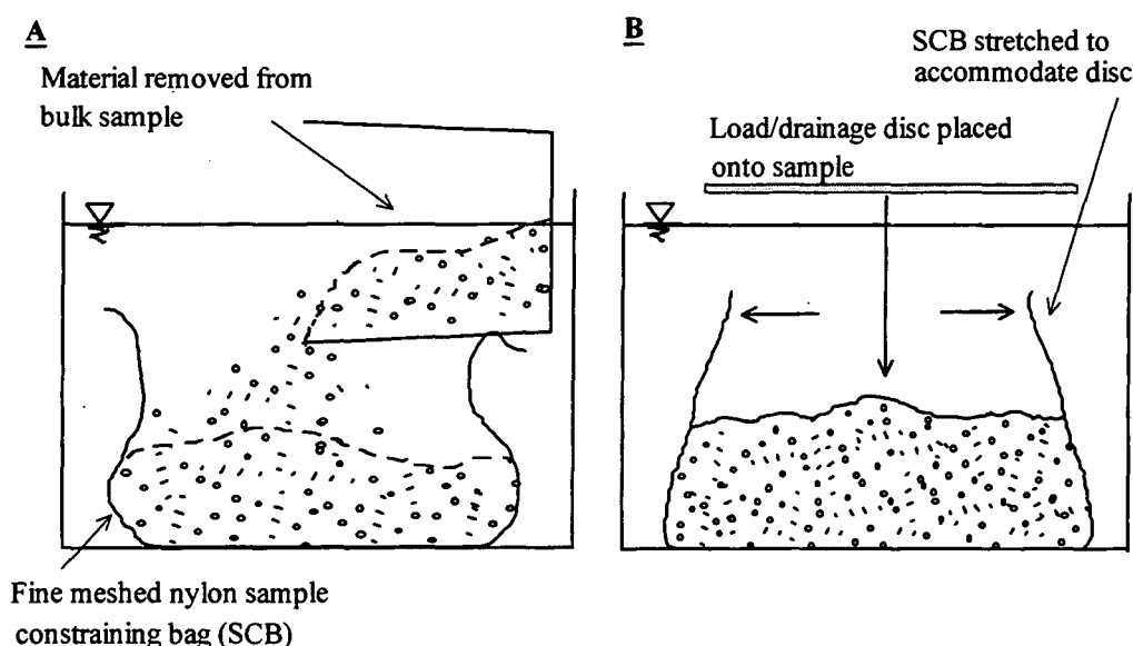
Figure 4.10. (A)The test-sample being placed into the sample confining bag (SCB), and (B) placing the load/drainage disc.
