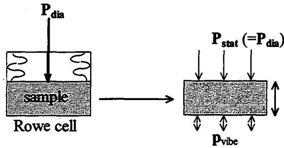
Figure 4.4. Variation in sample stress due to vibration.
