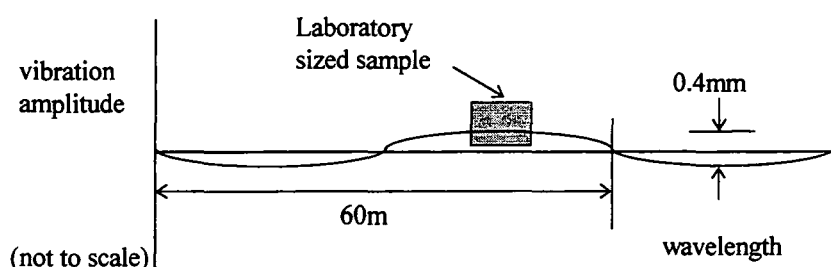
Figure 4.3. In-situ amplitude and wavelength ( 25\text{Hz} and 1g ).
