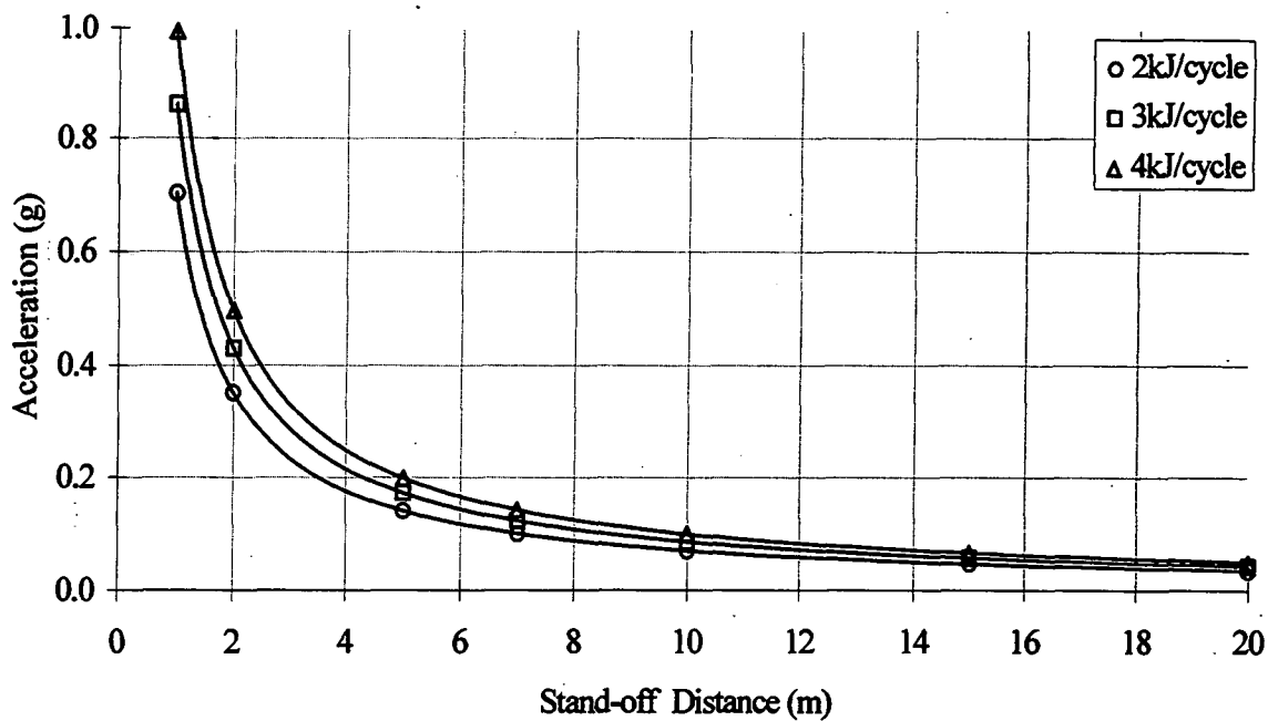
Figure 5.10.1. Attenuation of ground vibration with stand-off distance, using Equation 5.13.
