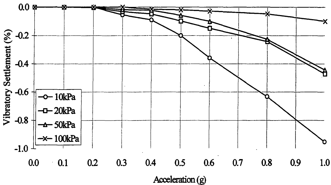
Figure 5.1.5b. Medium Leighton Buzzard sand vibration test settlement results. Saturated, at 40Hz (see Appendix 3: Table A3.5.2, for test data sheet).
