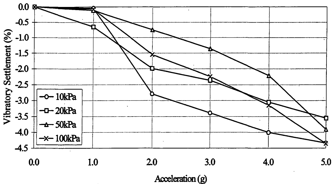
Figure 5.3.1. Silty fine sand, high acceleration vibration test settlement results. Saturated, at 25Hz (see Appendix 3: Table A3.1.3, for test data sheet).
