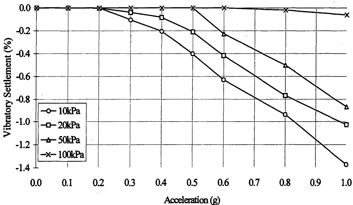
Figure 5.1.7a. Medium sharp sand vibration test settlement results. Saturated, at 25Hz (see Appendix 3: Table A3.7.1, for test data sheet).
