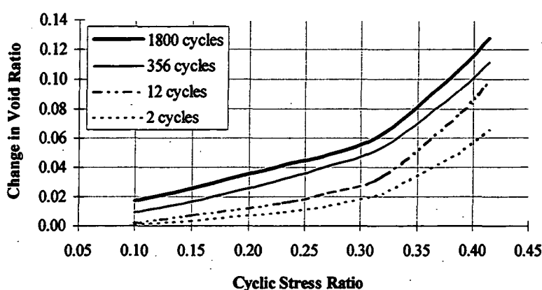
Figure 3.12 The relationship between applied stress ratio and the change in void ratio (after Tokue, 1979).
