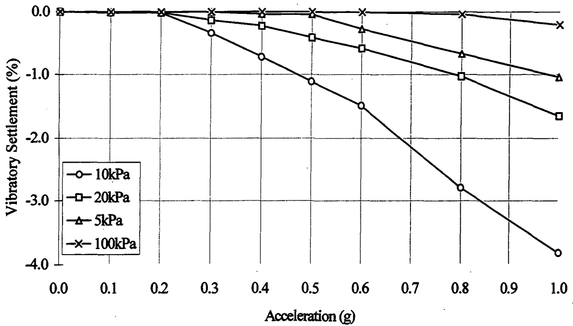
Figure 5.1.9a. Sandy fine to medium gravel vibration test settlement results.
