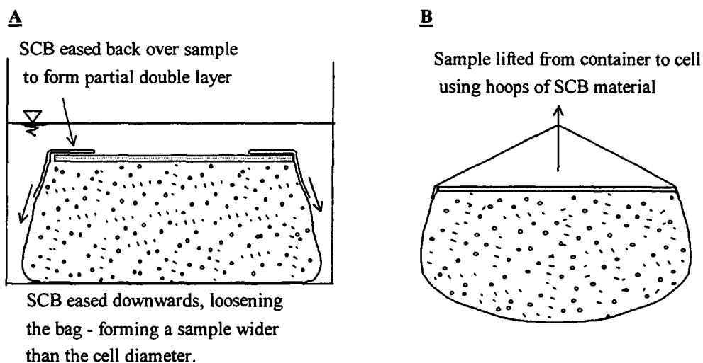
Figure 4.11. (A) Positioning the SCB onto the disc, and (B) removing to the Rowe cell.
