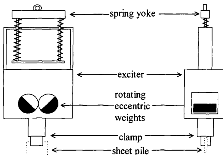
Figure 2.6. The basic components of a vibrodriver.
