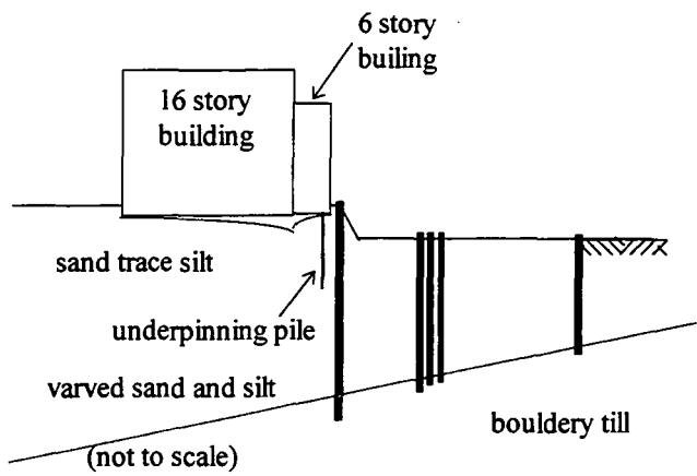
Figure 6.26. Cross-section of settlement of structure (Case A).
