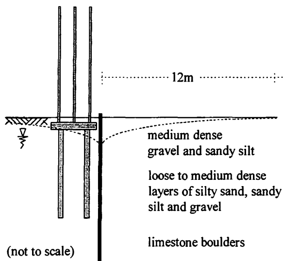
Figure 6.21. Cross-section of H-piles adjacent to existing structure (Paper #1).
