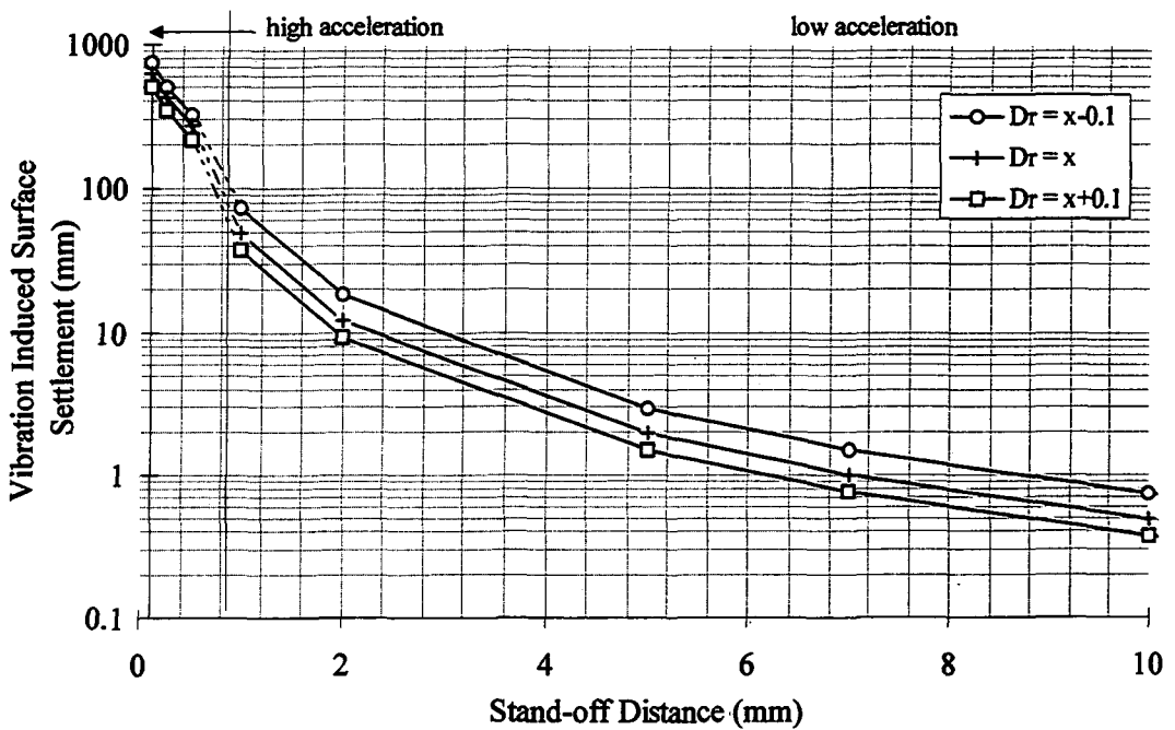
Figure 5.11.10a. Demonstrating the settlement generated using the high acceleration equation (ground condition 1.1) (see Appendix 4: Table 4.1.1, for test data sheet).
