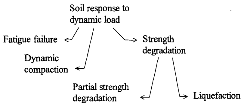
Figure 3.7. Typical soil response to dynamic loading (after Voznesensky, 1994).
