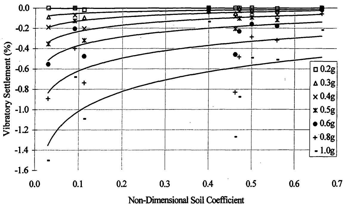
Figure 5.7.3b. Relationship between the non-dimensional coefficient ( D_x ) and settlement (mean stress values, saturated, 40Hz).
