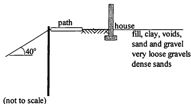
Figure 6.19. Cross-section of sheet pile works (Example #3).
