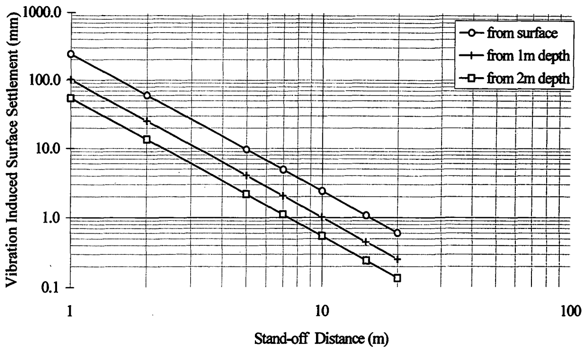
Figure 5.11.9a. Effect of depth below which settlement is calculated (ground condition 5, vibrodriver 1) (see Appendix 4: Table 4.1.8, for test data sheet).
