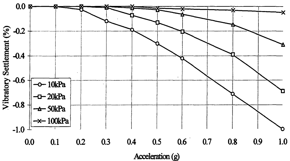
Figure 5.1.3b. Garside medium sand vibration test settlement results. Saturated, at 40Hz (see Appendix 3: Table 3.3.2, for test data sheet).
