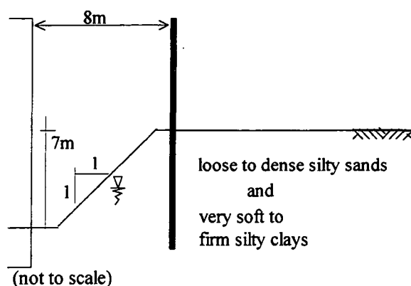
Figure 6.13. Cross-section of a retaining wall, Durham (Case Study 1).
