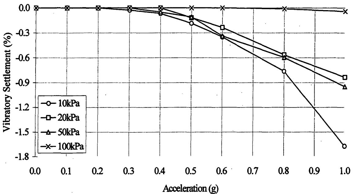
Figure 5.1.1b. Silty fine sand vibration test settlement results. Saturated, at 40Hz (see Appendix 3: Table A3.1.2, for test data sheet).
