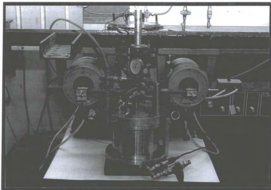
Plate 4.5. Rowe cell and shakers configured for torsional shear vibration.
