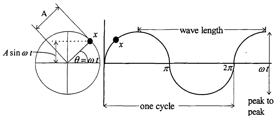
Figure 2.2. The character of sinusoidal vibration.
