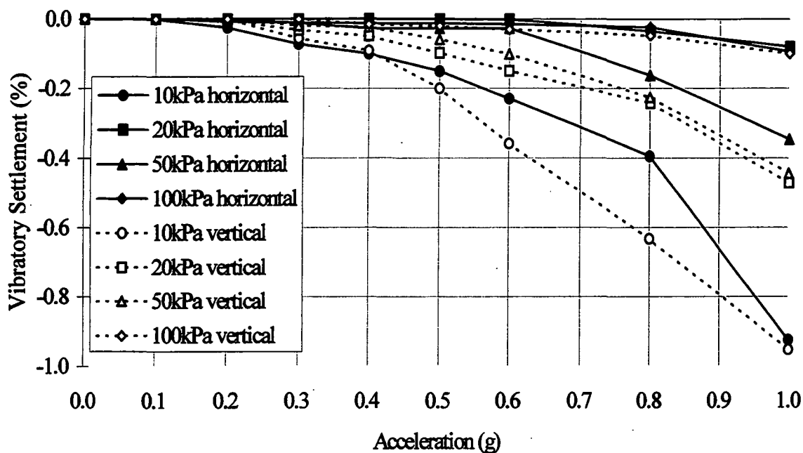
Figure 5.5.2a. Medium Leighton Buzzard sand, comparison of horizontal and vertical vibration orientation (40Hz, saturated) settlement tests (see Appendix 3: Table A3.5.2; A3.5.3, for test data sheet).
