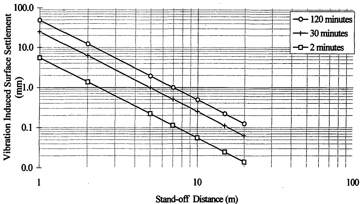
Figure 5.11.4a. Effect of varying vibration time on surface settlement (ground condition 1.1, vibrodriver 1) (see Appendix 4: Table 4.1.1, for test data sheet).
