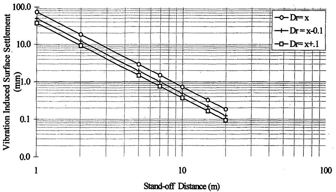
Figure 5.11.2a. Effect of varying relative density on surface settlement (ground condition 1.1, vibrodriver 1) (see Appendix 4: Table 4.1.1, for test data sheet).
