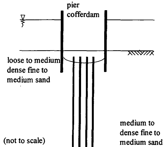
Figure 6.28. Cross-section of bridge pier (Case C).
