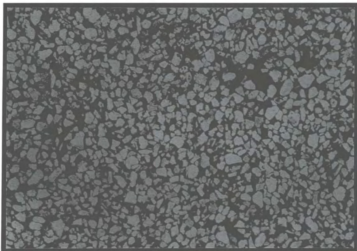
Plate 4.7. Thin-section of fine uniform sand (x 25 magnification).
