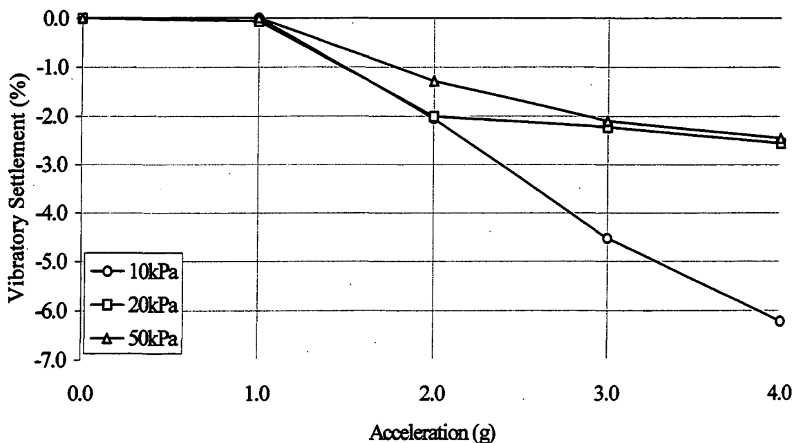
Figure 5.3.4. Medium uniform sand, high acceleration test settlement results. Saturated, at 25Hz (see Appendix 3: Table A3.4.5, for test data sheet).
