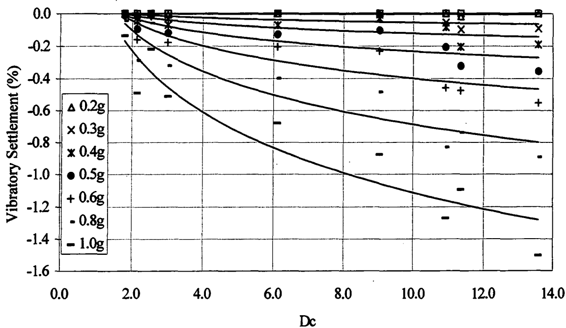
Figure 5.7.4b. Relationship between distribution coefficient ( D_c ) and settlement (mean stress values, saturated, 40Hz).
