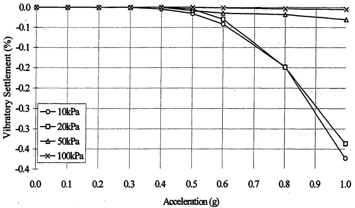
Figure 5.1.4a. Medium uniform sand vibration test settlement results. Saturated, at 25Hz (see Appendix 3: Table A3.4.1, for test data sheet).
