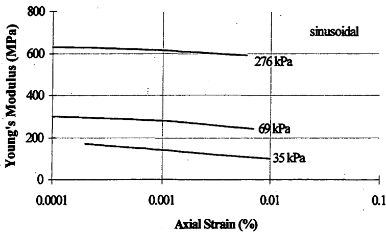
Figure 3.9 Effect of axial strain on Young's Modulus for three confining pressures (after Zhang and Aggour, 1995).
