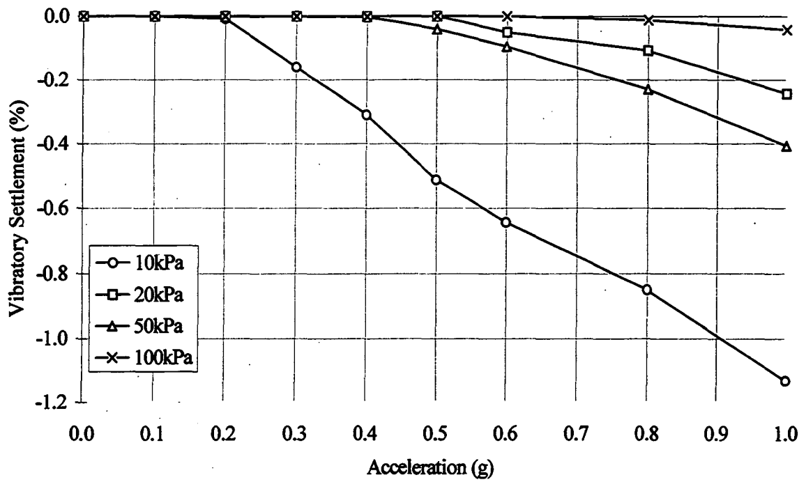
Figure 5.1.1a. Silty fine sand vibration test settlement results. Saturated, at 25Hz (see Appendix 3: Table A3.1.1, for test data sheet).
