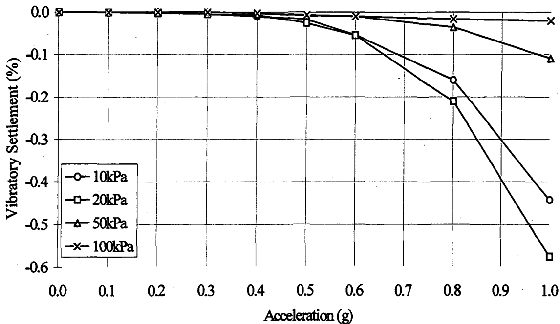
Figure 5.1.6a. Coarse Leighton Buzzard sand vibration test settlement results. Saturated, at 25Hz (see Appendix 3: Table A3.6.1, for test data sheet).
