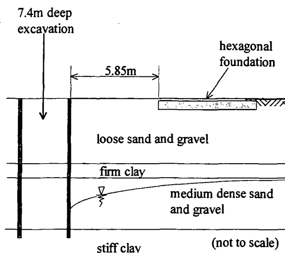
Figure 6.16. Cross-section of cofferdam (Case Study 5).
