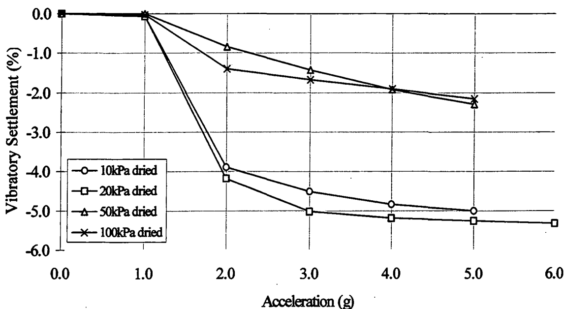
Figure 5.4.2. Garside medium sand dried high acceleration vibration test settlement results at 25Hz (see Appendix 3: Table A3.3.4, for test data sheet).
