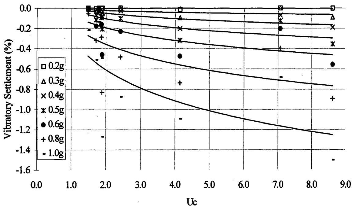
Figure 5.7.2b. Relationship between uniformity coefficient ( U_c ) and settlement (mean stress values, saturated, 40Hz).
