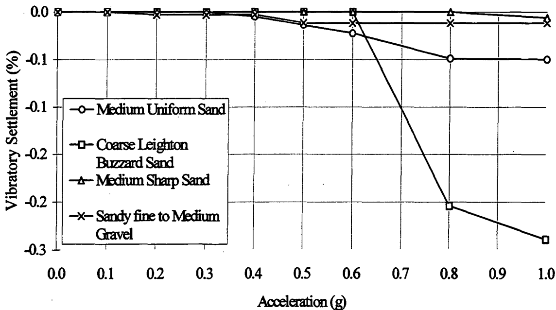
Figure 5.2.1. Dried vibration test settlement results, at 25Hz and 10kPa (see Appendix 3: Table A3.4.4; A3.6.3; A3.7.4; A3.11.5 for test data sheet).
