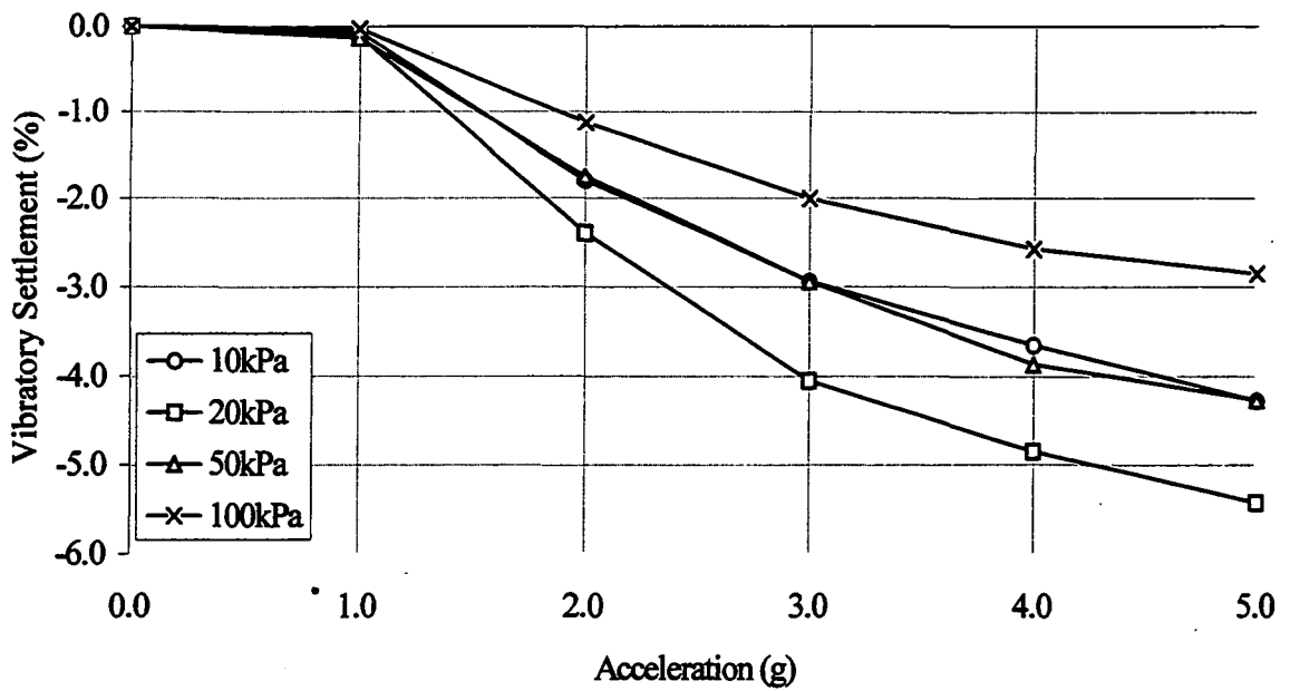
Figure 5.3.5. Medium Leighton Buzzard sand, high acceleration vibration test settlement results. Saturated, at 25Hz (see Appendix 3: Table A3.5.4, for test data sheet).
