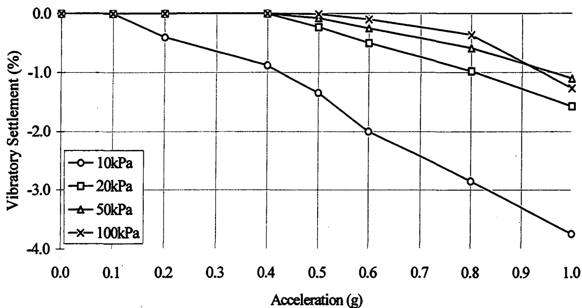
Figure 5.5.1. Sandy fine to medium gravel vibration test settlement results.
