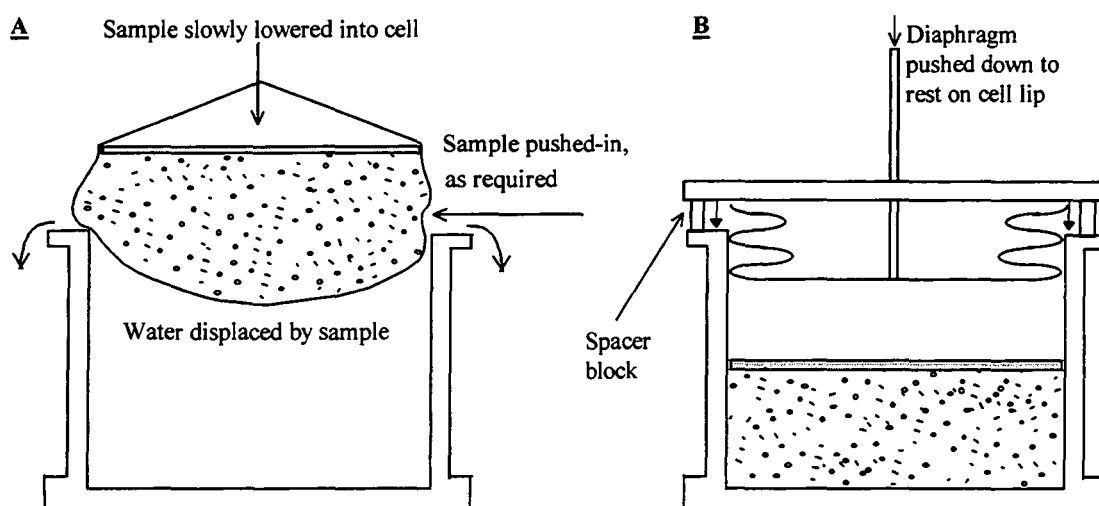
Figure 4.12. (A) Placement of the sample into the cell, and (B) lowering the diaphragm.
