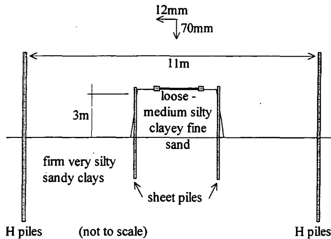
Figure 6.14. Cross-section of railway bridge construction (Case Study 3).
