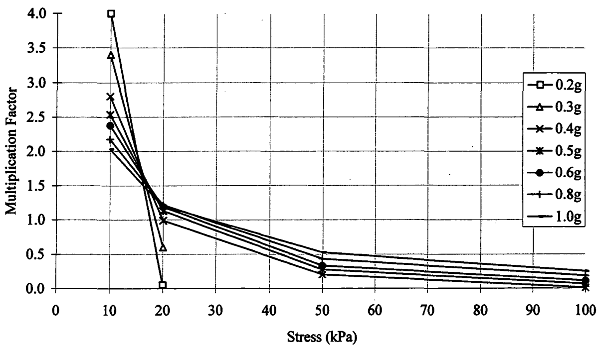
Figure 5.7.7b. Stress correction multiplication factor (using protosoil values, saturated, 40Hz).
