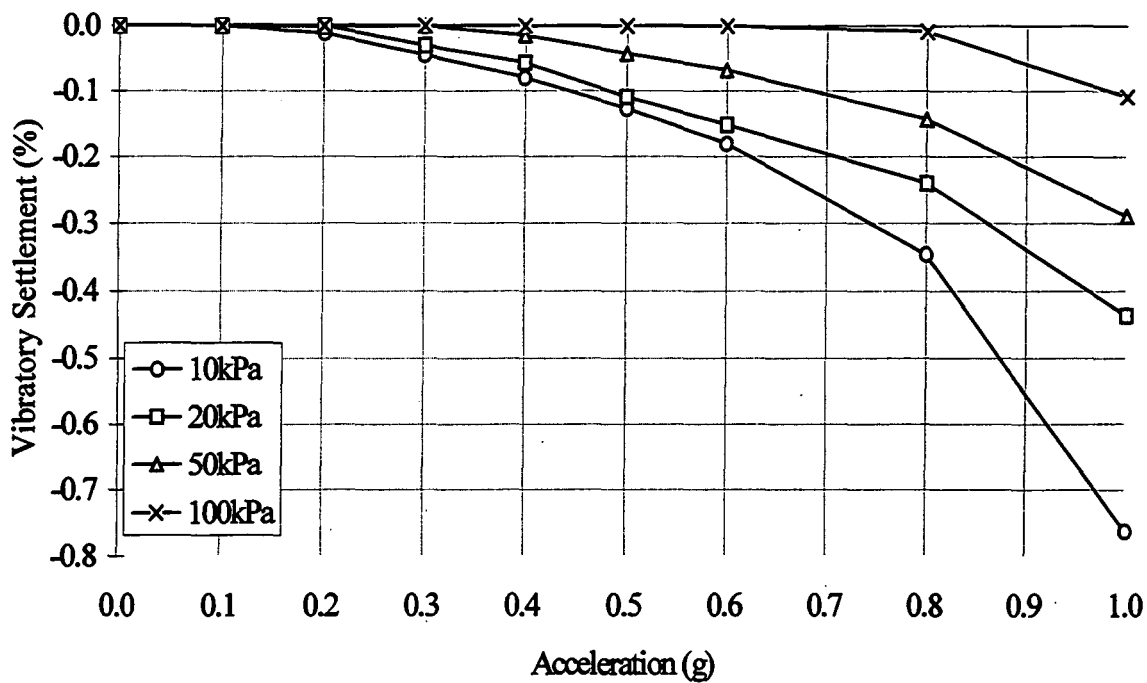
Figure 5.1.5a. Medium Leighton Buzzard sand vibration test settlement results. Saturated, at 25Hz (see Appendix 3: Table A3.5.1, for test data sheet).
