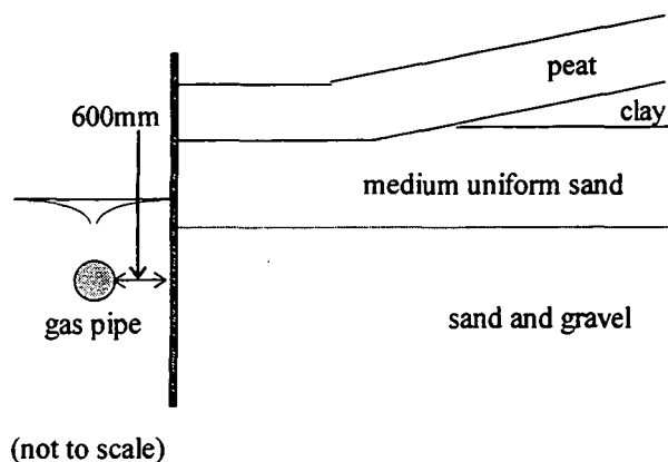
Figure 6.22. Cross-section of cofferdam construction (Paper #2).
