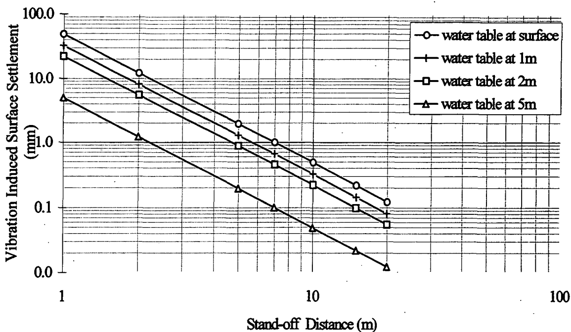
Figure 5.11.5a. Effect of varying water table position on surface settlement (ground condition 1.1, vibrodriver 1) (see Appendix 4: Table 4.1.1, for test data sheet).
