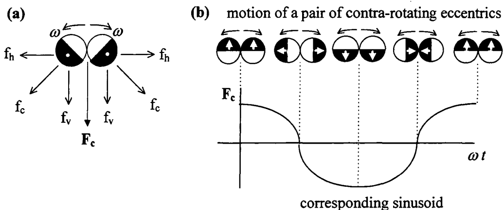
Figure 2.7. The principle of vibrodriver operation.
