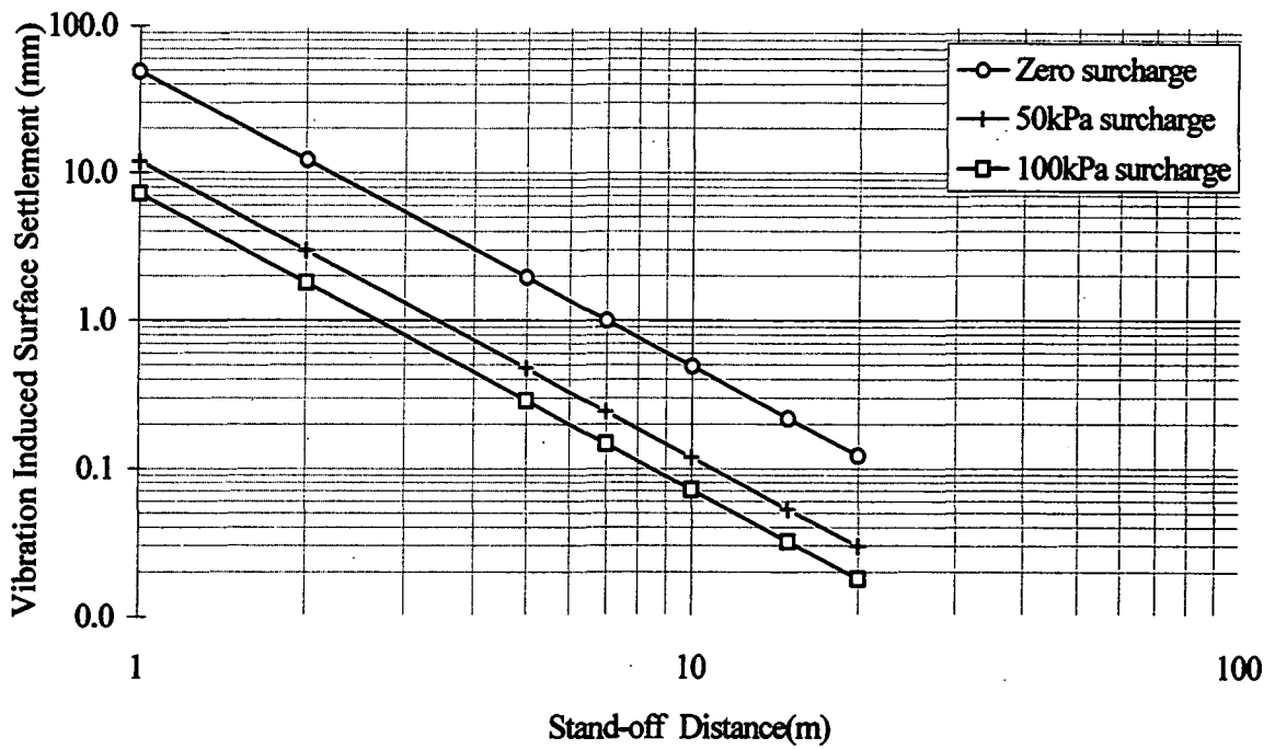
Figure 5.11.3a. Effect of varying surcharge on surface settlement (ground condition 1.1, vibrodriver 1) (see Appendix 4: Table 4.1.1, for test data sheet).
