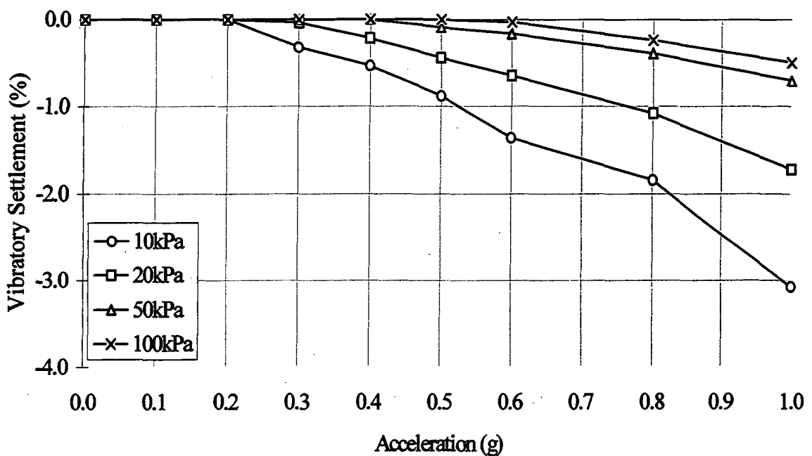
Figure 5.1.9b. Sandy fine to medium gravel vibration test settlement results.
