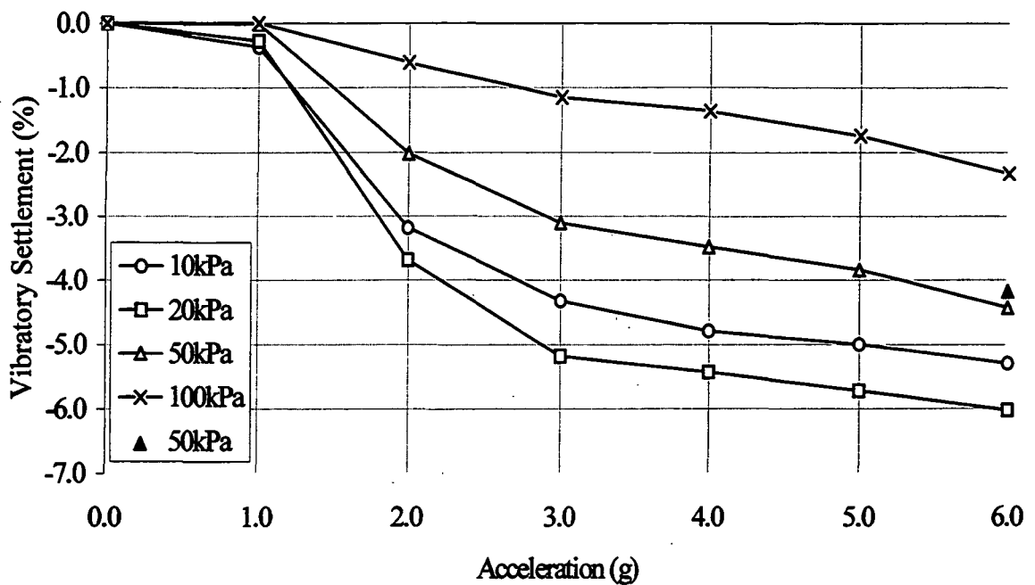
Figure 5.3.6. Coarse Leighton Buzzard sand, high acceleration vibration test settlement results. Saturated, at 25Hz (see Appendix 3: Table A3.6.5, for test data sheet).
