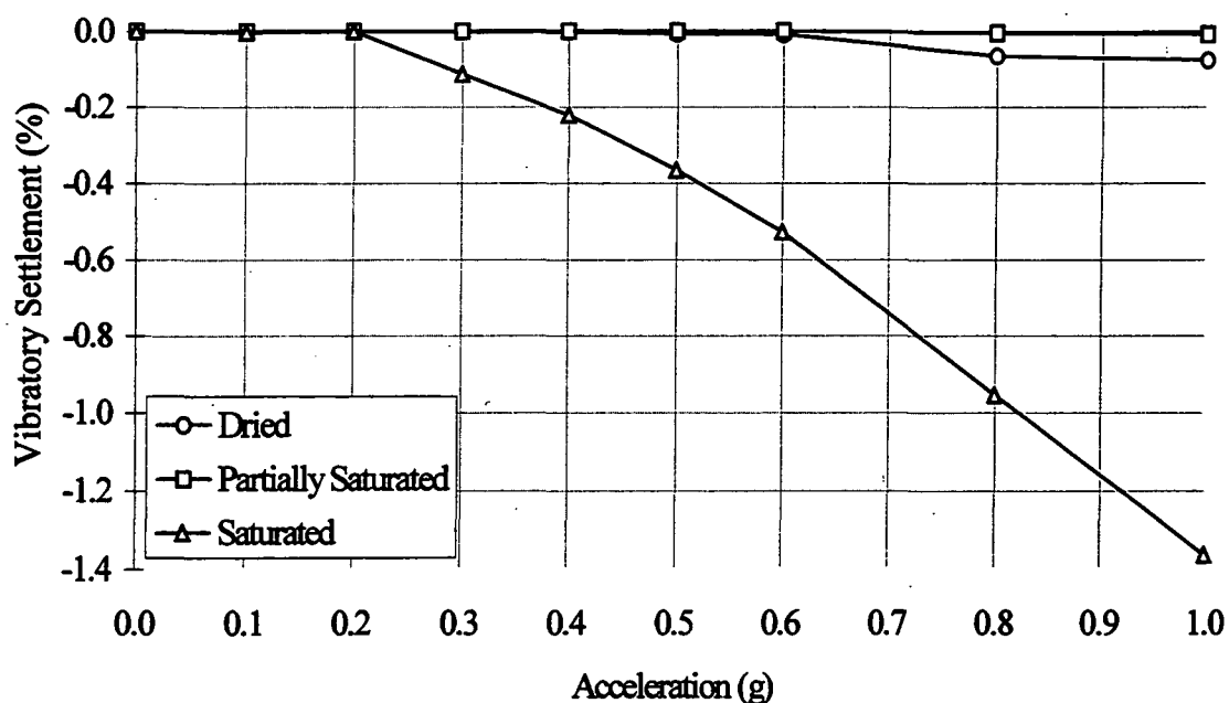
Figure 5.2.3. General comparison of saturated, partially saturated and dried vibration test results (using mean stress values, 25Hz, 10kPa) .
