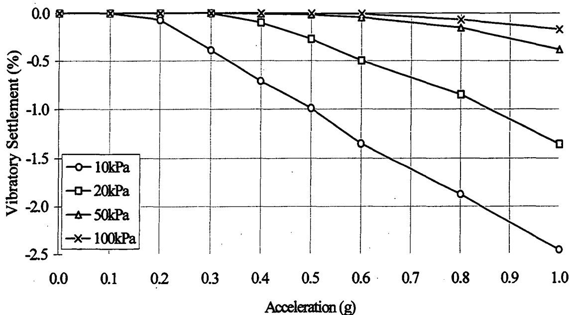
Figure 5.1.7b. Medium sharp sand vibration test settlement results. Saturated, at 40Hz (see Appendix 3: Table A3.7.2, for test data sheet).
