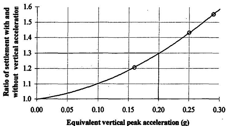
Figure 3.23. Effect of vertical motion superimposed on horizontal motion (after Pyke et al. , 1975) - a vertical acceleration of 0.2g modifies the settlement obtained by horizontal base acceleration by a factor of 1.3.
