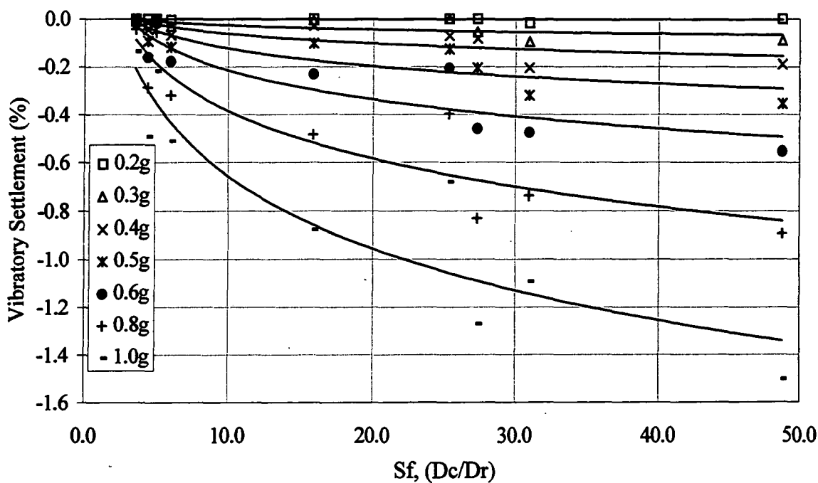
Figure 5.7.5b. Relationship between soil parameter ( S_f ) and settlement (mean stress values, saturated, 40Hz).
