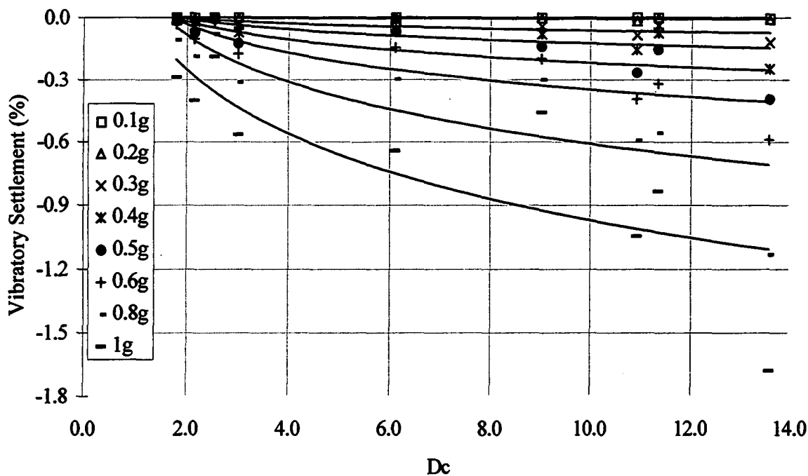
Figure 5.7.4a. Relationship between distribution coefficient ( D_c ) and settlement (mean stress values, saturated, 25Hz).
