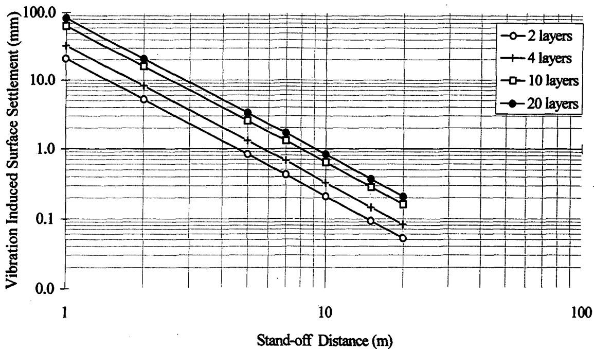
Figure 5.11.8a. Effect of layer resolution on surface settlement (ground condition 4.1, vibrodriver 1) (see Appendix 4: Tables 4.1.6, 4.1.7 for test data sheet).
