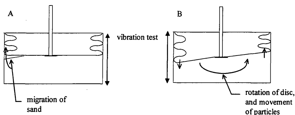
Figure 6.4. Illustrating the problem of sample migration and disc rotation.
