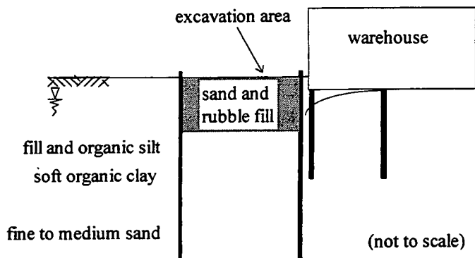
Figure 6.29. Cross-section of excavation adjacent to structure (Case D).
