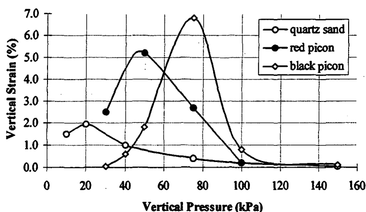
Figure 3.21. Vertical strain due to vibration under a range of maintained pressures (after Oteo, 1983).
