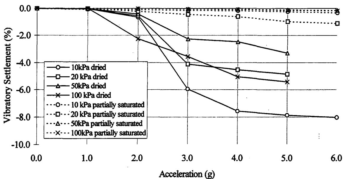
Figure 5.4.5. Medium sharp sand partially saturated and dried high acceleration vibration test settlement results at 25Hz (see Appendix 3: Table A3.7.7; A3.7.8, for test data sheet).
