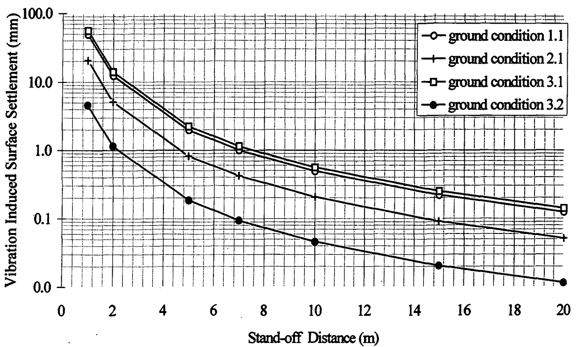
Figure 5.11.7b. As Figure 5.11.7a, semi-log plot.
