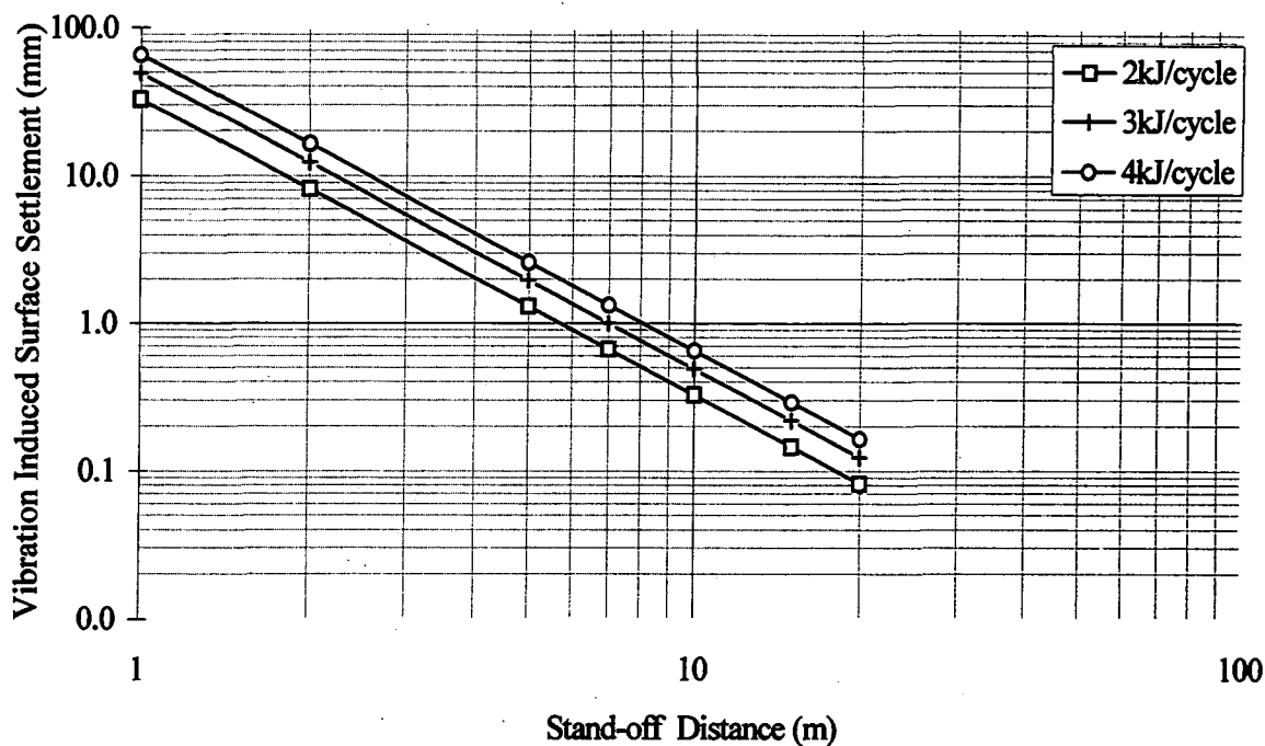
Figure 5.11.1a. Effect of vibrodriver (running at 25Hz) input energy on surface settlement (ground condition 1.1) (see Appendix 4: Table 4.1.1, for test data sheet).
