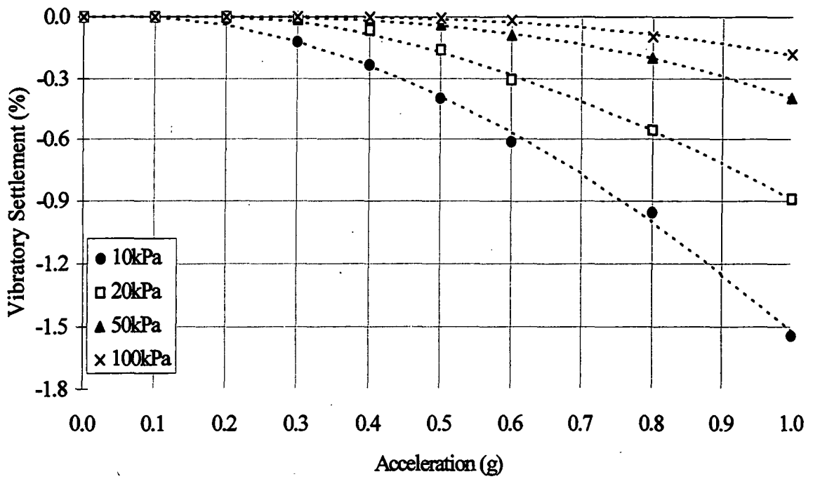
Figure 5.6.3a. Vibration settlement response of a protosoil to static stress (saturated, 40Hz).
