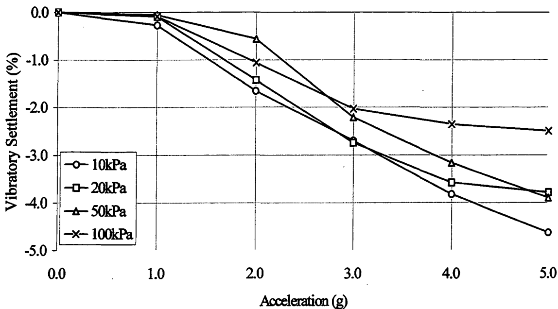
Figure 5.3.2. Fine uniform sand, high acceleration vibration test settlement results. Saturated, at 25Hz (see Appendix 3: Table A3.2.3, for test data sheet).
