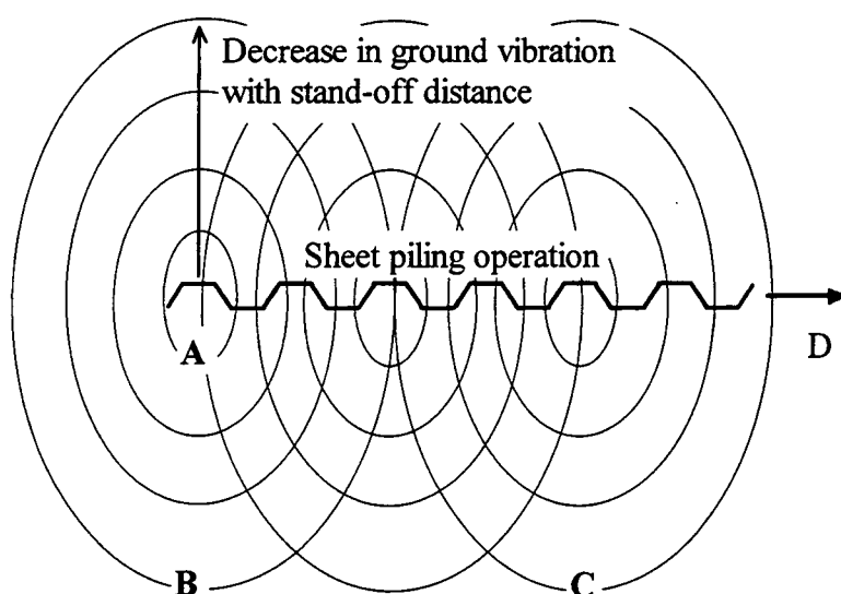
Figure 6.5. Ground vibration magnitudes experienced by various soil units.
