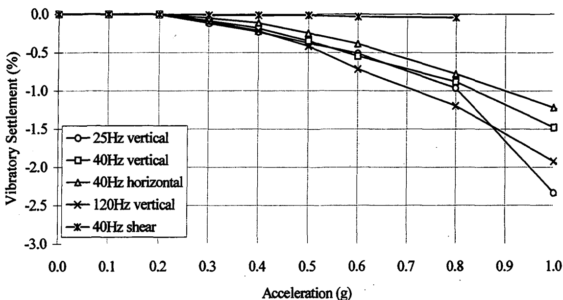
Figure 5.5.2c. Sandy fine to medium gravel settlement response to different vibration frequency and orientation (see Appendix 3: Table A3.11.7, for test data sheet).
