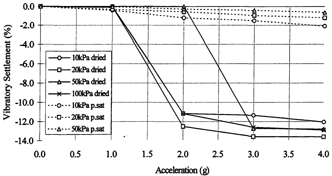
Figure 5.4.7. Coarse sharp sand partially saturated and dried high acceleration vibration test settlement results at 25Hz (see Appendix 3: Table A3.9.1; A3.9.2, for test data sheet).
