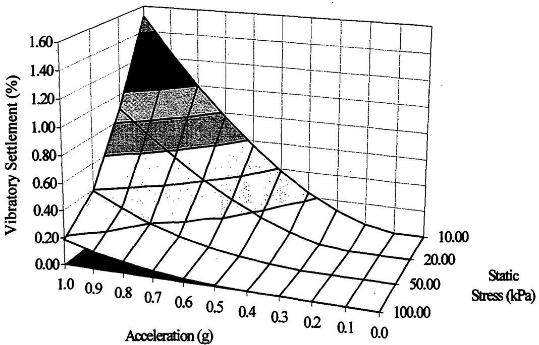
Figure 5.6.3b. Three-dimensional view of Figure 5.6.3a.
