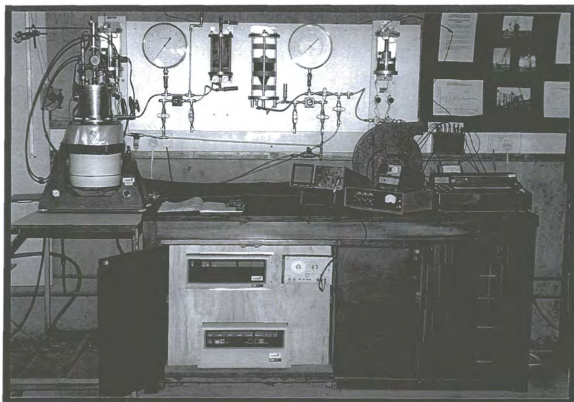
Plate 4.2. The laboratory test facility, with cell in the vertical vibration orientation.
