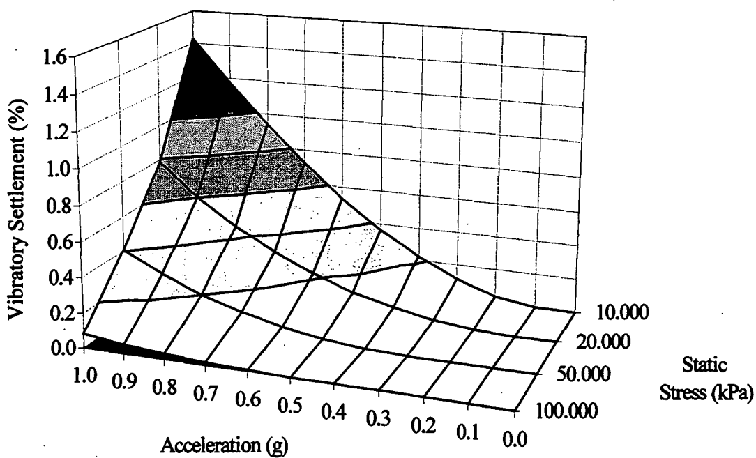
Figure 5.6.2b. Three-dimensional view of Figure 5.6.2a.
