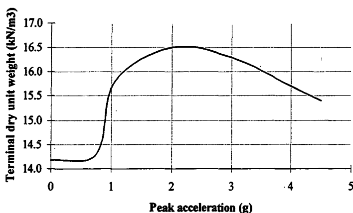
Figure 3.19. Density increase of sands under controlled vertical acceleration, with zero confining pressure (after d’Appolonia et al. , 1969).
