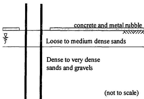
Figure 6.15. Cross-section of pile trials, Flitwick (Case Study 4).
