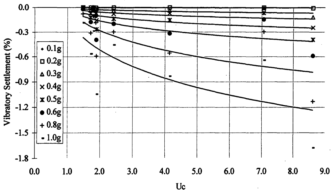
Figure 5.7.2a. Relationship between uniformity coefficient ( U_c ) and settlement (mean stress values, saturated, 25Hz).
