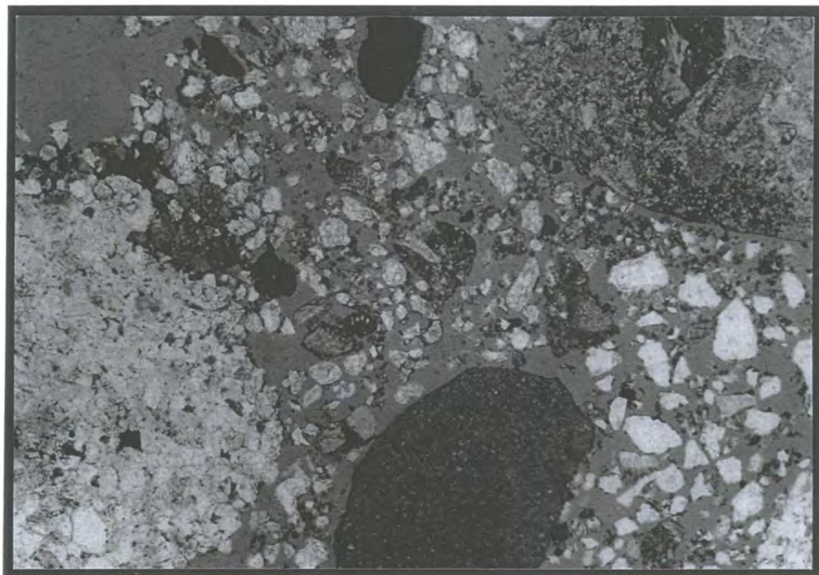
Plate 4.15. Thin-section of sandy fine to medium gravel (x 25 magnification).
