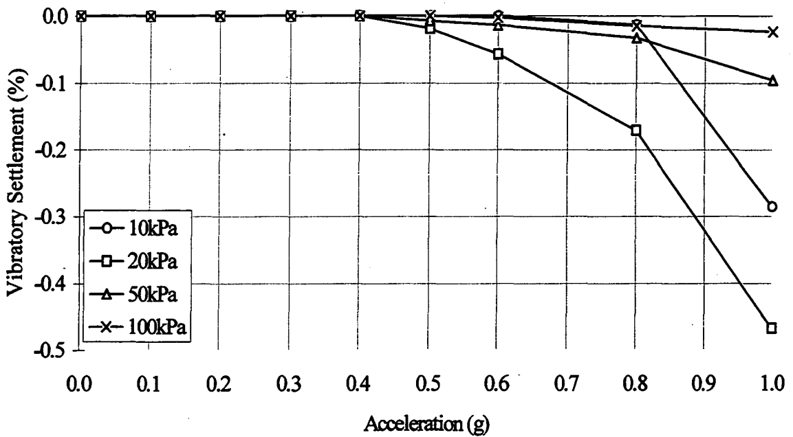
Figure 5.1.4b. Medium uniform sand vibration test settlement results. Saturated, at 40Hz (see Appendix 3: Table A3.4.2, for test data sheet).
