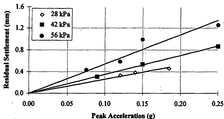
Figure 3.20 The effects of stress of foundation on settlement (after Brumund and Leonards, 1972).
