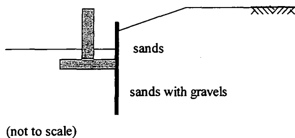
Figure 6.18. Cross-section of the pier construction (Example #2).
