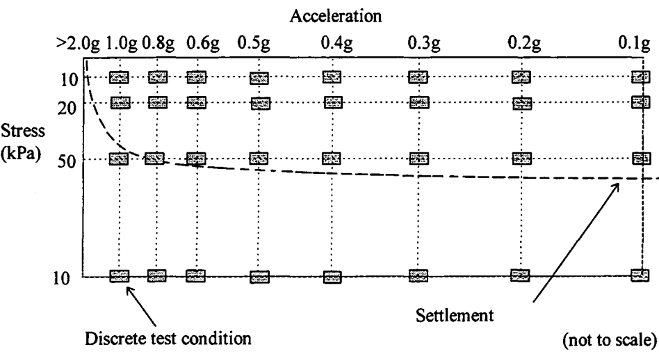
Figure 6.3. Illustrating the discrete points in a soil profile that the low acceleration laboratory test programme models.
