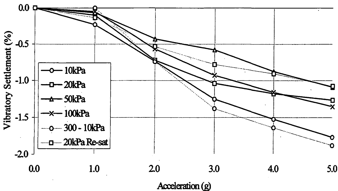
Figure 5.3.3. Garside medium sand, high acceleration vibration test settlement results. Saturated, at 25Hz (see Appendix 3: A3.3.3, for test data sheet).
