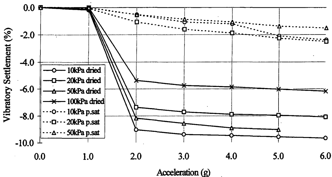
Figure 5.4.4. Medium Leighton Buzzard sand partially saturated and dried high acceleration vibration test settlement results at 25Hz (see Appendix 3: Table A3.5.5; A3.5.6, for test data sheet).
