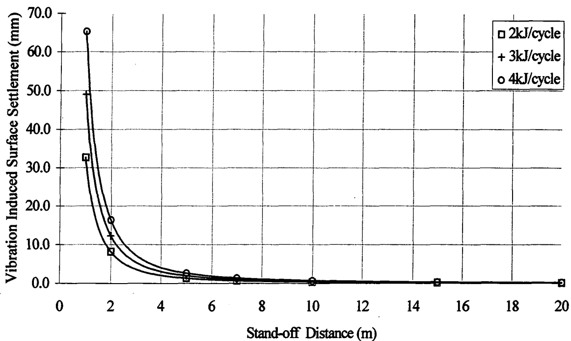
Figure 5.10.2. Surface settlement generated using Equation 5.13 and the vibration settlement equation, 5.8a (see Appendix 4: Table 4.1.1, for test data sheet).
