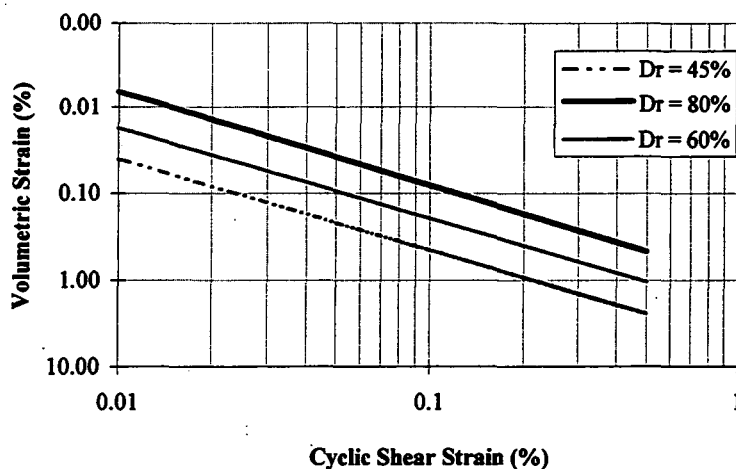
Figure 3.13b. The relationship between volumetric and shear strain for dry sands (after 15 cycles)(after Silver and Seed, 1971a).
