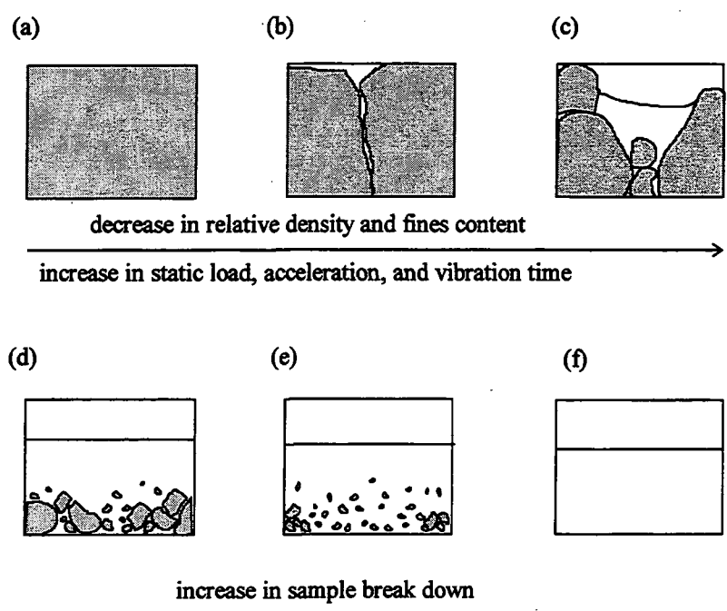
Figure 6.12. The mode of dried sample break-down under the effects of acceleration, stress and time.
