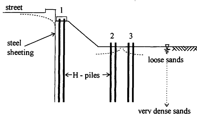
Figure 6.25. Cross-section of H-piles for a building foundation (Paper #5).
