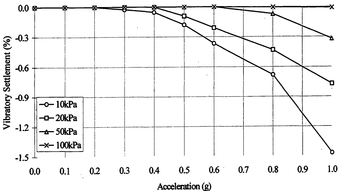
Figure 5.1.8b. Sandy fine gravel vibration test settlement results. Saturated, at 40Hz (see Appendix 3: Table A3.10.2, for test data sheet).
