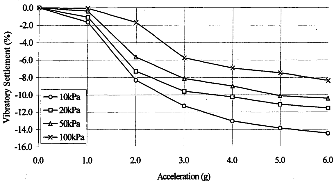
Figure 5.3.10. Sandy fine to medium gravel, high acceleration vibration test settlement results. Saturated, at 25Hz (see Appendix 3; Table A3.11.8, for test data sheet).
