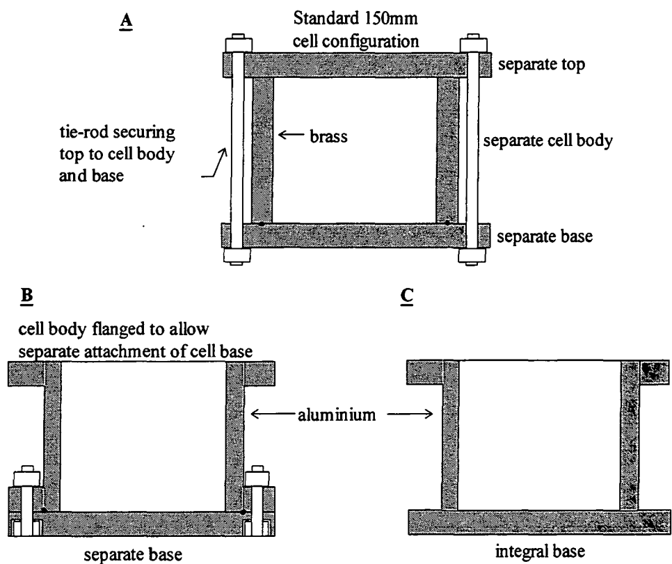
Figure 4.6. Modification of the standard 150mm Rowe Cell. Cell types B and C were used during the laboratory test programme.
