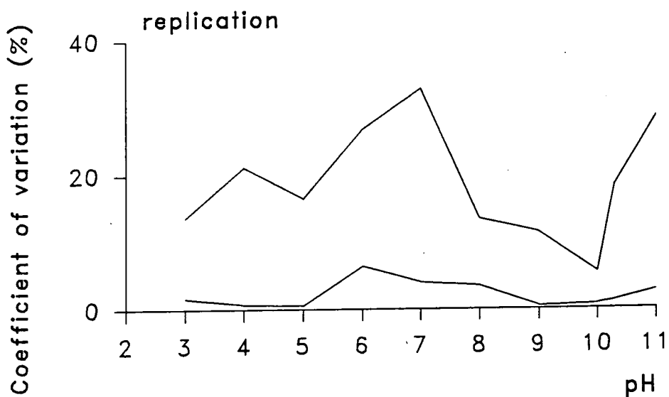
Fig. 5.5a Interplant variability and replication of PMEase activity in Cladonia arbuscula from Middleton Common, using 250 \mu\text{M} pNPP
