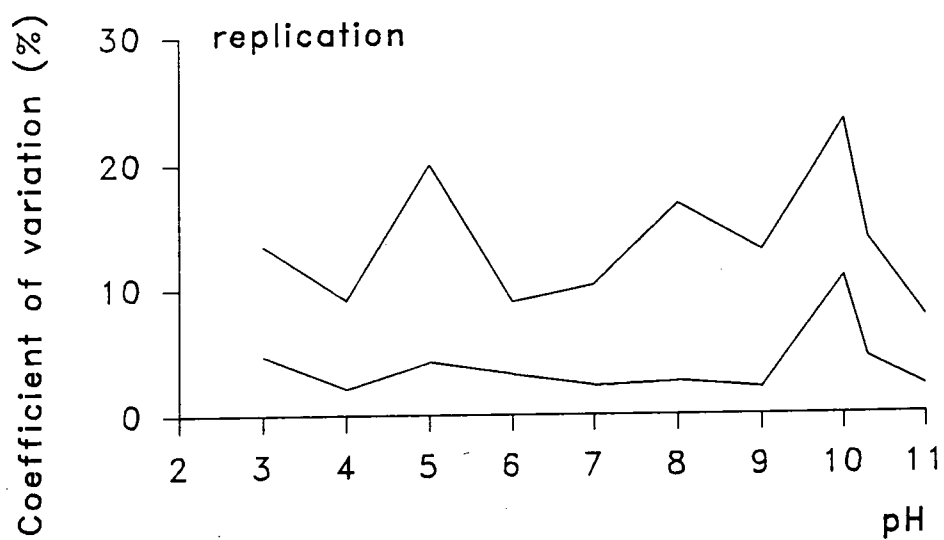
Fig. 5.1a Interplant variability and replication of PMEase activity in Peltigera canina from Windy Nook, using 250 \mu\text{M} pNPP
