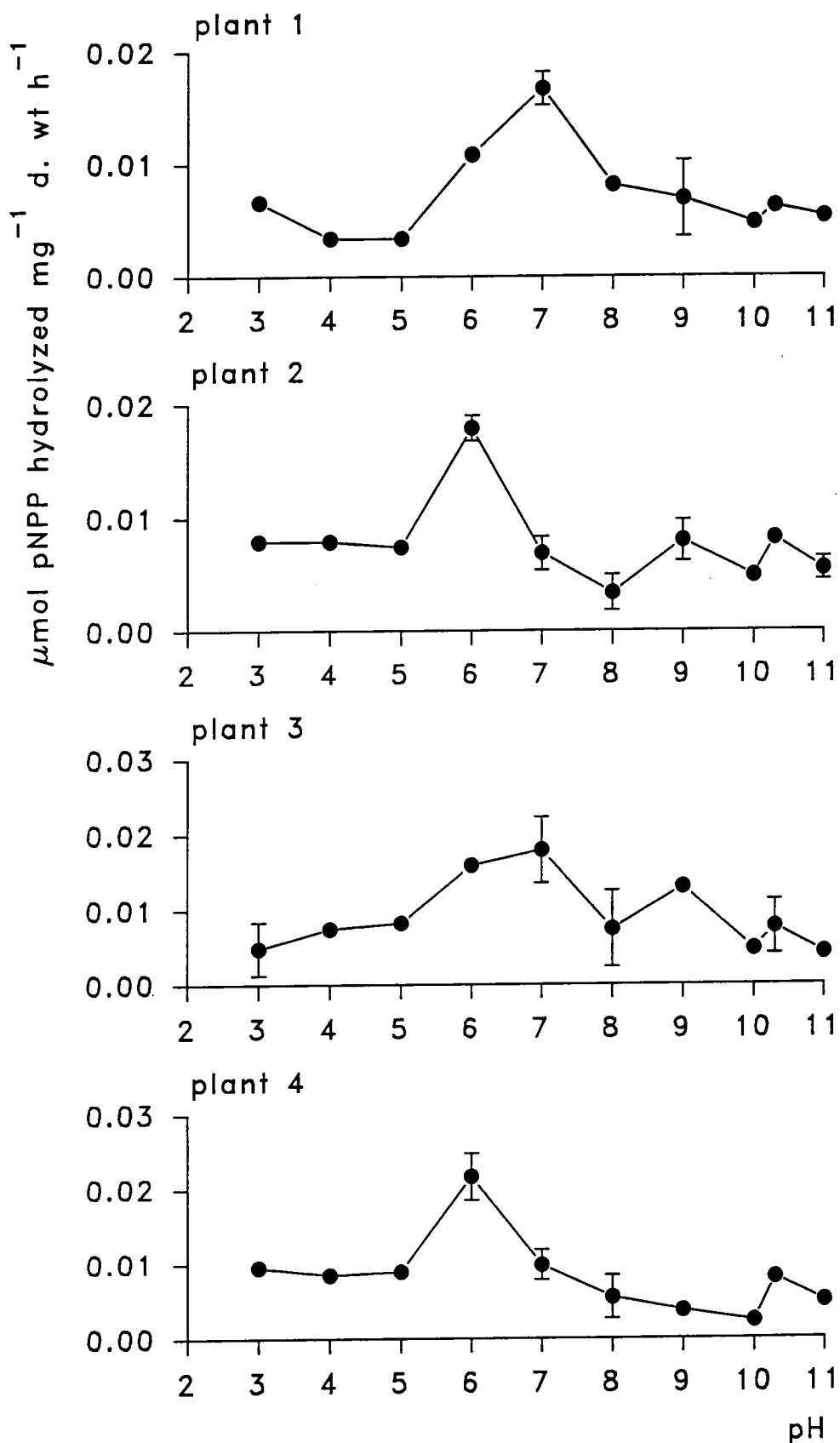
Fig. 5.6 Influence of pH on the PMEase activity of Cladonia arbuscula from Nenthead, using 250 \mu\text{M} pNPP
