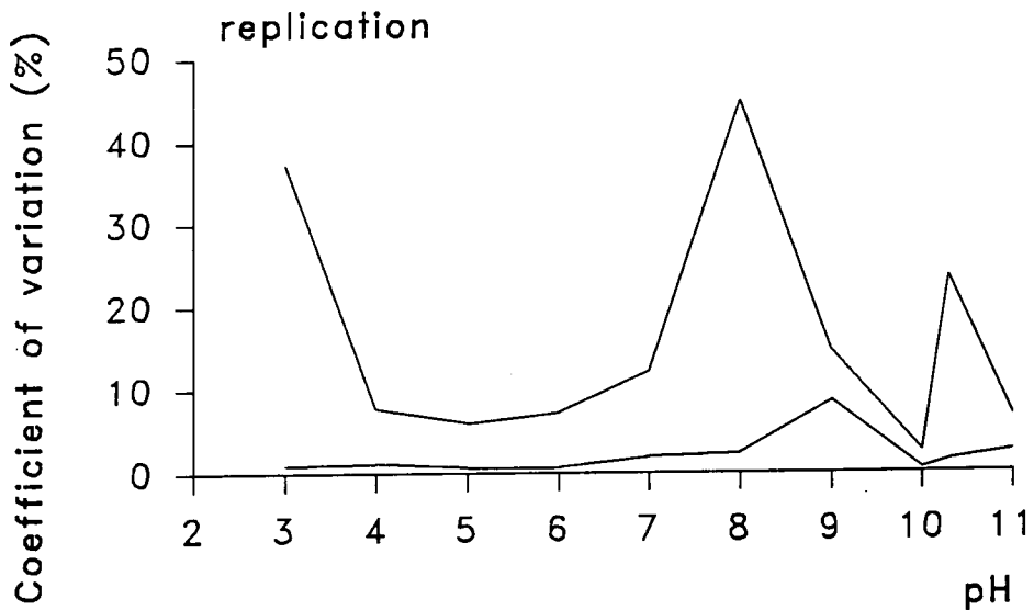
Fig. 5.6a Interplant variability and replication of PMEase activity in Cladonia arbuscula from Nenthead, using 250 \mu\text{M} pNPP
