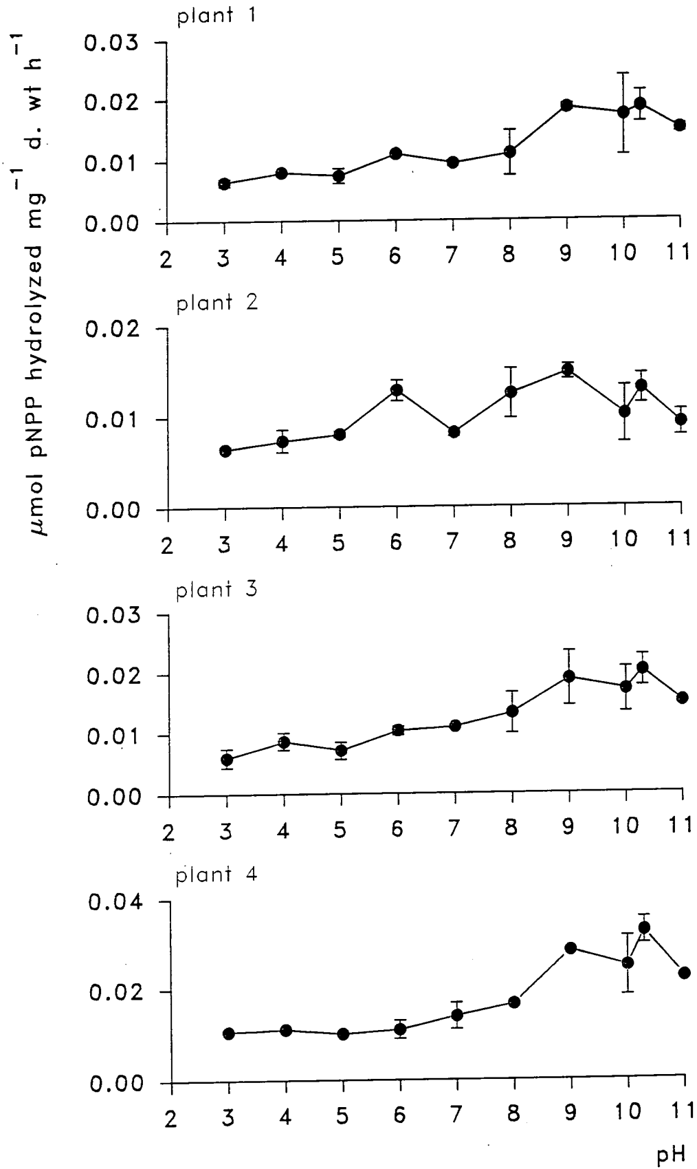
Fig. 5.1 Influence of pH on the PMEase activity of Peltigera canina from Windy Nook, using 250 \mu\text{M} pNPP
