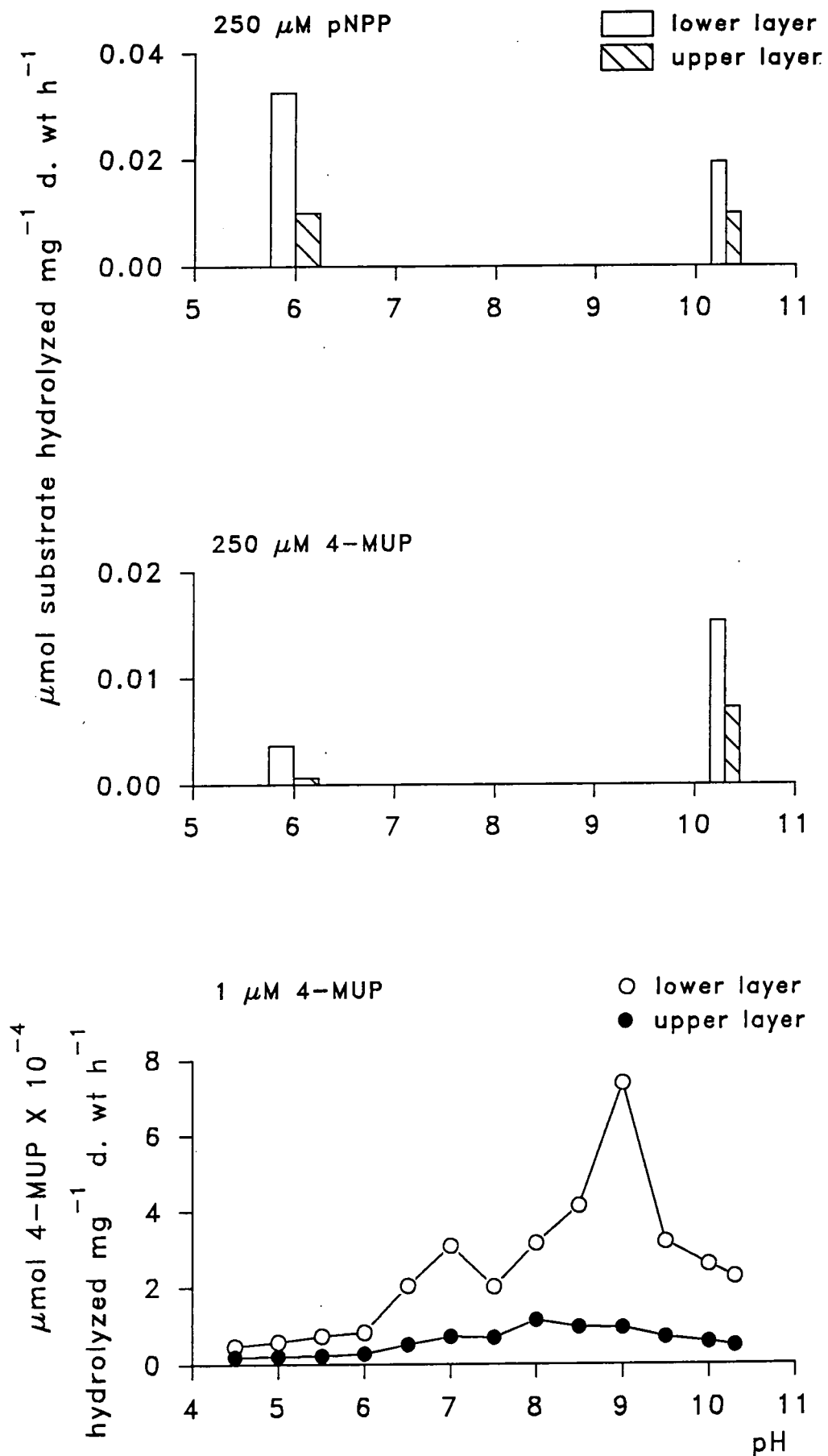
Fig. 5.15 Influence of pH and substrate on the PMEase activity of the symbionts of Peltigera canina 1 Nenthead
