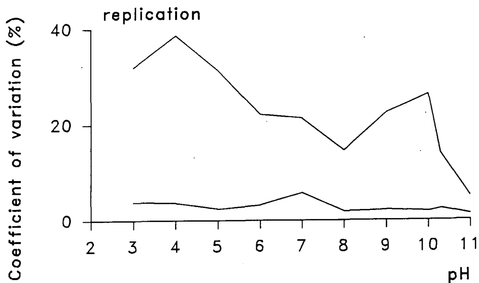
Fig. 5.4a Interplant variability and replication of PMEase activity in Peltigera praetextata from Nenthead, using 250 \mu\text{M} pNPP
