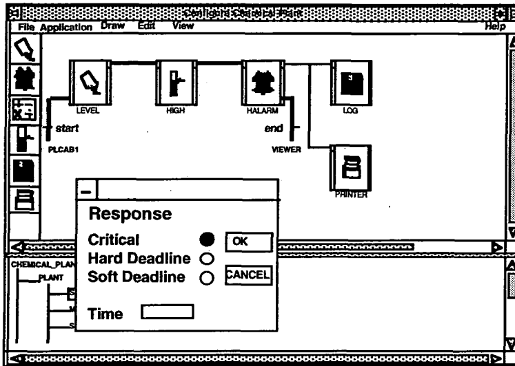
Figure 86 Example Control Flow Requirement
