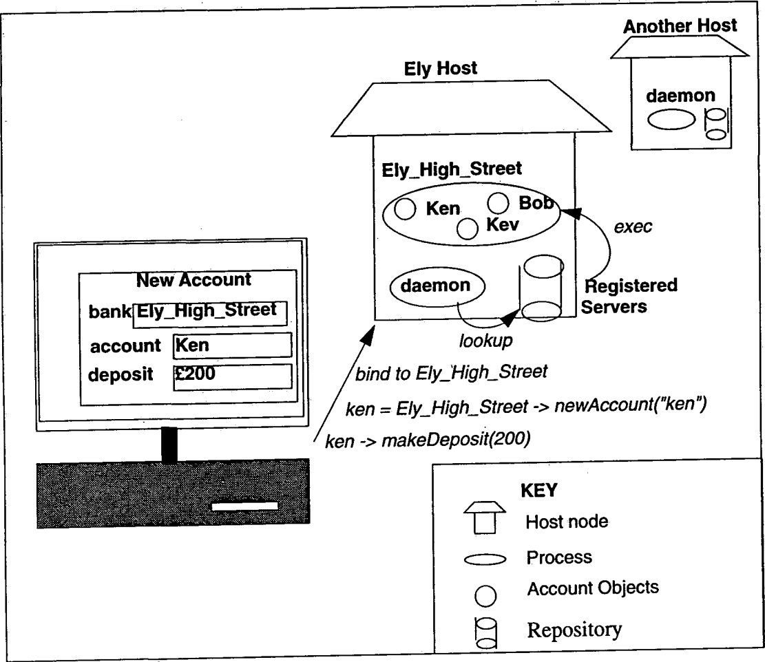
Figure 93 Scenario to Create a New Account
