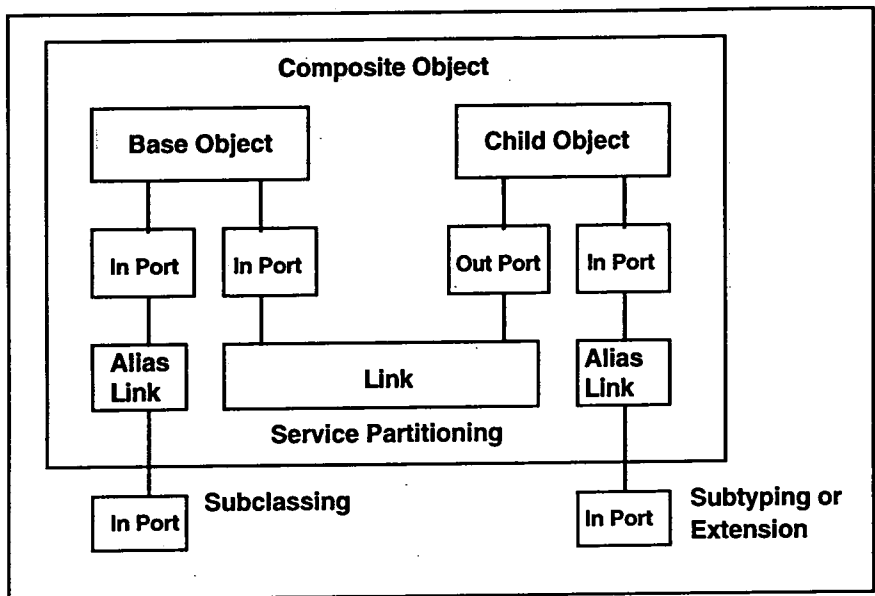
Figure 79 Using Hierarchical Composition to Synthesise Inheritance
