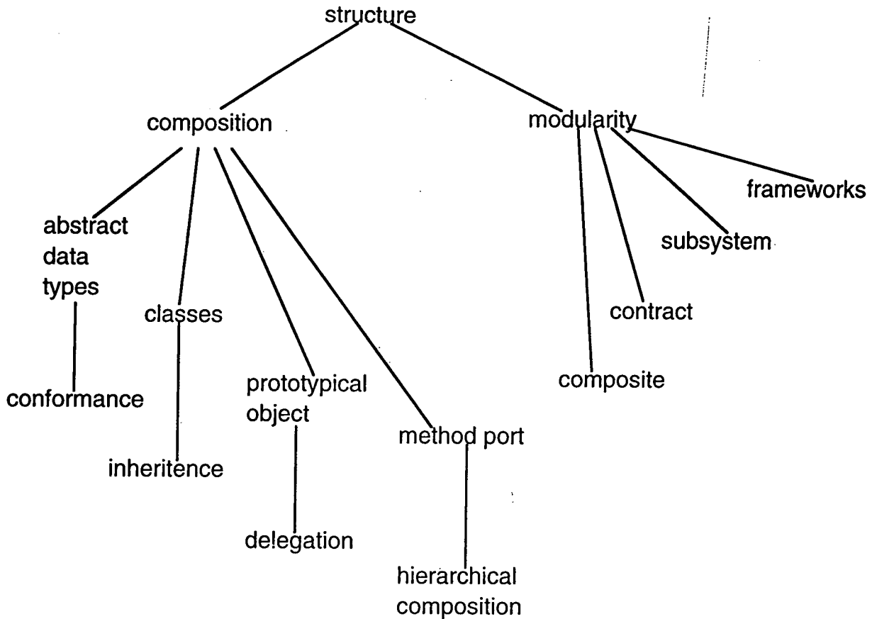
Figure 6 Types of structure
