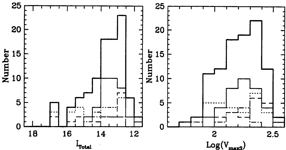
Figure 5.4: Total I-band magnitude and log-rotation velocity histograms for the final sample of 99 galaxies. On both plots the solid thick line indicates the distribution of the whole sample. Other line types show the respective distribution for each of the four clusters; Solid line for Coma, dotted line for A2199, dashed line for A2634 and dot-dashed for A194.
