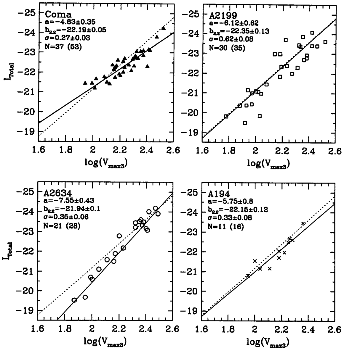
Figure 5.20: The results of applying Hendry's fitting technique to the separate clusters. A solid line on each relationship represents the maximum likelihood fit that attempts to correct for selection bias. The results of each fit are displayed in the upper left-hand corner of each panel. A dotted line represents the composite fit line.
