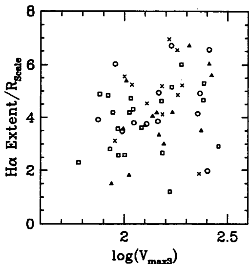
Figure 6.15: A graph of H \alpha rotation curve extent in terms of disk scale length plotted against log-rotation velocity. No trend is evident, so poor quality rotation curves are unlikely to have a systematic effect on the TF slope.
