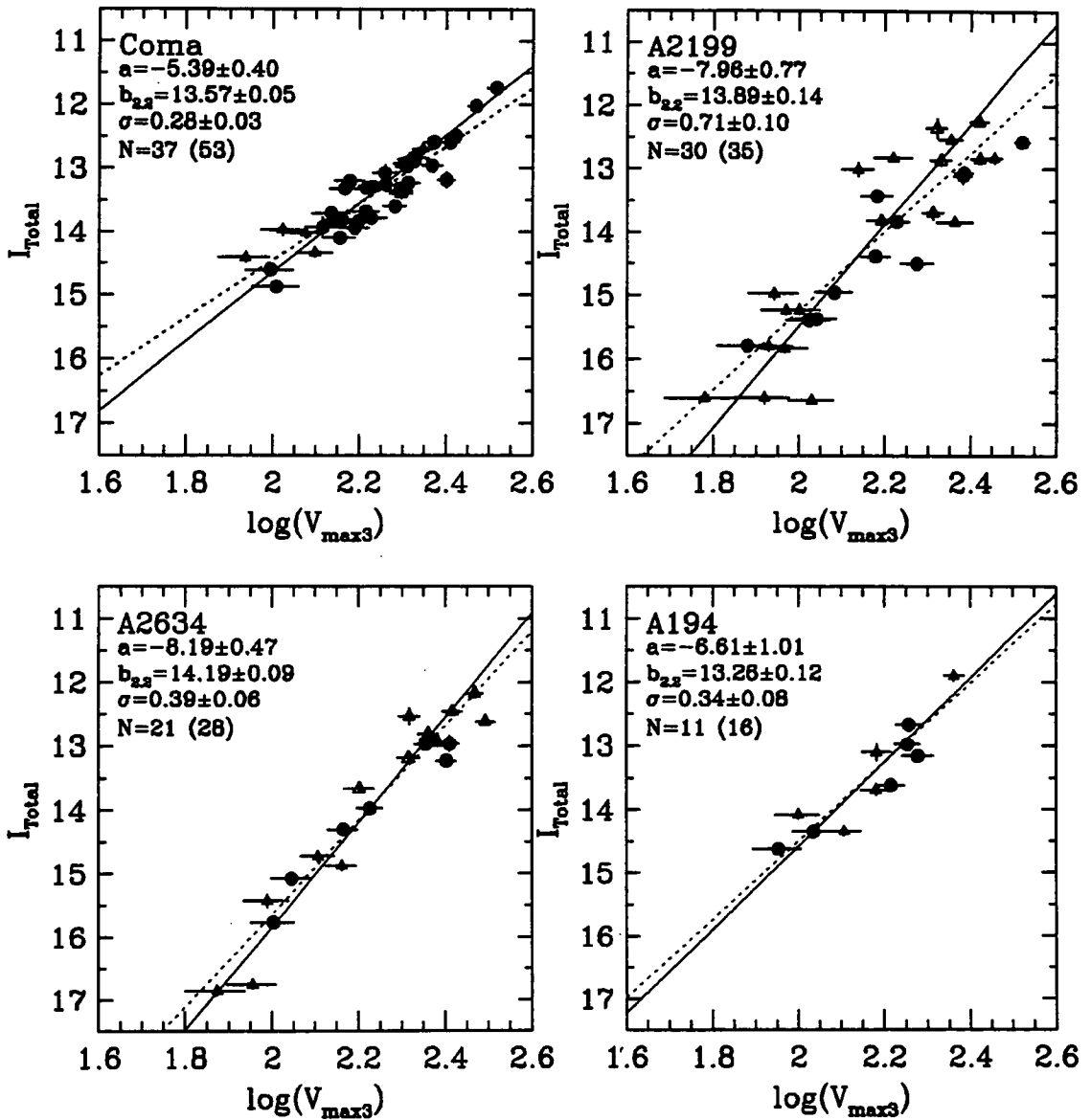
Figure 6.11: The same Tully-Fisher relations as displayed in Figure 5.18. In this instance, the data set is divided into groups of high and low quality. High quality points are marked with a filled circle, low quality points are indicated with a filled triangle.
