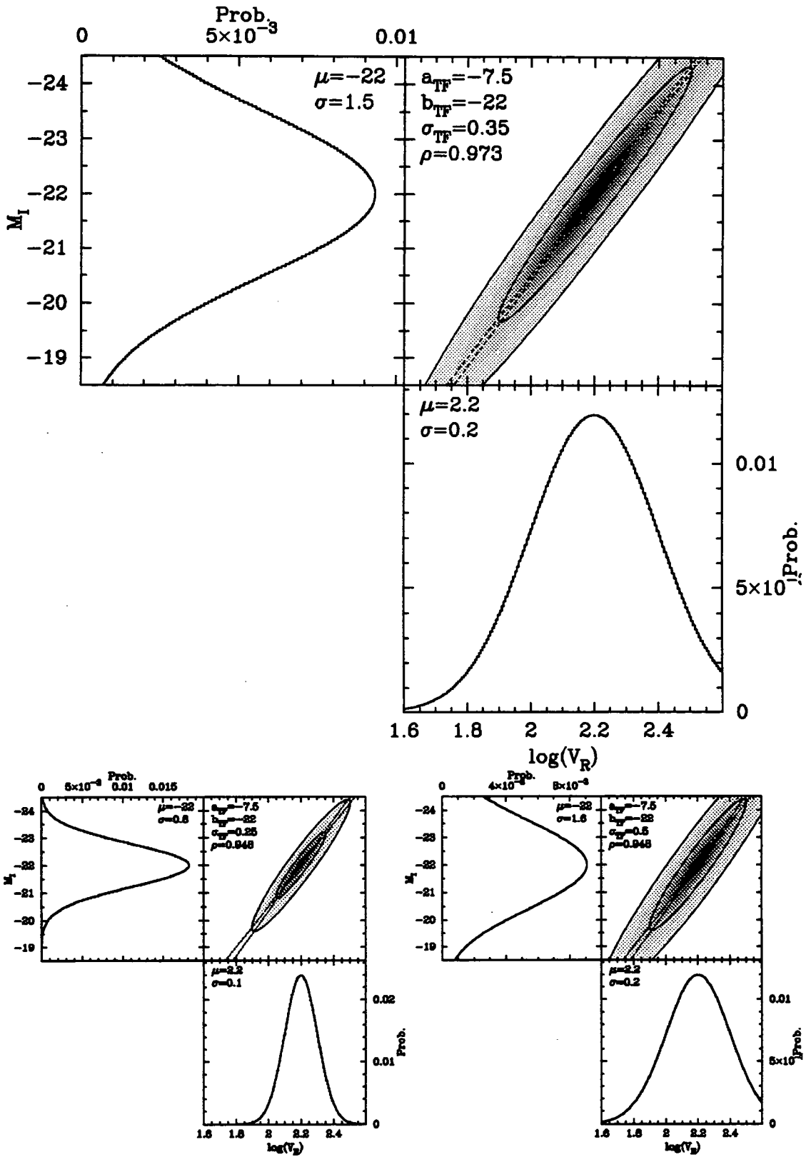
Figure 5.6: A graphical representation of the Tully-Fisher relation as a bivariate normal distribution. The upper portion of the figure displays a distribution with parameters similar to the selected sample. Plotted in the left-hand and lower panels is the probability distributions of total magnitude and rotation velocity. The greyscale image indicates the joint probability distribution where points of highest probability density are marked with black. Direct and inverse regression lines are marked with dotted lines. The two lower plots show how changes in the sample properties affect the probability distribution.
