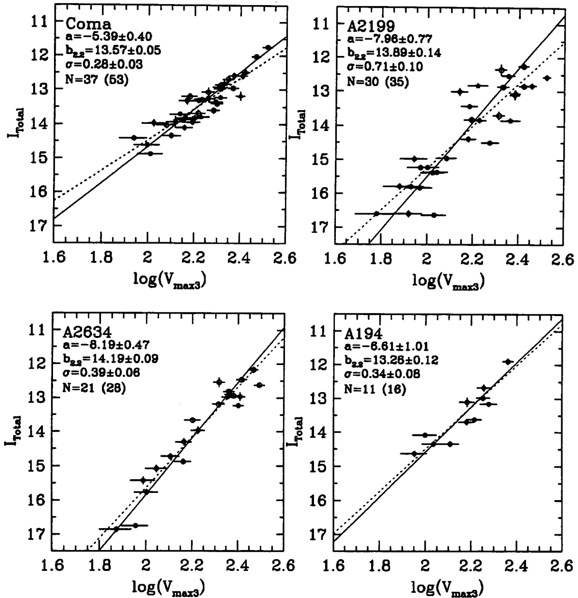
Figure 5.18: The Tully-Fisher relation within the four target clusters. The symbols are the same as in figure 5.2. \pm 1\sigma error estimates in magnitude and log-rotation velocity are marked on each point. The weighted inverse regression line of \log V_{\text{max}3} upon I_{\text{Total}} is marked as a solid line on each relation. The details of each of these fits are marked in the upper left of each panel. The regression of I_{\text{Total}} upon \log V_{\text{max}3} is represented in each case as a dotted line.
