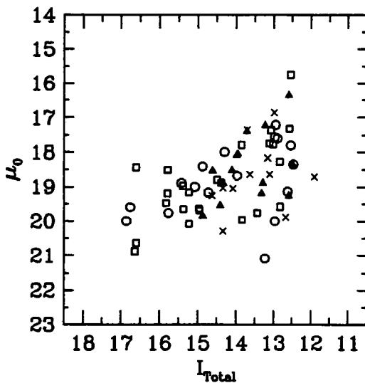
Figure 5.13: Plots of surface brightness against apparent total I-band magnitude for 99 galaxies within the final TF sample. In both cases different symbols indicate the cluster to which each galaxy belongs. Filled triangles mark Coma galaxies, A2634 galaxies are represented by circles, A2199 by squares and A194 by crosses.
