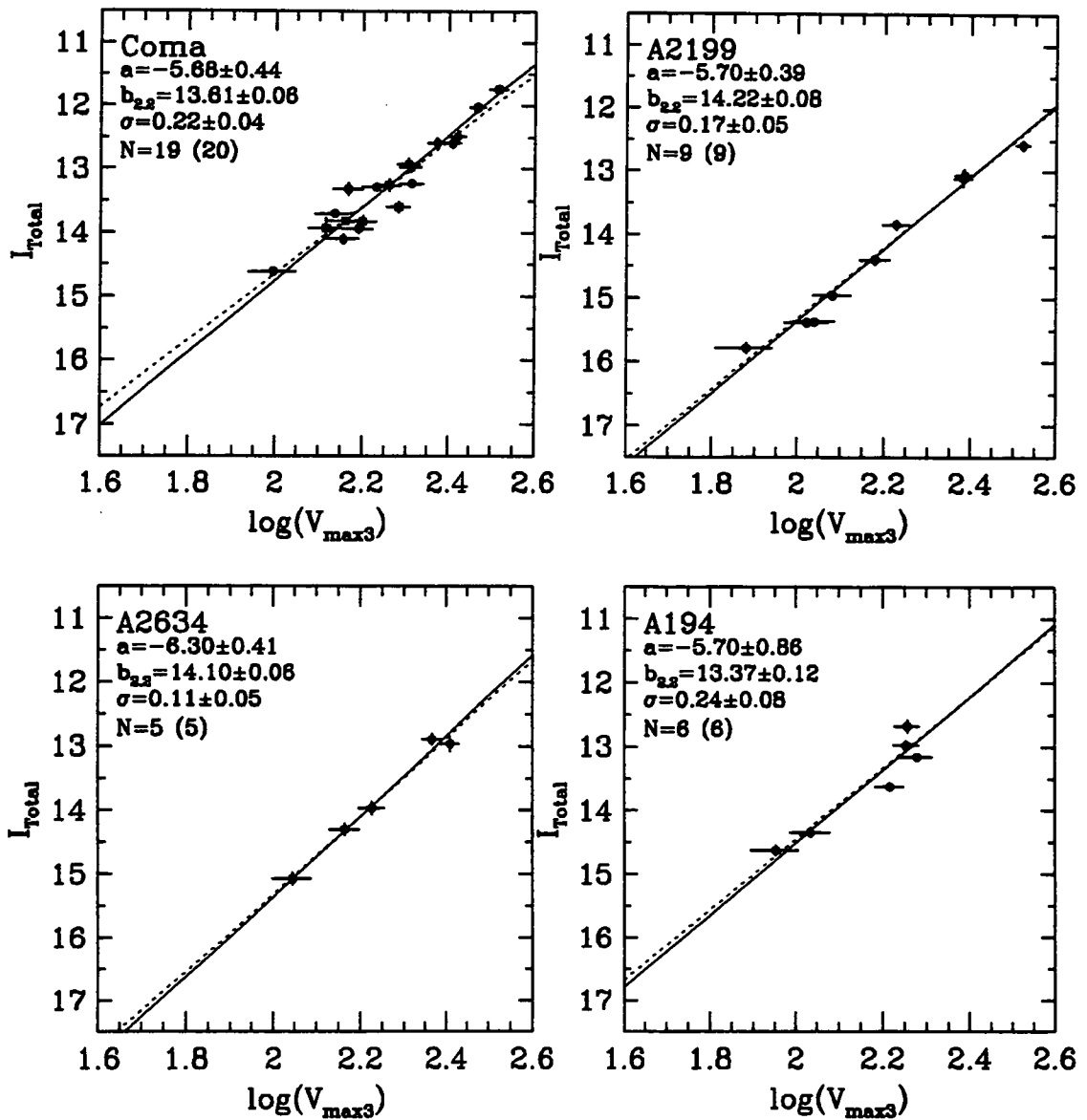
Figure 6.17: Four plots of the Tully-Fisher relation for the four cluster samples after rejection of low quality points and a \pm 1000 \text{ km s}^{-1} redshift cut has been applied.
