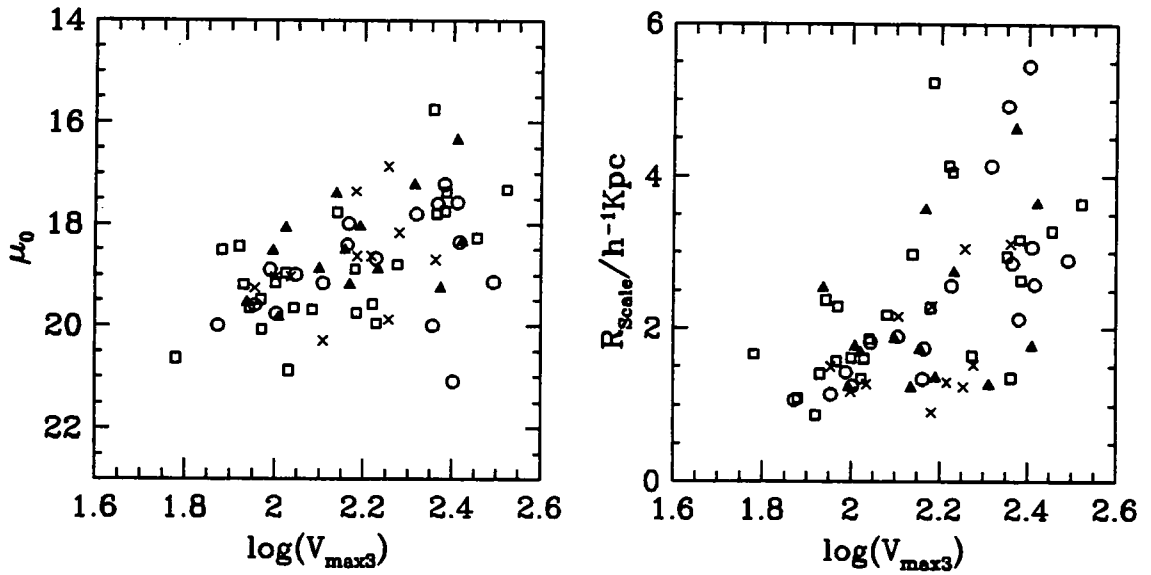
Figure 5.10: Two plots of surface brightness against log-rotation velocity and disk scale length against log-rotation velocity for galaxies within the TF sample. In both cases different symbols indicate the cluster to which each galaxy belongs. Filled triangles mark Coma galaxies, A2634 galaxies are represented by circles, A2199 by squares and A194 by crosses.
