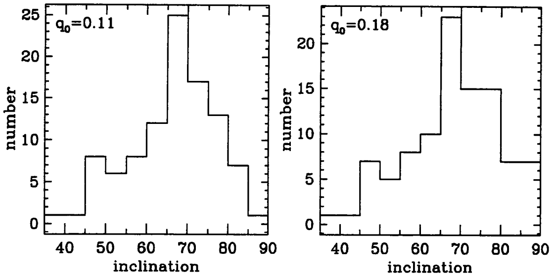
Figure 5.21: Histograms indicating two possible inclination distributions for the sample. The left-hand panel shows the calculated distribution assuming that the mean edge-on axial ratio, q_0 , of the sample galaxies is 0.11. The right-hand graph shows the distribution if q_0 is 0.18. As randomly oriented disks are more likely to be viewed edge-on, q_0 = 0.18 is considered more likely.
