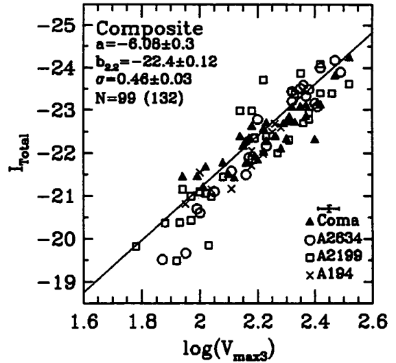
Figure 5.19: A Composite Tully-Fisher formed by combining the four separate cluster TF relations. The entire dataset was simultaneously fitted for a single slope and three distance moduli relative to Coma using a maximum likelihood technique developed by Martin Hendry. The error bars indicate the mean errors for the sample.
