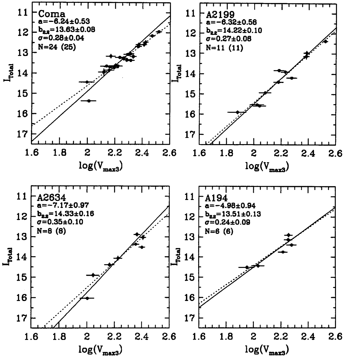
Figure 6.16: The same Tully-Fisher relations for each cluster that appear in Figure 6.12 after the expanding cluster correction has been applied. The scatter is only reduced in the A2199 sample the scatter increases in the other cluster. The marked lines and symbols have the same meaning as in Figure 5.18. 6.12
