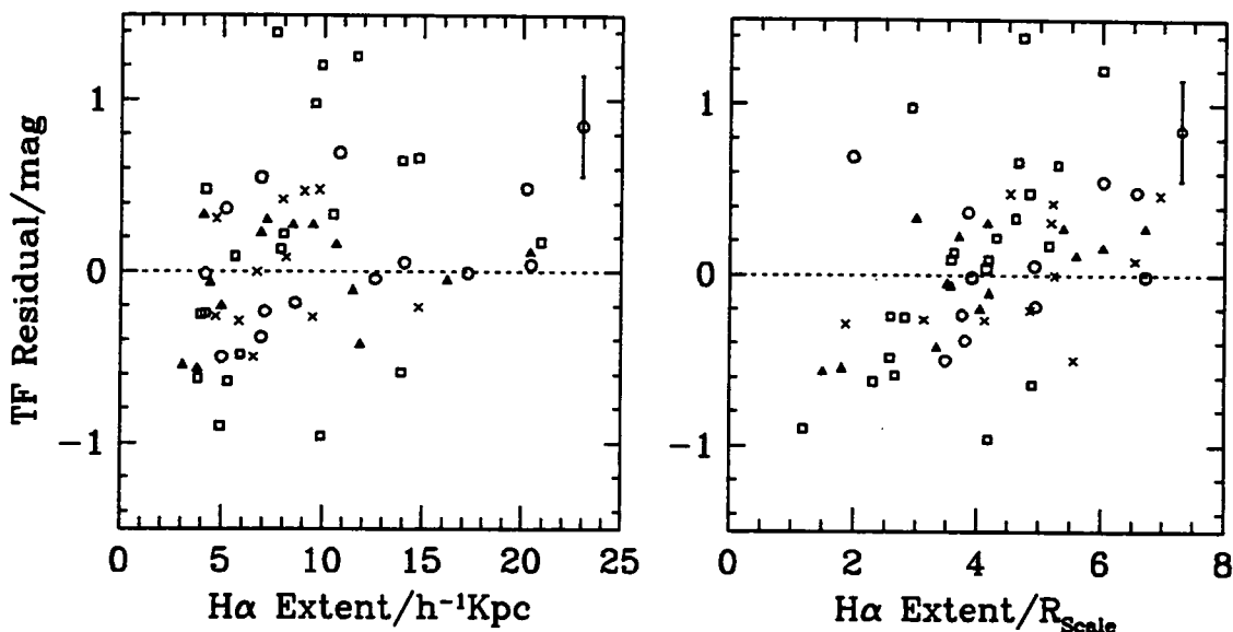
Figure 6.14: Left: The Tully-Fisher residuals for each galaxy plotted against the maximum extent of each objects H \alpha rotation curve in h^{-1} Kpc. Right: The same points plotted against rotation curve extent in terms of disk scale length. Galaxies with poor H \alpha extent with respect to their size tend to have negative TF residuals, i.e. lower rotation velocities than expected.
