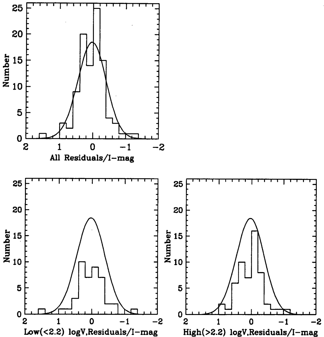
Figure 6.4: Histograms of the magnitude residuals about the fitted relation for all 99 galaxies in the main sample. The Gaussian curve marked on all graphs has a standard deviation of 0.43 mags. The lower plots shows the same data divided into two parts. The lower left histogram displays the residuals for galaxies with \log V_{\text{Rot}} below 2.2. The right-hand plot show residuals for objects with \log V_{\text{Rot}} > 2.2 .
