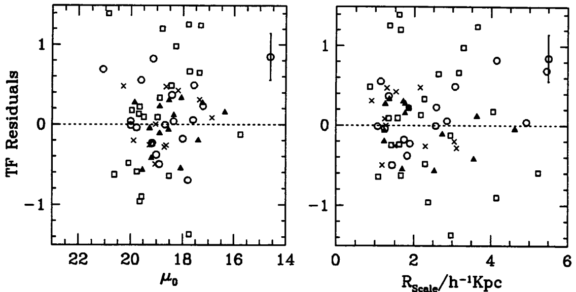
Figure 6.13: Left: A graph showing TF residuals against surface brightness for the sample galaxies. Right: TF residuals versus disk scale length for the same galaxies. The four symbol types indicate data from each cluster; filled triangles denote Coma, Open circles Abell 2634, Open squares Abell 2199, and Crosses mark Abell 194 points.
