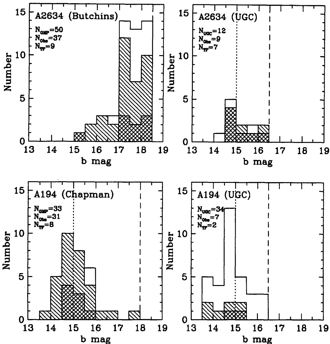
Figure 5.9: Four histograms showing the B-band magnitude distribution for galaxies selected from the Abell 2634 and Abell 194 clusters. The left-hand plots show the distribution for the samples selected from plate scans. The right-hand plots indicate the sample magnitude distribution of objects taken from the UGC catalogue. The imposed magnitude limits of 18.0 and 16.5 are marked as dashed lines. The suspected completeness limit of the UGC catalogue is shown with a dotted line. The open histograms indicate selected objects and hatched and cross-hatched bars indicate observed and final TF galaxies.
