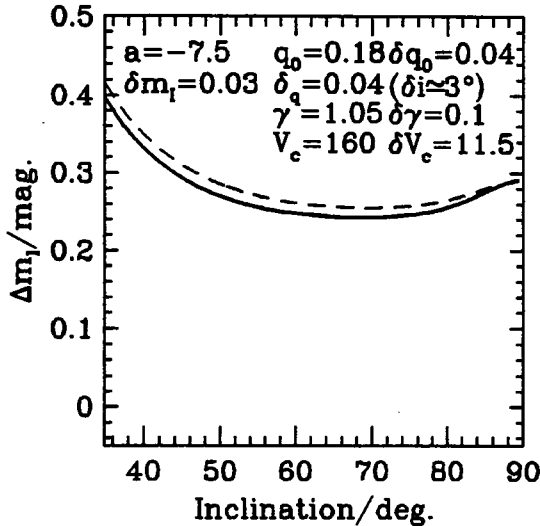
Figure 6.2: The scatter introduced by disk ellipticity errors for galaxies at different inclinations. If all sources of error are considered the effects of correlation between errors becomes relatively unimportant. The marked lines have the same meaning as in Figure 6.1.
