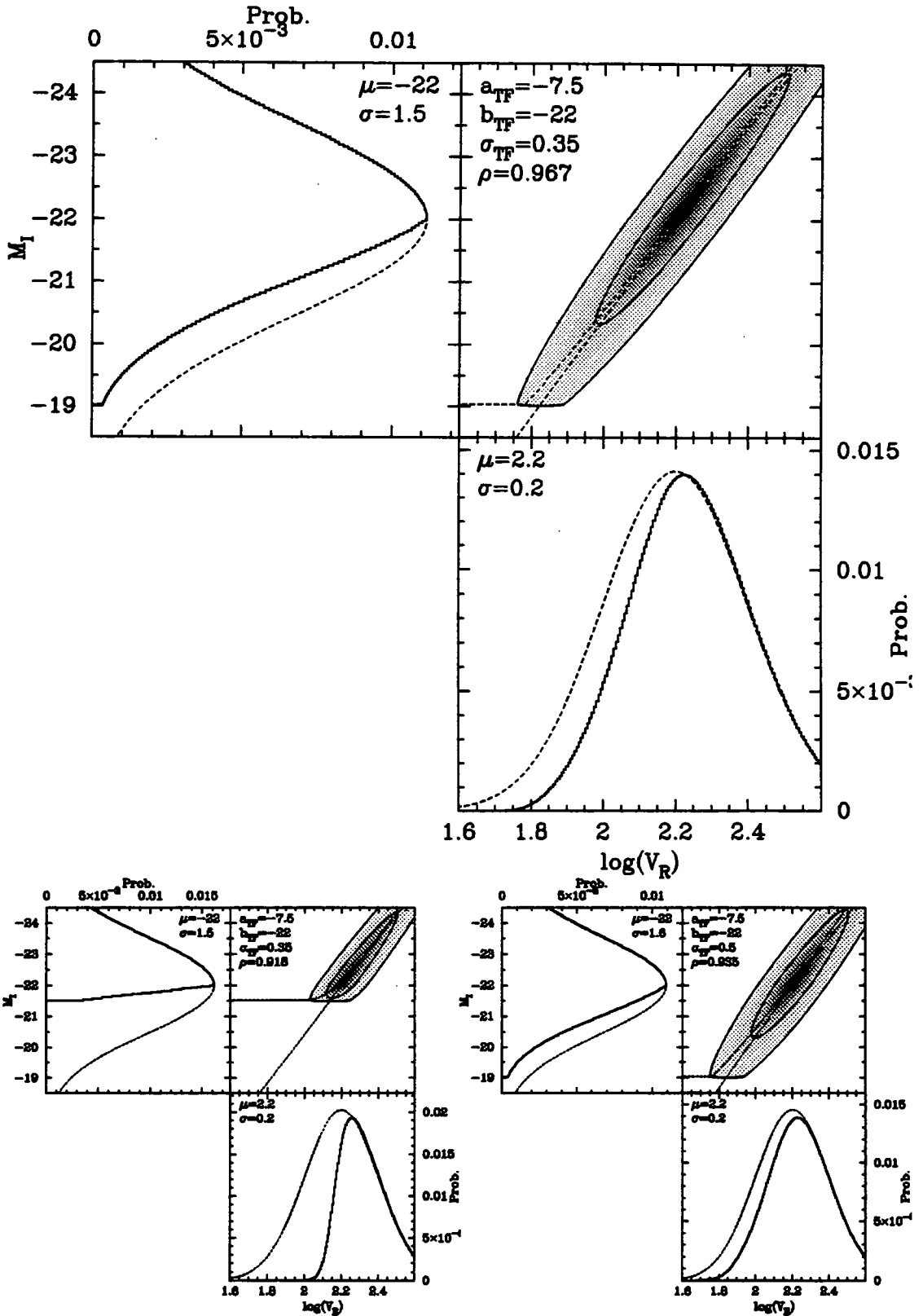
Figure 5.7: The same distributions as shown in Figure 5.6 with magnitude selection effects added. Histograms marked with dashed lines indicate the original distribution before selection. Note how the inverse regression line (lower of dashed lines on greyscale) remains unchanged, whereas the direct line is biased towards brighter magnitudes. The lower plots depict the result of a brighter selection limit or larger TF scatter on the amount of bias. See text for detailed discussion.
