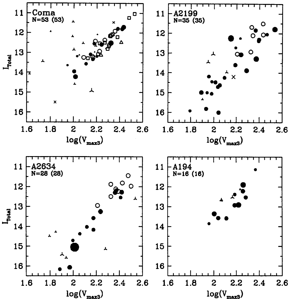
Figure 5.2: The Tully-Fisher relation for the four clusters within our sample. No points have been rejected, all galaxies with measurements are shown. Solid circles represent galaxies from the present sample, galaxies with poor quality measurements are marked with crosses. In both cases the size of the point indicates the extent of the H \alpha rotation curve. Open circles represent data from previous observations and for the Coma cluster open squares and triangles represent measurements by Bernstein et al. (1994).
