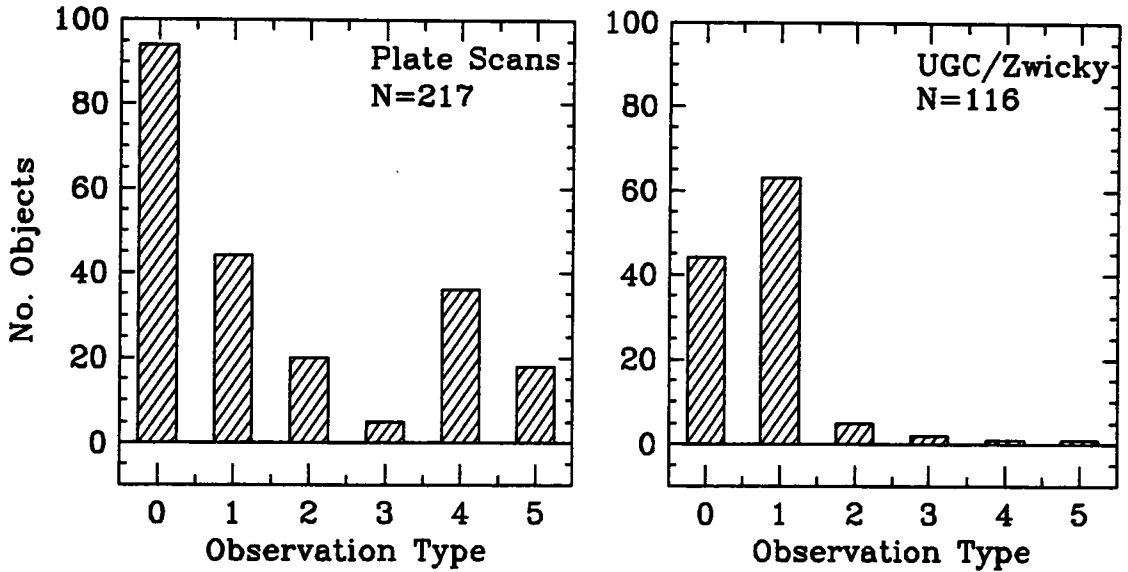
Figure 5.5: Two Histograms displaying the outcome of observations of 333 galaxies selected from photographic plate scans or either UGC or Zwicky catalogues. The observation type codes indicate; 0=not observed, 1=in final TF sample, 2=rotation curve with poor extend, 3=only nuclear H \alpha emission, 4=no H \alpha emission, 5=wrong morphology (e.g. star or elliptical). A larger fraction of the fainter objects selected have proved to have weak or no H \alpha emission lines.
