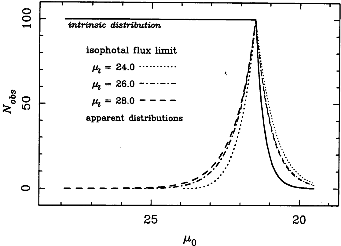
Figure 5.12: A reproduction of McGaugh (1996), Figure 3. Showing the apparent distribution of disk surface brightness of galaxies selected from catalogues limited by isophotal magnitude.
