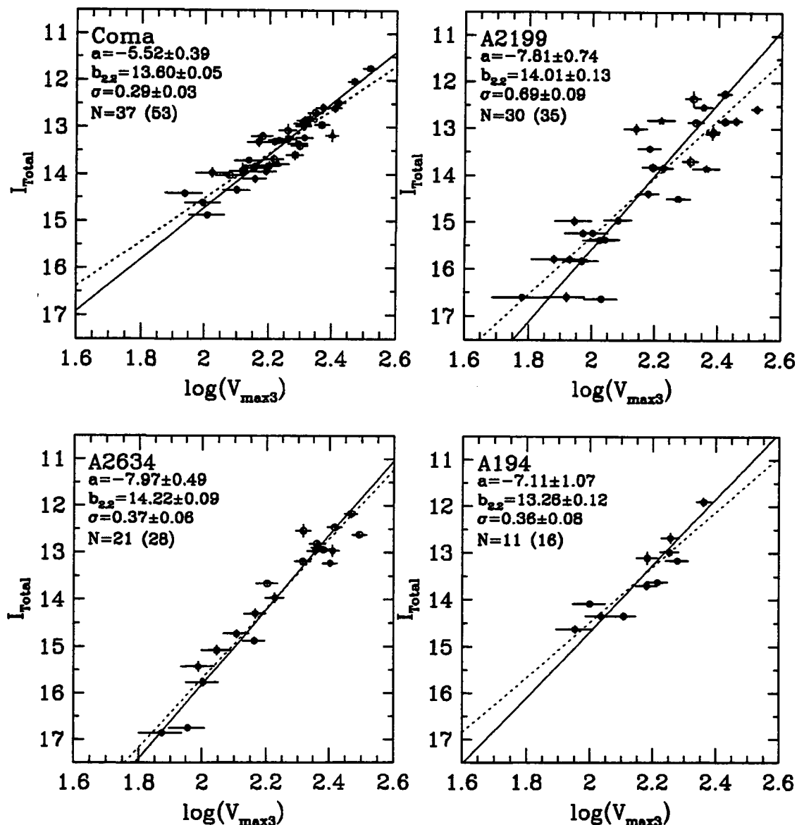
Figure 5.17: The Tully-Fisher relation within the four target clusters. The symbols are the same as in figure 5.2. \pm 1\sigma error estimates in magnitude and log-rotation velocity are marked on each point. The regression line of \log V_{\text{max}3} upon I_{\text{Total}} is marked as a solid line on each relation. The details of each of these fits are marked in the upper left of each panel. The regression of I_{\text{Total}} upon \log V_{\text{max}3} is represented in each case as a dotted line.
