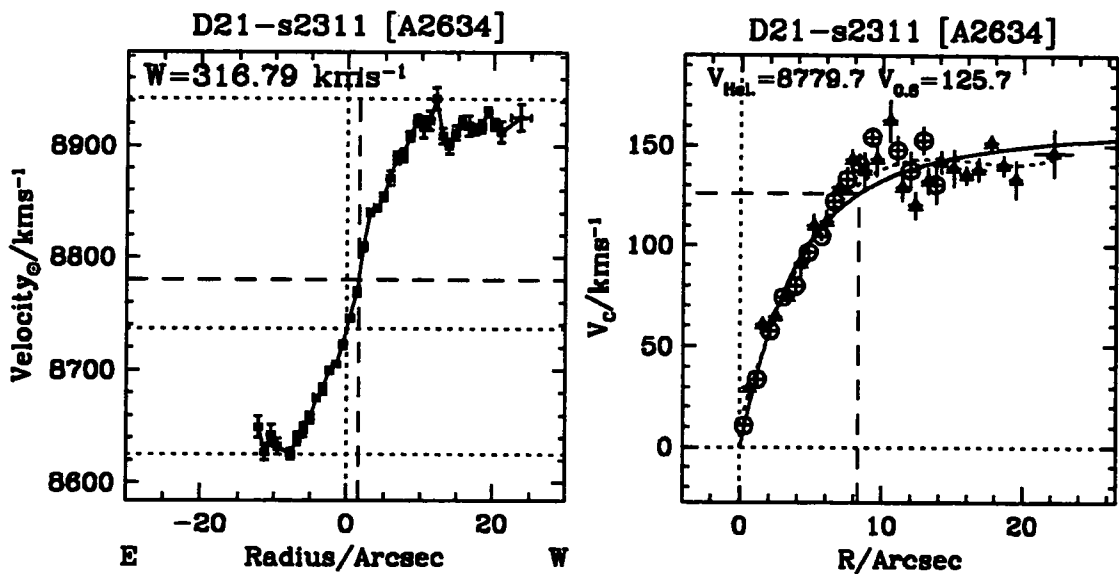
Figure 4.2: Left Panel: An example of a H\alpha rotation curve generated from the spectrum shown in Figure 4.4.1. The heliocentric radial velocity of each point on the galaxy is plotted against radius in arcseconds. The vertical dotted line represents the optical centre of the rotation curve where the emission line crosses the peak in the continuum emission. The dashed vertical line shows the kinematic centre found by folding the curve, the two central horizontal lines show the different radial velocities which would be attributed to these centres. This shows that finding the correct centre is crucial in giving the galaxy a correct radial velocity. The top and bottom horizontal dotted lines show the maximum and minimum velocities within the curve and demonstrate how a velocity width parameter based on the difference between the two is affected by noise. Right Panel: The same rotation curve is displayed after being folded in such a way as to maximise the symmetry between the two halves of the curve. The solid curve is the result of the three parameter fitting function and the dotted curve is the smoothed spline fit. The dashed line marks V_{0.6R_{opt}} , the interpolated rotation velocity at 0.6 of the optical radius.
