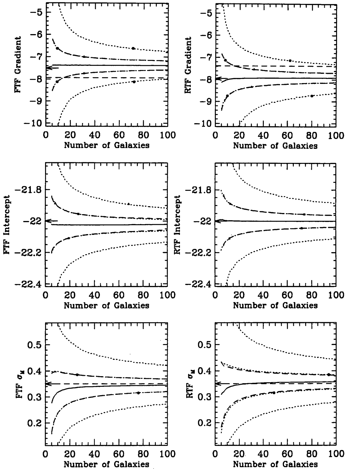
Figure 5.15: Six line plots of output from a Monte-Carlo simulation of the Tully-Fisher fitting procedure for sample sizes ranging from 5 to 100 galaxies. With magnitude selection effects that closely match the present sample. The marked lines have the same meaning as in Figure 5.14. The circles, triangles and squares indicate at which point the \pm 1\sigma and \pm 2\sigma confidence limit lines are within 10%, 5% and 2% of the mean predicted value. Note that in the case of magnitude-only selection the forward regression line becomes biased, whereas the reverse regression remains unaffected.
