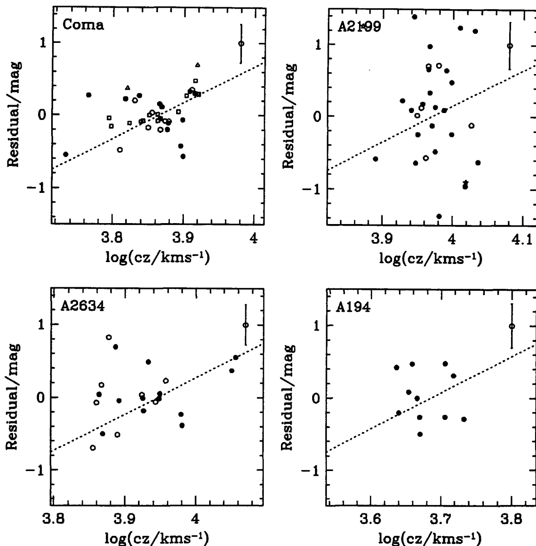
Figure 6.8: Tully-Fisher residuals versus log-redshift for galaxies in the sample. The symbols have the meaning as those shown in Figure 5.2. The dotted line has a gradient of 5 and passes through zero at the redshift of each cluster. Field galaxies on the Hubble flow would be expected to follow this line.
