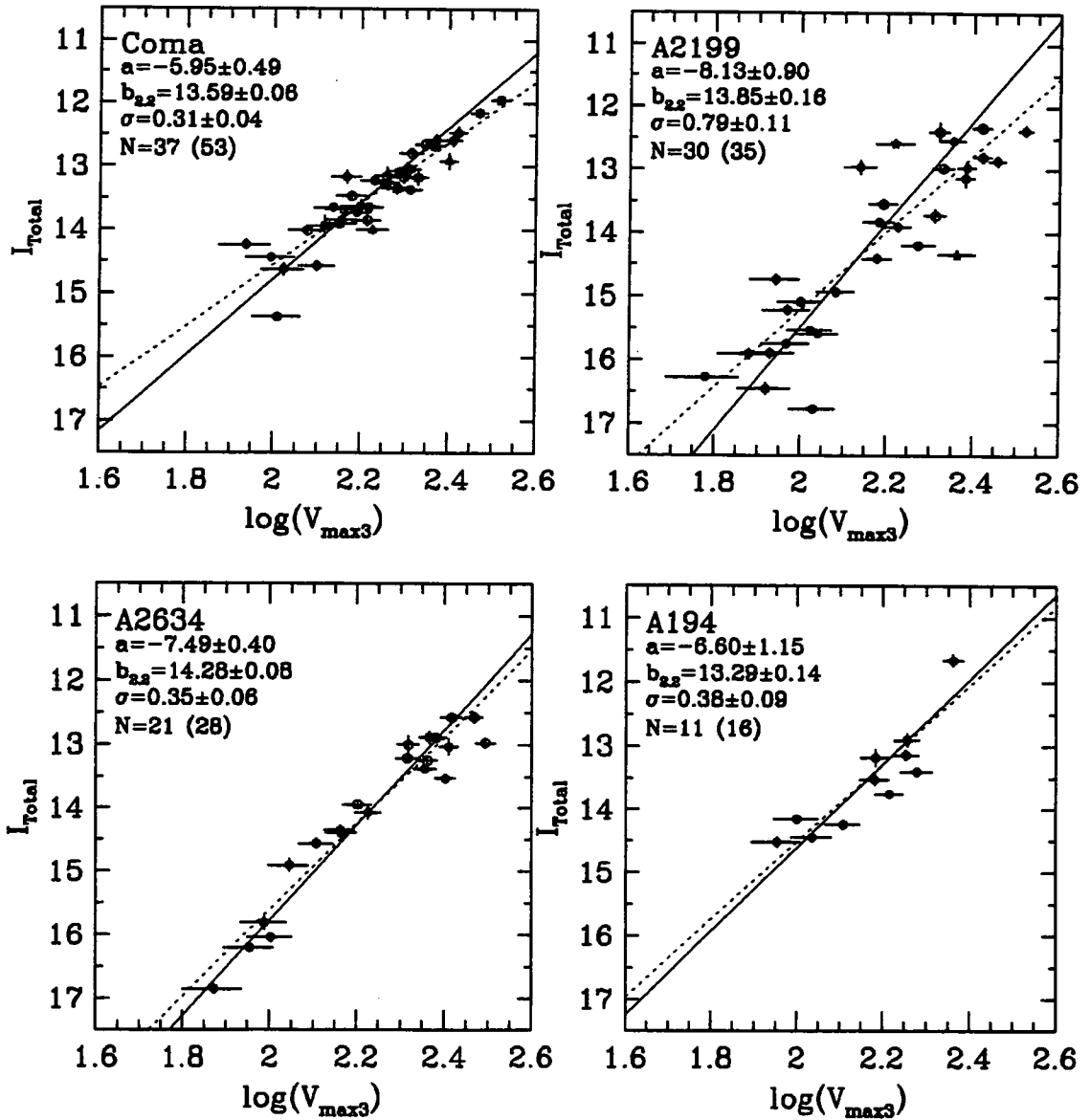
Figure 6.9: The Tully-Fisher relation within the four target clusters. The symbols are the same as in figure 5.2. \pm 1\sigma error estimates in magnitude and log-rotation velocity are marked on each point. The weighted inverse regression line of \log V_{\max 3} upon I_{\text{Total}} is marked as a solid line on each relation. The details of each of these fits are marked in the upper left of each panel. The regression of I_{\text{Total}} upon \log V_{\max 3} is represented in each case as a dotted line. The “expanding” cluster model correction adopted by Willick et al. has been applied to all points. Open circles represent data from previous observations and for the Coma cluster open squares and triangles represent measurements by Bernstein et al. (1994).
