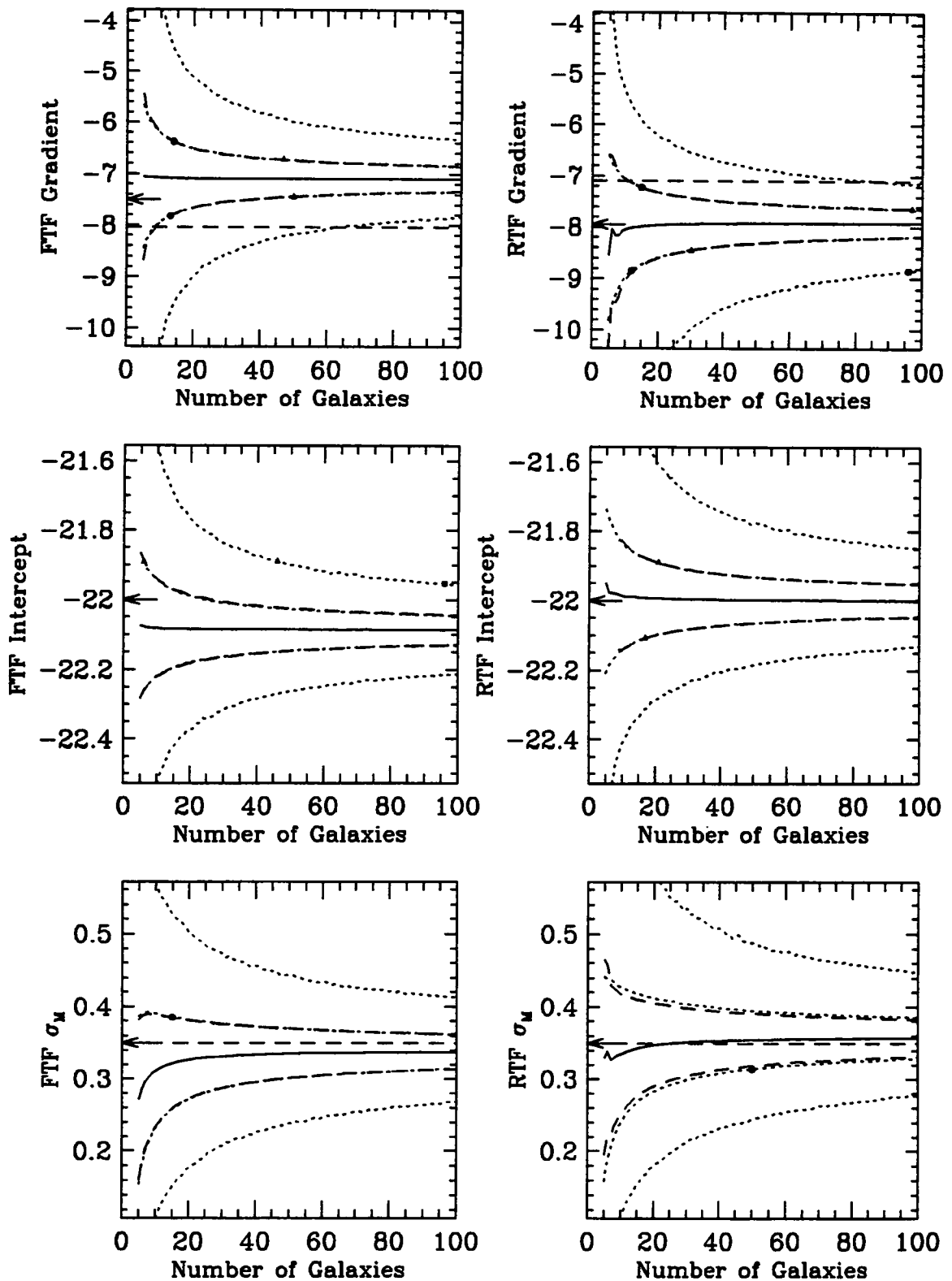
Figure 5.16: Six line plots of output from a Monte-Carlo simulation of the Tully-Fisher fitting procedure for sample sizes ranging from 5 to 100 galaxies. With magnitude selection effects that resemble those depicted in the lower left plot of Figure 5.7. The marked lines and symbols have the same meaning as in figures 5.14 and 5.15. Note that even in the case of strong selection effects, sample sizes of 30 galaxies or over are needed before the amount of bias on the forward regression line becomes significant.
