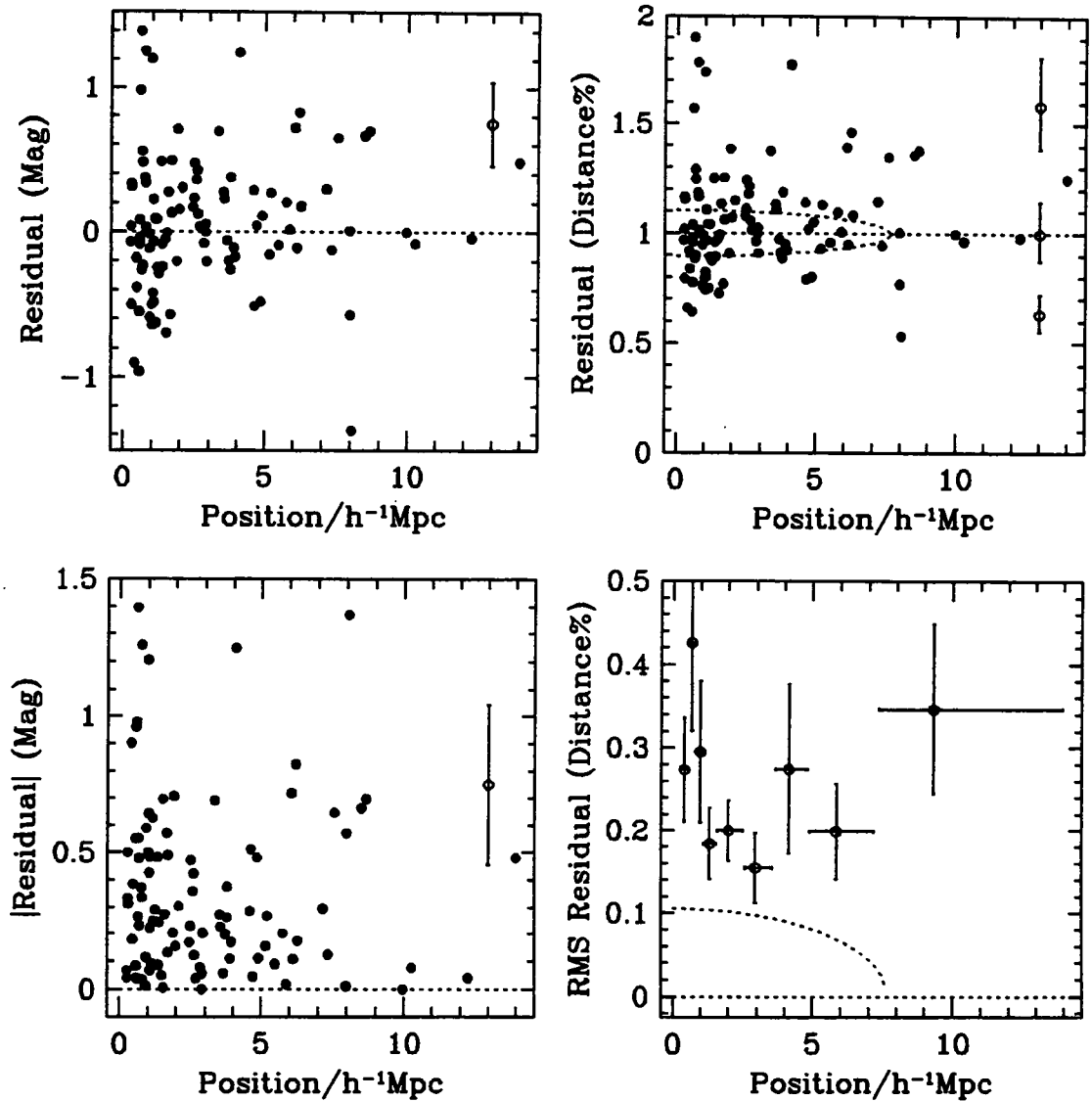
Figure 6.7: A composite plot of all TF fit residuals against radial cluster position in h^{-1}\text{Mpc} for all galaxies in the sample. The lower left-hand plot shows the same data in terms of absolute residuals. The residuals in terms of distance errors are shown in the upper right-hand panel. Marked curves represent the approximate cluster line-of-sight depth in terms of distance. The lower right-hand panel displays the results of binning the data in nine bins each consisting of eleven galaxies. Mean errors are indicated on each plot by an error bar.
