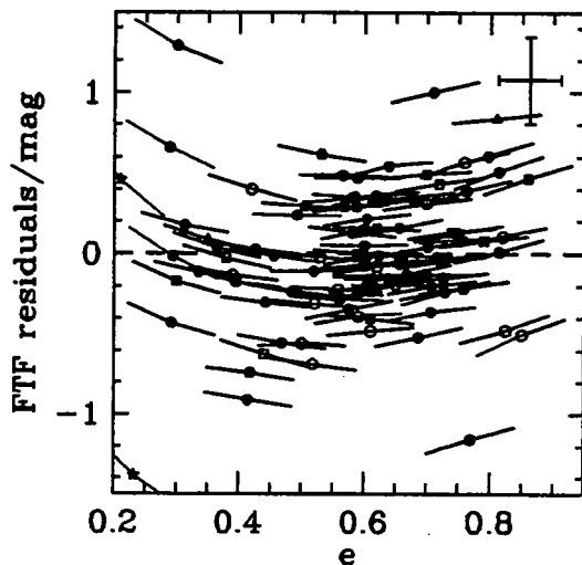
Figure 5.25: A graph of the fit residuals against ellipticity before correction for the effects of internal absorption. The mean errors are marked by a errorbar. The correlation between errors is indicated by a line marked on each point which represents how each point would be shifted by a \pm 1\sigma_e change in ellipticity.
