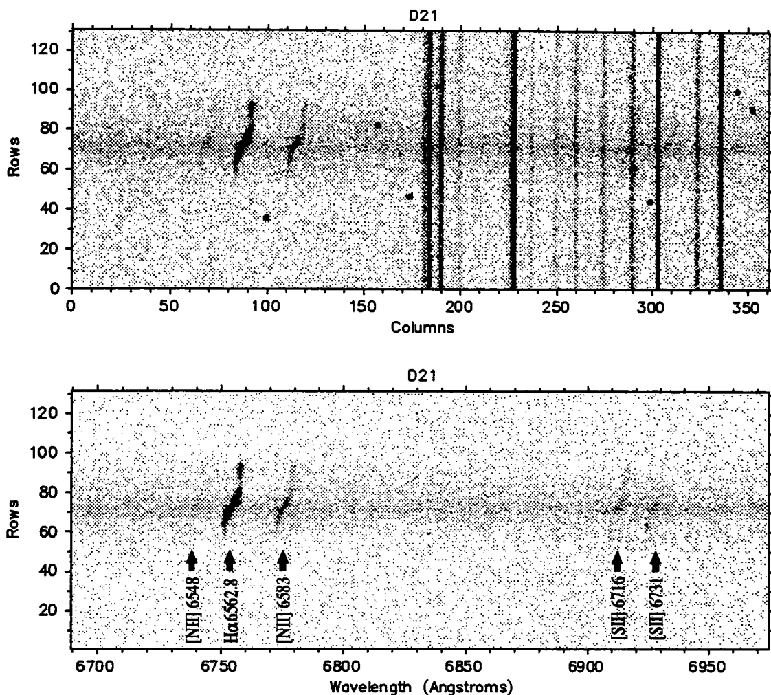
Figure 4.1: Top Image, An example of a “raw” galaxy spectrum. The curved H \alpha and N[II] emission lines can be seen in the left portion of the image along with the faint horizontal continuum light. The vertical lines on the right are emission lines from the night’s sky and the dark points are caused by cosmic rays hitting the CCD. Lower Image, The full reduced version of the same frame, once the sky has been subtracted from the frame and the cosmic rays removed all five of the emission lines can be seen clearly. Also notice the slight reduction in noise compared to the original image which is the result of the flat-fielding process.
