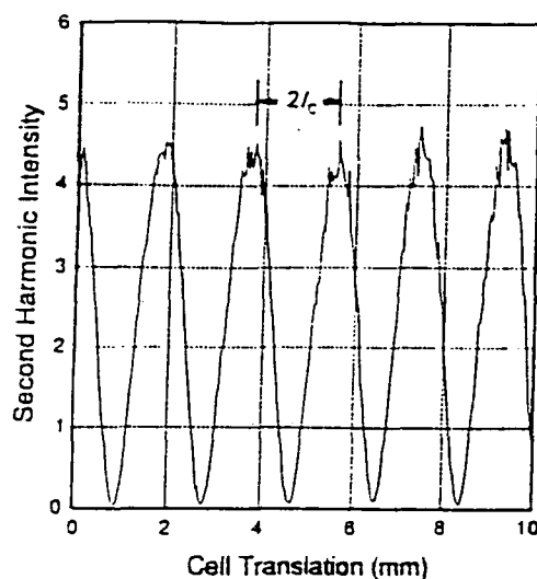
Figure 1.5.2(b) - An example of a wedge fringe pattern (obtained for chloroform) (Prasad & Williams, 1991).
