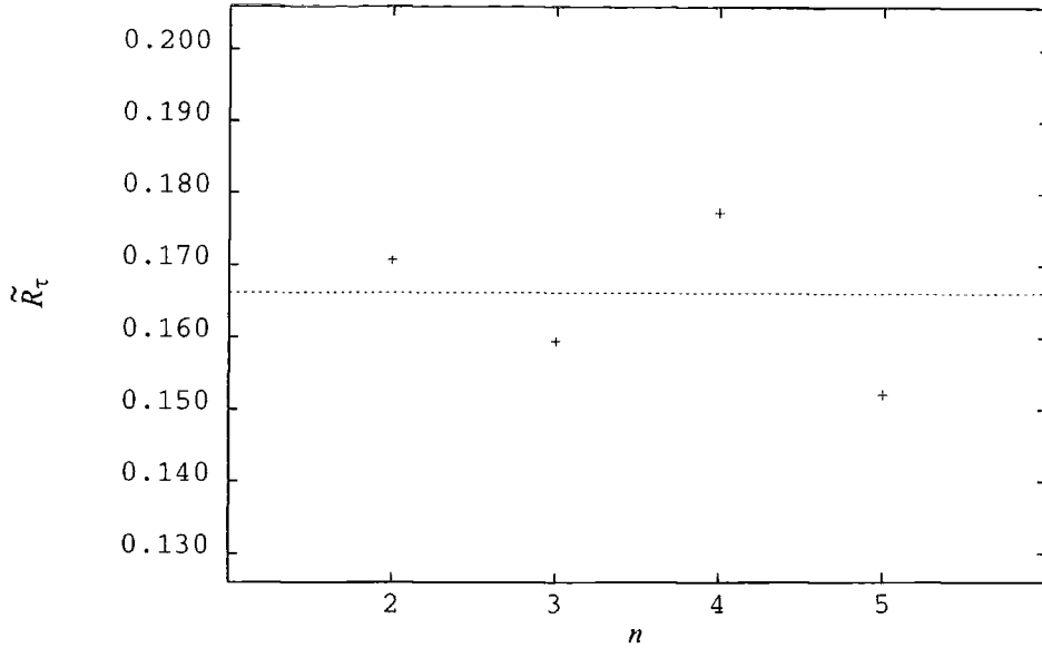
Figure 4.5: Comparison of fixed-order EC perturbation theory (denoted “+”) with the RS-invariant resummation (dashed line) for \tilde{R}_\tau .
