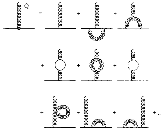
Figure 1.2: The effective quark-gluon coupling is the bare coupling plus loop corrections; only one-loop (NLO) corrections are shown above.
