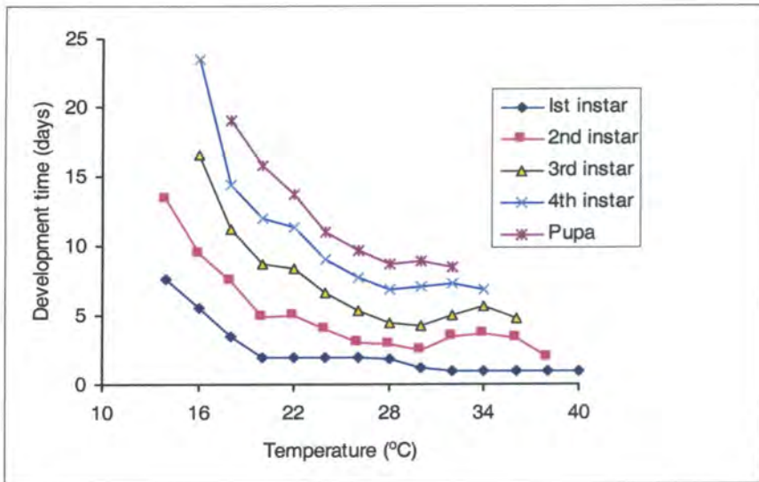
Fig. 3.1 Development times of instar stages of An. gambiae s.s. at different temperatures.
