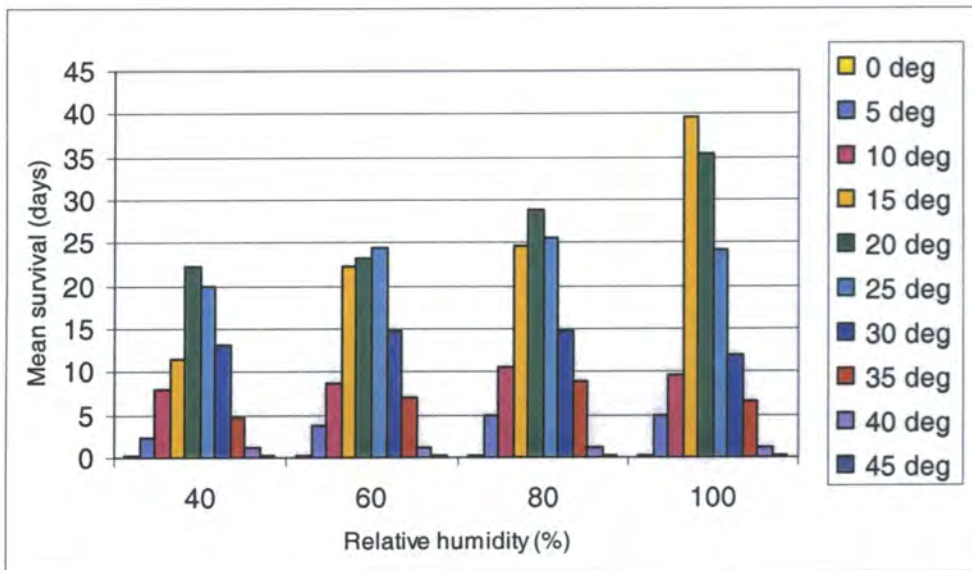
Fig. 6.2 Effect of increasing temperature on the survival of adult An. gambiae s.s. at various humidities.
