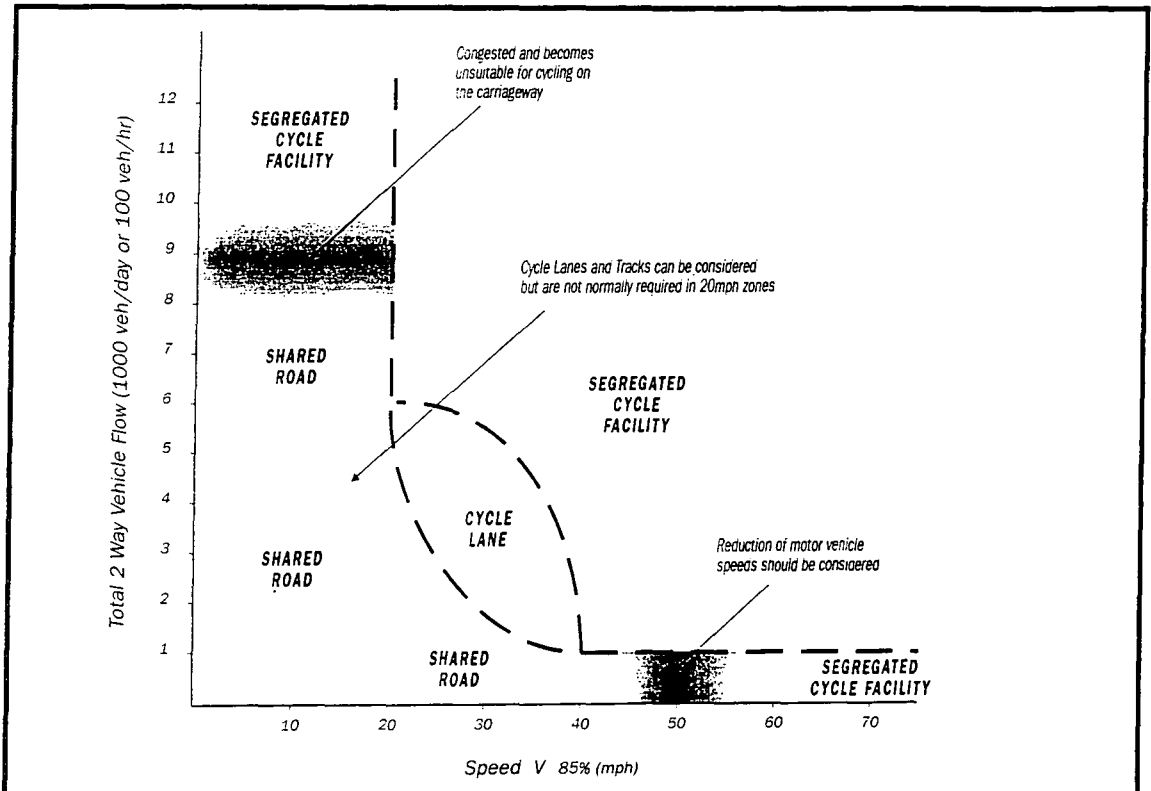
Fig. 5.6 Motorised Traffic Flow and Speed Specification Criteria for Selection of Cycle Facility (After Sustrans, 1996).
