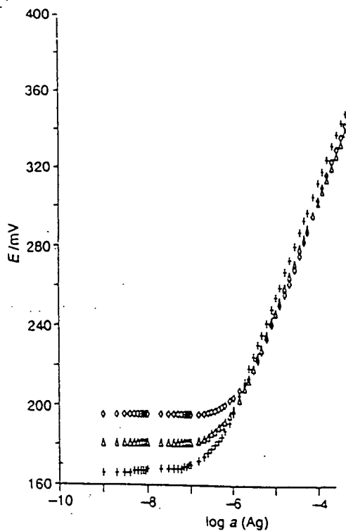
Figure 4.4. Polythia ethers prepared by Casabó 40 and their response to silver 2(+), 3(□) and 4(△)
