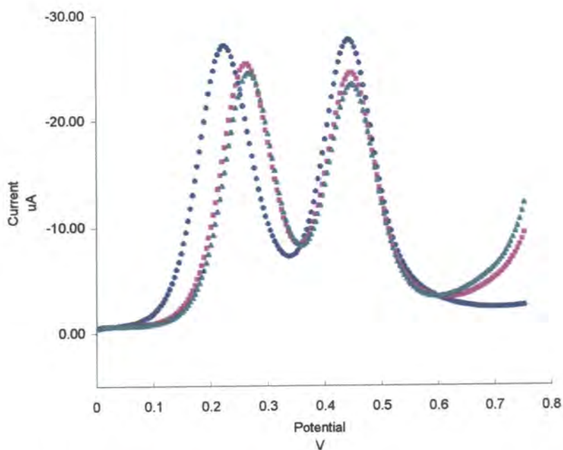
Figure 3.10 Square wave voltammograms of 9 (—) in acetonitrile ( 5 \times 10^{-4} \text{ mol dm}^{-3} ) with the addition of 1 (---) and 3 (····) equivalents of \text{AgNO}_3 .
