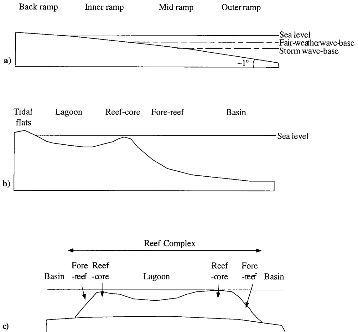
Figure 1-1 Schematic diagrams showing the geometries of carbonate platforms in the study area. a) carbonate ramp b) rimmed shelf c) isolated platform.
