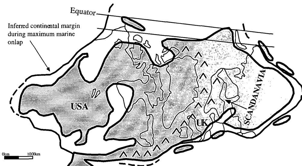
Figure 2-5 Likely palaeogeography for Early Devonian Euramerica (Lochkovian to Emsian). The shaded area indicates the extent of the land mass, \blacktriangle indicates mountains (adapted from Witzke, 1990).
