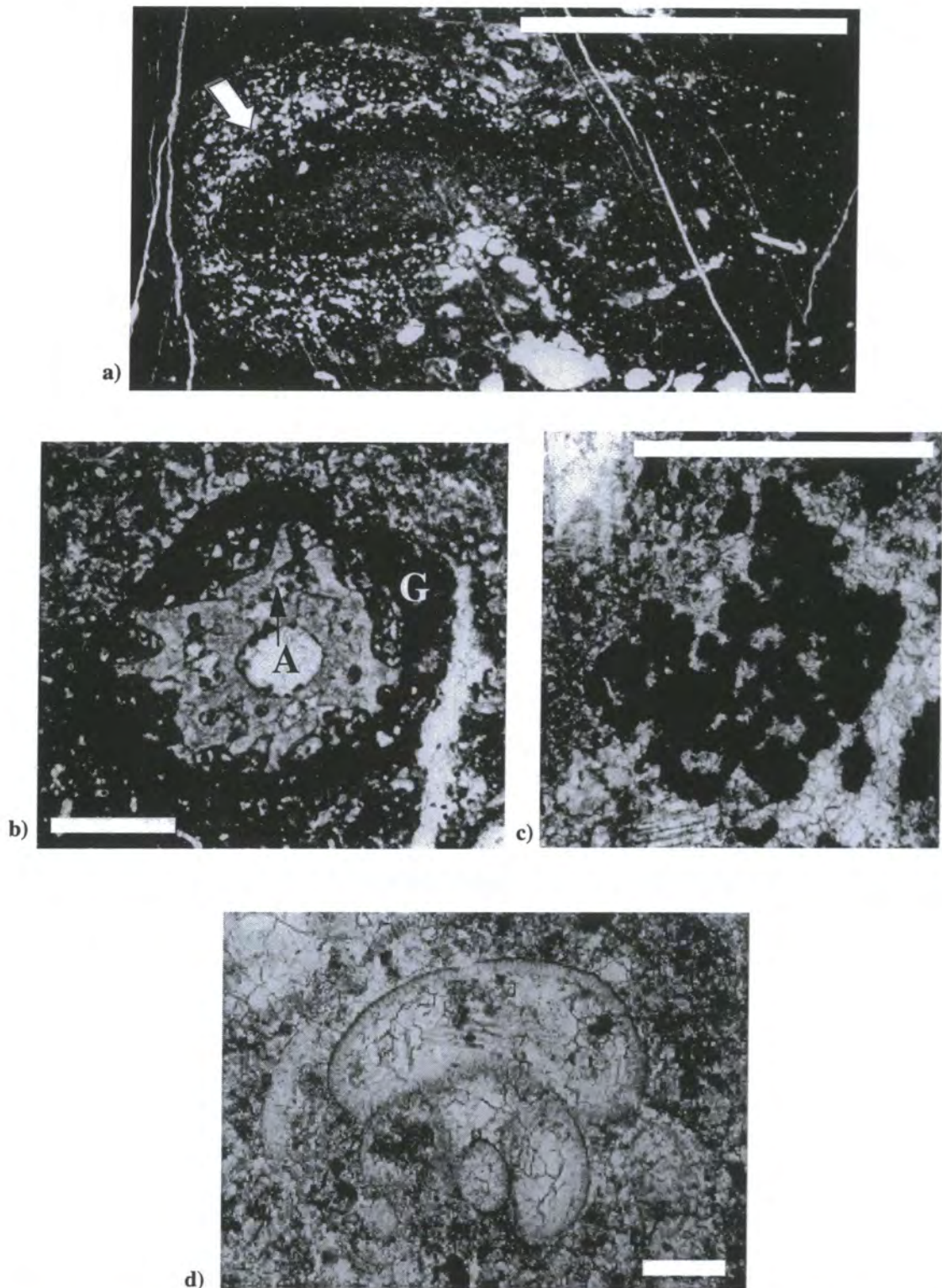
Figure 3-9 a) Photomicrograph of a cyanobacterially-coated oncooid. The cyanobacteria (arrowed) is difficult to identify, yet is likely to belong to the Girvanella group. The nucleus of the oncooid is a micrite lump (M). Sample D6, Dourbes quarry, southern Belgium. Scale bar = 5mm. b) Photomicrograph of Girvanella (G) coating/encrusting an Amphipora branch (A). Sample number BL25, Bleiwäsche quarry, Brilon Reef Complex, Germany. Scale bar = 1mm. c) Photomicrograph of Renalcis/Izhella aggregates displaying inflated hollow chambers. Sample number MB4, Medenbach quarry, Langenaubach Reef Complex, Germany. Scale bar = 1mm. d) Photomicrograph of Wetheredella displaying hemispherical shape and thin micritic walls. Sample number MB18, Medenbach quarry, Langenaubach Reef Complex, Germany. Scale bar = 0.2mm.
