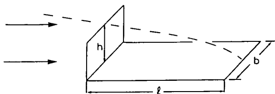
Fig. A1. The calculation from particle trajectories of deposition velocity to a flat plate l , b , length and width of plate; h , height on passing leading edge of plate of that trajectory (shown as broken line) that just strikes trailing edge of plate. Air flow over the plate is indicated by arrows.
