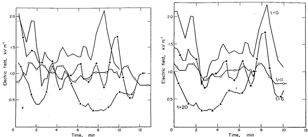
Fig. 6. (i) The variation in electric field at four sites downwind of the stack: 1300 m —; 1650 m —●—●—; 2057 m —○—○—; 2790 m —▲—▲—. Fig. 6. (ii) Electric field variations for the same sites as in Fig. 6 (i). The electric field values are displaced along the time axis by lag number l (unit of 15 seconds) for maximum correction between the sites.
