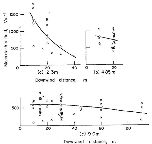
Fig. 5. Mean values (averaged over a 24 min run) of observed electric field at points downwind of an ion source (a) 2.3 m, (b) 4.85 m and (c) 9.0 m above the ground. The typical fair weather electric field upwind of the source is 120 \text{ Vm}^{-1} .
