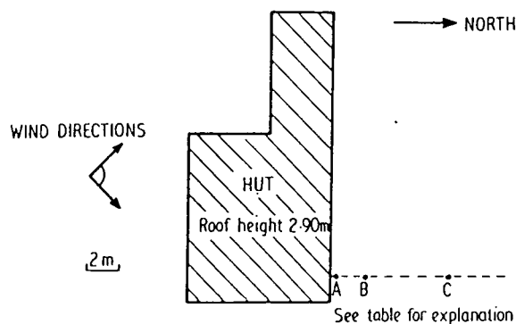
Fig. 1. Arrangements for the continuous source (May 1982) experiments.
