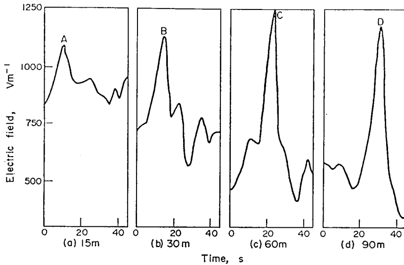
Fig. 3. Simultaneous electric field variations observed at four points on the ground 15, 30, 60 and 90 m in line downwind of an ion source 9 m high. A particular charge distribution travelling with the wind produces peaks A, B, C and D at the corresponding observing points at progressively later times. Mean wind speed = 4.4 \text{ ms}^{-1} .
