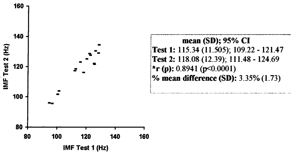
Figure 4.2.12: Repeatability of the IMF of the SMES (extensor channel) from standard grip tests at 2/3 MGS performed 5 minutes apart by 16 female controls.
