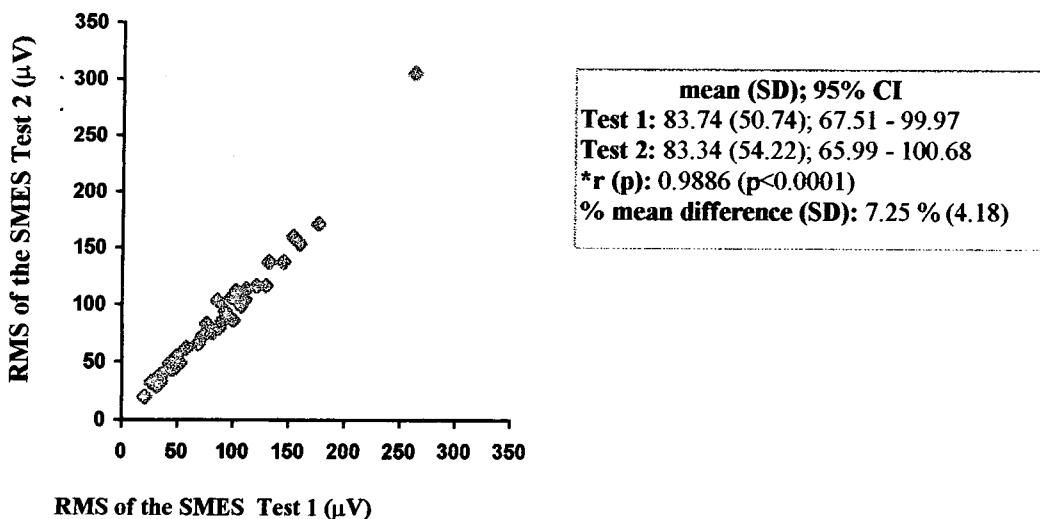
Figure 4.2.5: Repeatability of the RMS of the SMES (extensor channel) from standard grips at 2/3 MGS performed 5 minutes apart by 40 females with RA.
