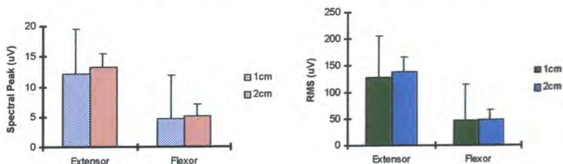
Figure 4.1.8: The effect of IES distance upon the spectral peak and the RMS of the SMES (expressed as the mean (SD)) recorded from the extensor and flexor forearm musculature during standard grip tests at 2/3 MGS by 10 right handed female controls.
