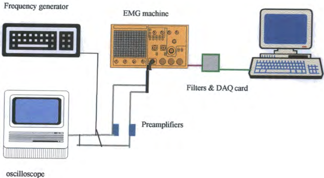
Figure 3.2.1: Calibration of the SMES acquisition and analysis system.
