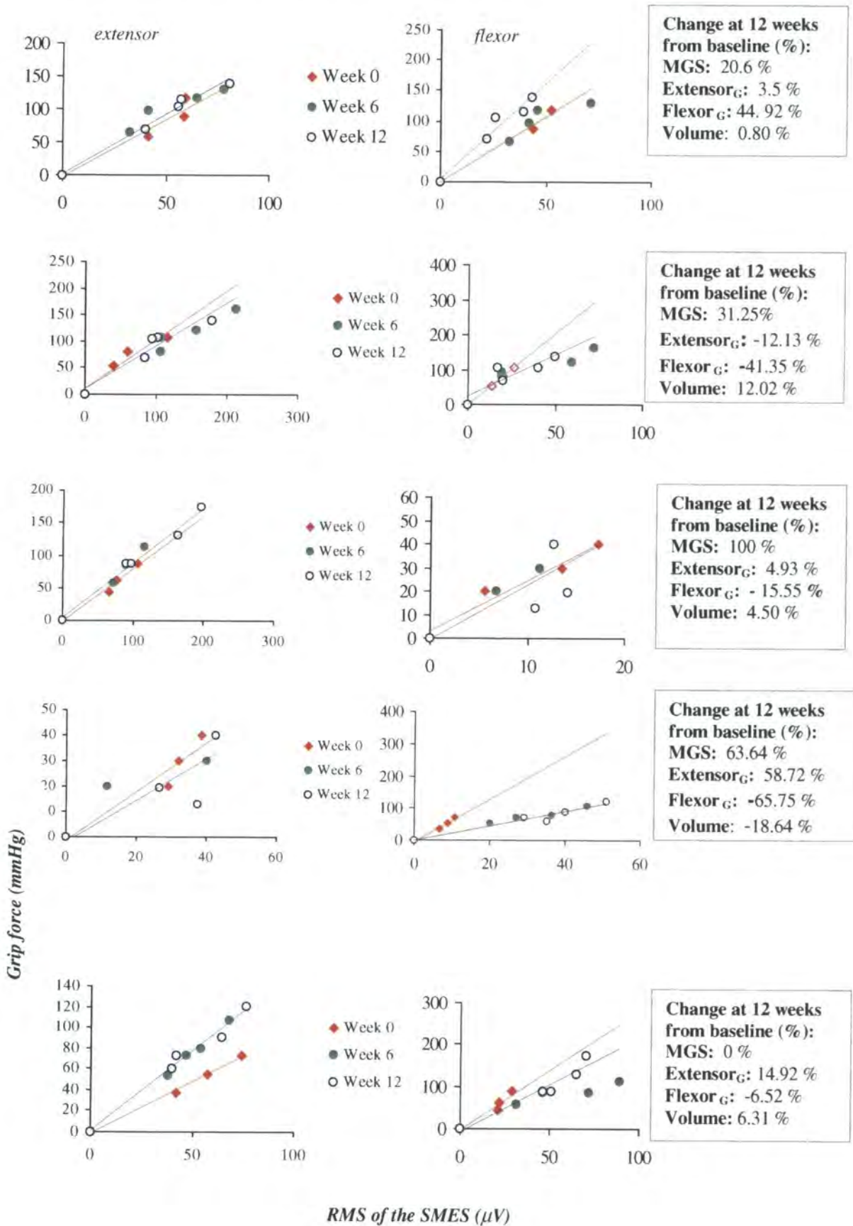
Figures 8.3.6: Grip strength vs RMS of the SMES for extensor & flexor channels in 14 females with RA over a 12-week exercise programme. The % changes in slope of the given regression lines, MGS and forearm muscle volume are given in the associated tables.
