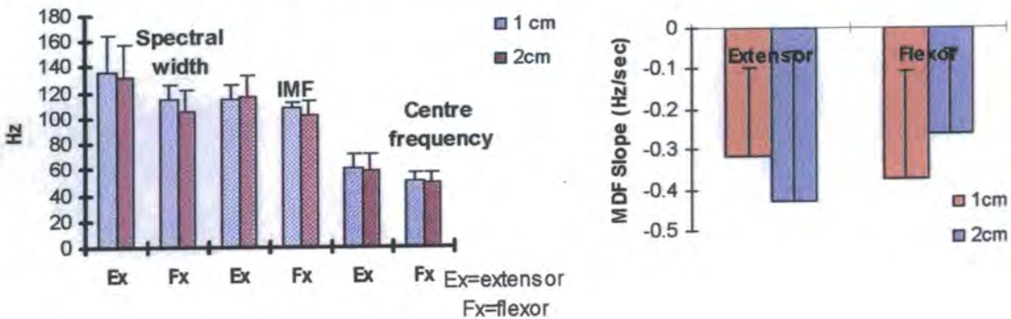
Figure 4.1.7: The effect of IES distance upon spectral parameters (expressed as the mean (SD)) recorded from the extensor and flexor forearm musculature during standard grip tests at 2/3 MGS by 10 right handed female controls.
