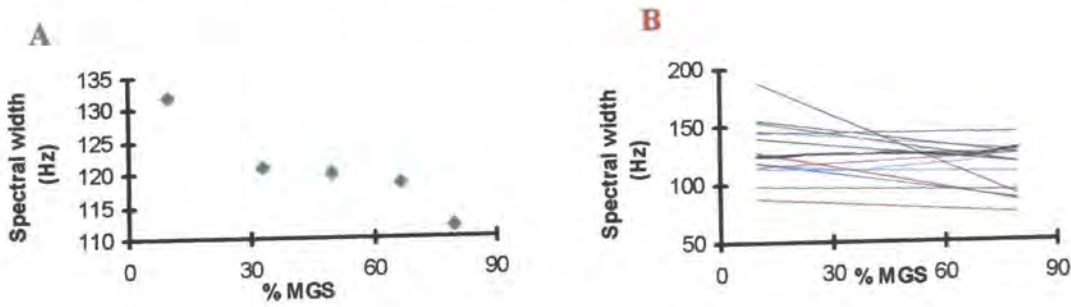
Figure 4.3.8: Mean spectral width (A) and linear regression lines (B) from extensor forearm musculature during standard grip tests versus percentage maximal grip pressure in 17 female controls. ANOVA F = 1.732 ; p = 0.1522 .
