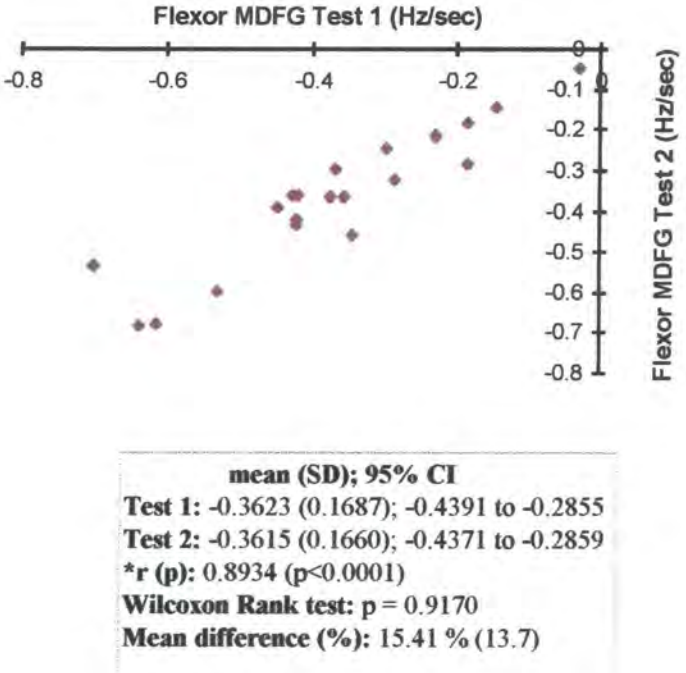
Figure 4.2.24: The repeatability of the MDFG of the SMES (flexor channel) from standard grip tests at 2/3 MGS performed 3 weeks apart by 18 females with RA.
