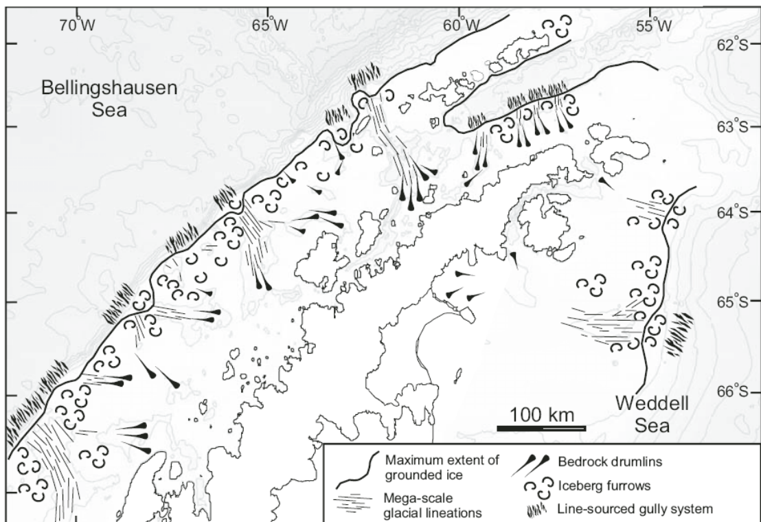
Fig. 2.2 Reconstruction of the geomorphic features mapped on the continental shelf and the resulting reconstruction of the maximum extent of grounded ice around the northern Antarctic Peninsula at the LGM (Source: Heroy and Anderson, 2005)
