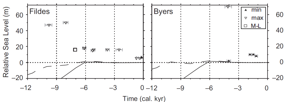
Fig. 2.12 Modelled sea level variations for Fildes Peninsula (King George Island) and Byers Peninsula (Livingston Island). Predictions are based on the reference earth model and two end member meltwater pulse-1A scenarios (both tuned to fit the Barbados sea level record): a sole northern hemisphere contribution (dashed line) and a dominant Antarctic contribution (solid line). Under either scenario the model predictions fail to match the observed RSL response to deglaciation. The symbols identify the type of sea level constraint; shells are interpreted as minimum sea level constraints, whereas seal hairs, penguin guano and remains in ornithogenic soils provide maximum sea level constraints. Isolation basins provide a 'fix' for sea level and are labeled as marine-lacustrine (M-L) (Source: Bassett et al. , 2007)
