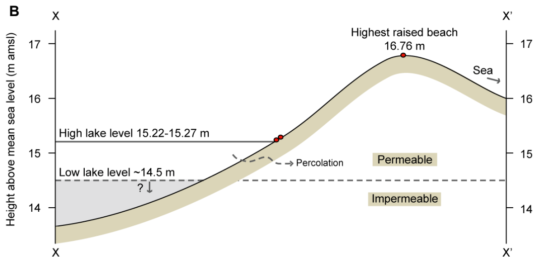
Fig. 3.6 Calculation of the sill height at Yanou, (a) GPS data from the catchment with implications on the sill height (all heights are metres above mean sea level; (b) schematic cross section across X-X' showing the high and low lake levels with respect to the height of the highest raised beach; (c) photograph showing the difference between high and low lake levels, taken at the site where the GPS lake level measurements were taken (rucksack on the high lake level for scale).
