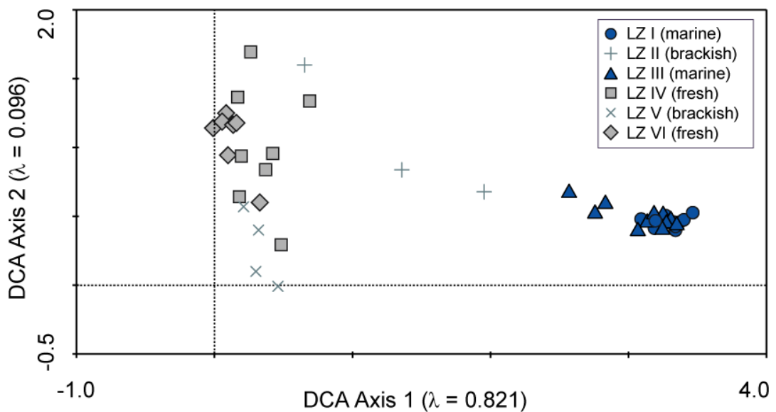
Fig. 4.7 Detrended correspondence analysis of samples from Long Lake. Samples plotting close to one another have similar diatom compositions. Eigenvalues ( \lambda ) are a measure of the importance of ordination axes.
