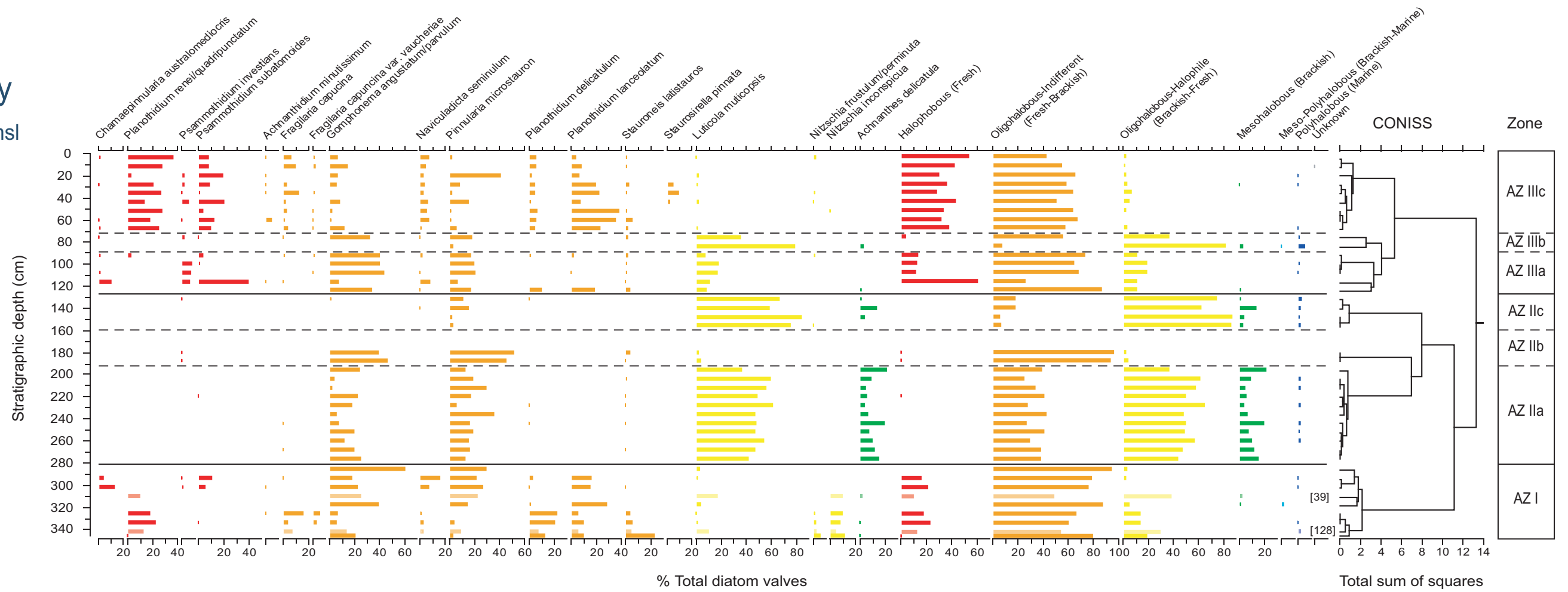
Fig. 4.9 Diatom assemblage of Ardley Lake. Species are grouped by salinity tolerance. Only species >5% of the total valves counted are shown. Where diatom concentrations were too low to achieve a full count of 250 valves, counts are shown as paler bars and the number of valves counted is shown in brackets
