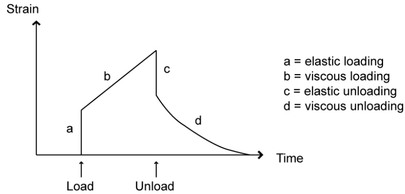
Fig. 5.3 Response of a viscoelastic material to loading
