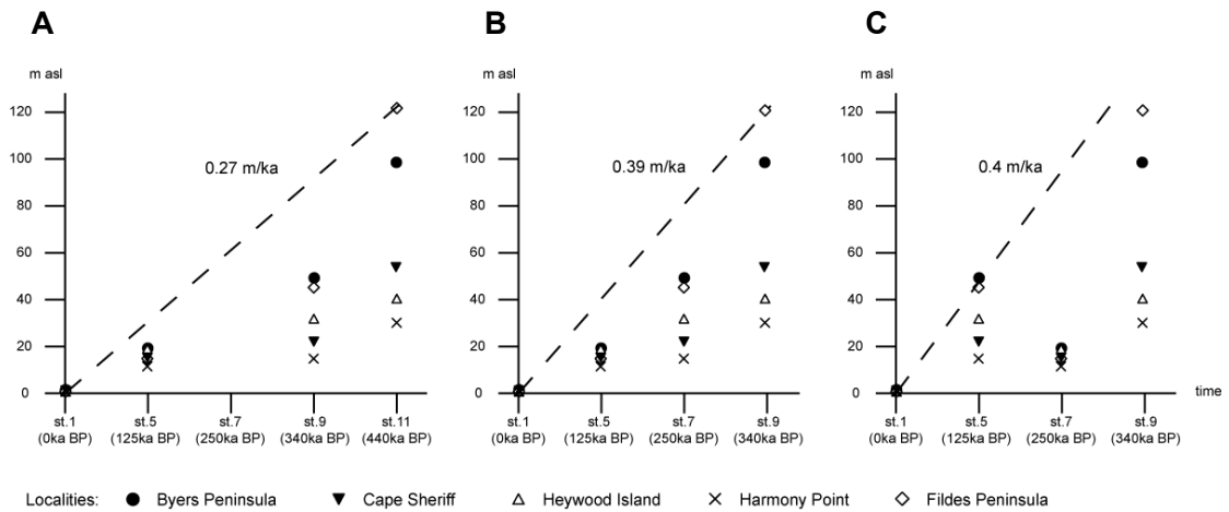
Fig. 7.11 Predicted tectonic uplift rates for the SSIs according to Pallàs et al. (1997), based on the assignment of the ages of the most recent interglacials to sets of emerged platforms, (a) assuming platforms formed during marine isotope stages (MIS) 1, 5e, 9 and 11; (b) assuming MIS 7 was also a time of platform formation; (c) assuming platforms of MIS 7 are below those of MIS 5e.
