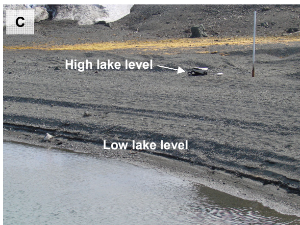
Fig. 3.6 Calculation of the sill height at Yanou, (a) GPS data from the catchment with implications on the sill height (all heights are metres above mean sea level; (b) schematic cross section across X-X' showing the high and low lake levels with respect to the height of the highest raised beach; (c) photograph showing the difference between high and low lake levels, taken at the site where the GPS lake level measurements were taken (rucksack on the high lake level for scale).
