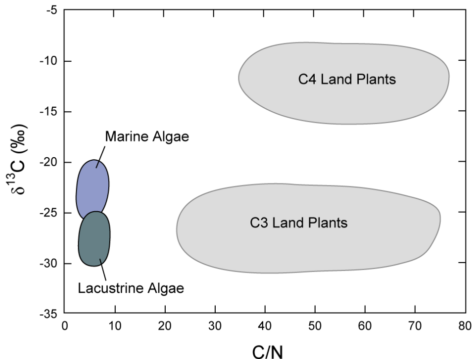
Fig. 3.17 Elemental (atomic C/N ratio) and isotopic ( \delta^{13}\text{C} value) identifiers of bulk organic matter produced by marine algae, lacustrine algae, \text{C}_3 and \text{C}_4 land plants (Redrawn from Meyers, 1997)
