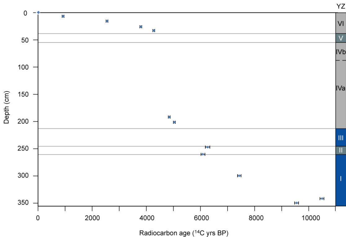
Fig. 4.4 Depth versus radiocarbon age (uncalibrated) for the Yanou core. Error bars are shown to 1-sigma. The five lowermost dates have been corrected using the marine reservoir correction of 1064 \pm 10 yrs, reported for Maxwell Bay by Milliken et al. (2009) (details on reservoir correction are given in the caption to Table 4.2).
