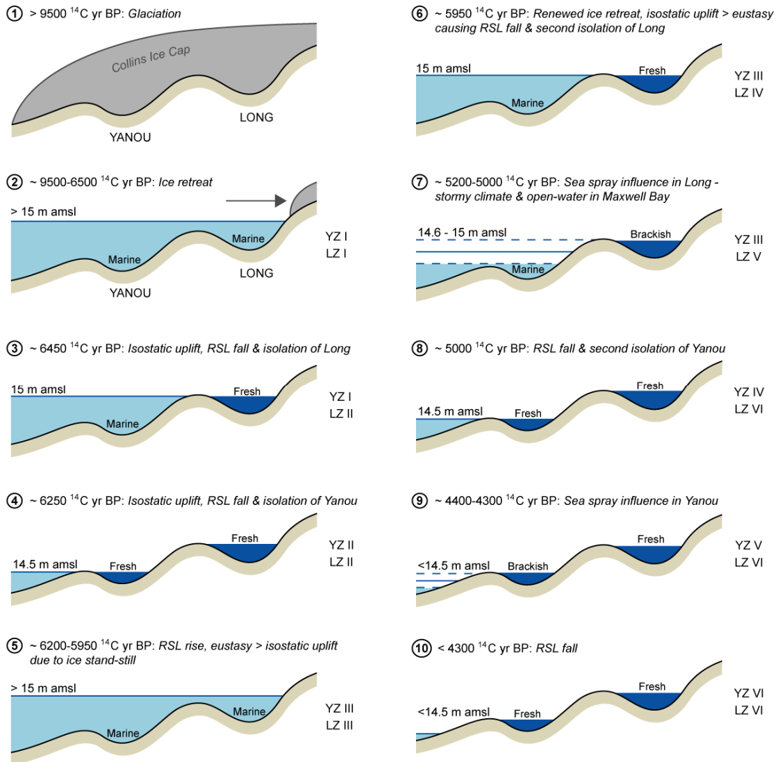
Fig. 5.7 Schematic representation of the isolation process at Long and Yanou lakes with RSL interpretations and the correspondence to the zones identified from diatom, isotope and physical analyses
