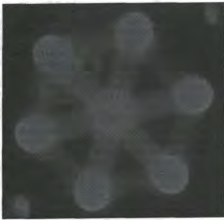
Figure 7.14: Photograph of the back projected pupil image formed by the input microlens array. The central pupil is that which corresponds to the telescope secondary. The other pupils project onto the sky. If the IFU were unbaffled then the fibres would receive background sky contamination from these areas on the sky. Note the diffraction spikes and the blurring of the pupil image edge.
