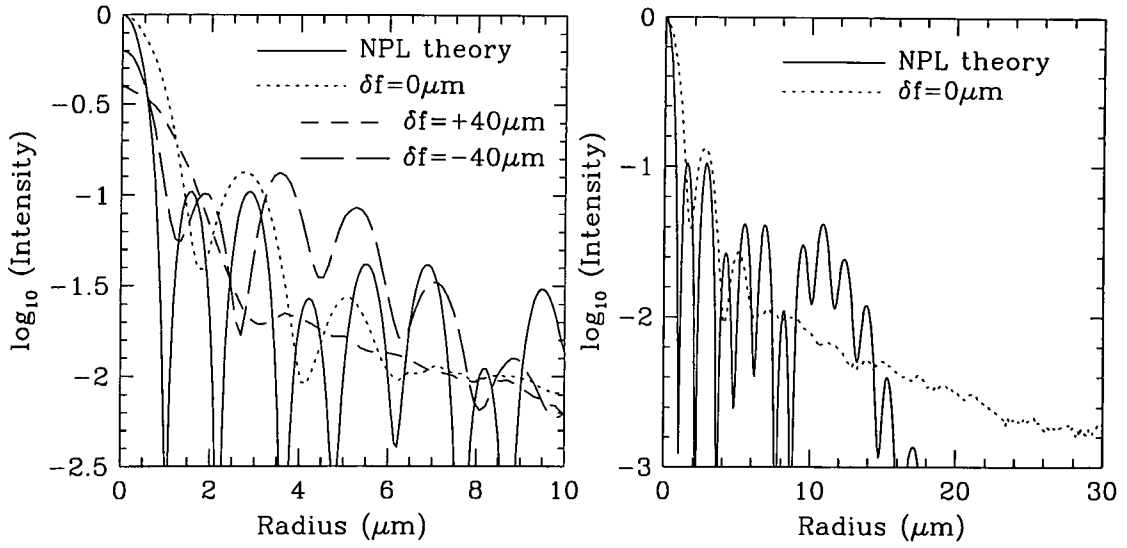
Figure B.1: Point spread function of NPL microlens test array taken with \times 100 magnification. The labelled focus positions, \delta f , are measured relative to the MCI focus. The psf shows the radius of the Airy disk is \sim 1.5\mu\text{m} which is in agreement with the predicted value of 1.5\mu\text{m} . May need to include diffraction limit in this plot.
