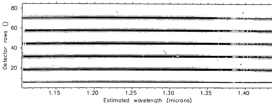
Figure 8.15: J-band magnification set-up mask exposure taken with the ‘big-mask’ design described in section 8.2.3 and shown in figure 8.4. Each spectrum is due to approximately two adjacent IFU elements being illuminated. As well as measurement of magnification the spectra can be used to calibrate the image distortions of CGS4 and the variation in spatial PSF with detector position.
