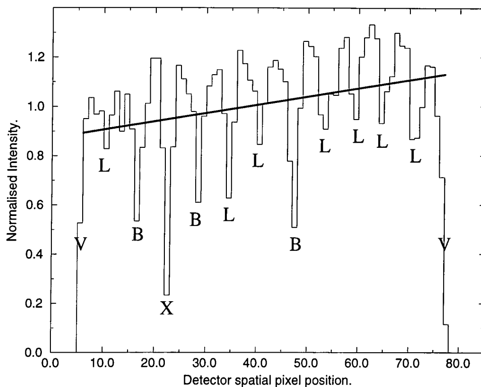
Figure 8.7: Cut along the spatial direction of the fibre to fibre dome flat-field image shown in figure 8.5. The letters indicate the following: V = vignetted pixels, B = bad fibres, X = broken fibre, L = low throughput fibres. The solid line shows the best fit to the intensity in (\text{Intensity} = 0.00334x + 0.873) the area occupied by the fibres. The fit shows there is a considerable gradient across the flat-field. The intensity increases by 24% from left to right although this may be slightly biased by the bad fibres being predominantly on one half of the detector.
