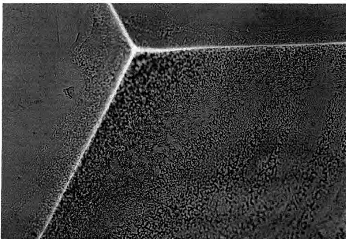
Figure B.8: Reproduction of a microphotograph of the SAURON microlens array surface taken with a microscope and a 35mm camera attachment. The severe marking (orange peel) on the surface of the lens is evident. This is thought to be the cause of the high scattered light and image quality obtained with this lens. The surface defects are worse in the corners than the centre of the lens.
