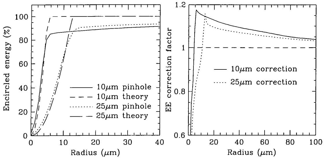
Figure 6.16: The left plot shows a comparison of the theoretical EE curve for a pinhole and the observed EE curve. The right plot shows the ratio obtained by dividing the theoretical EE curve by the measured EE curve.
