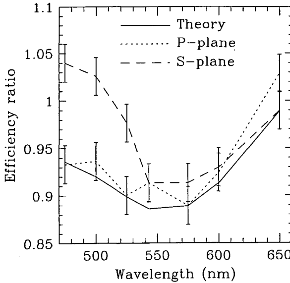
Figure 3.10: Plot to show the ratio of immersed to un-immersed grating absolute efficiency curves in Littrow configuration (adapted from figure 3.9). The ratio has been corrected to remove the effect of air-glass losses at the prism surface. Also shown is the theoretical prediction obtained from the change in reflectivity of an immersed Aluminium surface.
