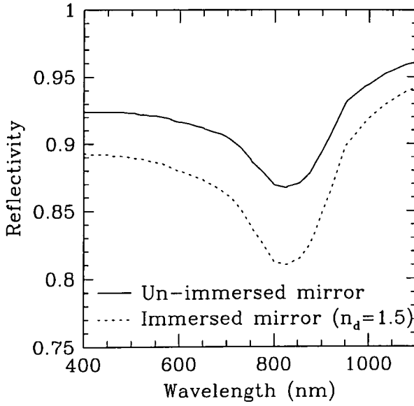
Figure 3.11: Plot of the reflectivity of an Aluminium surface versus wavelength for unpolarized light. The angle between the incident and reflected beams is 45^\circ . Two curves are shown, the curve with higher reflectivity is for front surface reflection, and the lower curve is when the surface is immersed in a medium of refractive index equal to 1.5.
