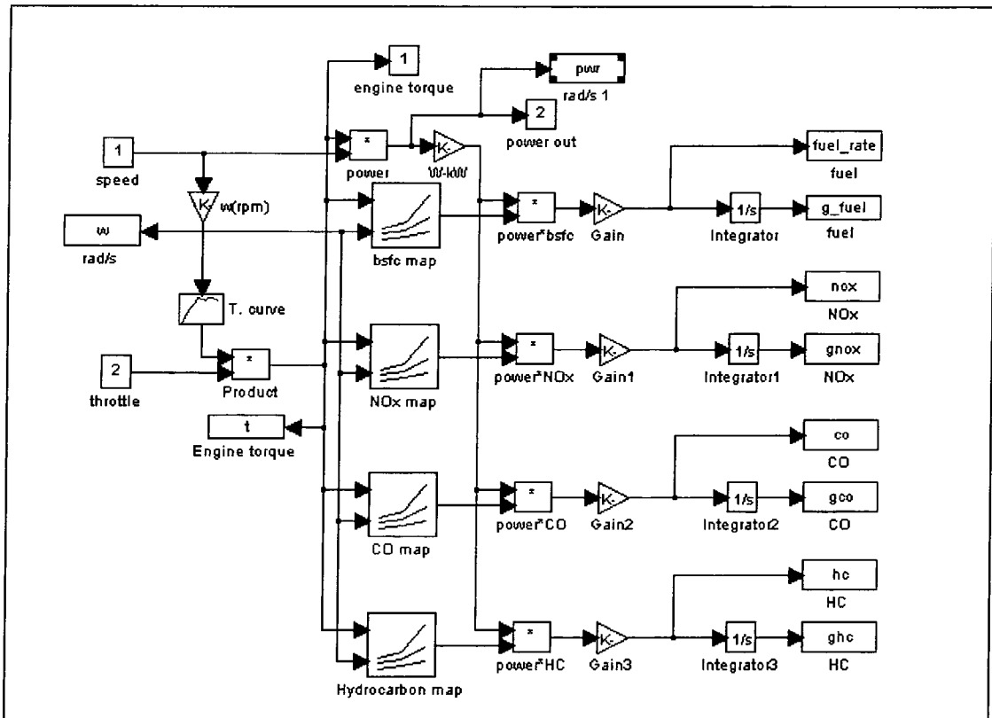
Figure3. 6 The Structure of the Series Hybrid Vehicle Engine
