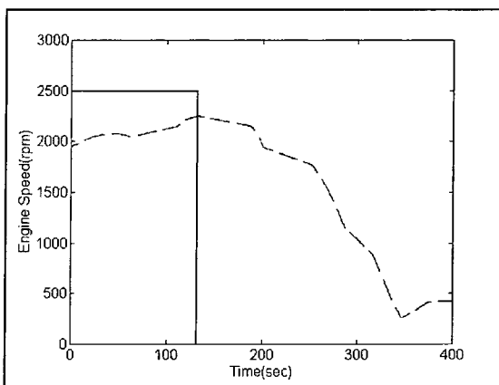
Figure 6.12 Engine Speed Result
