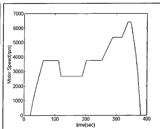
Figure 6.9 Motor Speed Result
