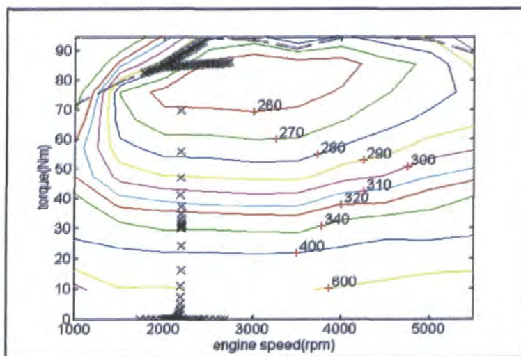
Figure 7.11 Reduced Engine (without Throttle Limit)
