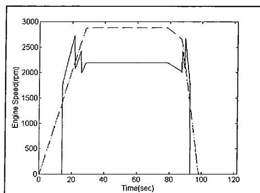
Figure 7.9 Engine Speed Result
