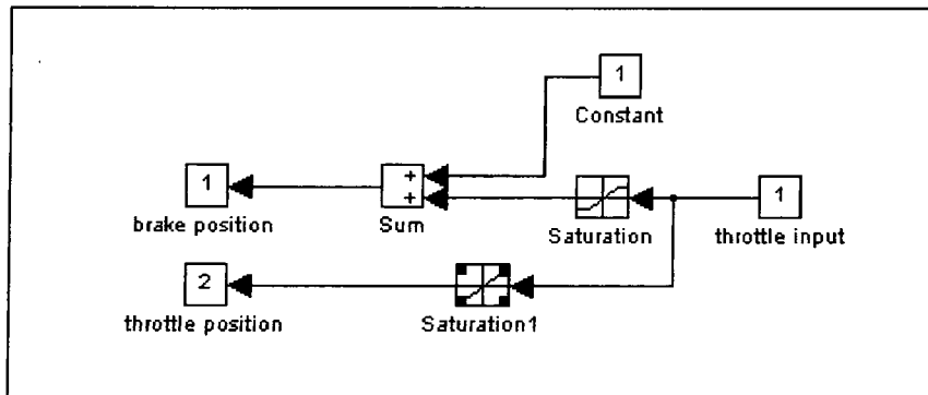
Figure 5.2 Throttle Controller
