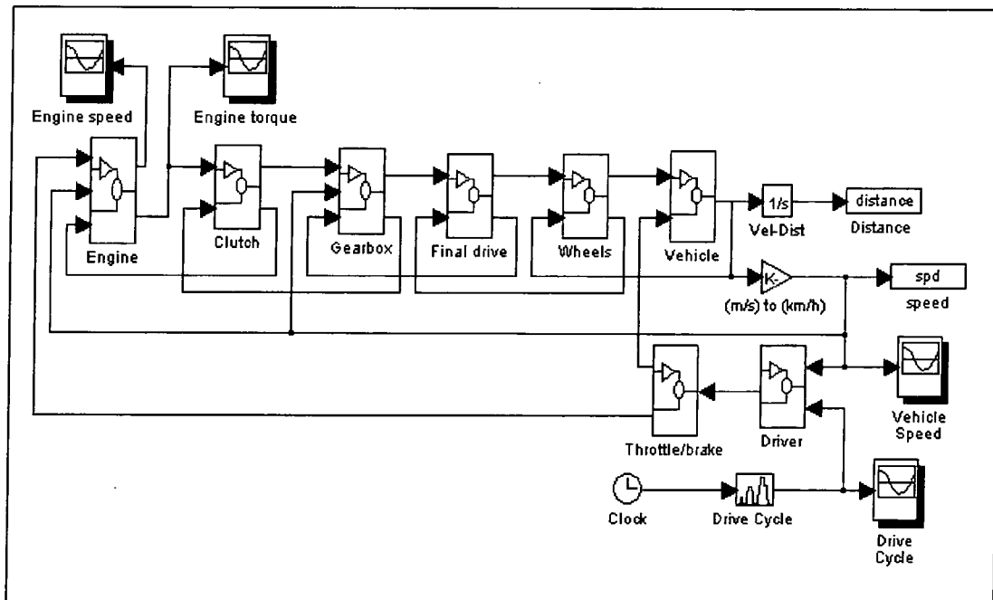
Figure 4. 2 IC Engine Vehicle Model
