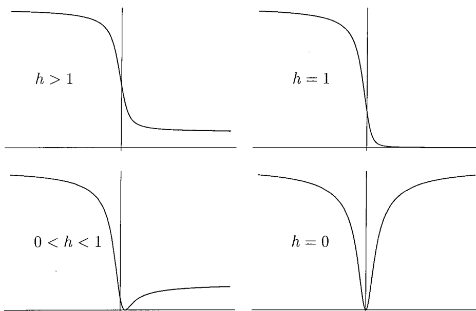
Figure 4.11: One dimensional potential V(r) (vertical axis) versus r (horizontal axis). For a given h , the mirror image of V(r) with respect to the vertical axis gives V(r) for -h .
