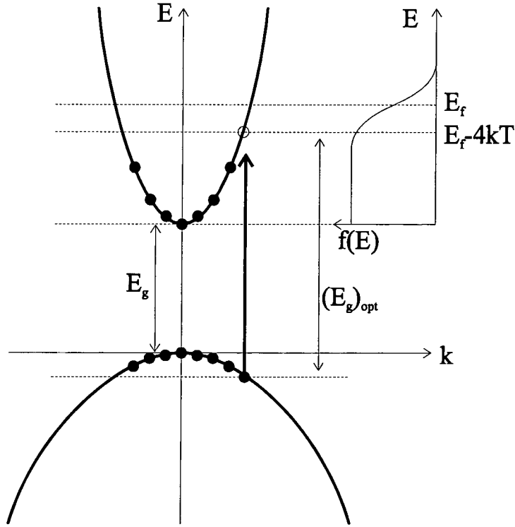
Figure 28: The Moss-Burstein Shift
