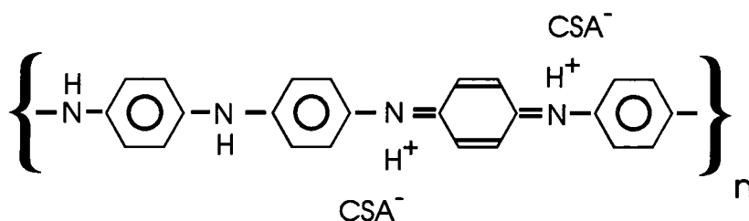
Figure 36: Polyaniline camphor sulfonic acid
