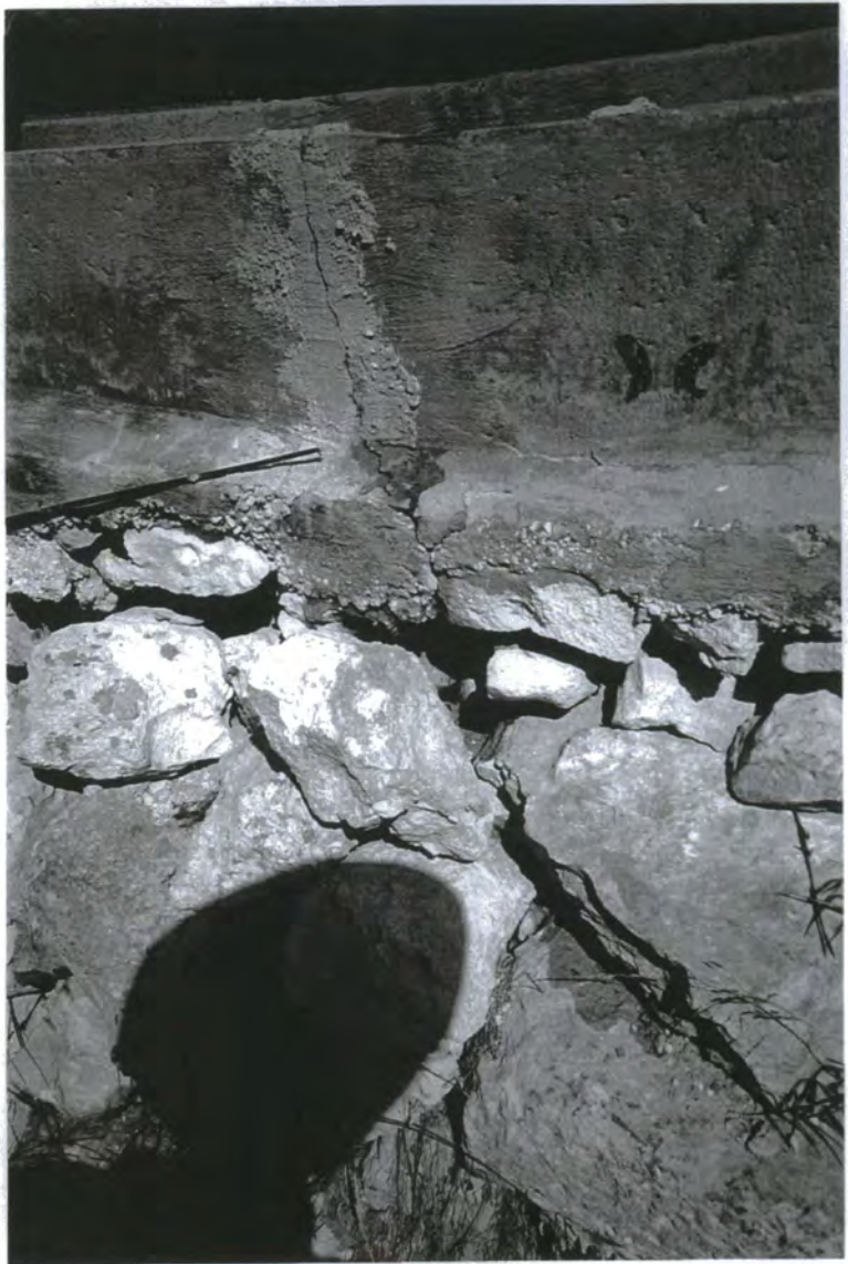
Plate 5.8. A small leak which is difficult to detect and represents a large water loss.
