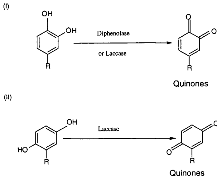
Figure 1.5 A Reaction of polyphenol oxidase and laccase with phenol. (I) Diphenolase action by polyphenol oxidase or laccase. (II) Action of laccase on p-diphenol.
