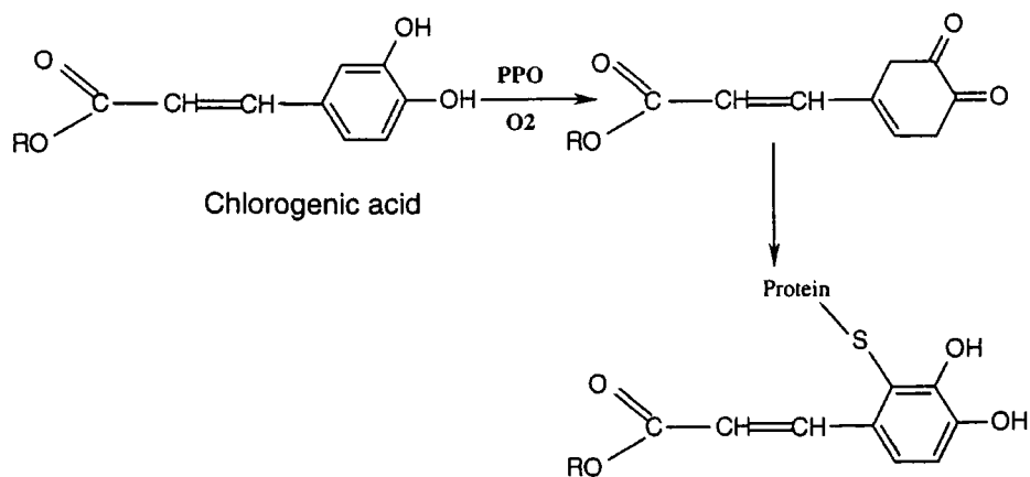
Figure 1.5 B Oxidation of chlorogenic acid and subsequent alkylation of proteins. PPO = polyphenol oxidase; S = thiol.
