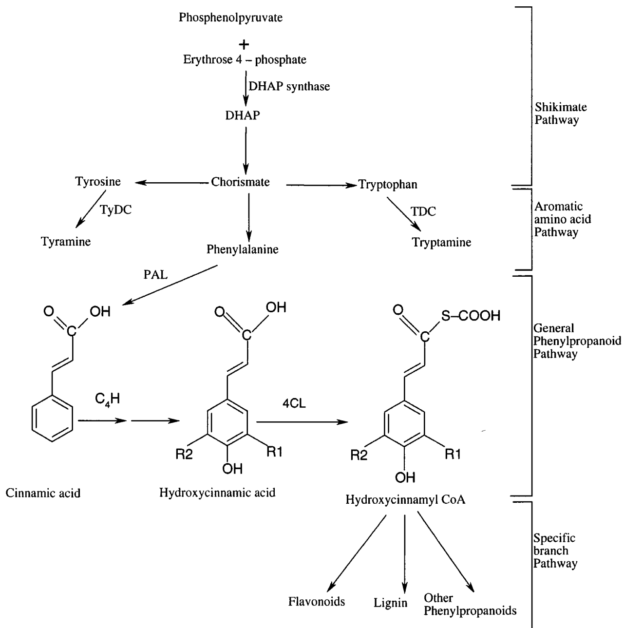
Figure 1.7 Overview of carbon flow in secondary metabolism in plants. The basic steps in the shikimate aromatic amino acids, general phenylpropanoid and specific phenylpropanoid branch pathways are indicated. The metabolic intermediates and end products are shown. Abbreviations: R1 & R2 group on hydroxycinnamic acid may be hydroxyl and/ or methoxyl groups; TyDC, tyrosine decarboxylase; TDC, tryptophan decarboxylase; PAL, phenylalanine ammonia lyase; C 4 H, cinnamyl-4-hydroxylase; 4CL, 4-coumarate: CoA ligase. (Adapted and redrawn from Douglas, 1996).
