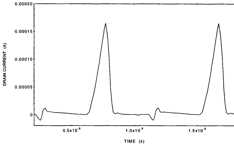
Figure 5.4 (a) Drain current for device N5 of DL1 during the simulation cycle (Process EC/3, Device 1/0.8)
