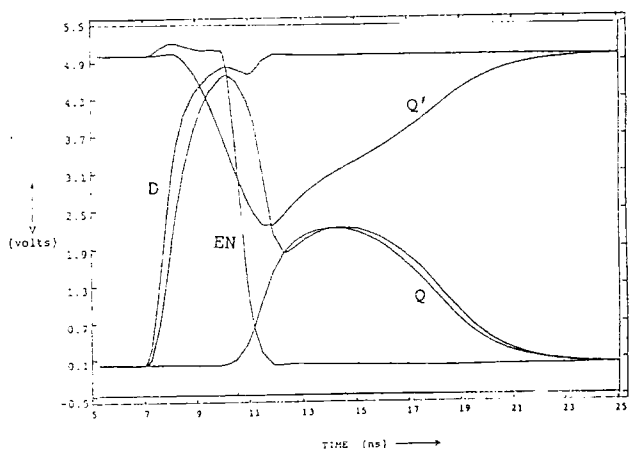
Fig 8. Metastable simulation for TX-NOR
