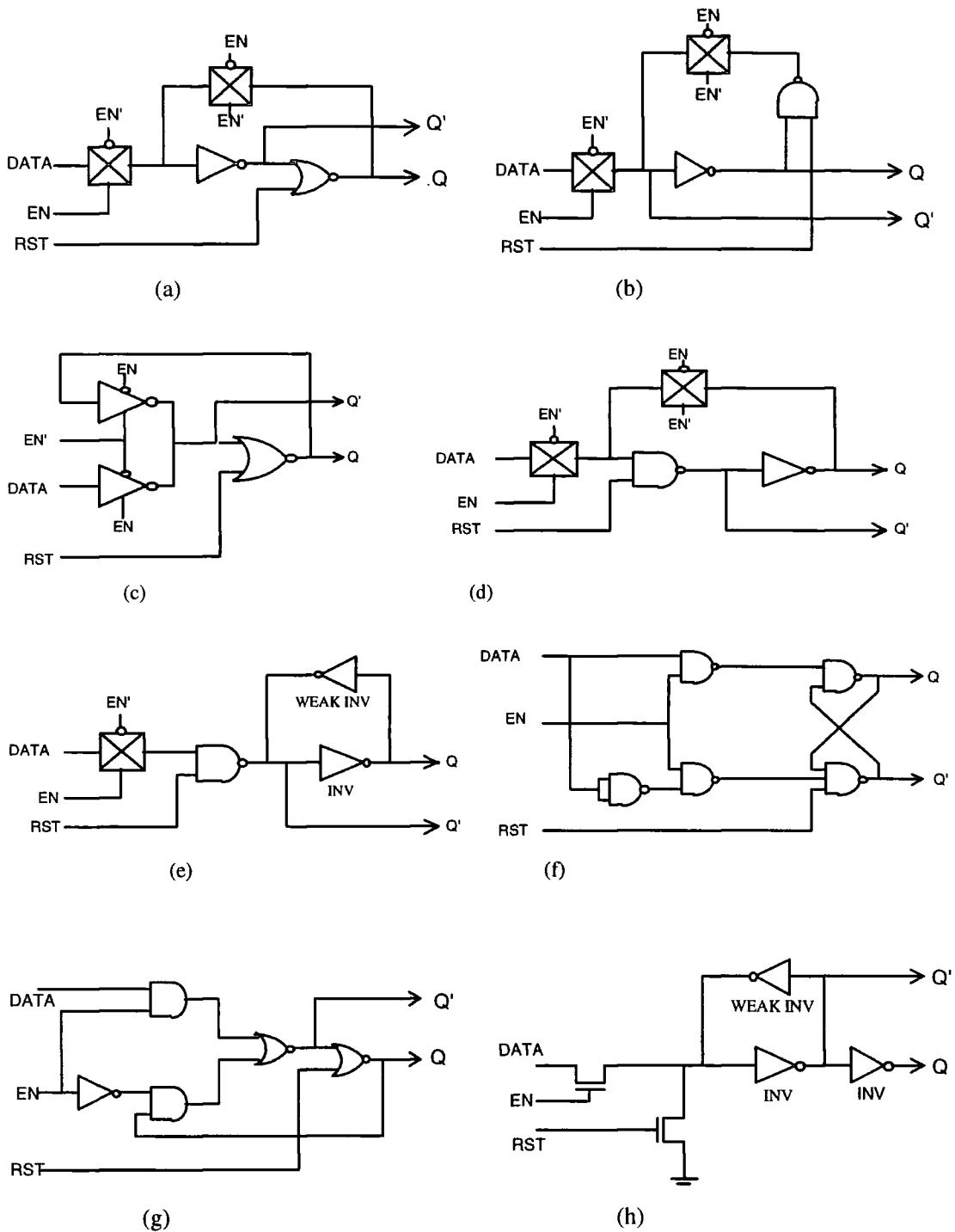
Figure 4.1 D-latch circuits
