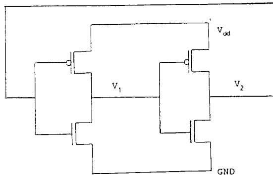
Fig 3. Transistor level circuit for the latch
